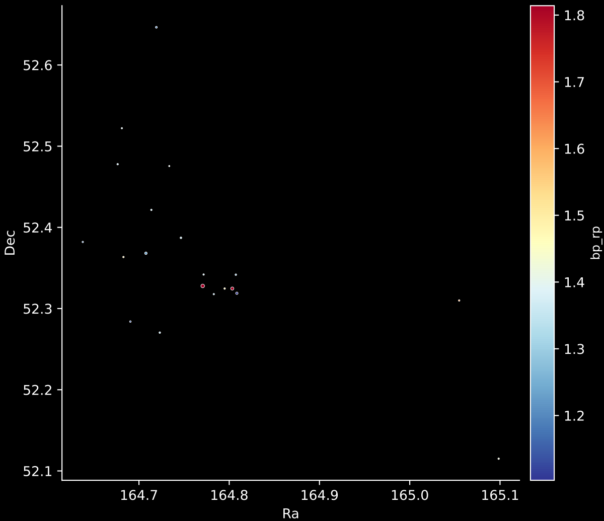
Stars: 20
