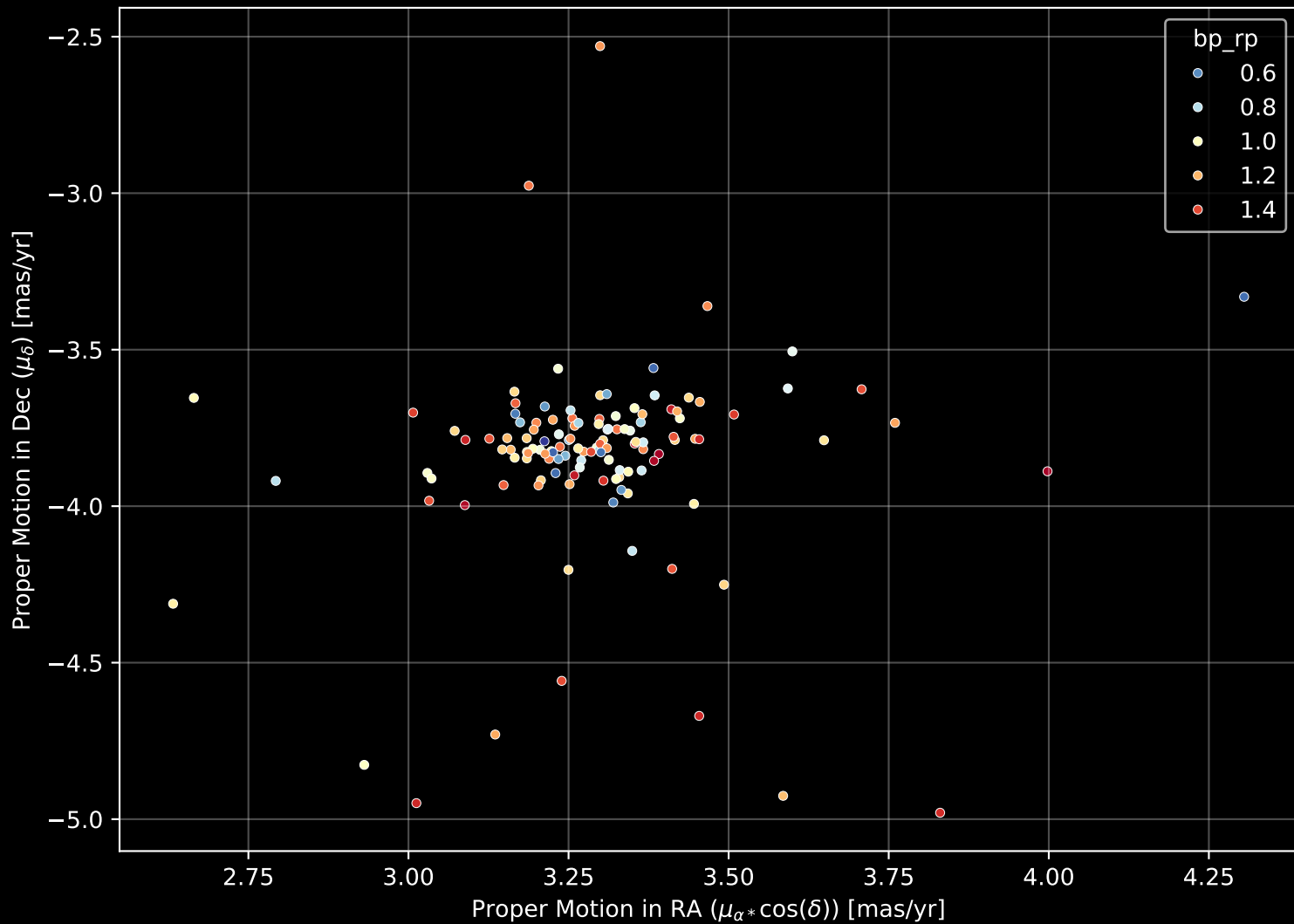
Gaia Cluster: [UBC_54] Proper Motion Diagram (n= 125)
