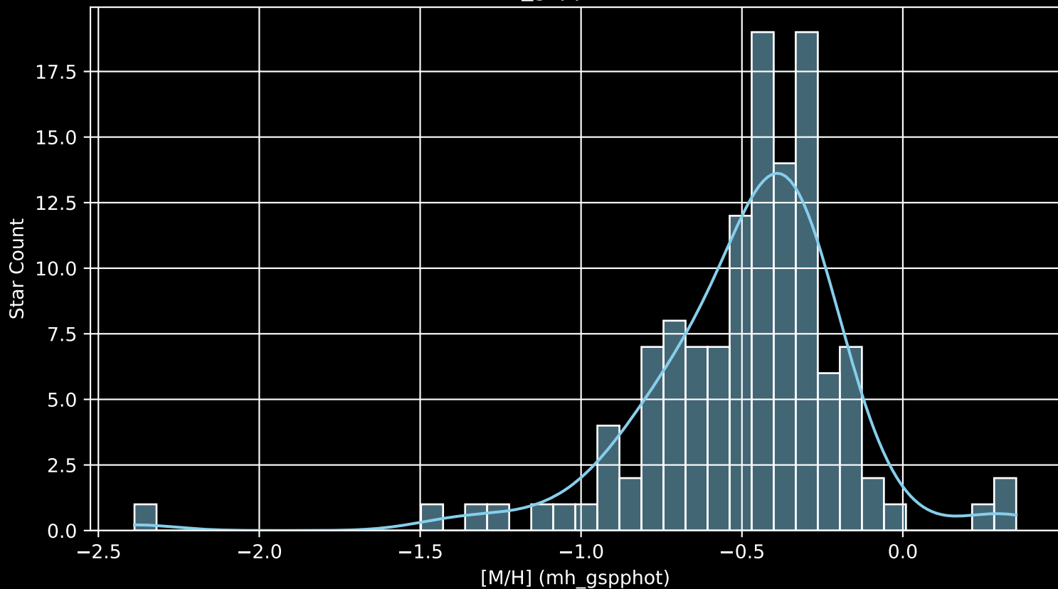
Gaia Cluster: [UBC_54 [M/H] (mh_gspphot) (n= 125)
