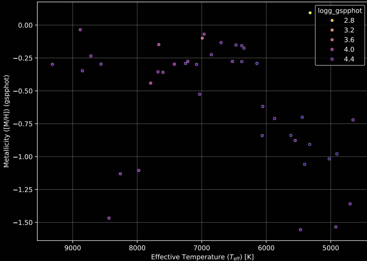
Gaia Cluster: [UBC_61] Stellar Population Parameters (n= 42)
