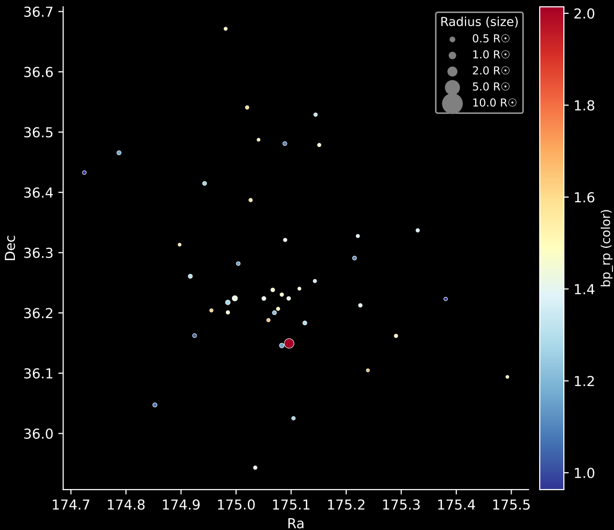
Gaia Cluster: [UBC_61] Stars: 42
