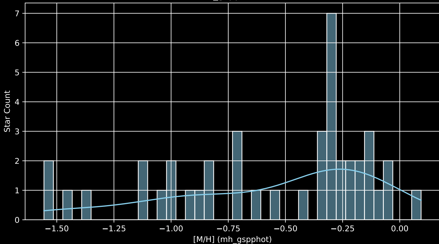
Gaia Cluster: [UBC_61 [M/H] (mh_gspphot) ( \bar{n}= 42 )
