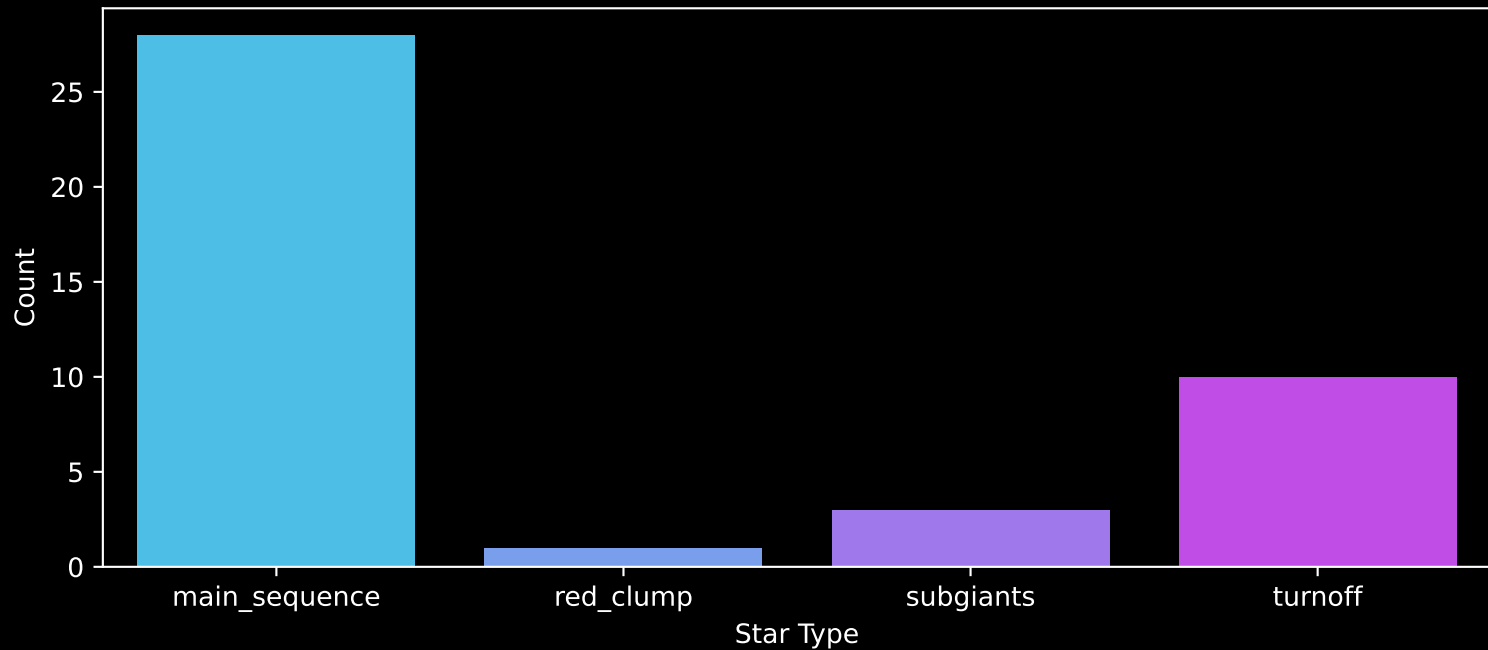
Gaia Cluster: [UBC_61] Count plot of Star Type
