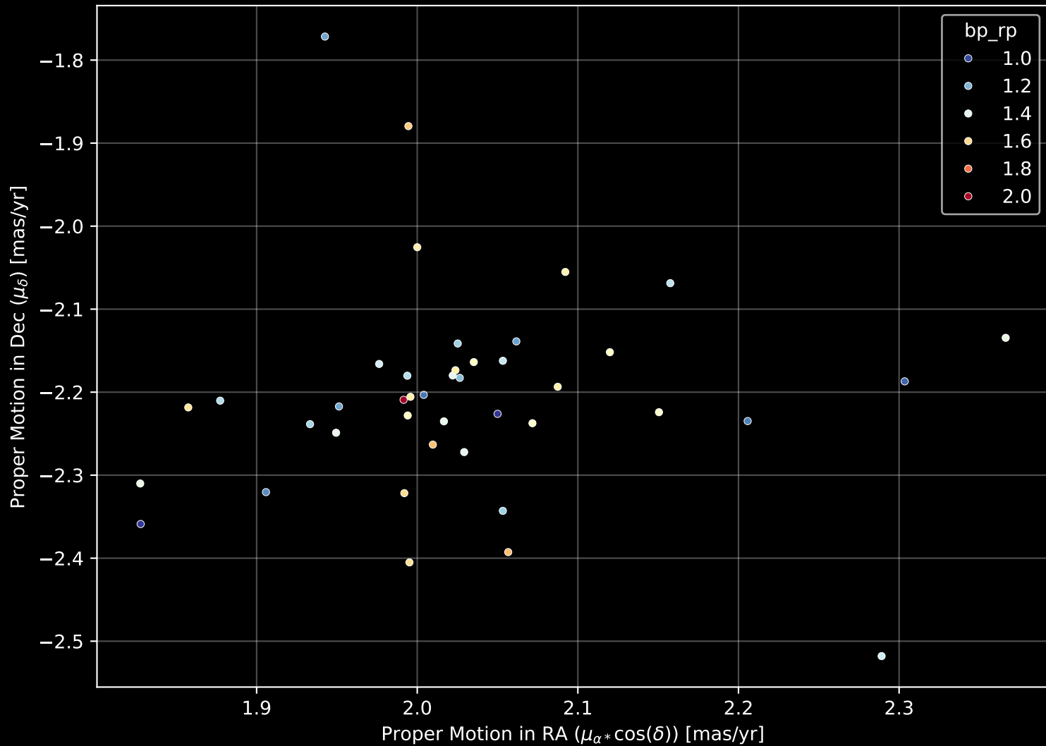
Gaia Cluster: [UBC_61] Proper Motion Diagram (n= 42)
