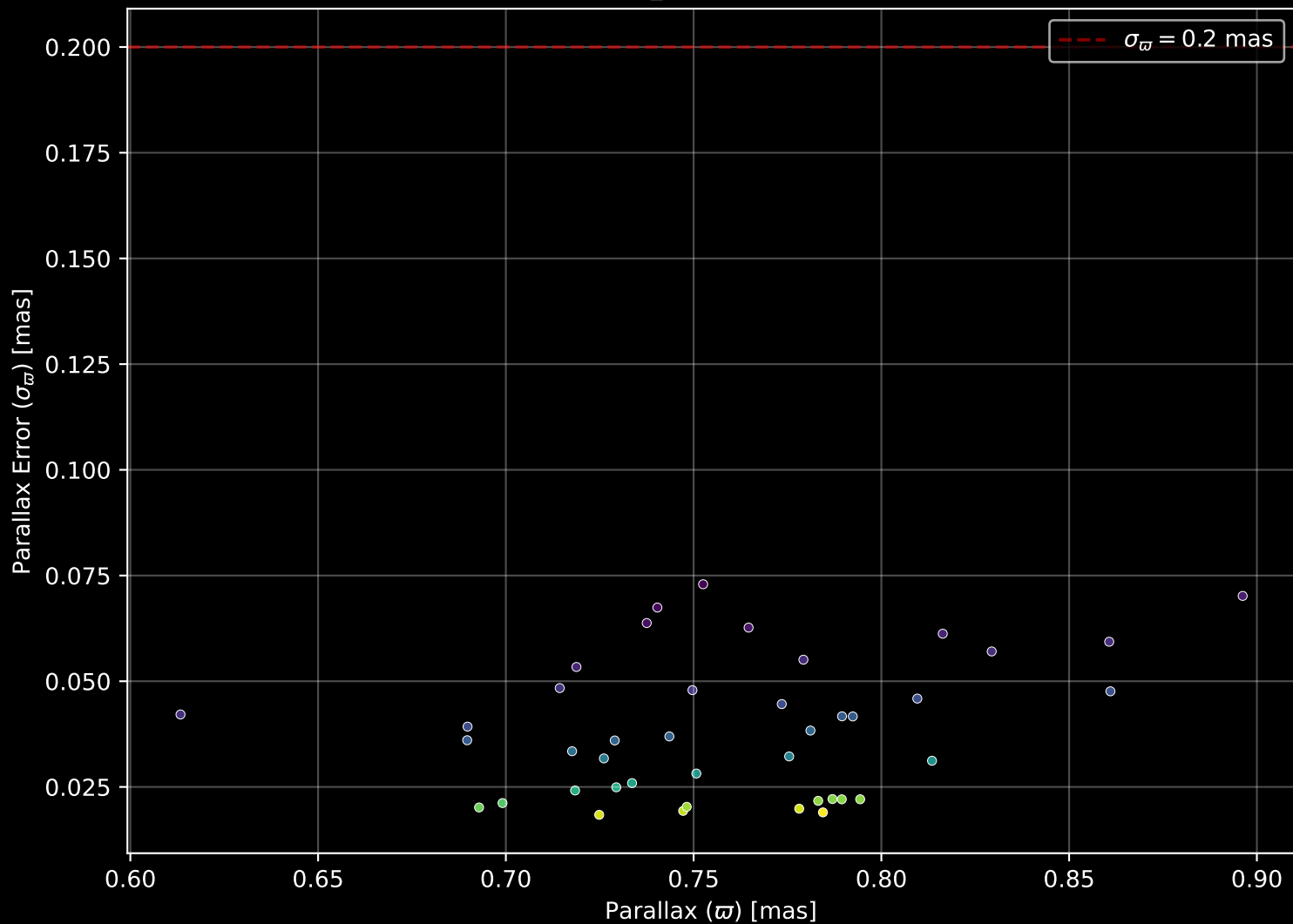
Gaia Cluster: [UBC_61] Parallax Quality (n= 42)
