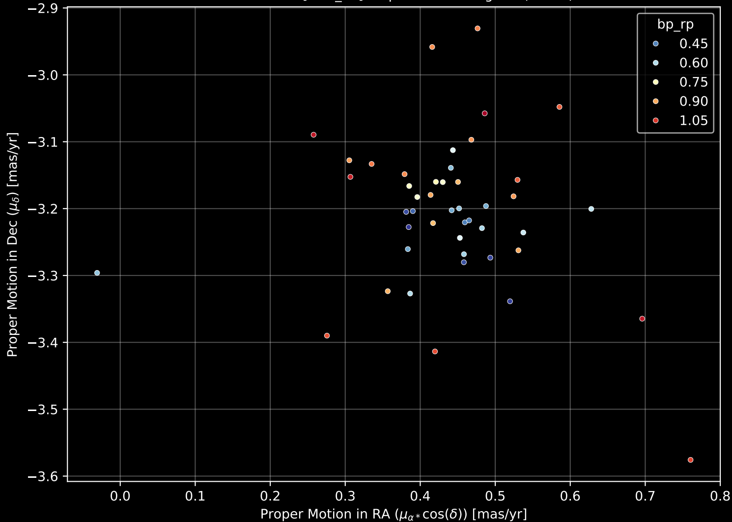
Gaia Cluster: [UBC_73] Proper Motion Diagram (n= 46)
