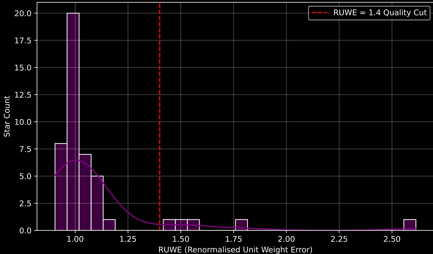
Gaia Cluster: [UBC_73] RUWE Distribution (n= 46)
