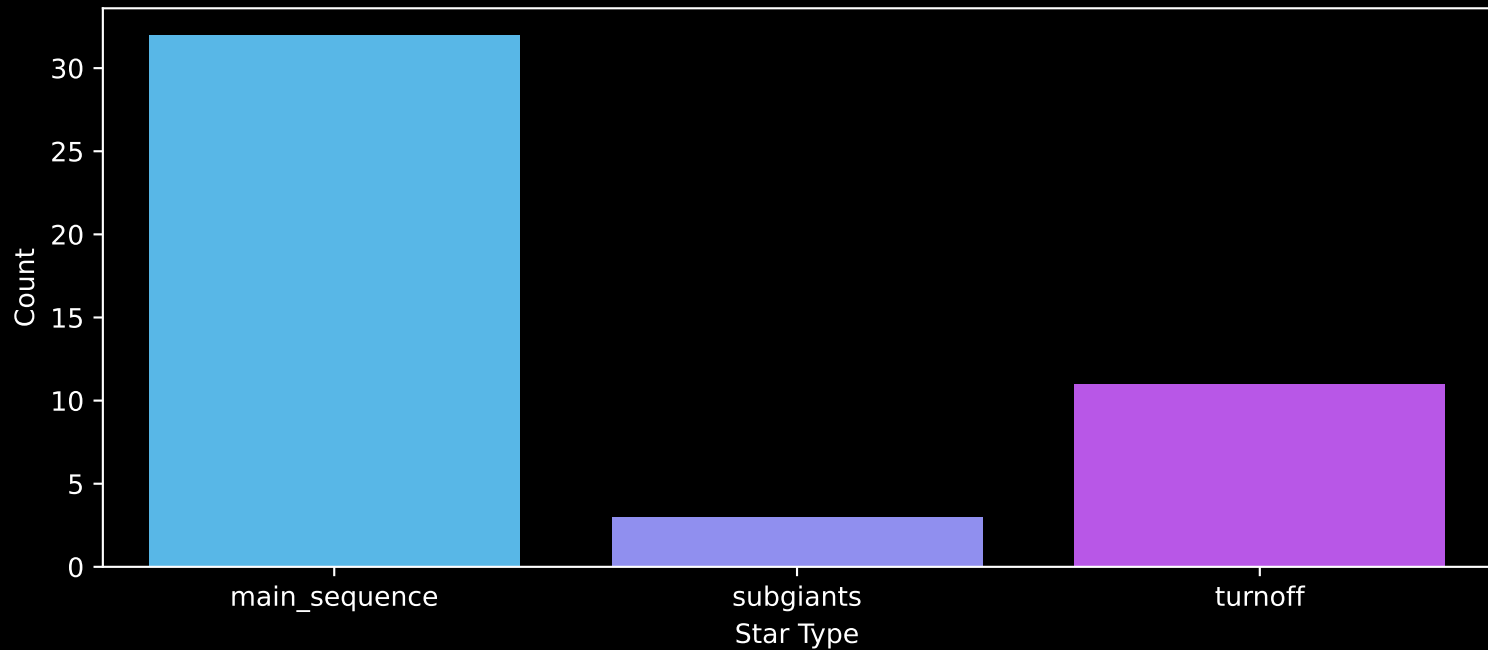
Gaia Cluster: [UBC_73] Count plot of Star Type
