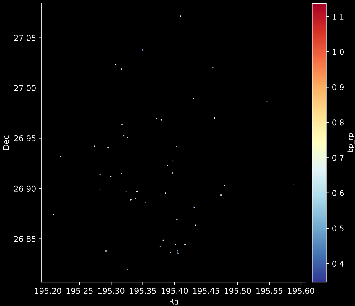
Gaia Cluster: [UBC_73] Stars: 46
