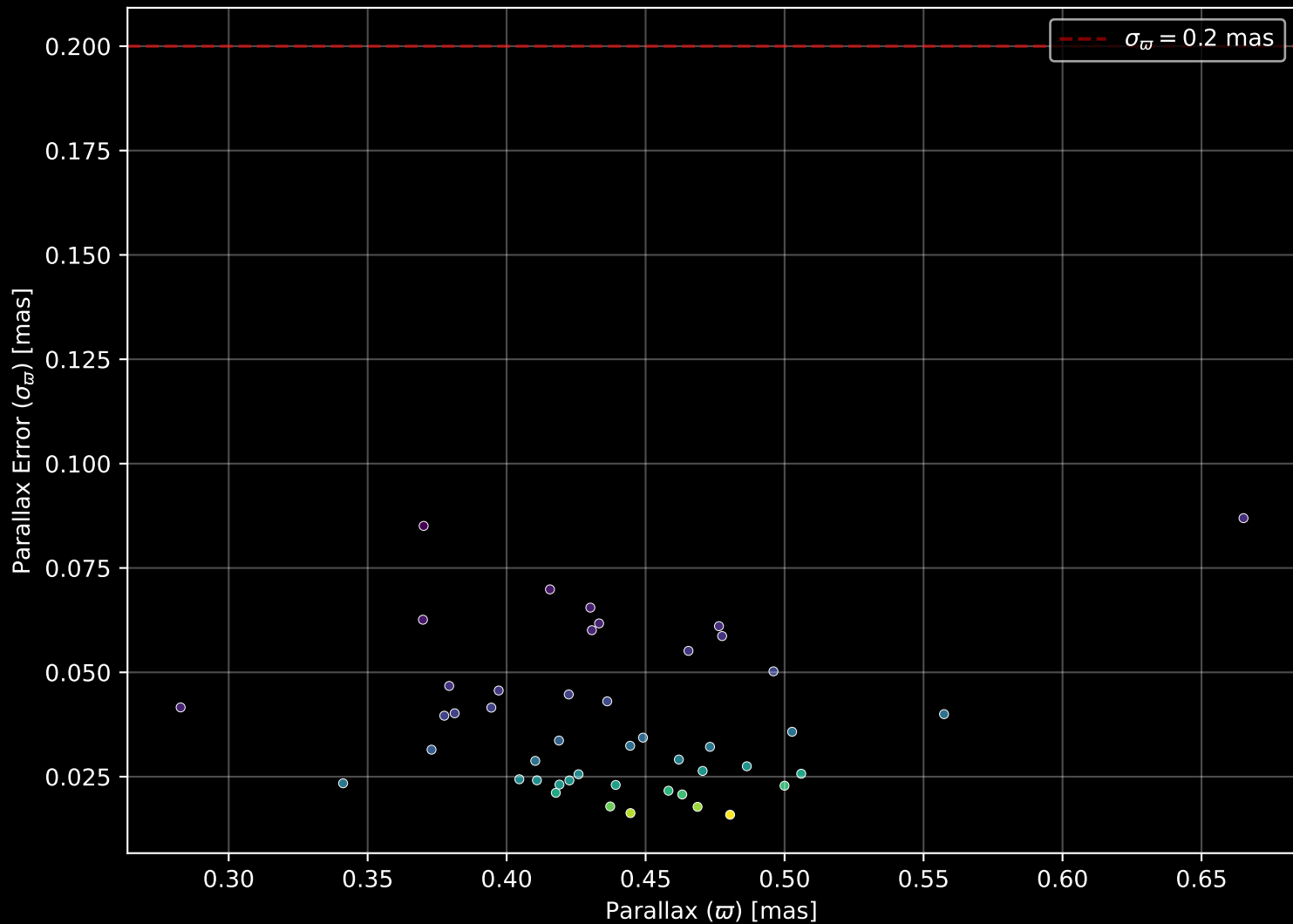
Gaia Cluster: [UBC_73] Parallax Quality (n= 46)
