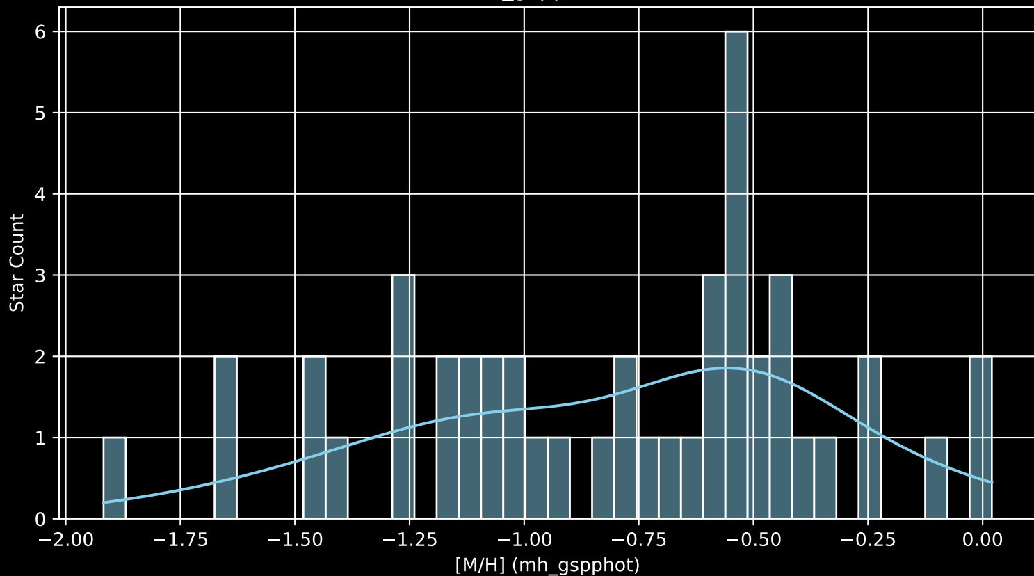
Gaia Cluster: [UBC_73 [M/H] (mh_gspphot) (n= 46)
