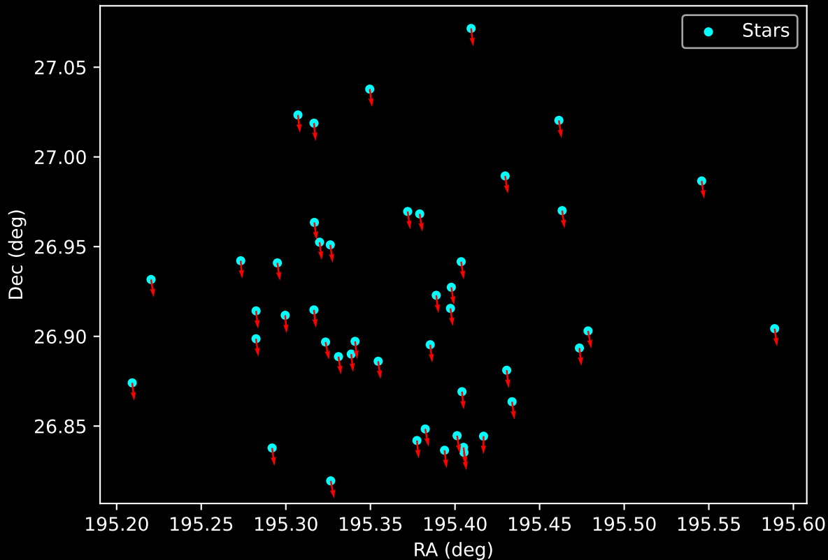
Gaia Cluster: [UBC_73] Proper Motion Vectors for Gaia Star Field (n= 46)
