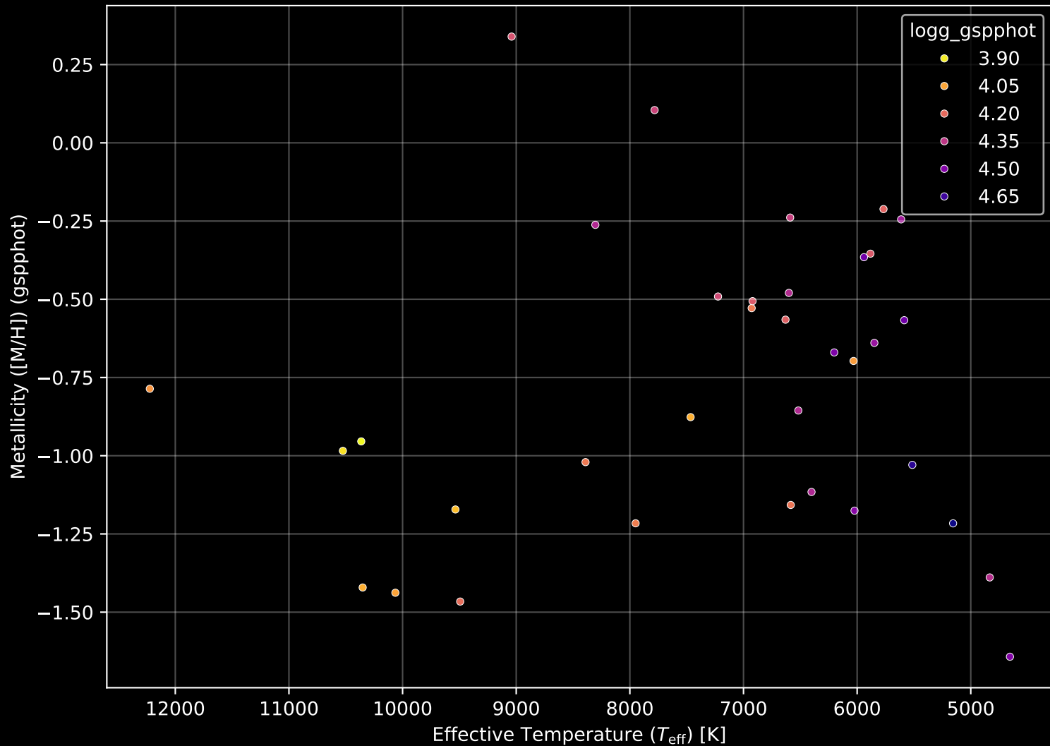
Gaia Cluster: [UBC_77] Stellar Population Parameters (n= 35)
