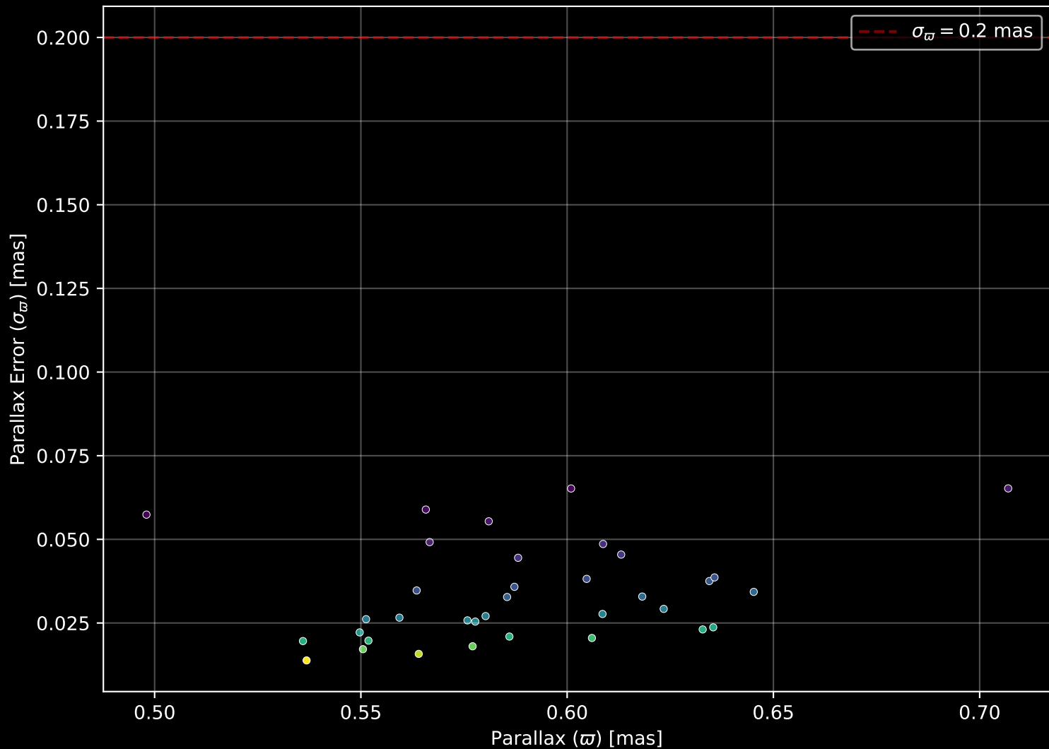
Gaia Cluster: [UBC_77] Parallax Quality (n= 35)
