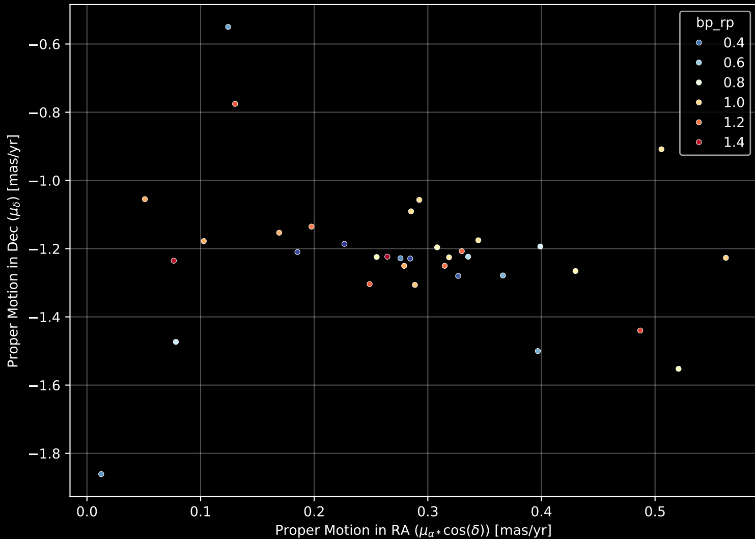
Gaia Cluster: [UBC_77] Proper Motion Diagram (n= 35)
