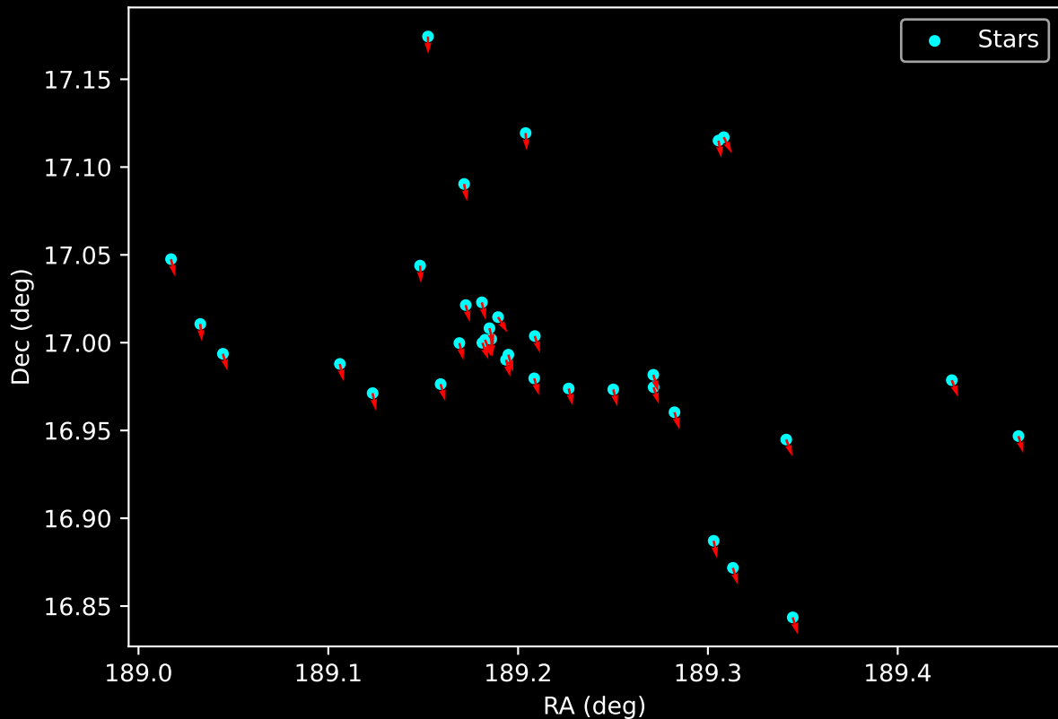
Gaia Cluster: [UBC_77] Proper Motion Vectors for Gaia Star Field (n= 35)
