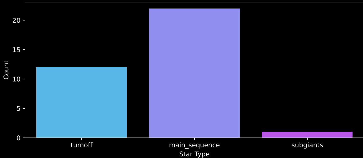
Gaia Cluster: [UBC_77] Count plot of Star Type
