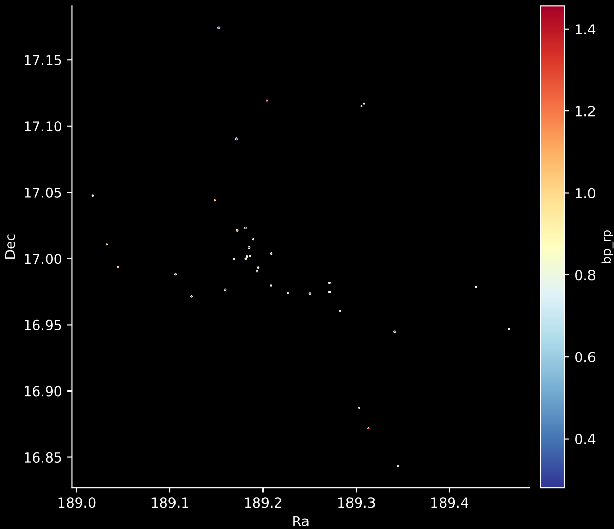
Gaia Cluster: [UBC_77] Stars: 35
