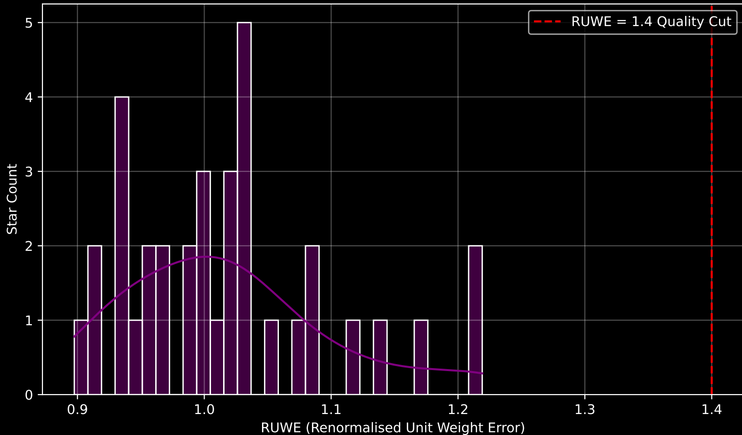
Gaia Cluster: [UBC_77] RUWE Distribution (n= 35)
