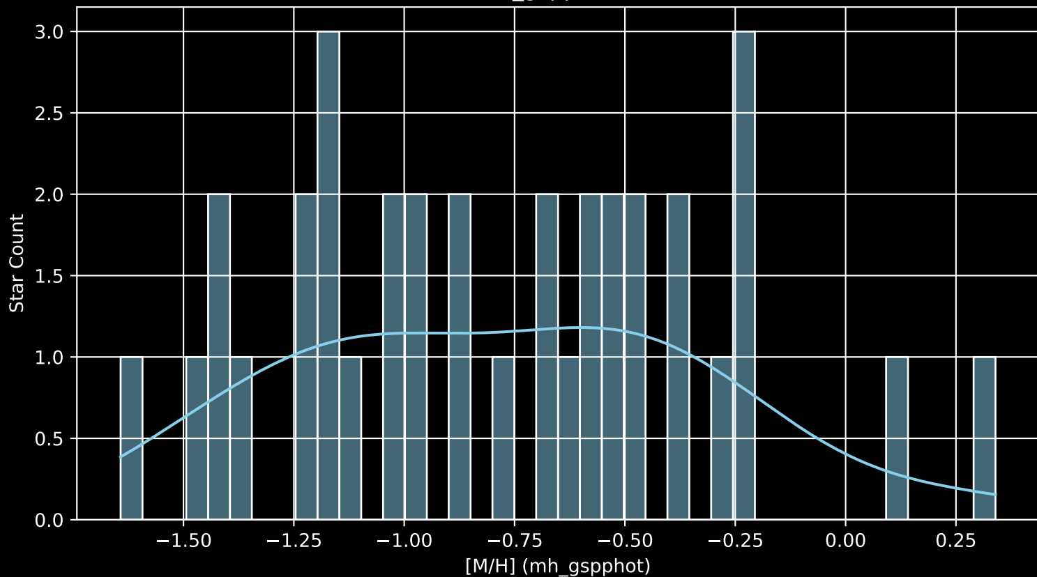
Gaia Cluster: [UBC_77 [M/H] (mh_gspphot) (n= 35)
