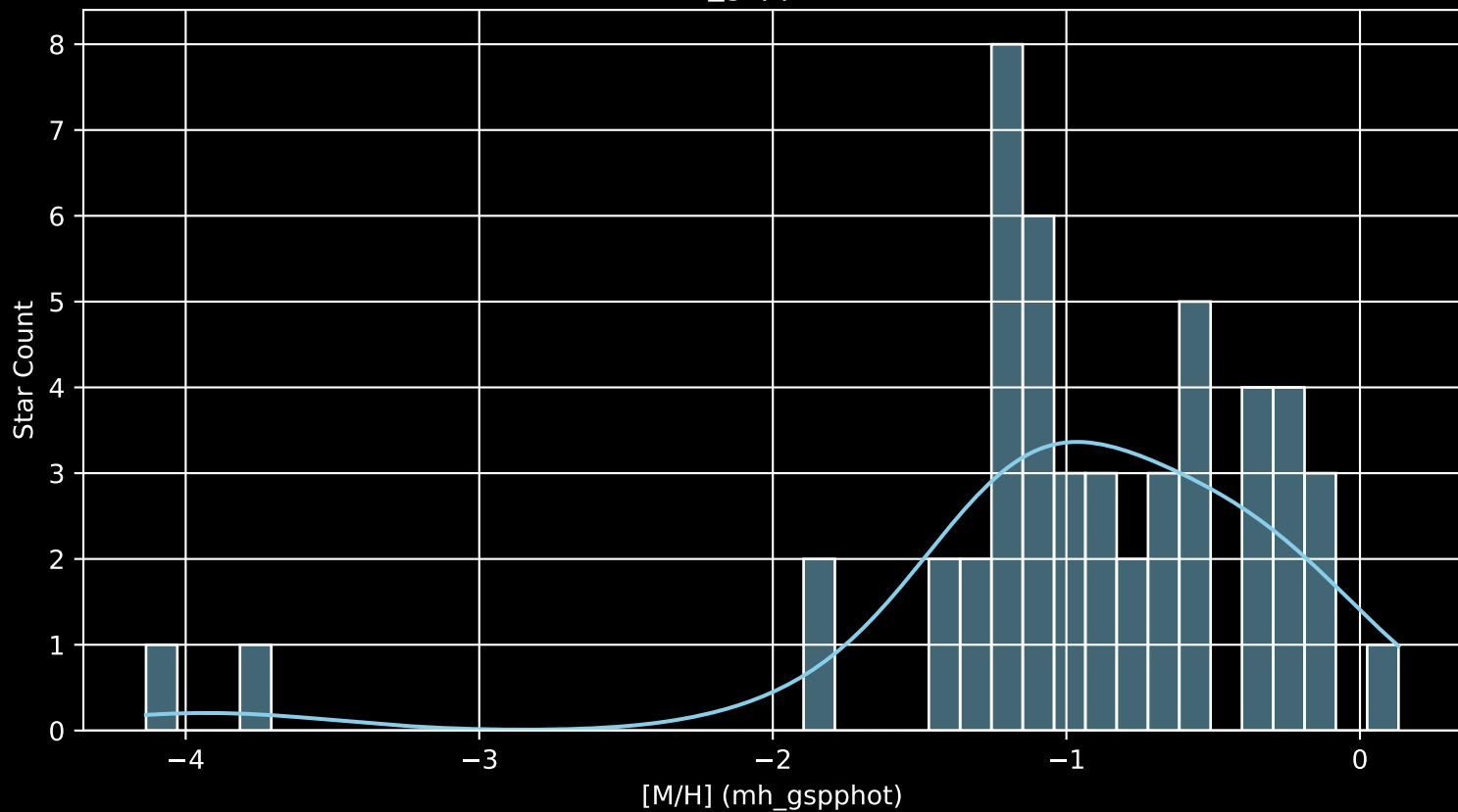
Gaia Cluster: [UBC_84 [M/H] (mh_gspphot) ( \bar{n}= 50 )
