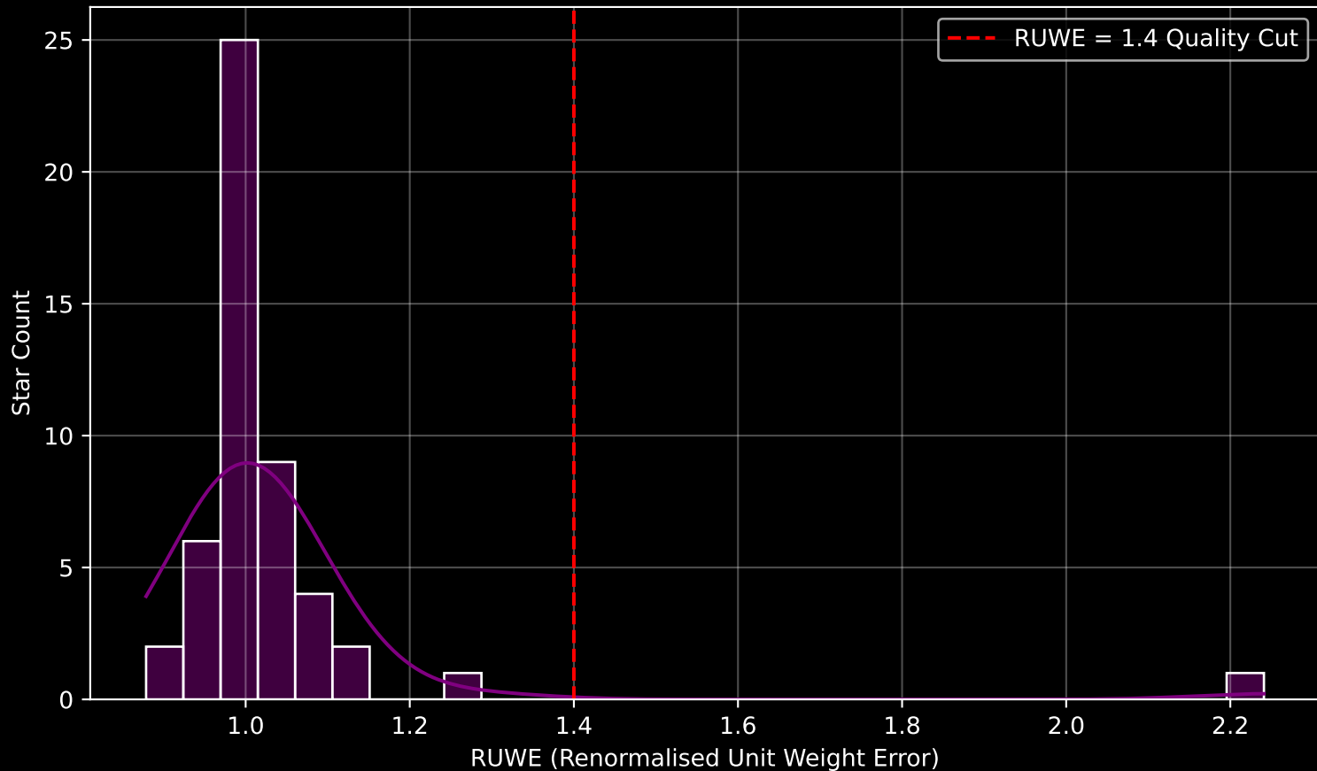
Gaia Cluster: [UBC_84] RUWE Distribution (n= 50)
