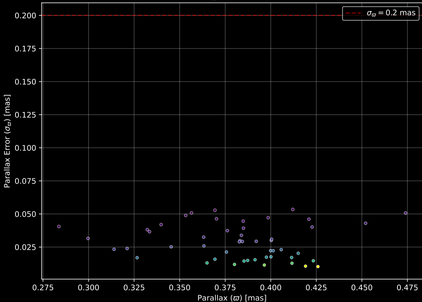
Gaia Cluster: [UBC_84] Parallax Quality (n= 50)
