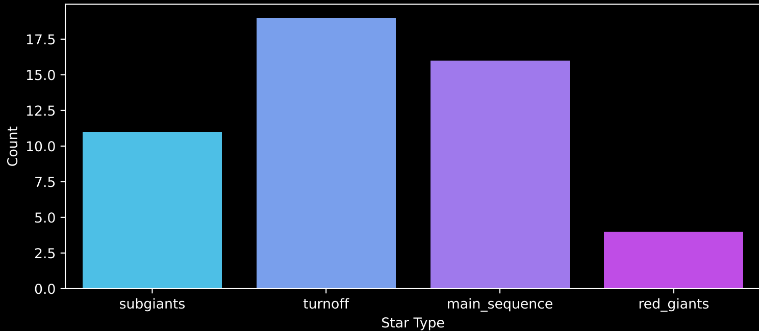
Gaia Cluster: [UBC_84] Count plot of Star Type
