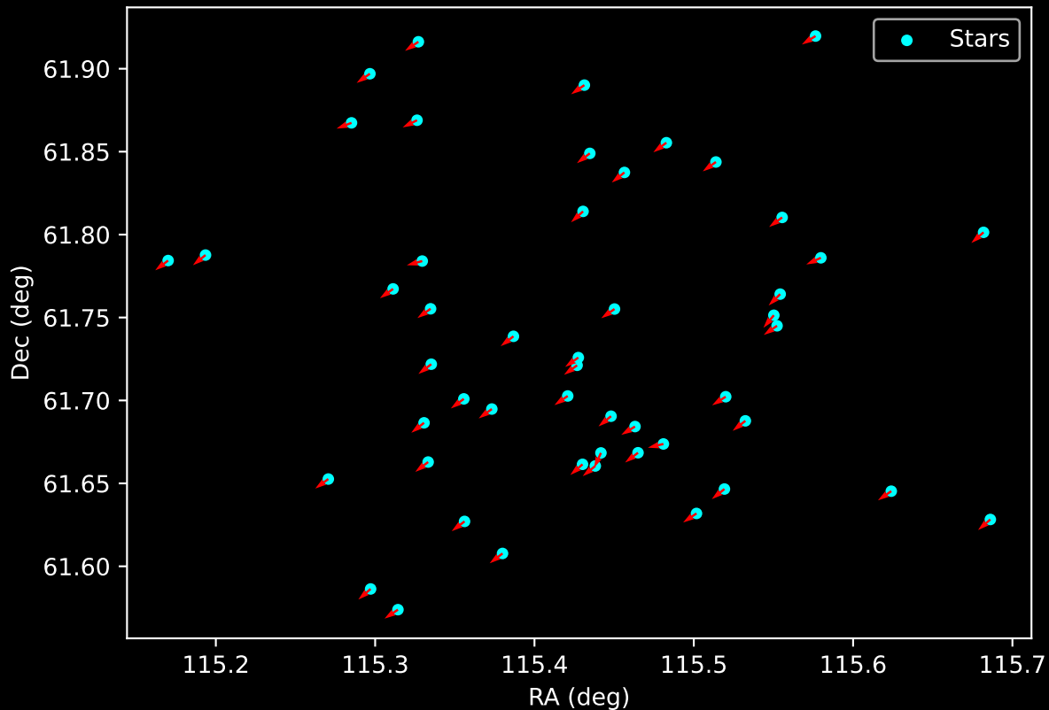
Gaia Cluster: [UBC_84] Proper Motion Vectors for Gaia Star Field (n= 50)
