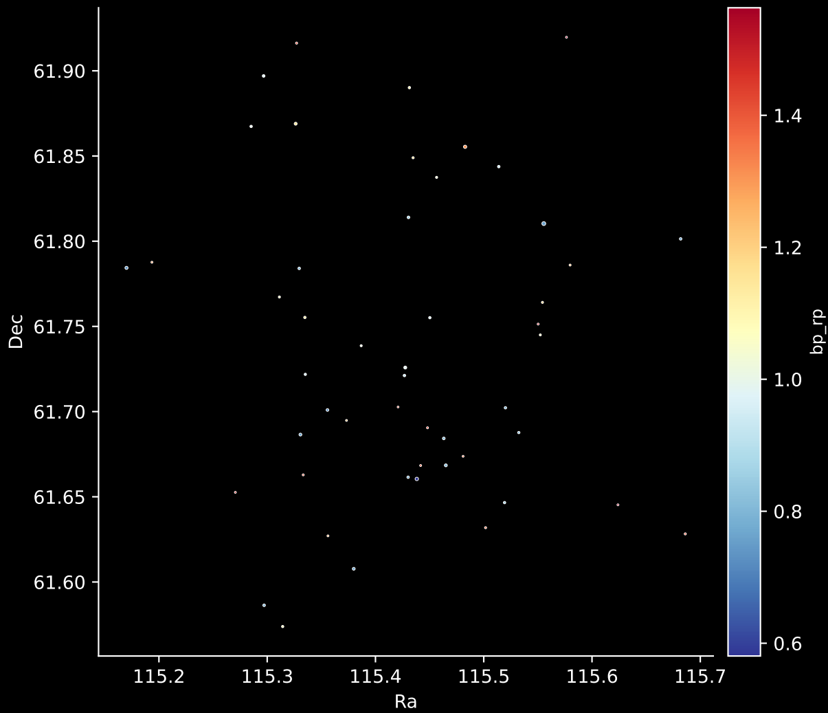
Gaia Cluster: [UBC_84] Stars: 50
