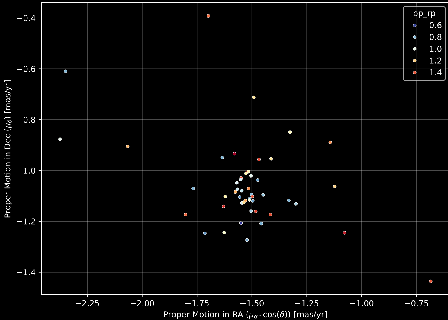
Gaia Cluster: [UBC_84] Proper Motion Diagram (n= 50)
