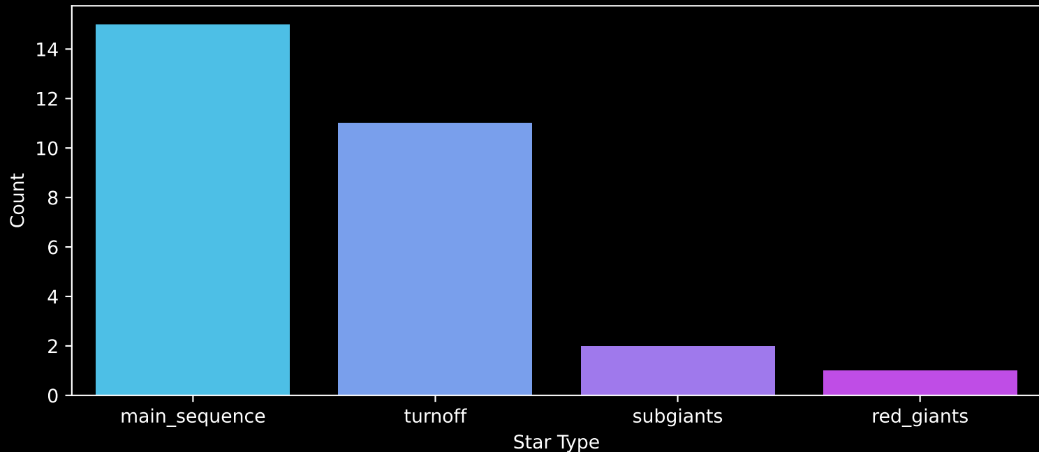
Gaia Cluster: [UBC_85] Count plot of Star Type
