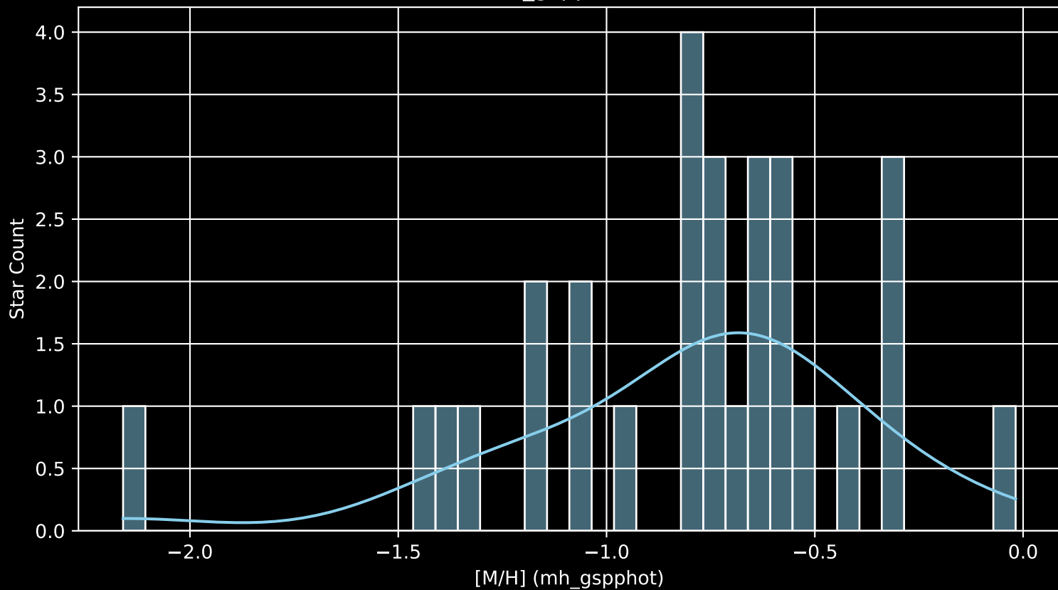
Gaia Cluster: [UBC_85 [M/H] (mh_gspphot) (n= 29)
