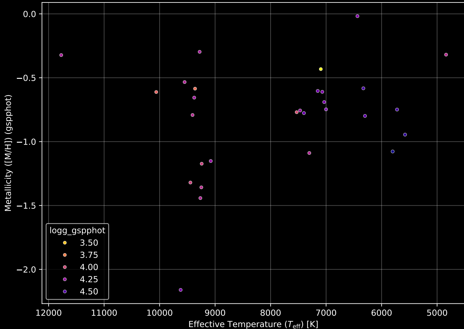
Gaia Cluster: [UBC_85] Stellar Population Parameters (n= 29)
