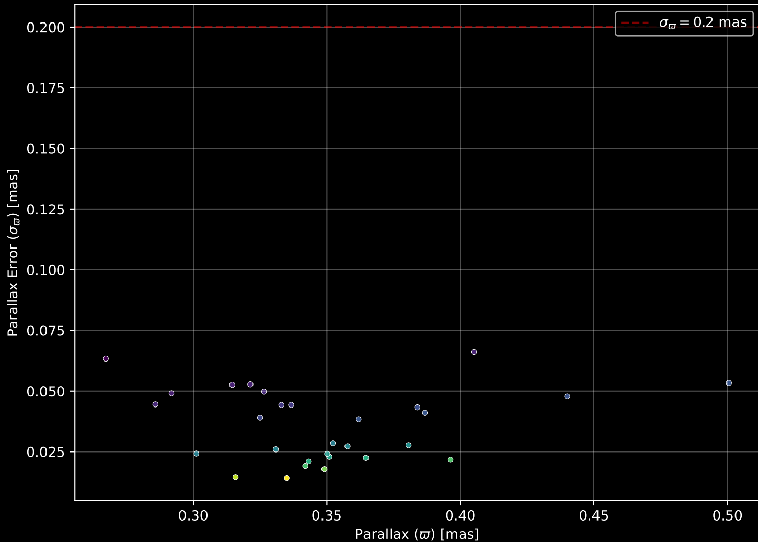
Gaia Cluster: [UBC_85] Parallax Quality (n= 29)
