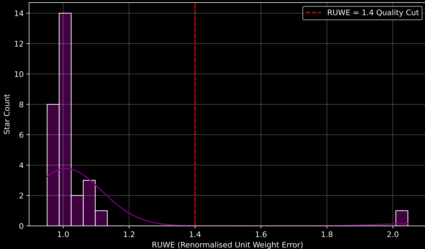
Gaia Cluster: [UBC_85] RUWE Distribution (n= 29)
