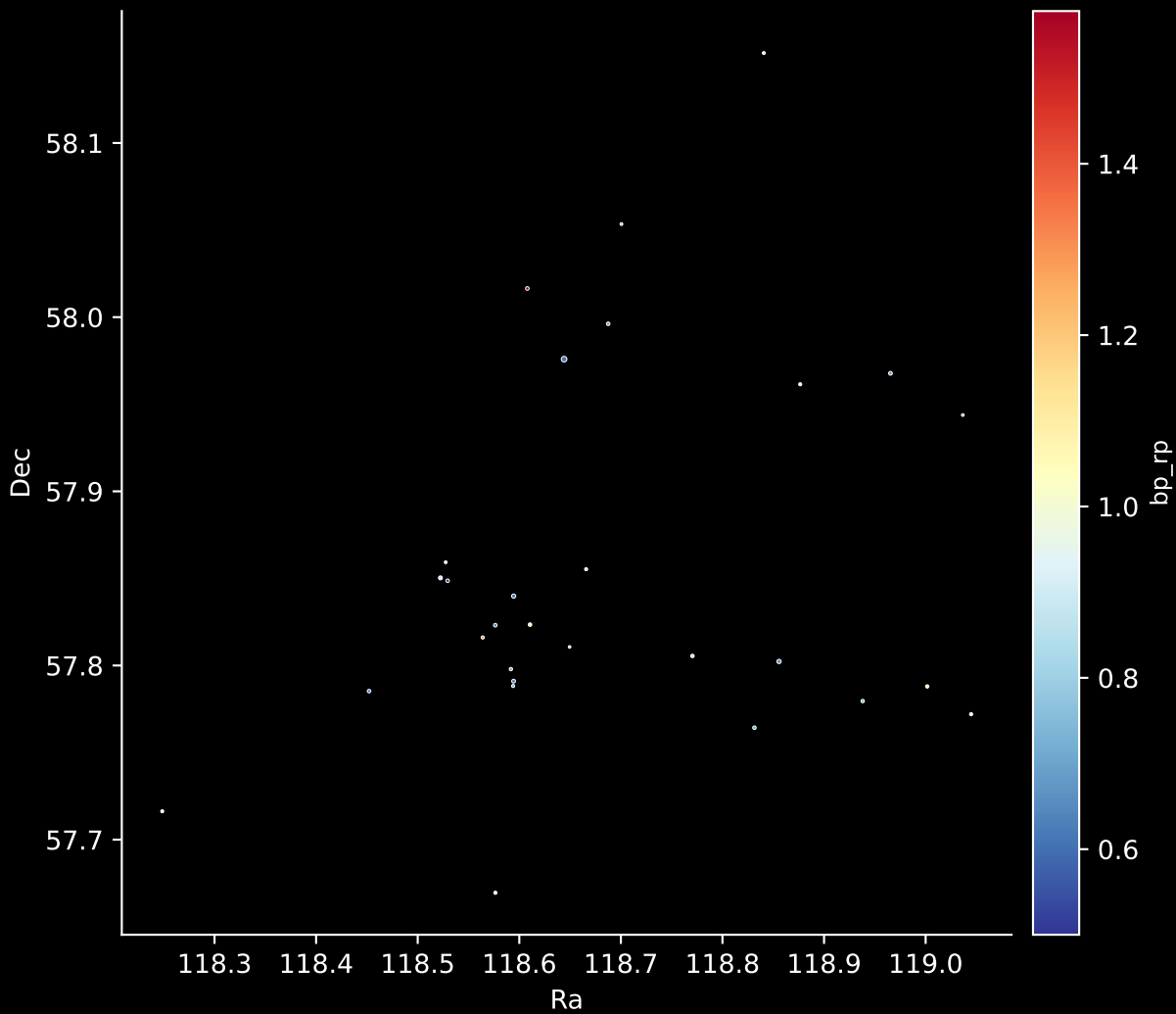
Gaia Cluster: [UBC_85] Stars: 29
