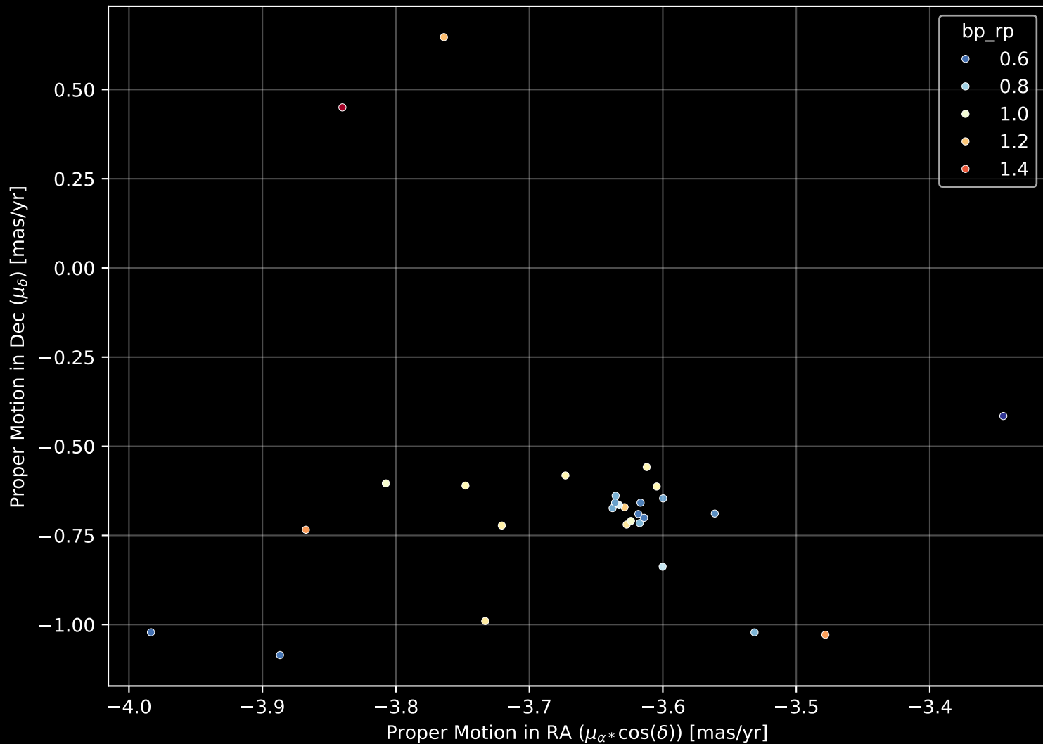
Gaia Cluster: [UBC_85] Proper Motion Diagram (n= 29)
