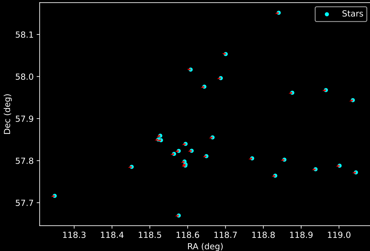
Gaia Cluster: [UBC_85] Proper Motion Vectors for Gaia Star Field (n= 29)
