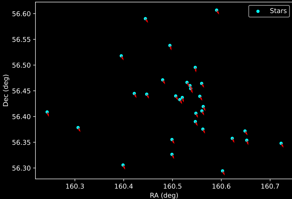
Gaia Cluster: [UBC_87] Proper Motion Vectors for Gaia Star Field (n= 31)
