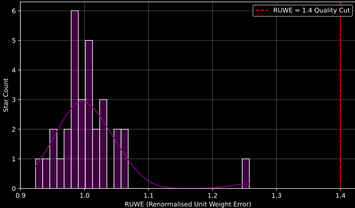
Gaia Cluster: [UBC_87] RUWE Distribution (n= 31)
