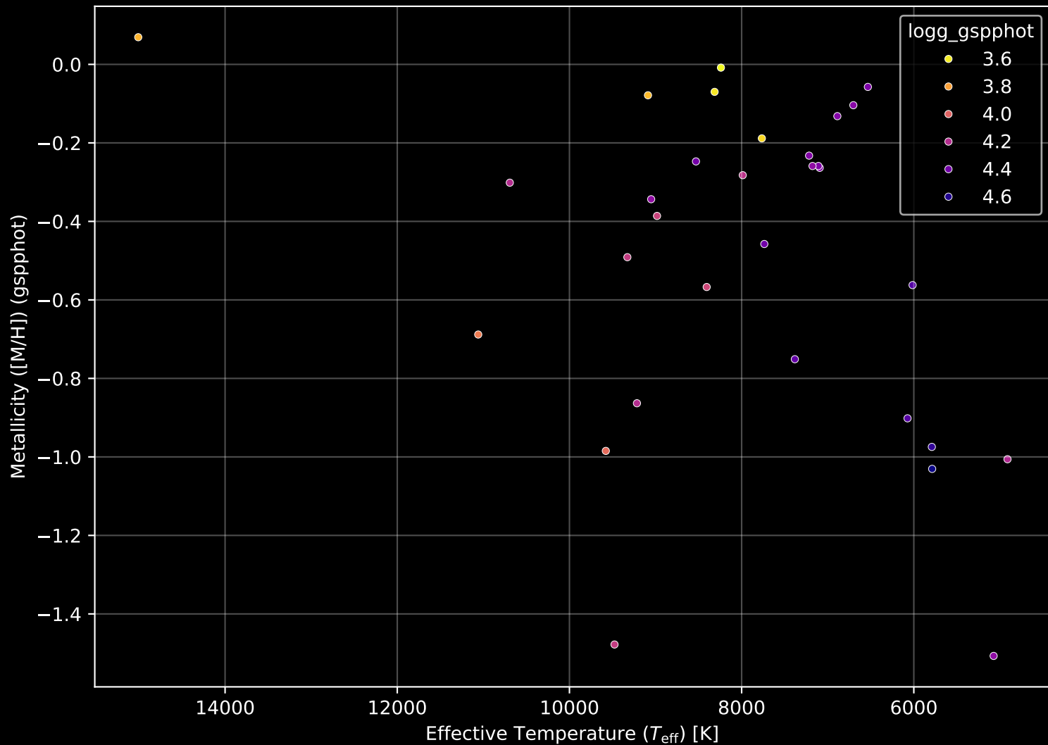
Gaia Cluster: [UBC_87] Stellar Population Parameters (n= 31)
