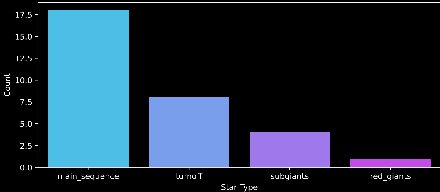
Gaia Cluster: [UBC_87] Count plot of Star Type
