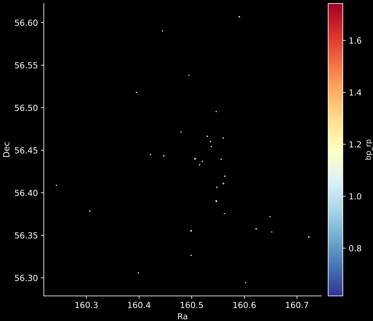
Gaia Cluster: [UBC_87] Stars: 31
