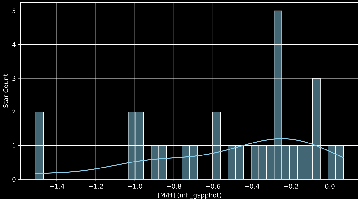
Gaia Cluster: [UBC_87 [M/H] (mh_gspphot) ( \bar{n}= 31 )
