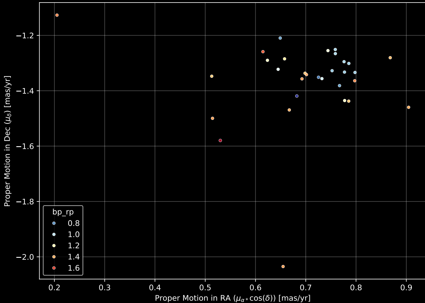
Gaia Cluster: [UBC_87] Proper Motion Diagram (n= 31)
