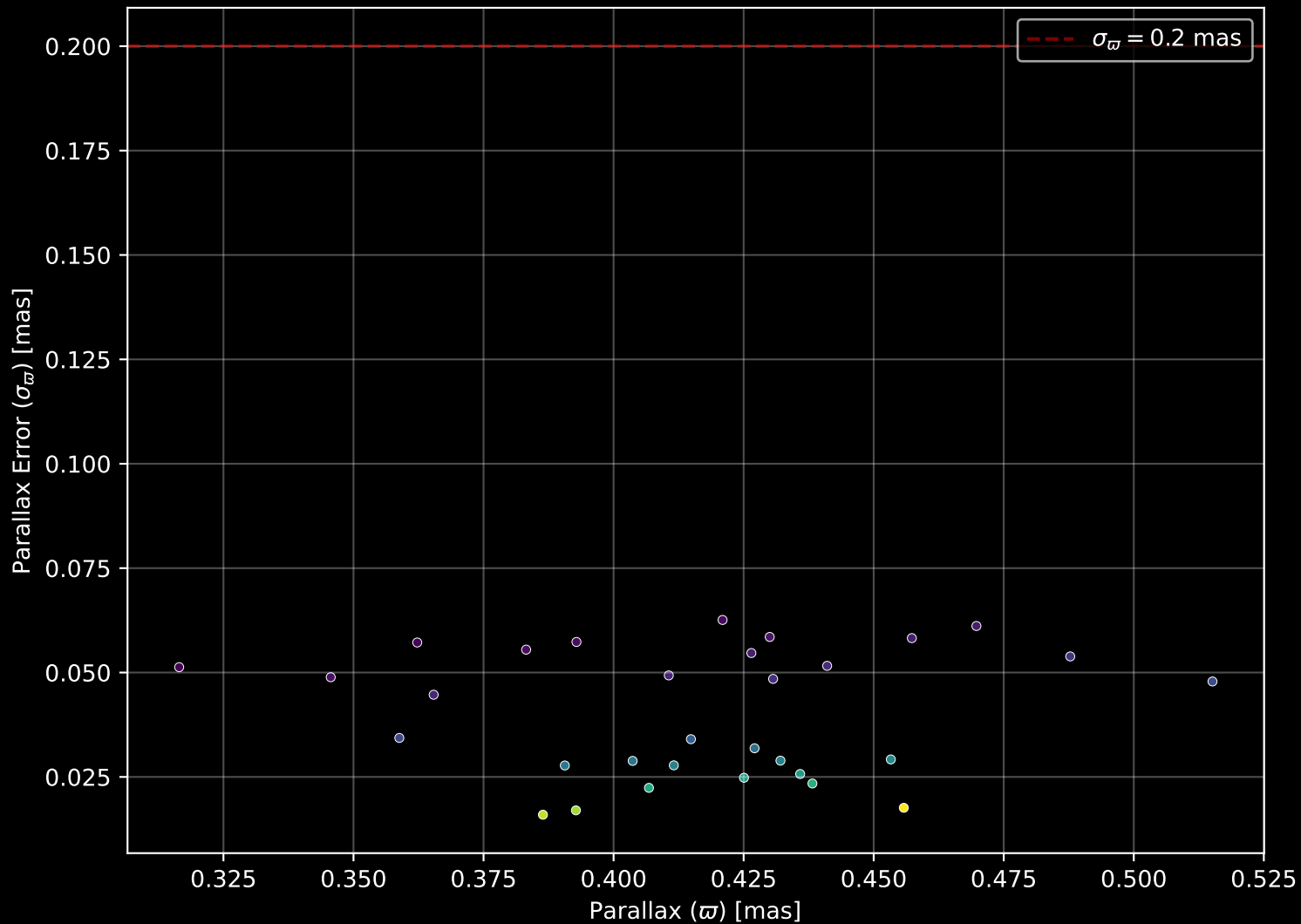
Gaia Cluster: [UBC_87] Parallax Quality (n= 31)
