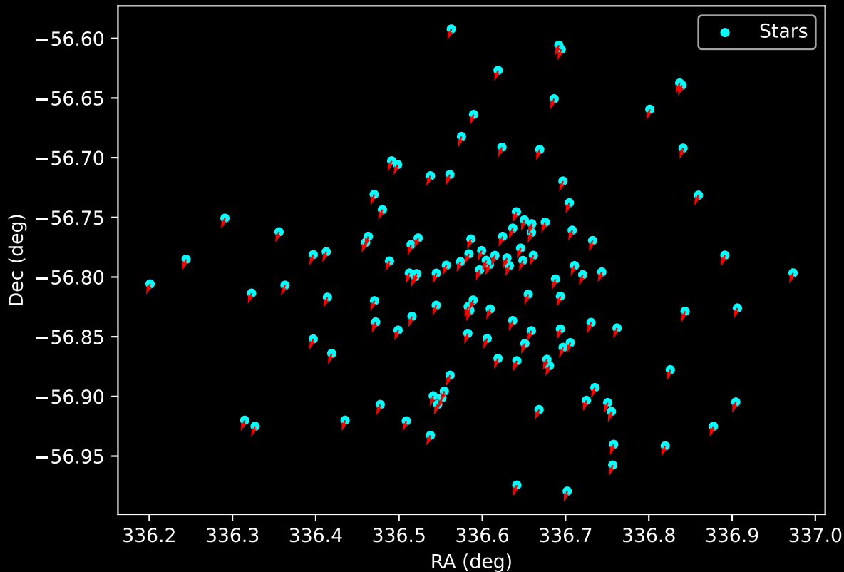
Gaia Cluster: [UFMG_1] Proper Motion Vectors for Gaia Star Field (n= 122)
