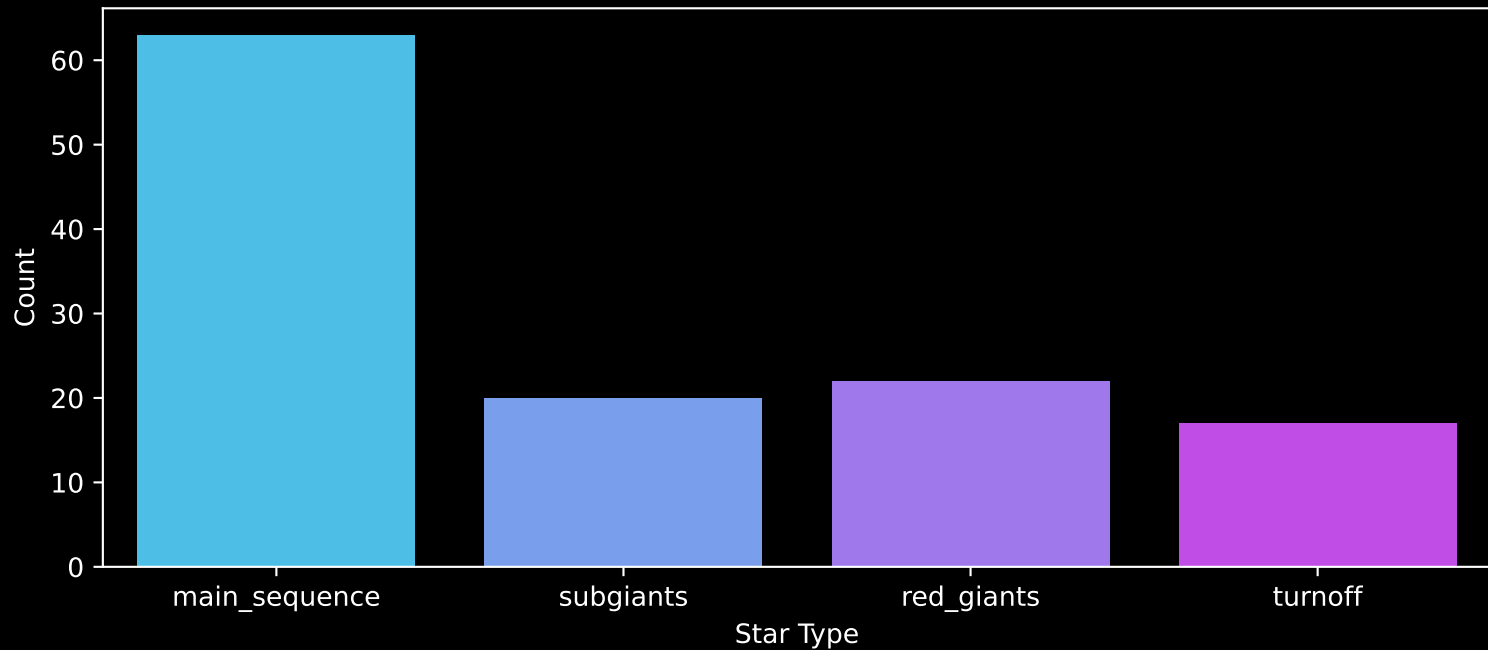
Gaia Cluster: [UFMG_1] Count plot of Star Type
