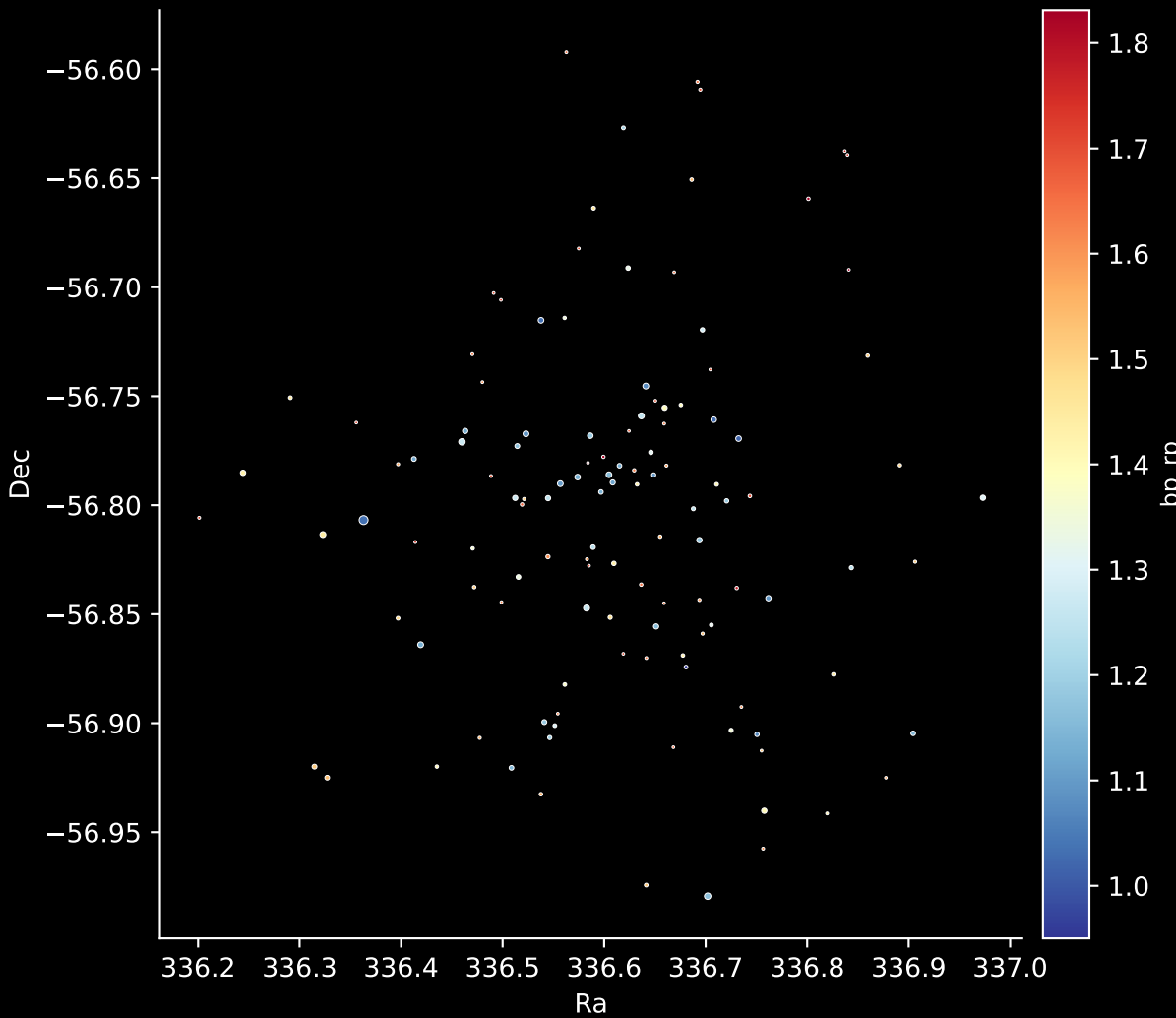
Gaia Cluster: [UFMG_1] Stars: 122
