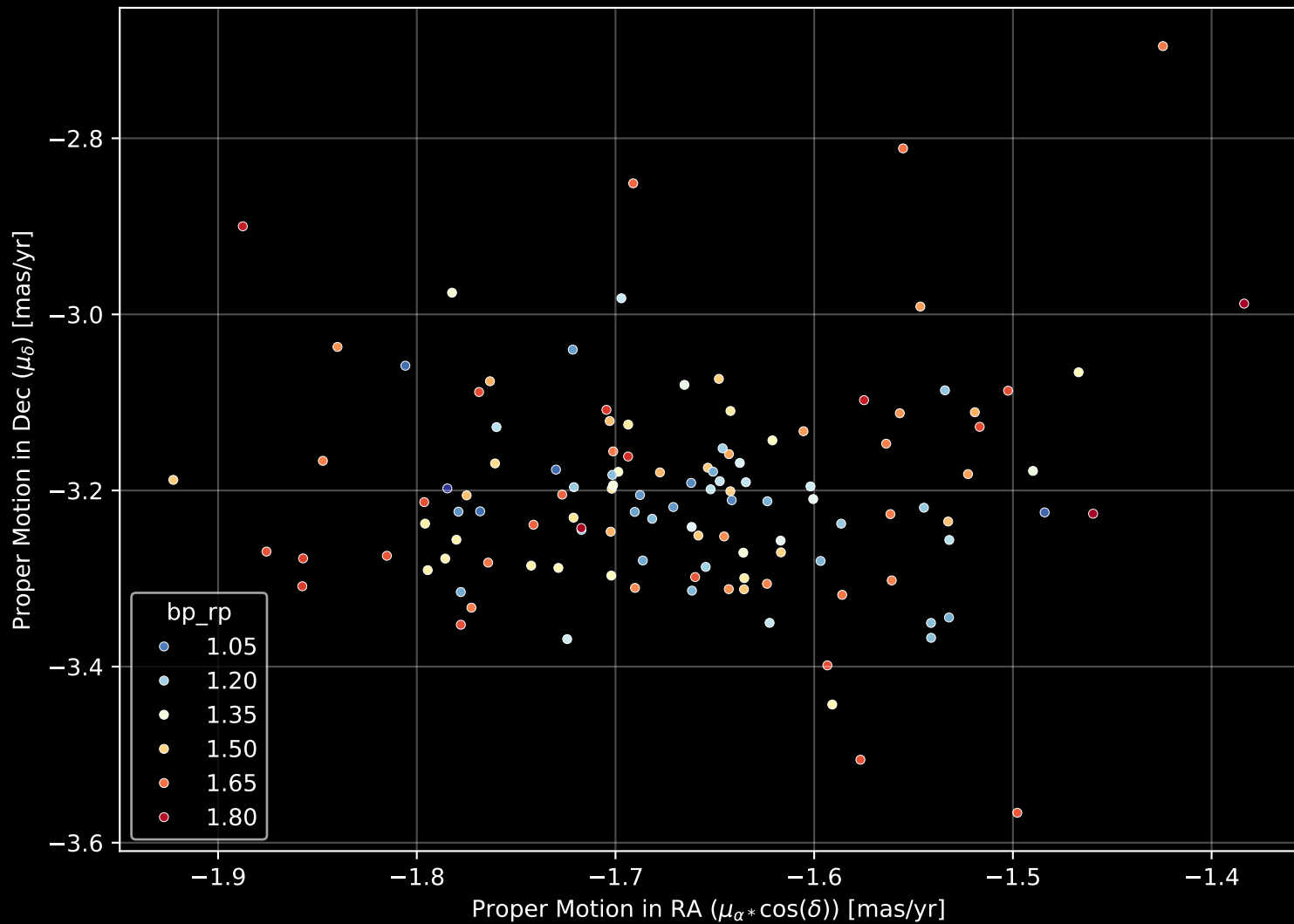
Gaia Cluster: [UFMG_1] Proper Motion Diagram (n= 122)
