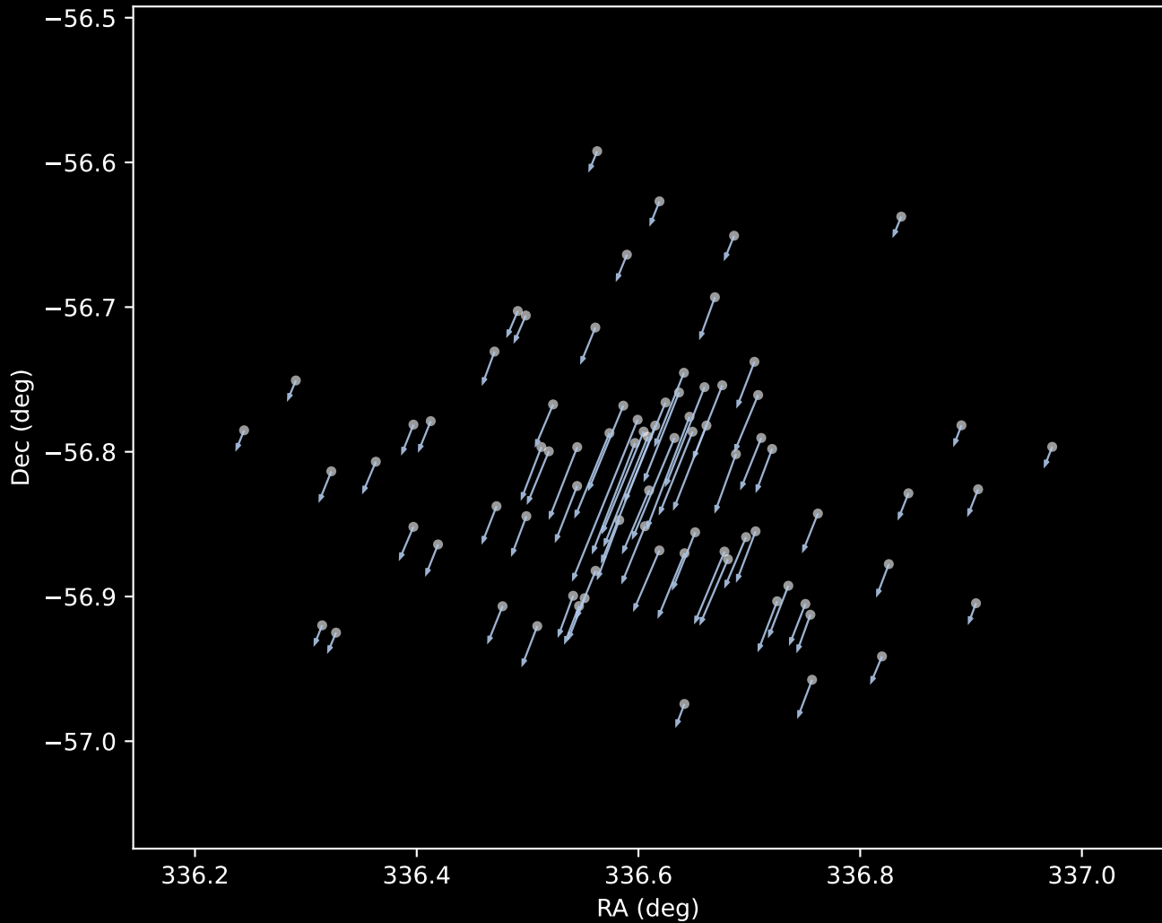
Gaia DR3 Cluster 1 Proper Motion Vectors (n=78)
