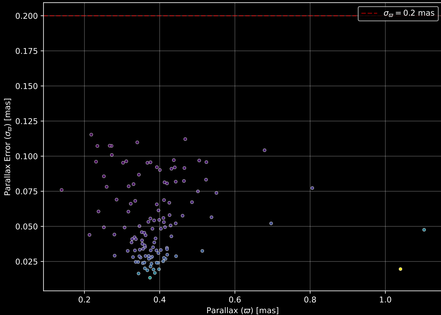
Gaia Cluster: [UFMG_1] Parallax Quality (n= 122)
