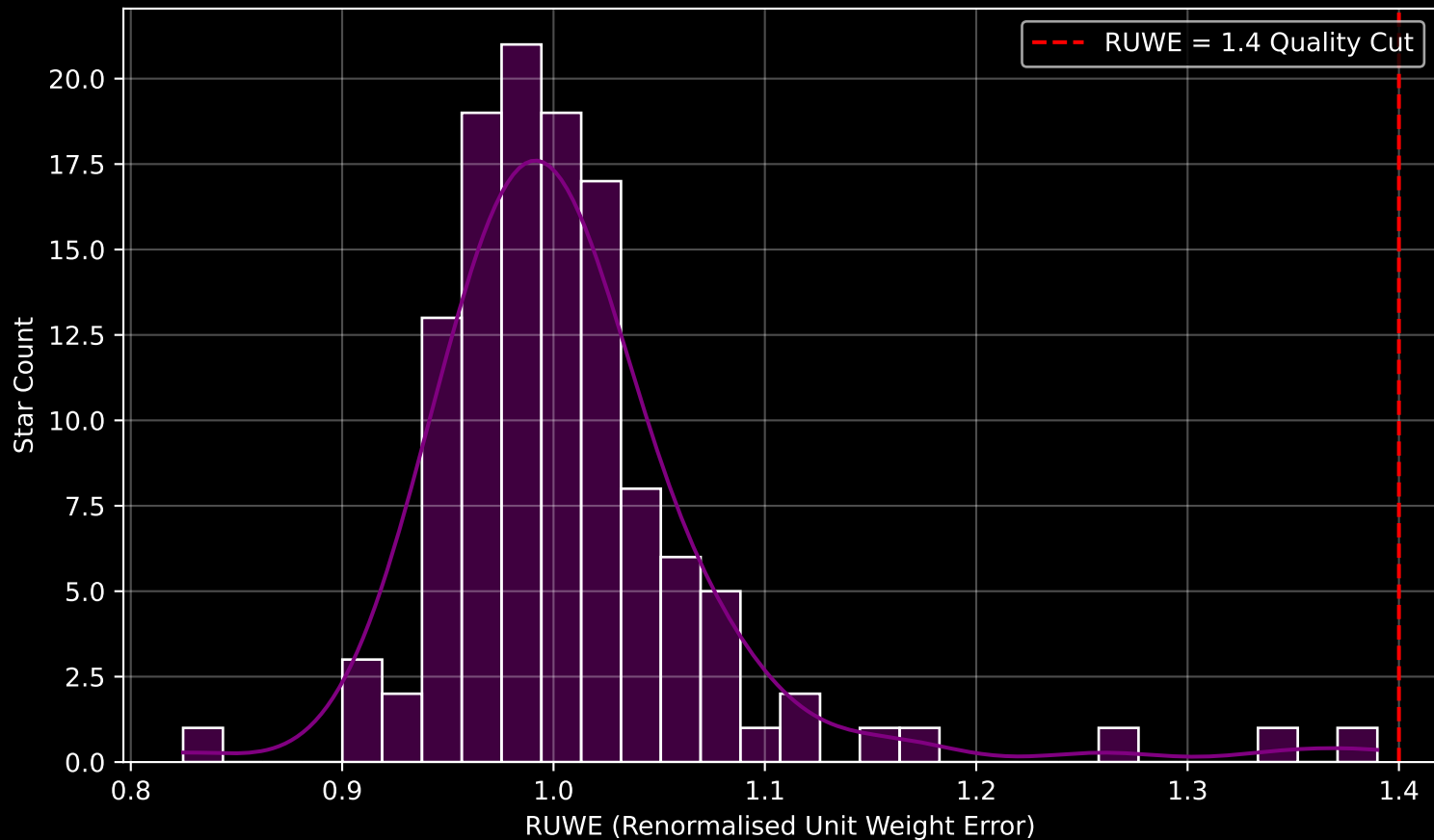
Gaia Cluster: [UFMG_1] RUWE Distribution (n= 122)
