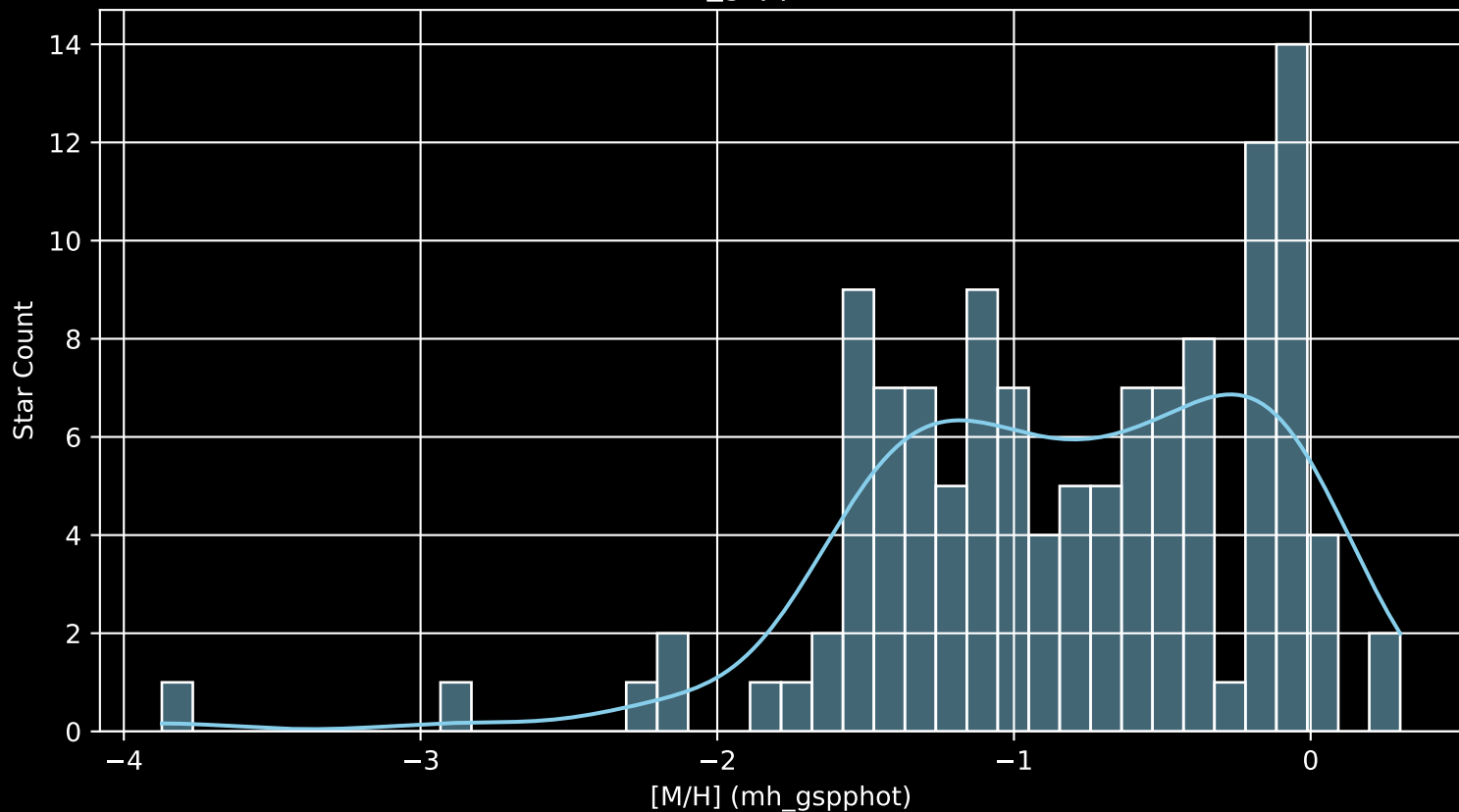
Gaia Cluster: [UFMG_1 [M/H] (mh_gspphot) (n= 122)
