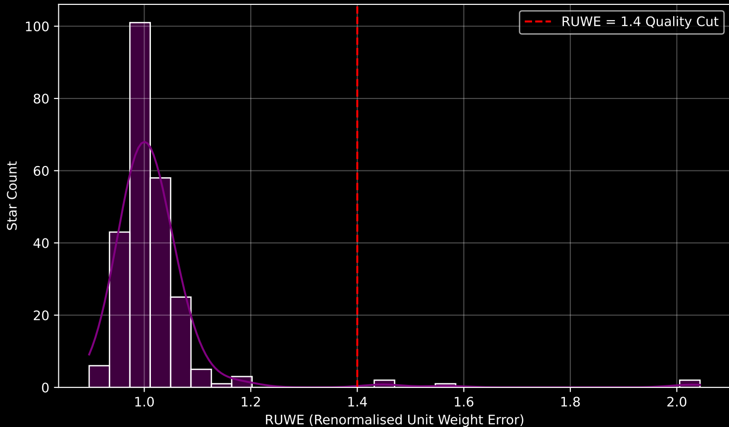
Gaia Cluster: [UFMG_2] RUWE Distribution (n= 247)
