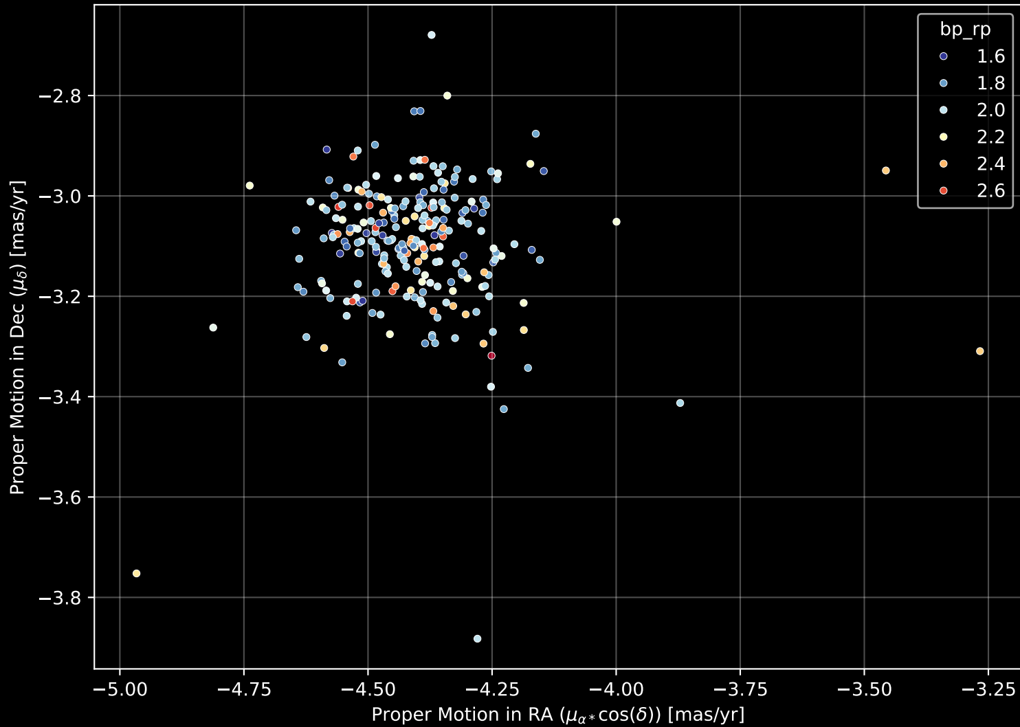
Gaia Cluster: [UFMG_2] Proper Motion Diagram (n= 247)
