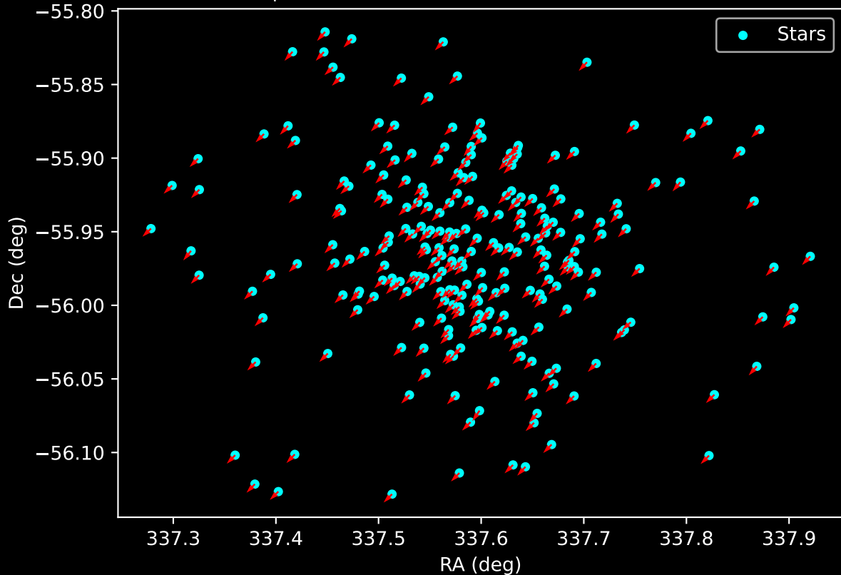
Gaia Cluster: [UFMG_2] Proper Motion Vectors for Gaia Star Field (n= 247)
