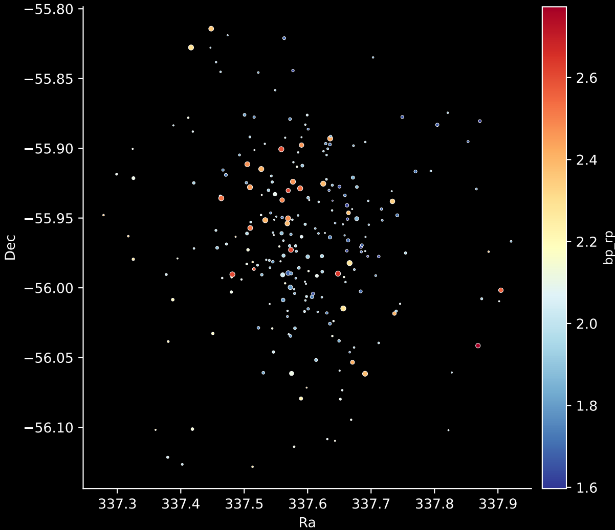
Gaia Cluster: [UFMG_2] Stars: 247
