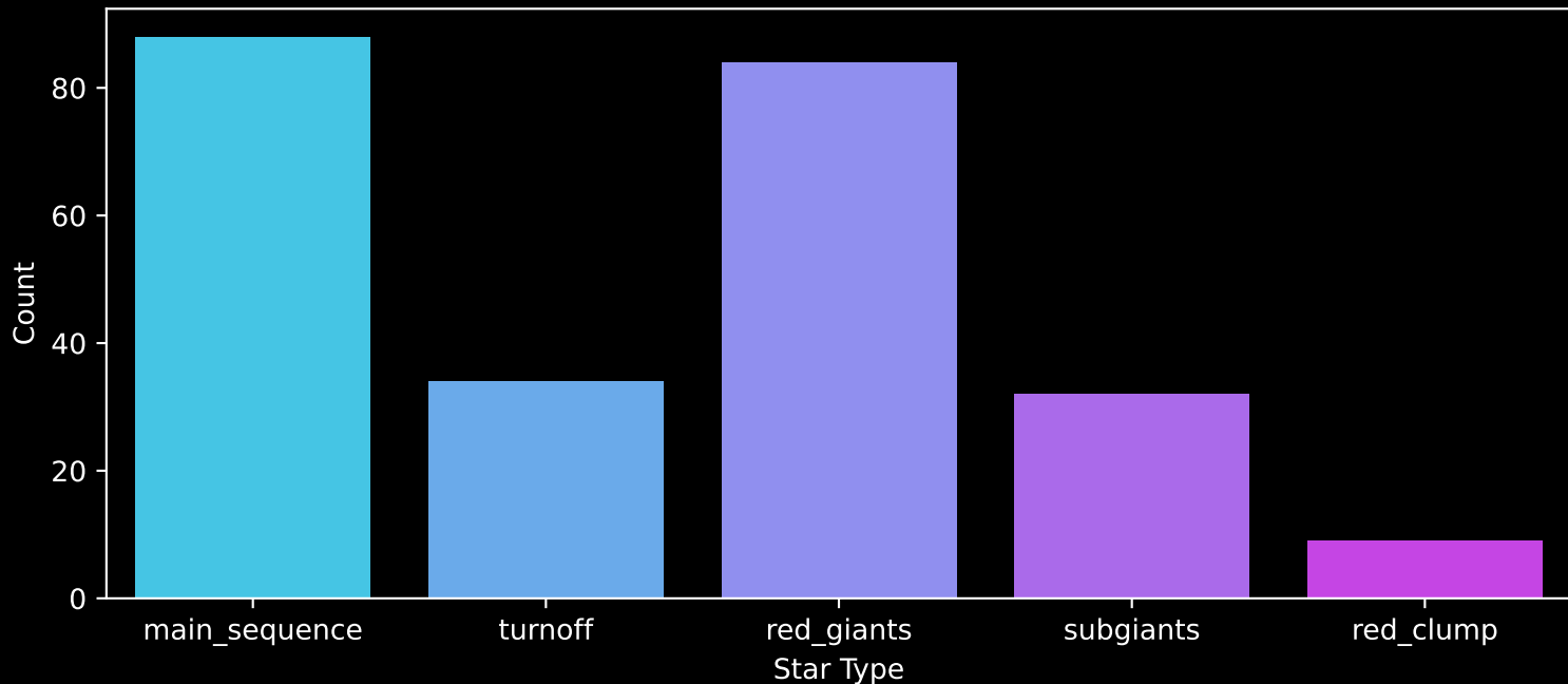
Gaia Cluster: [UFMG_2] Count plot of Star Type
