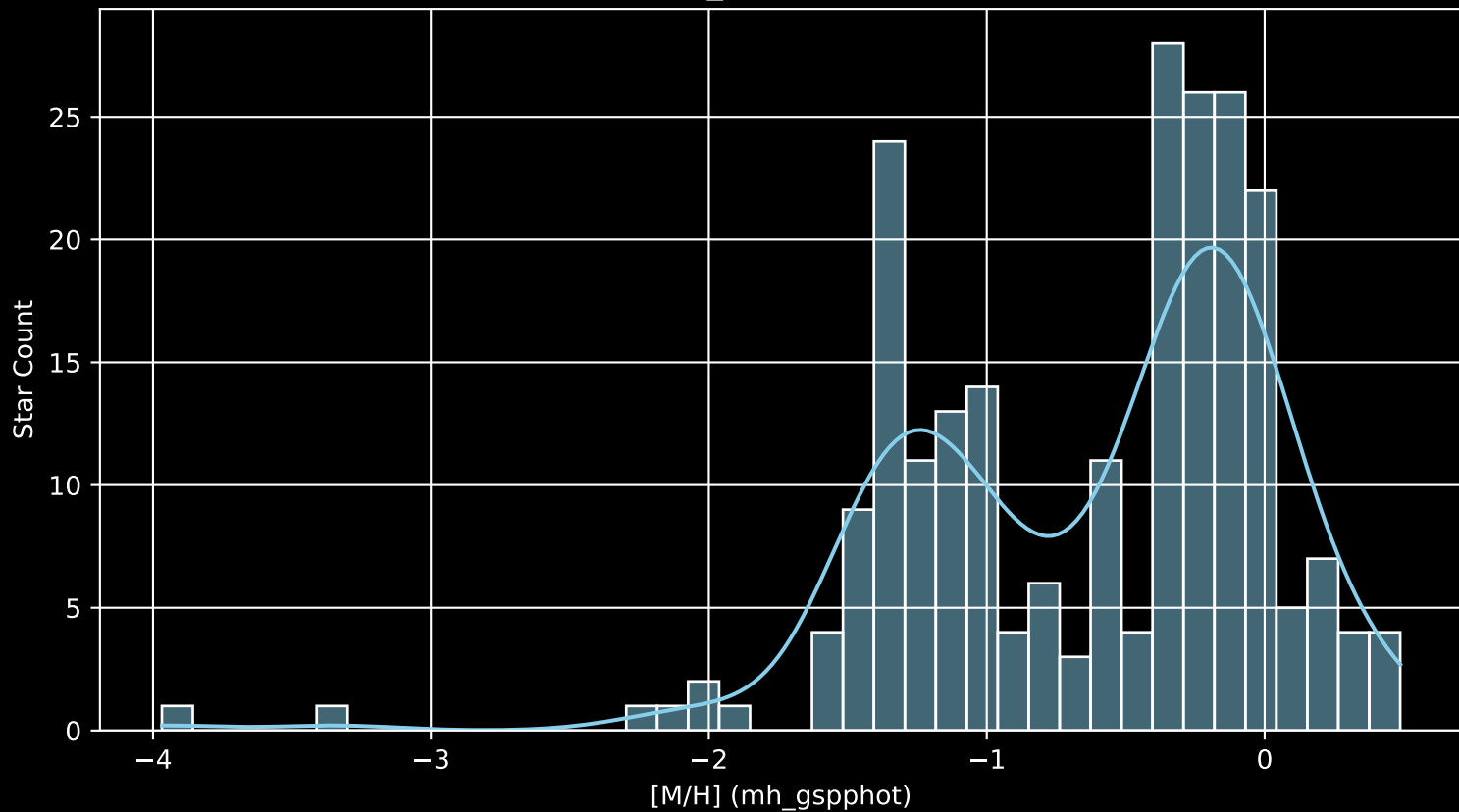
Gaia Cluster: [UFMG_2 [M/H] (mh_gspphot) (n= 232)
