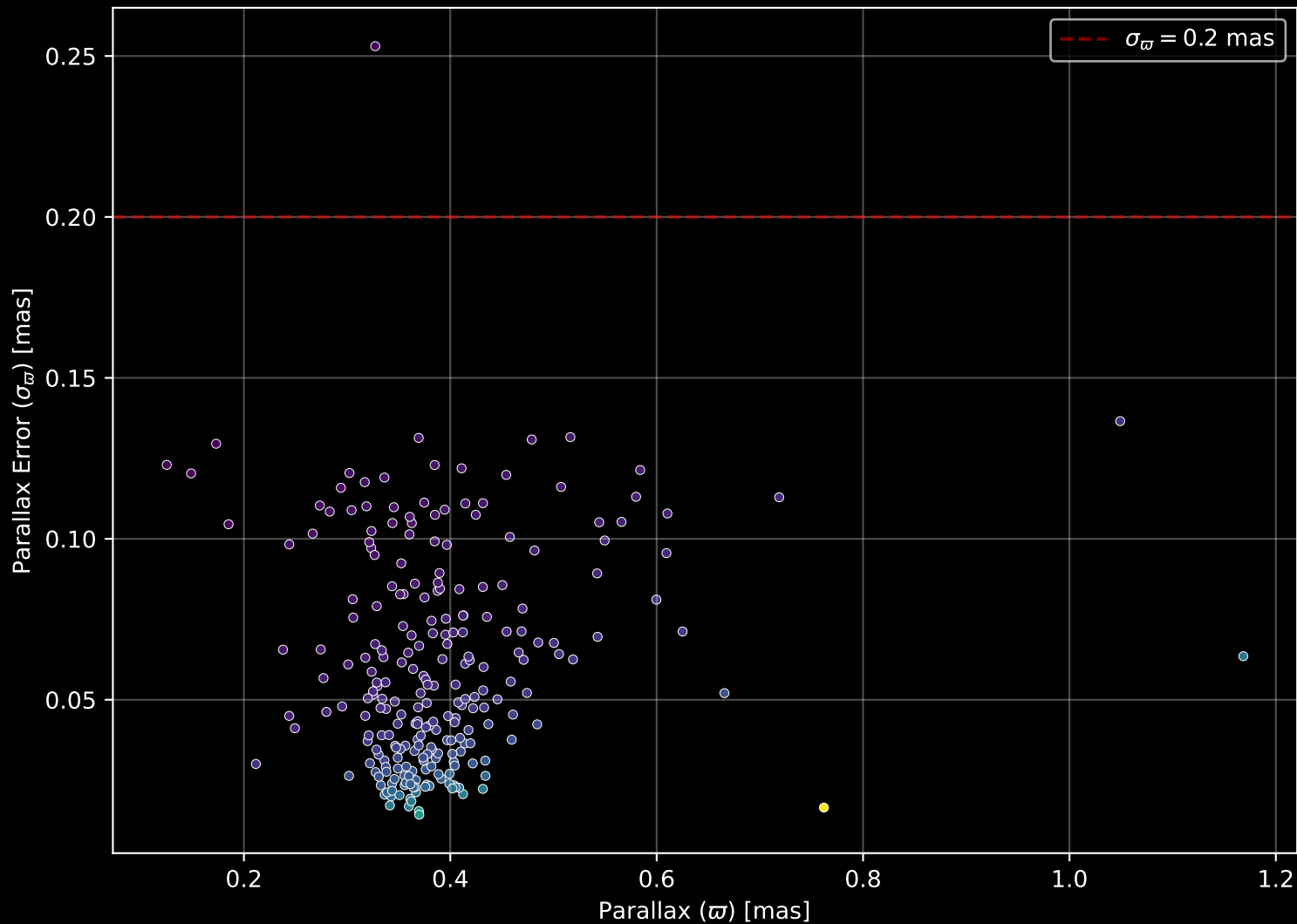
Gaia Cluster: [UFMG_2] Parallax Quality (n= 247)
