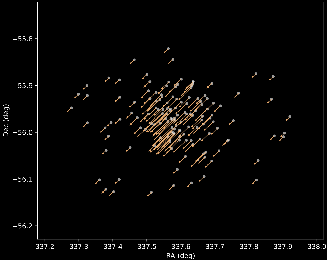
Gaia DR3 Cluster 3 Proper Motion Vectors (n=142)
