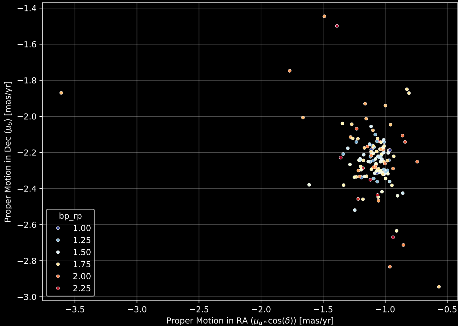
Gaia Cluster: [UFMG_3] Proper Motion Diagram (n= 135)
