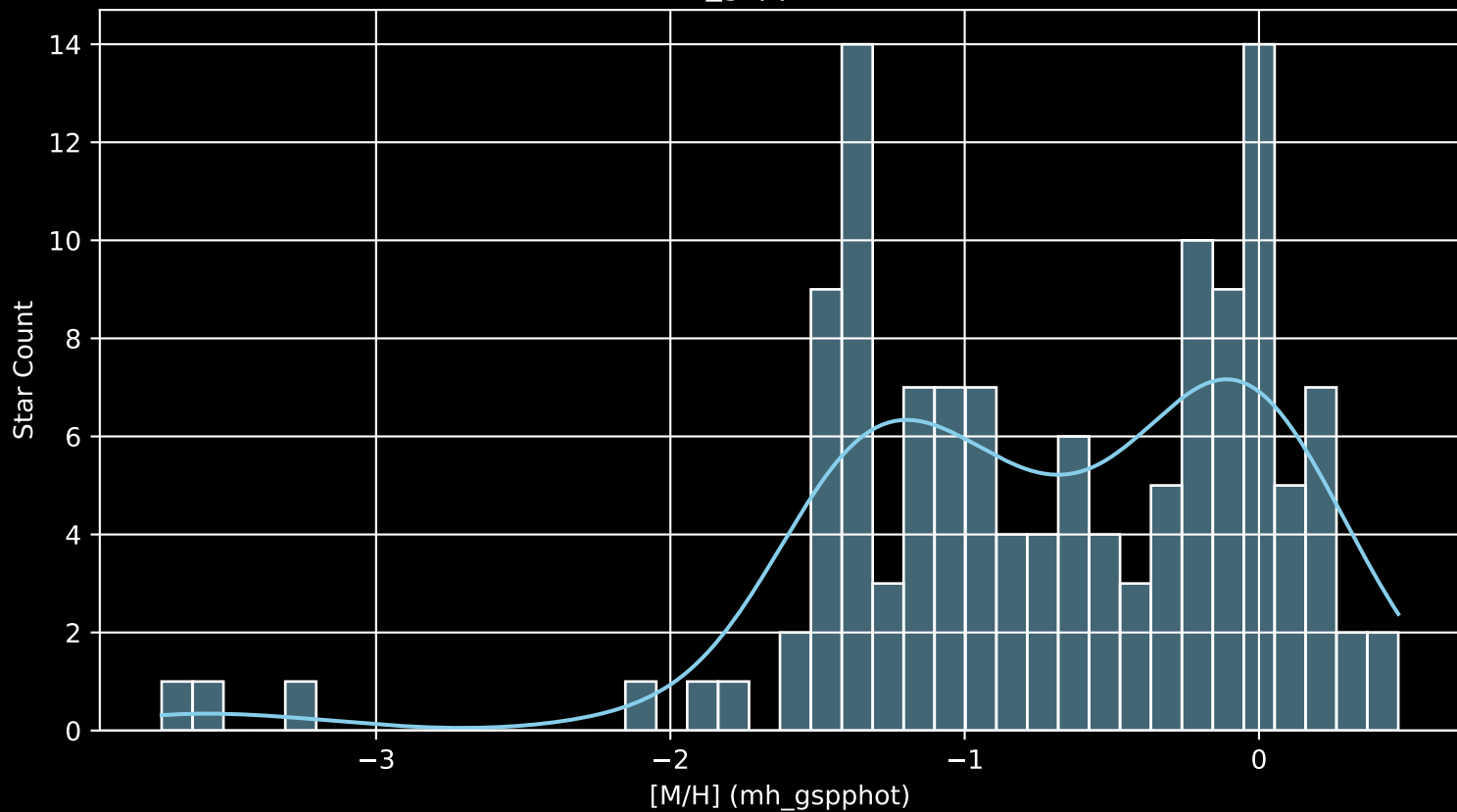
Gaia Cluster: [UFMG_3 [M/H] (mh_gspphot) (n= 130)
