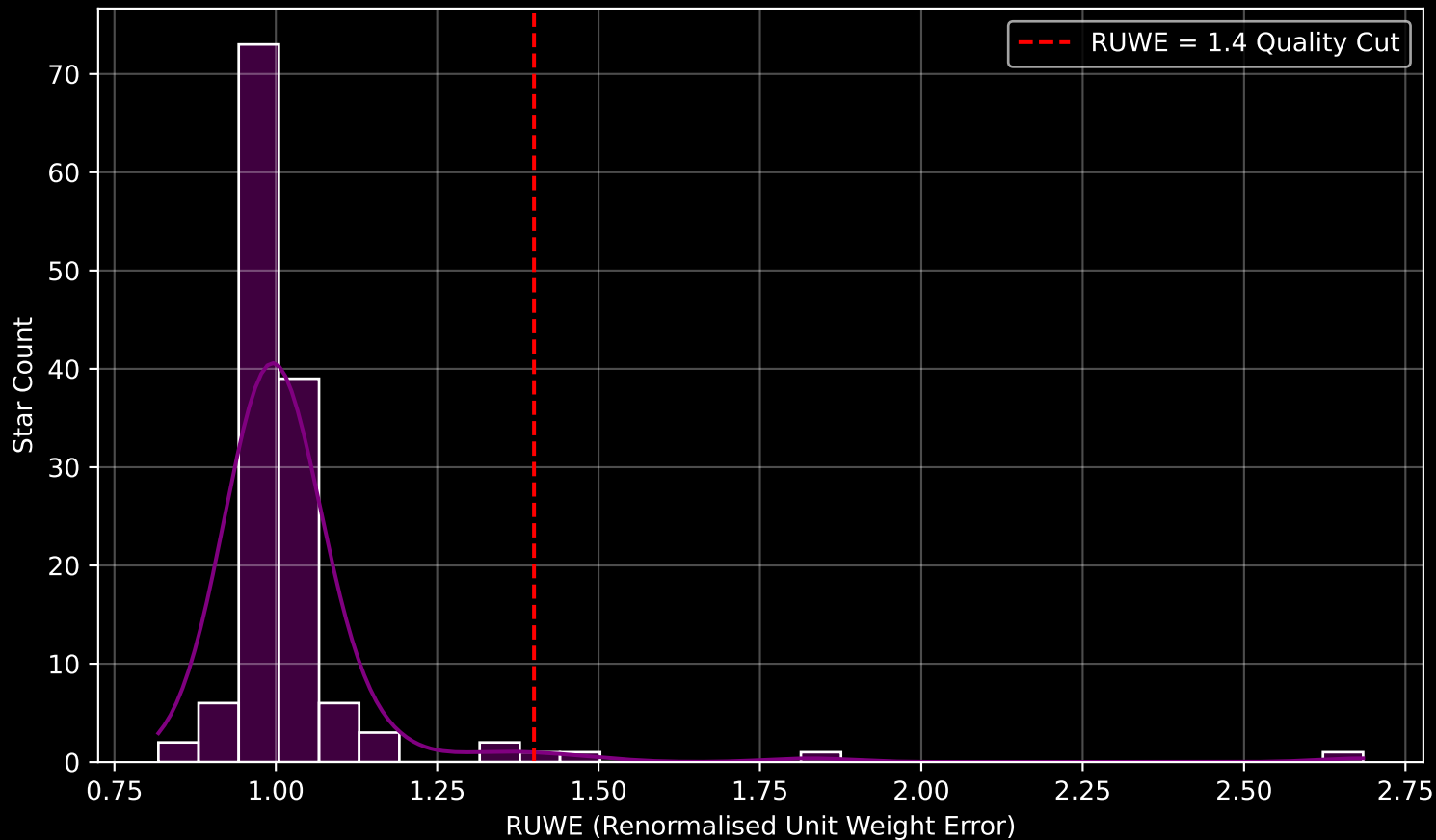
Gaia Cluster: [UFMG_3] RUWE Distribution (n= 135)
