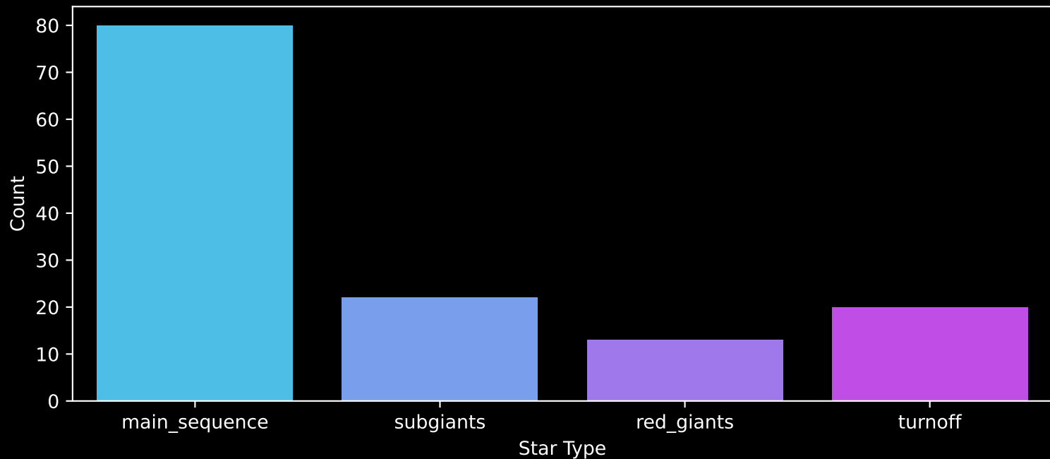
Gaia Cluster: [UFMG_3] Count plot of Star Type
