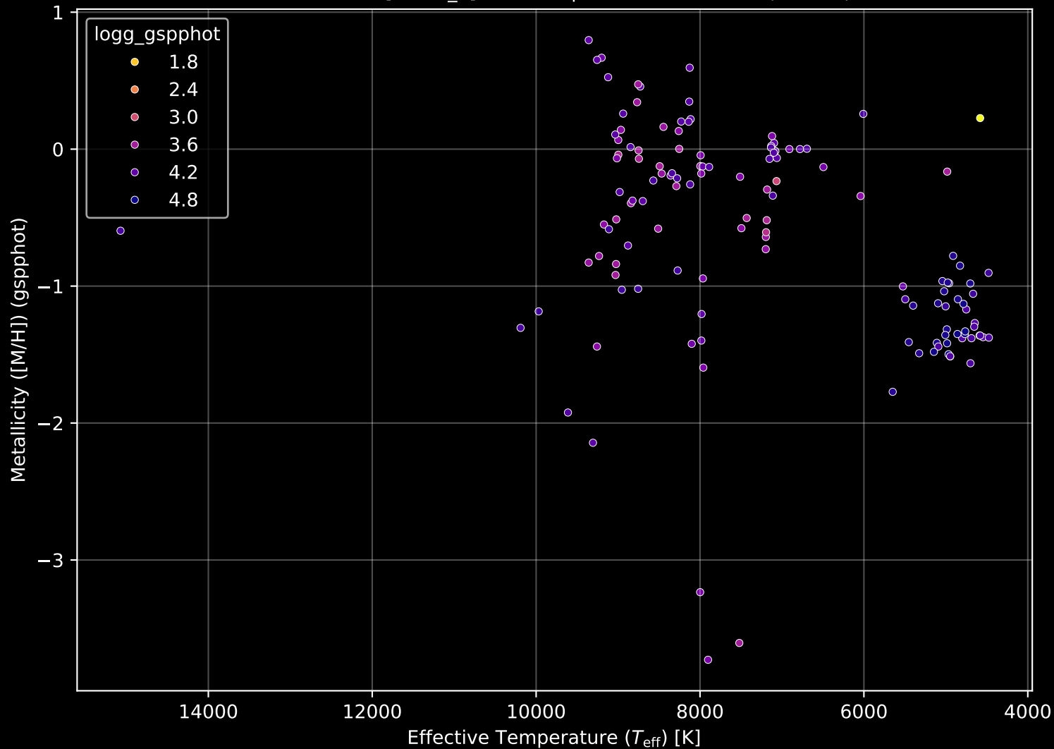
Gaia Cluster: [UFMG_3] Stellar Population Parameters (n= 135)
