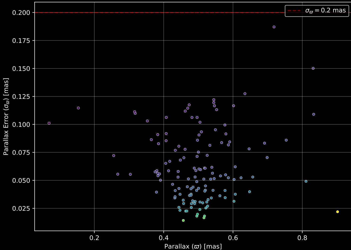
Gaia Cluster: [UFMG_3] Parallax Quality (n= 135)
