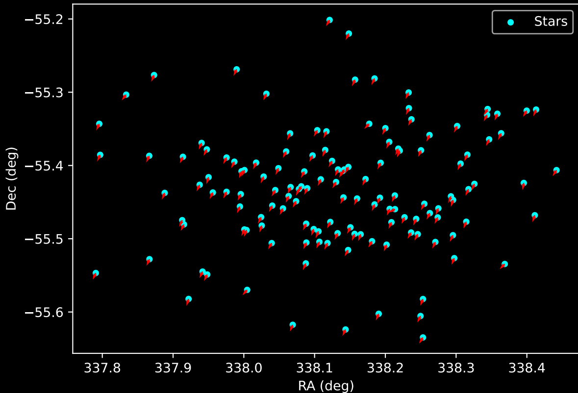
Gaia Cluster: [UFMG_3] Proper Motion Vectors for Gaia Star Field (n= 135)
