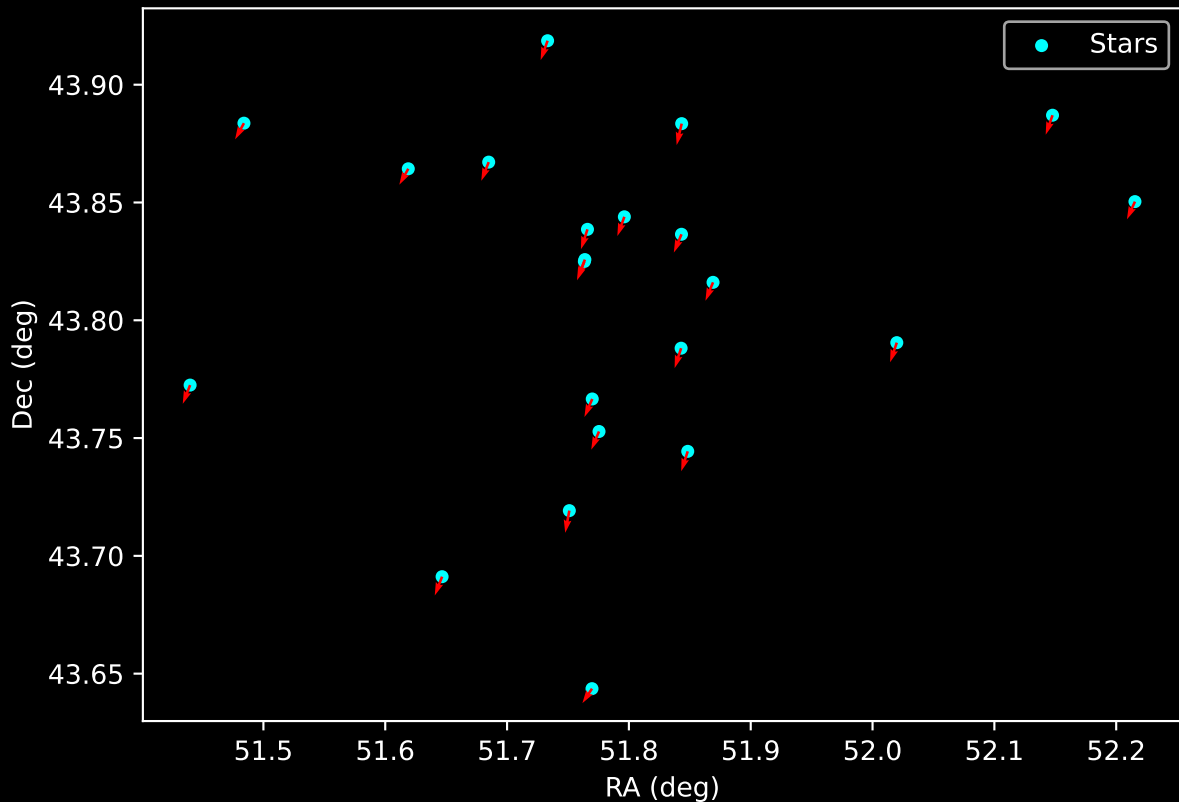
Gaia Cluster: [UPK_126] Proper Motion Vectors for Gaia Star Field (n= 22)
