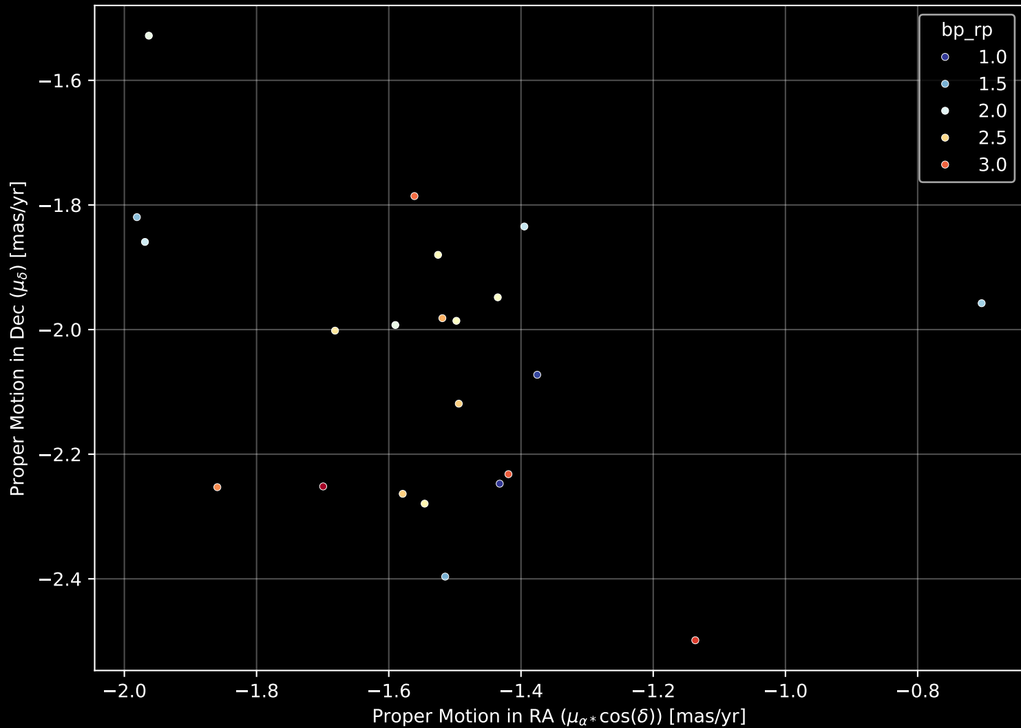
Gaia Cluster: [UPK_126] Proper Motion Diagram (n= 22)
