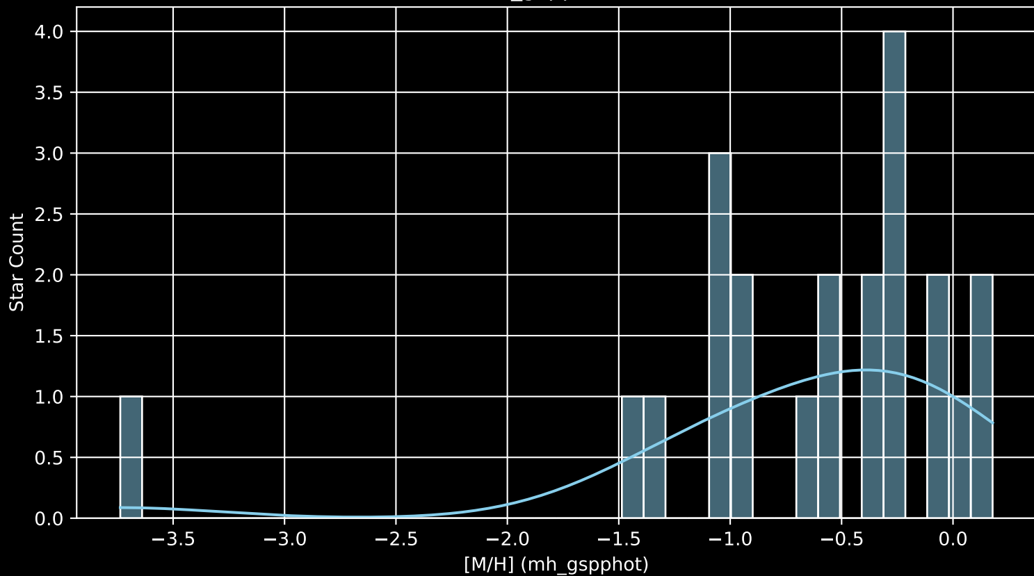
Gaia Cluster: [UPK_126 [M/H] (mh_gspphot) (n= 22)
