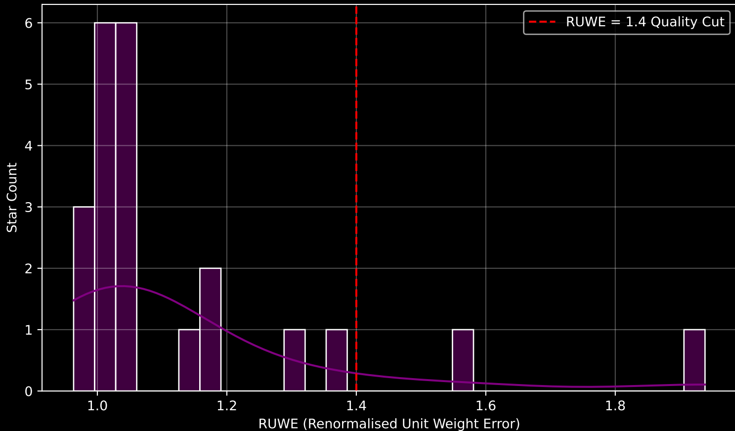
Gaia Cluster: [UPK_126] RUWE Distribution (n= 22)
