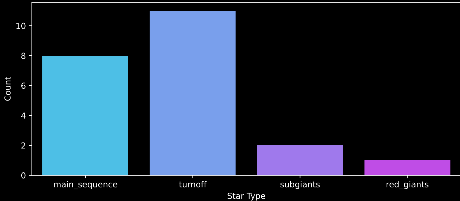
Gaia Cluster: [UPK_126] Count plot of Star Type
