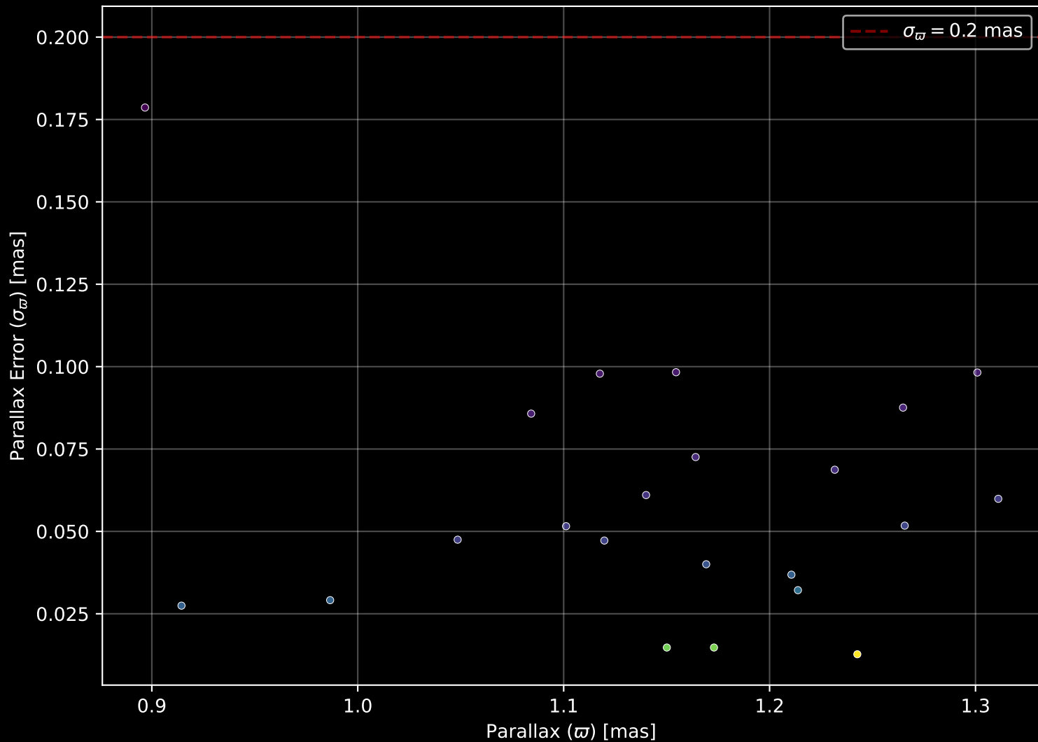
Gaia Cluster: [UPK_126] Parallax Quality (n= 22)
