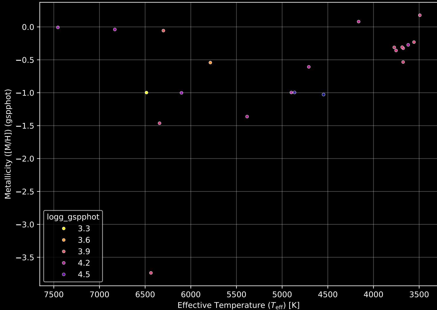
Gaia Cluster: [UPK_126] Stellar Population Parameters (n= 22)
