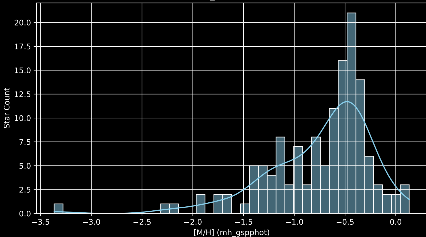
Gaia Cluster: [UPK_13 [M/H] (mh_gspphot) (n= 136)
