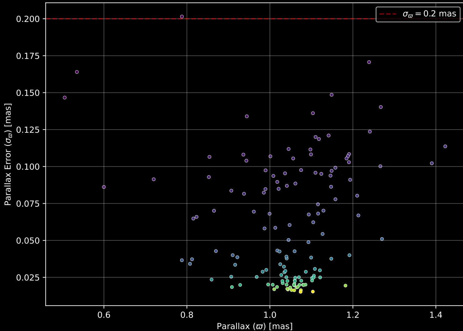
Gaia Cluster: [UPK_13] Parallax Quality (n= 136)
