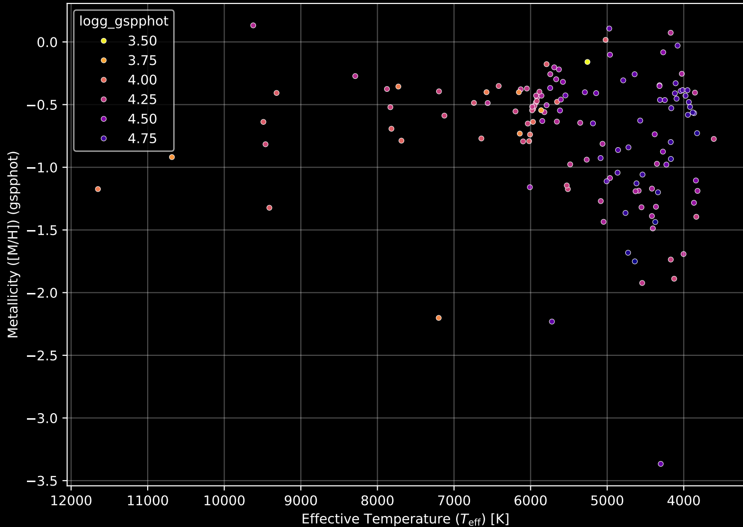
Gaia Cluster: [UPK_13] Stellar Population Parameters (n= 136)
