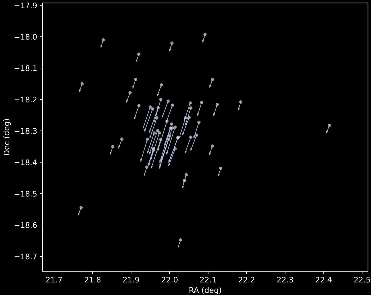
Gaia DR3 Cluster 1 Proper Motion Vectors (n=54)
