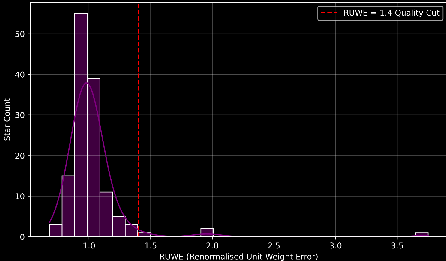
Gaia Cluster: [UPK_13] RUWE Distribution (n= 135)
