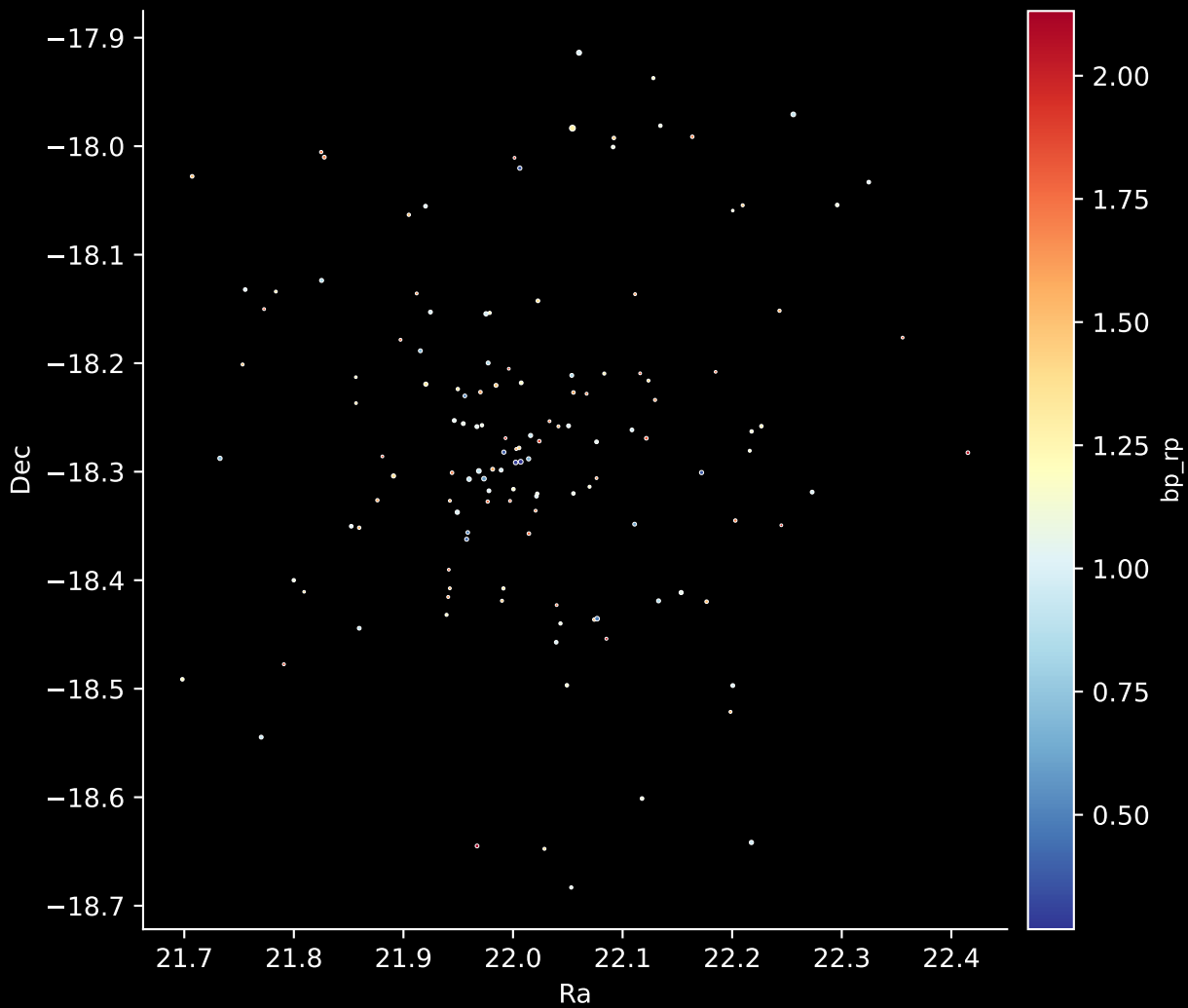
Gaia Cluster: [UPK_13] Stars: 136
