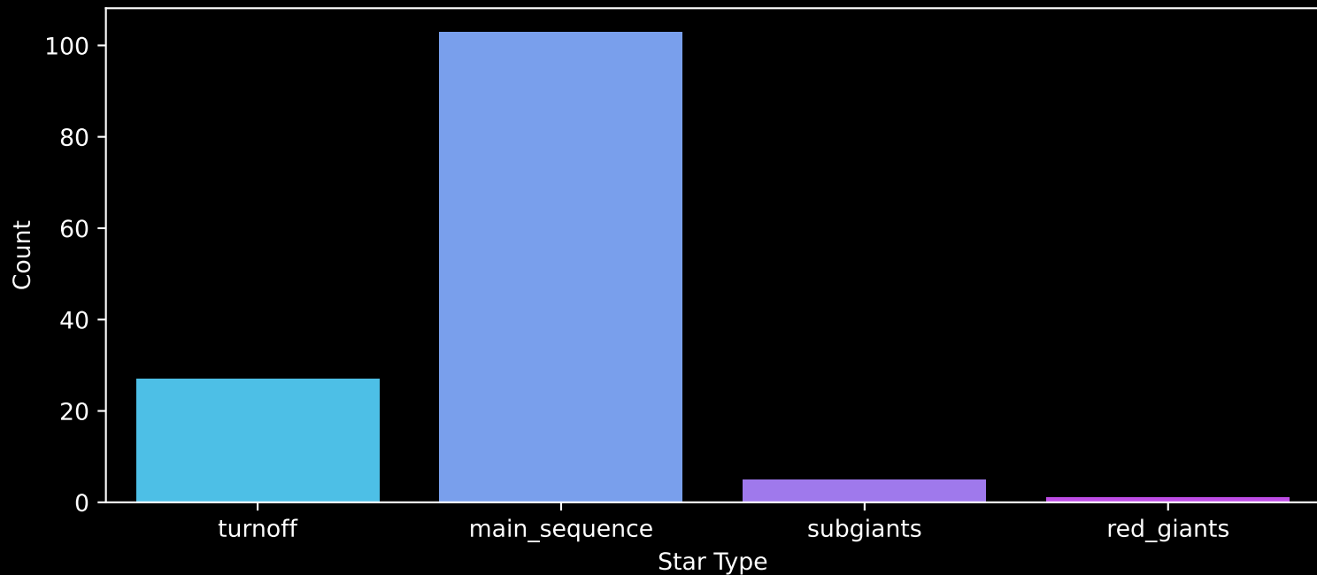
Gaia Cluster: [UPK_13] Count plot of Star Type
