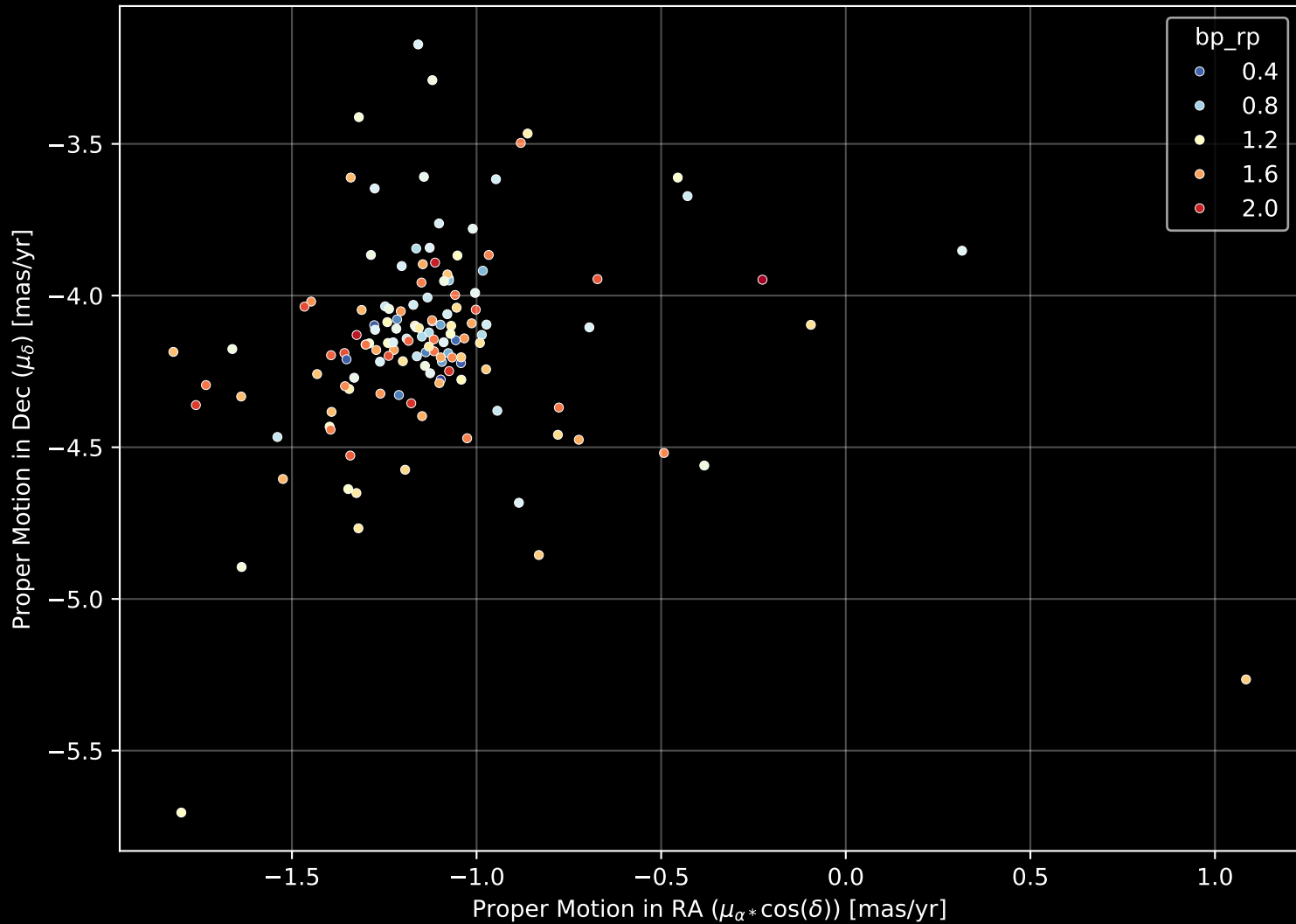
Gaia Cluster: [UPK_13] Proper Motion Diagram (n= 136)
