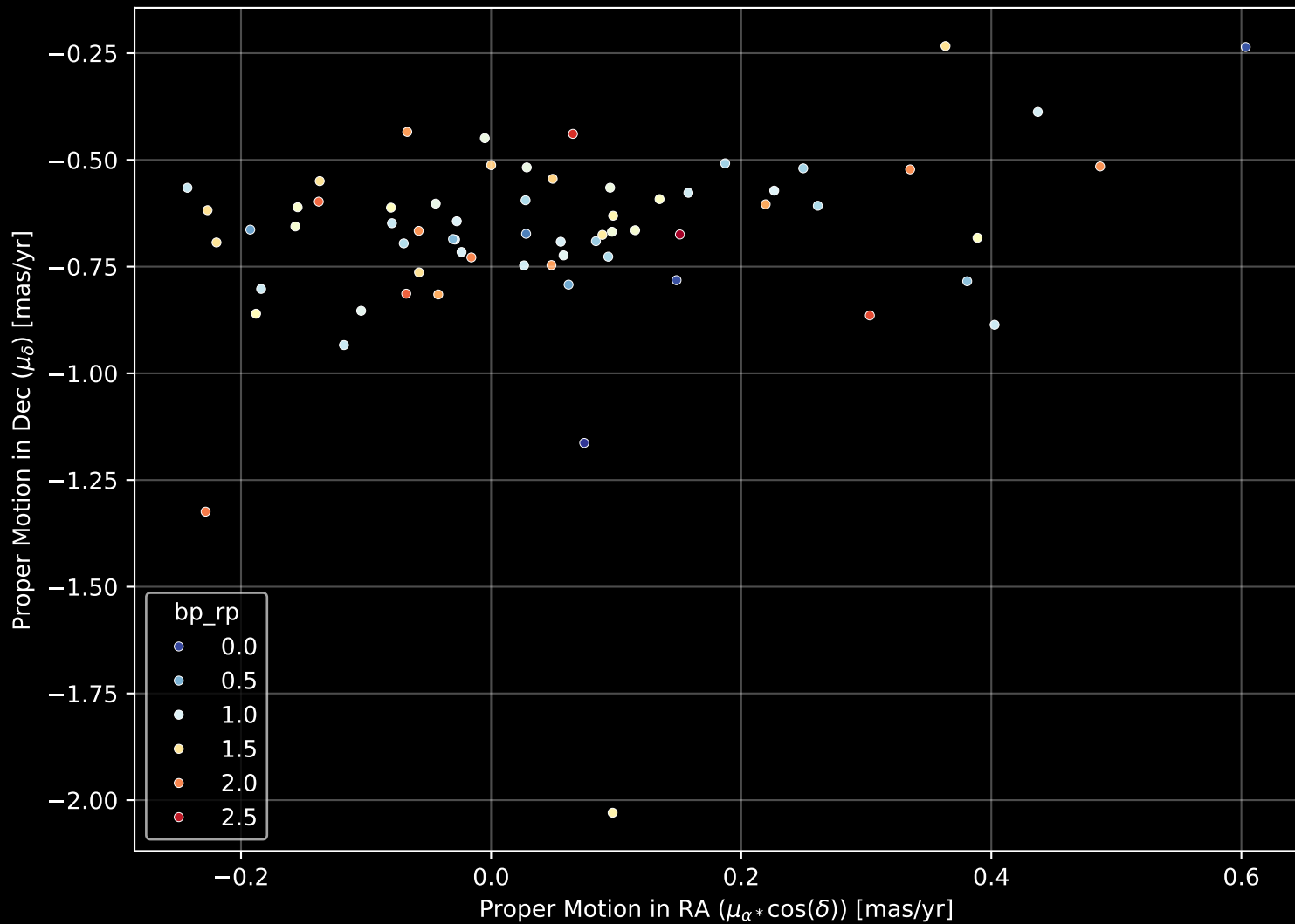
Gaia Cluster: [UPK_136] Proper Motion Diagram (n= 66)
