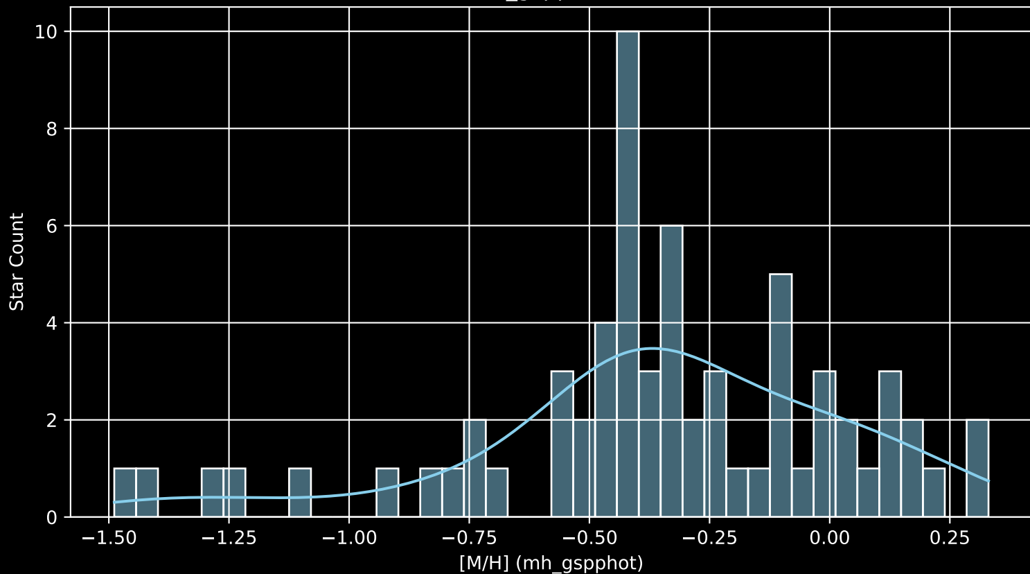
Gaia Cluster: [UPK_136 [M/H] (mh_gspphot) (n= 66)
