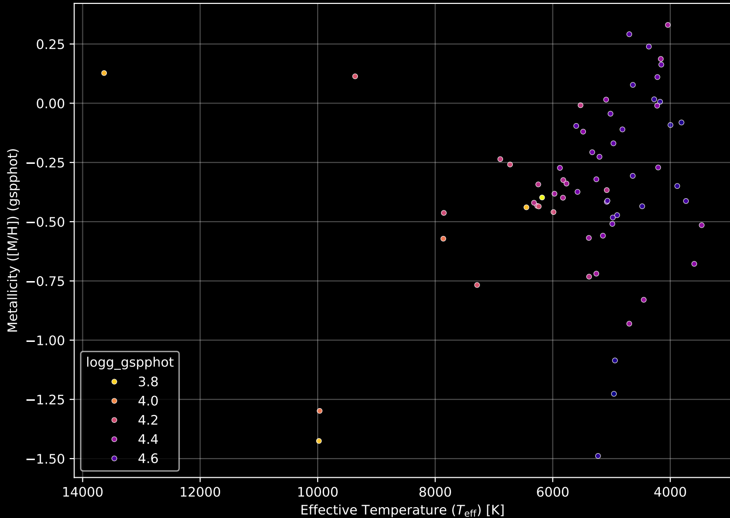
Gaia Cluster: [UPK_136] Stellar Population Parameters (n= 66)
