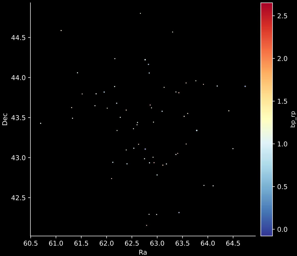
Gaia Cluster: [UPK_136] Stars: 66
