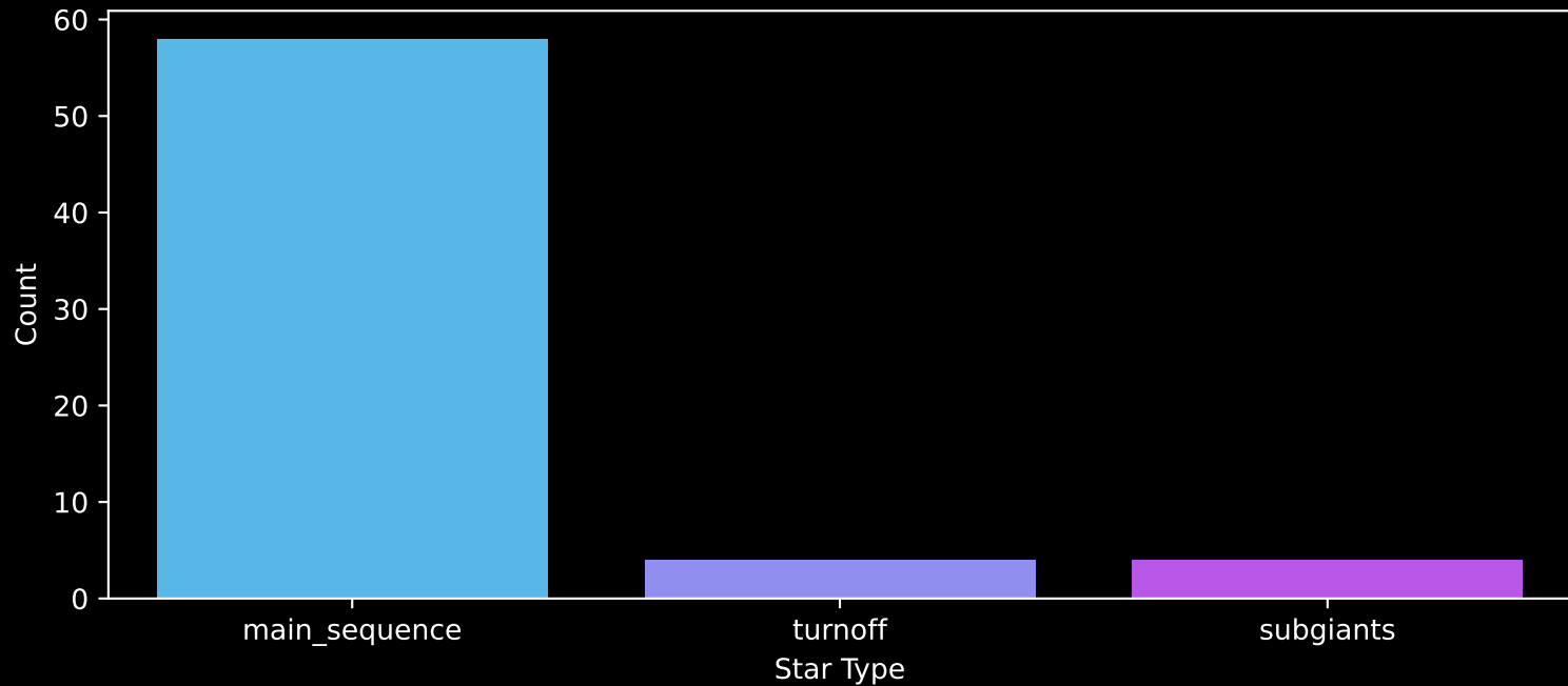
Gaia Cluster: [UPK_136] Count plot of Star Type
