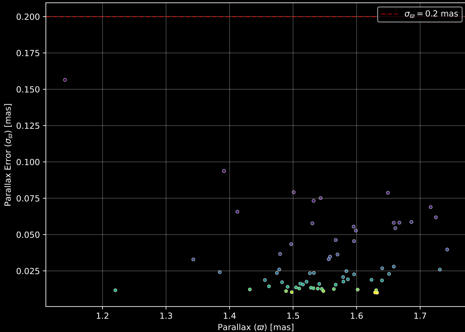
Gaia Cluster: [UPK_136] Parallax Quality (n= 66)
