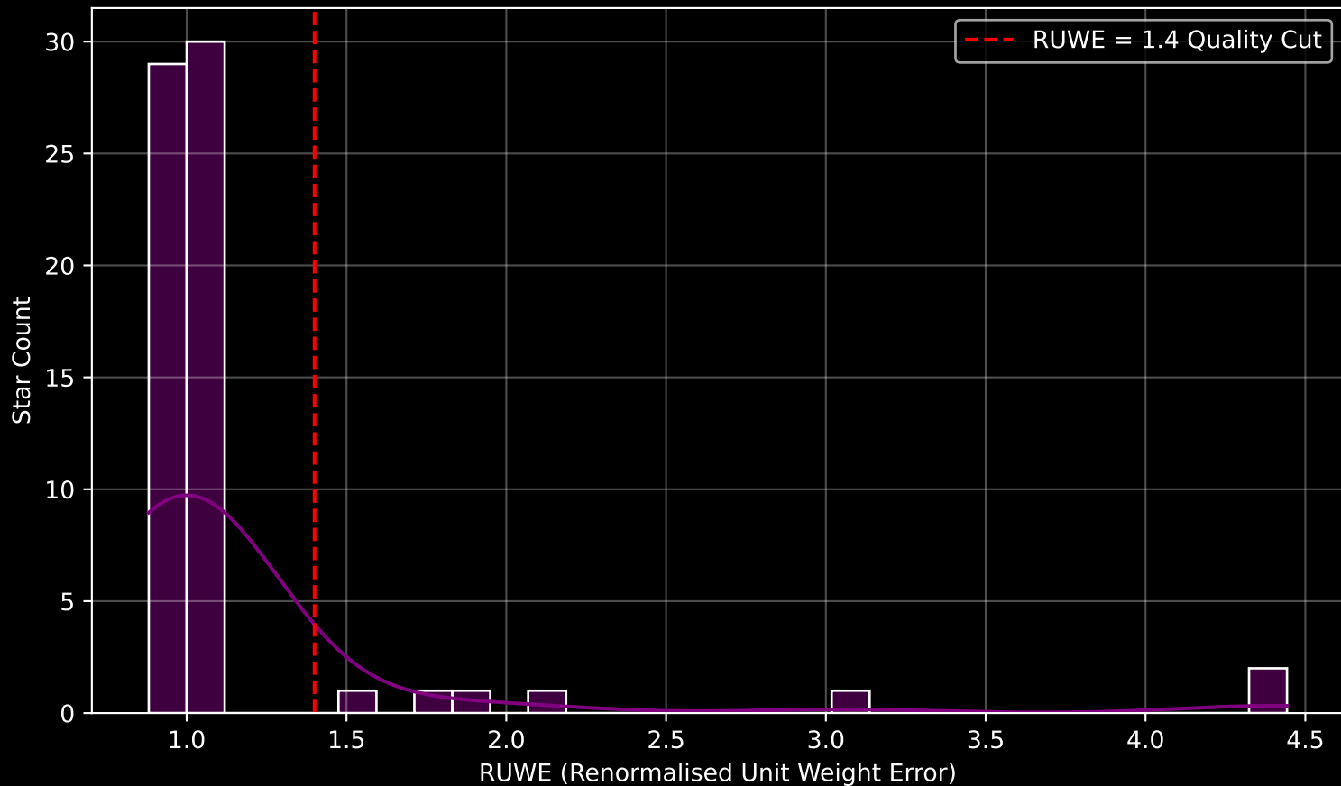
Gaia Cluster: [UPK_136] RUWE Distribution (n= 66)
