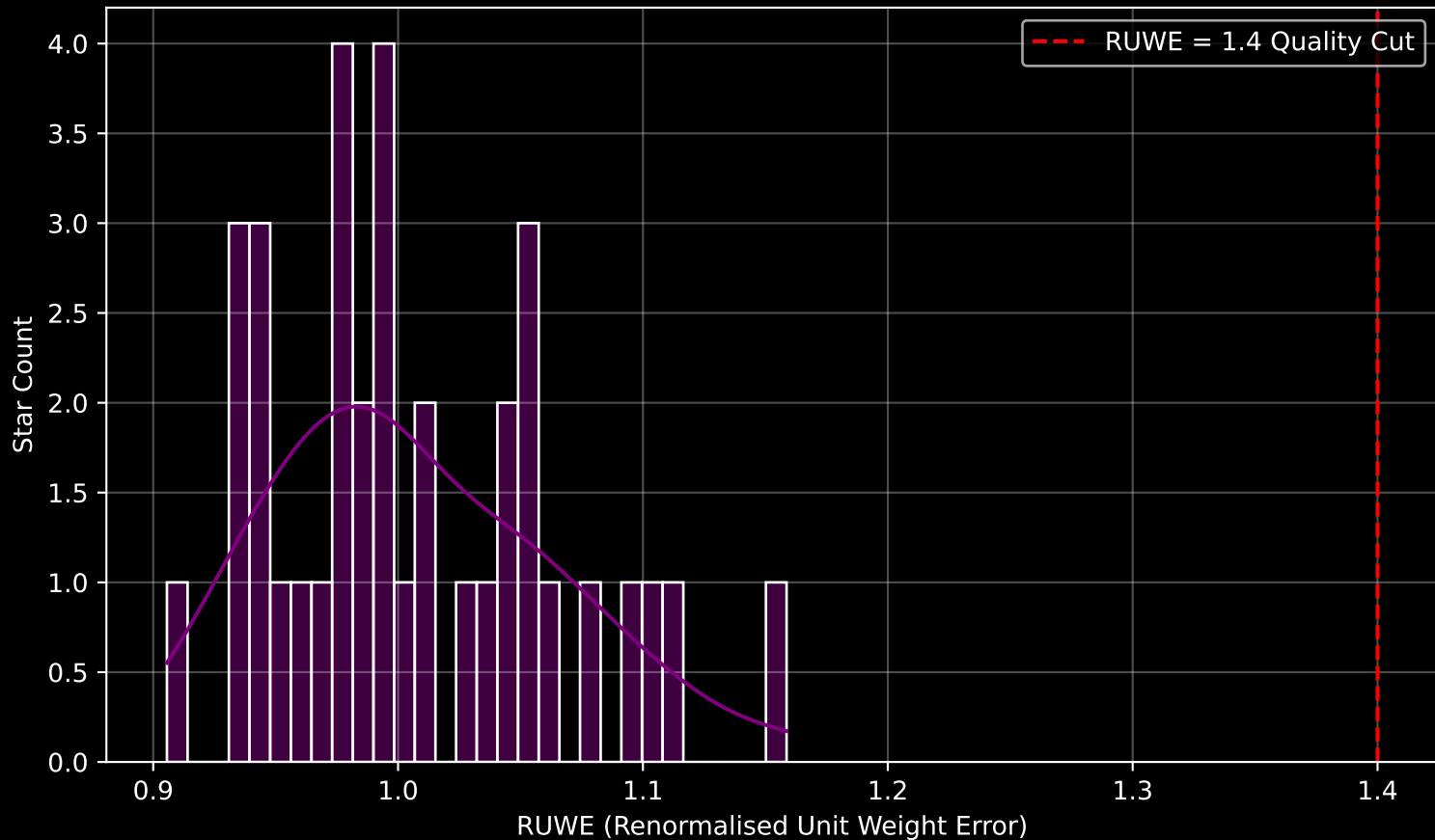
Gaia Cluster: [UPK_137] RUWE Distribution (n= 36)
