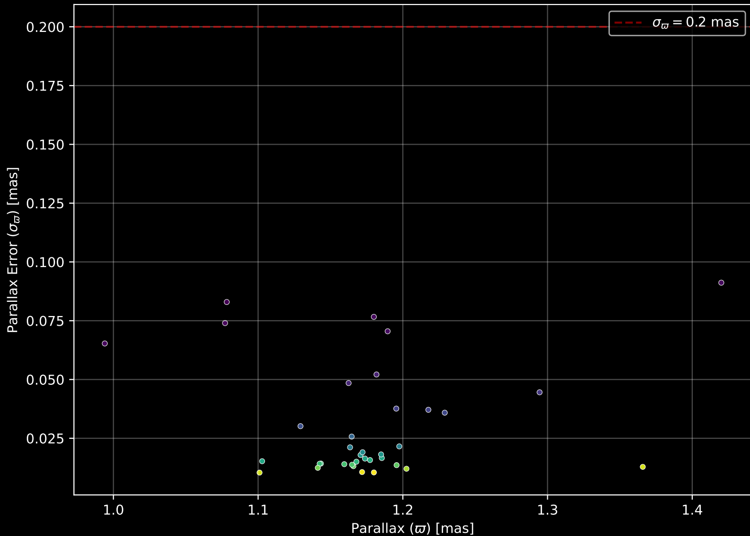
Gaia Cluster: [UPK_137] Parallax Quality (n= 36)
