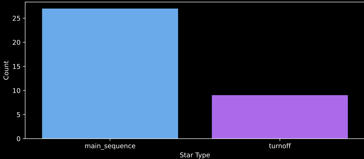
Gaia Cluster: [UPK_137] Count plot of Star Type
