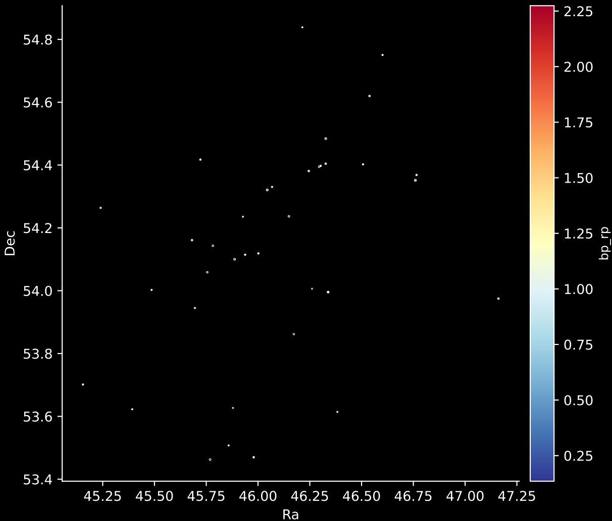
Gaia Cluster: [UPK_137] Stars: 36
