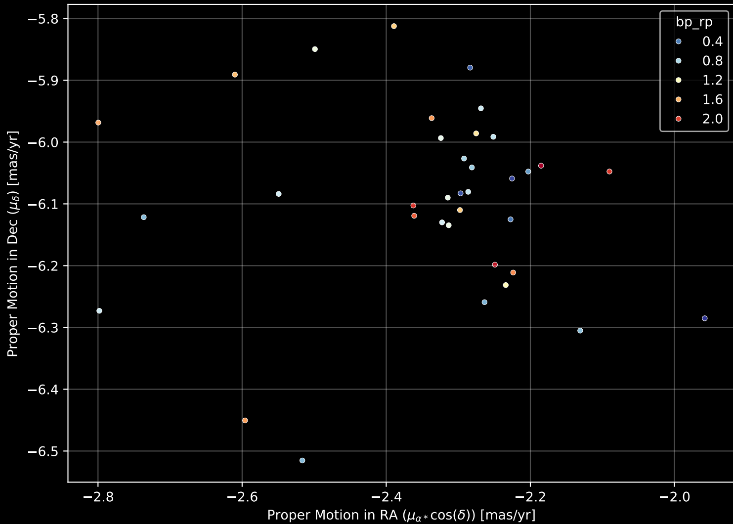
Gaia Cluster: [UPK_137] Proper Motion Diagram (n= 36)
