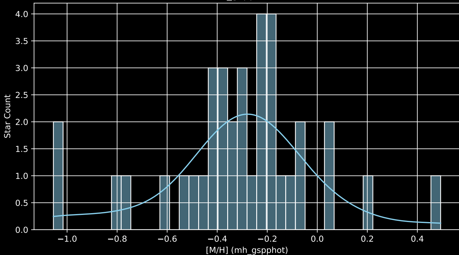
Gaia Cluster: [UPK_137 [M/H] (mh_gspphot) (n= 36)
