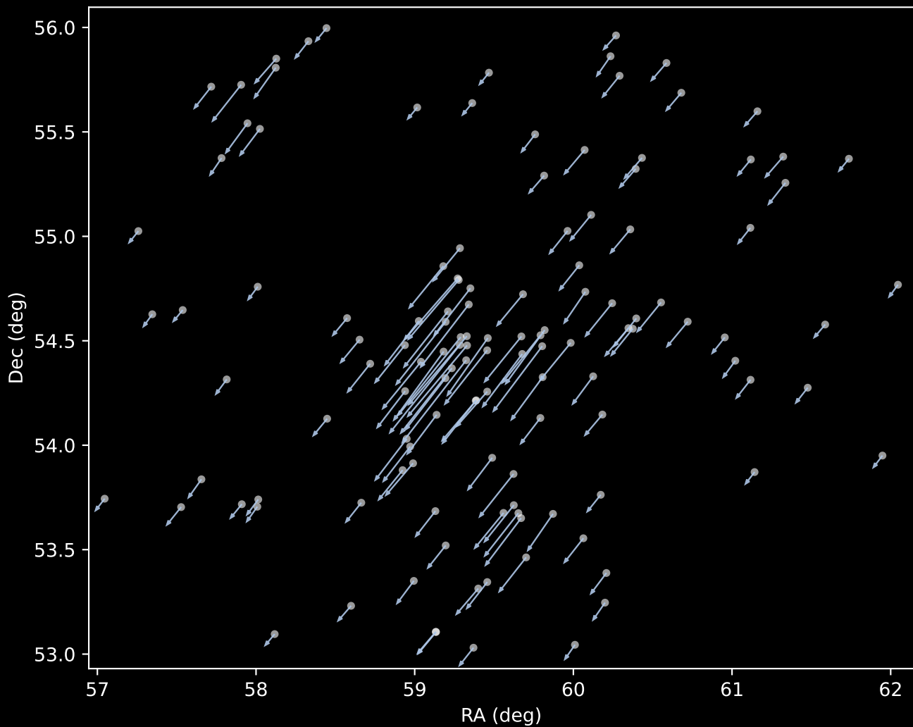
Gaia DR3 Cluster 1 Proper Motion Vectors (n=127)
