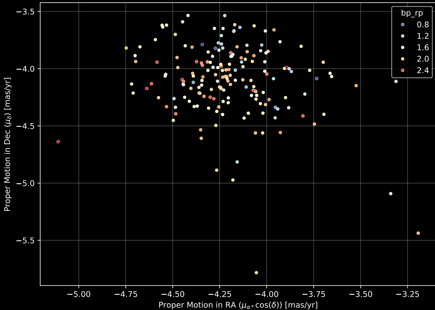
Gaia Cluster: [UPK_150] Proper Motion Diagram (n= 178)
