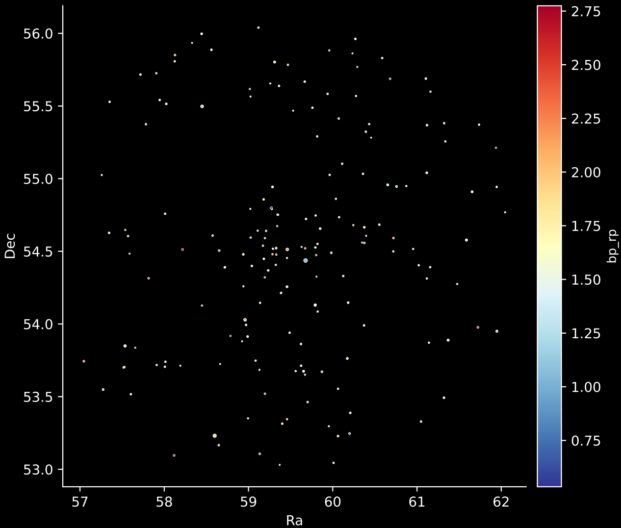
Gaia Cluster: [UPK_150] Stars: 178
