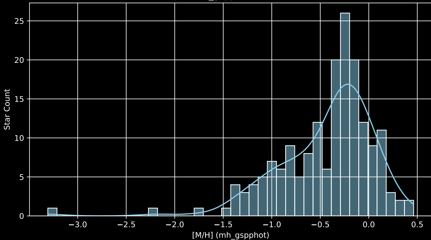
Gaia Cluster: [UPK_150 [M/H] (mh_gspphot) (n= 178)
