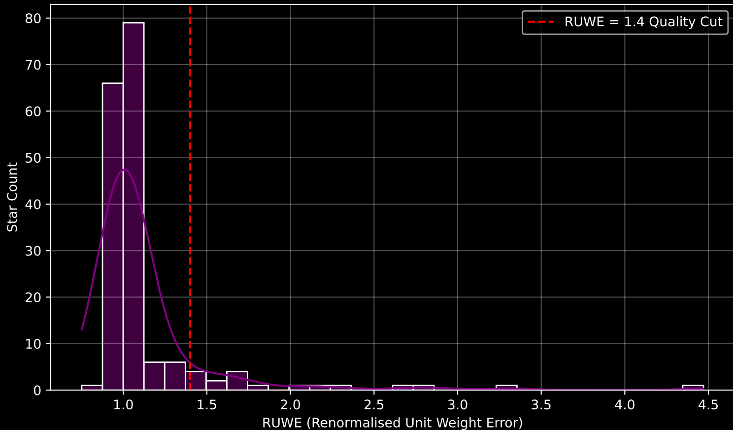
Gaia Cluster: [UPK_150] RUWE Distribution (n= 176)
