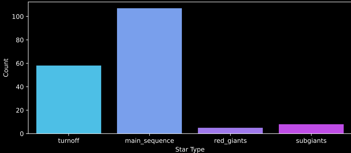
Gaia Cluster: [UPK_150] Count plot of Star Type
