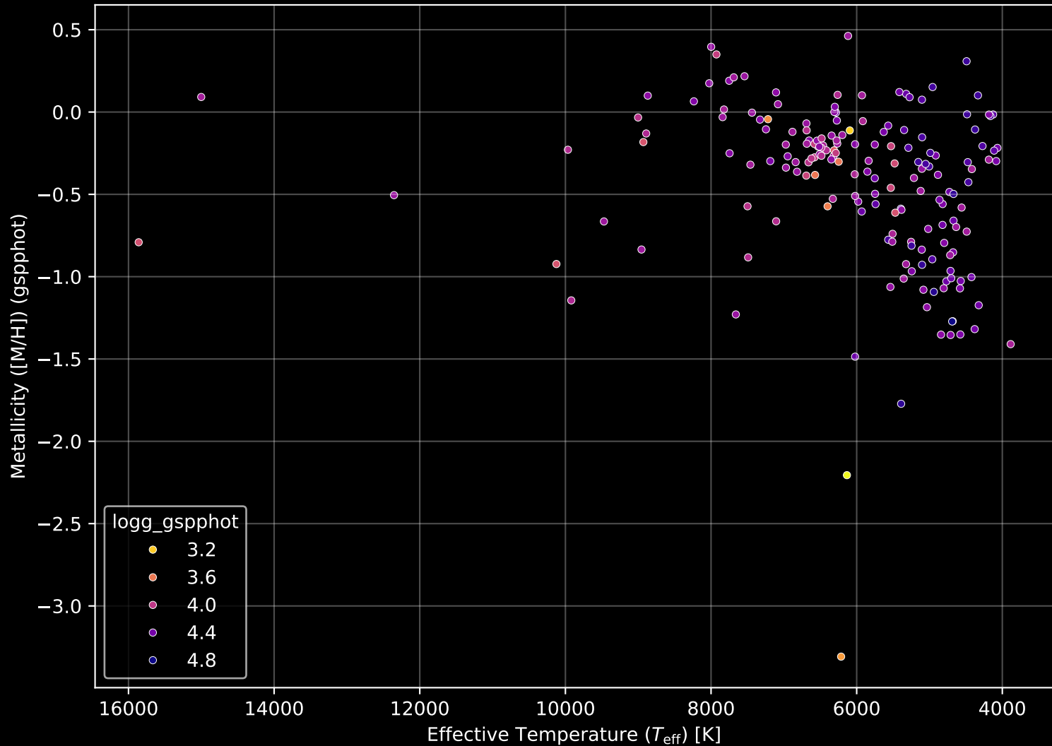
Gaia Cluster: [UPK_150] Stellar Population Parameters (n= 178)
