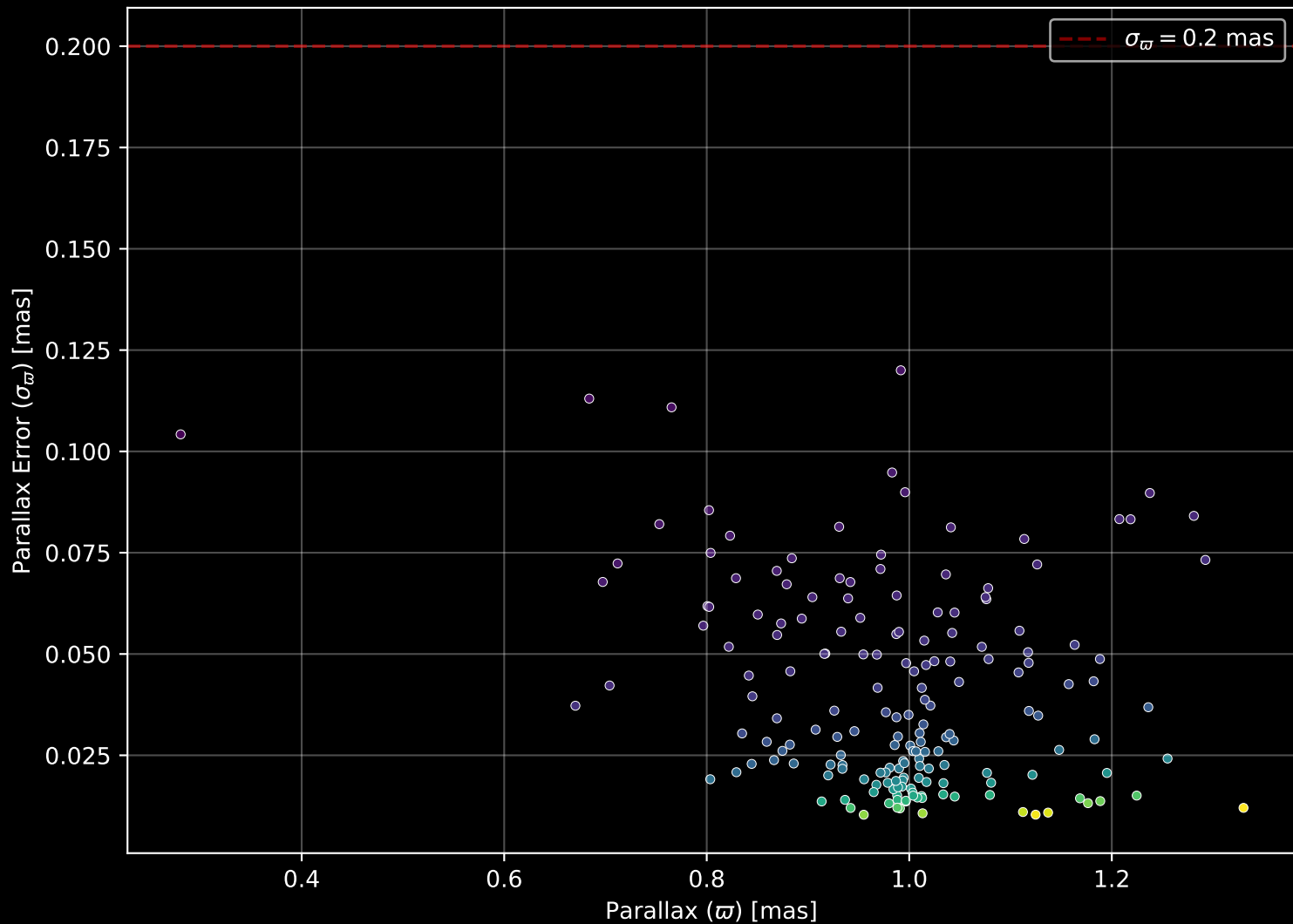
Gaia Cluster: [UPK_150] Parallax Quality (n= 178)
