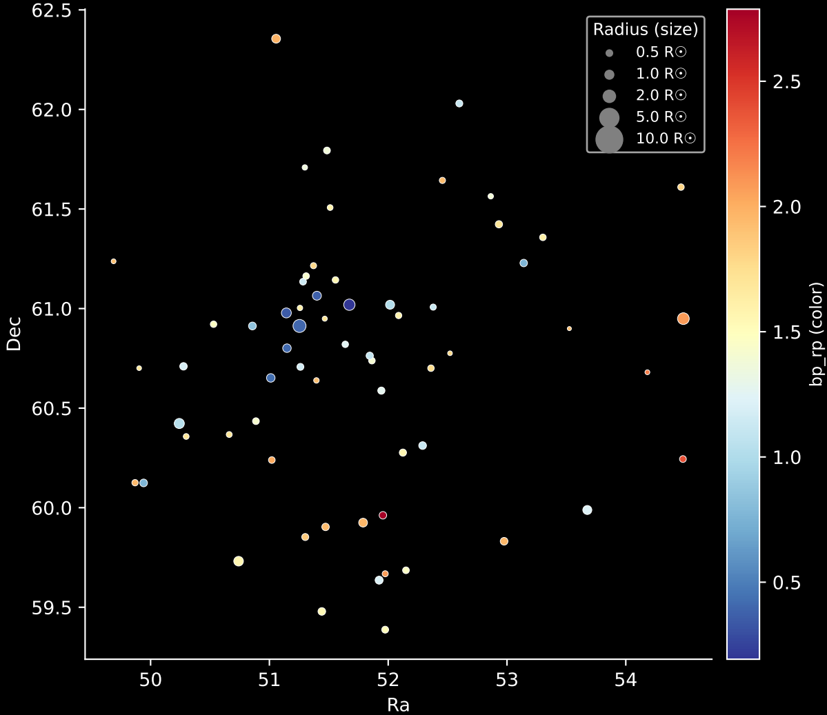
Gaia Cluster: [UPK_155] Stars: 64
