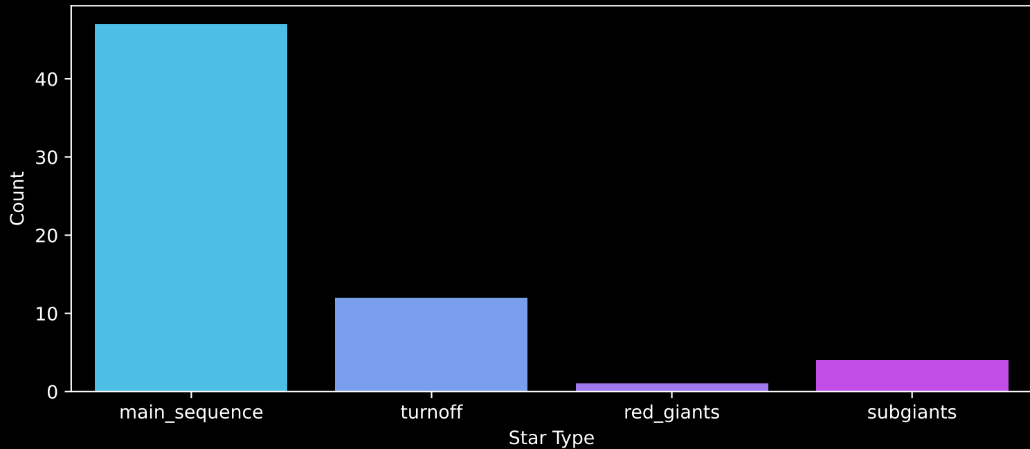
Gaia Cluster: [UPK_155] Count plot of Star Type
