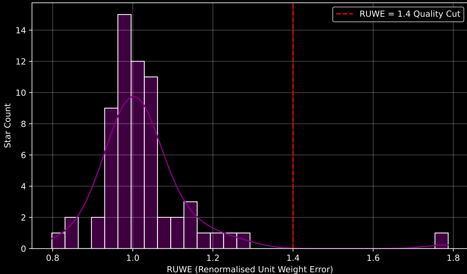
Gaia Cluster: [UPK_155] RUWE Distribution (n= 64)
