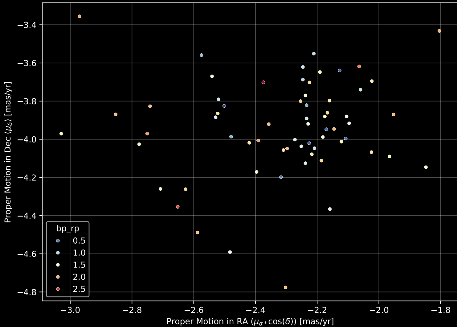
Gaia Cluster: [UPK_155] Proper Motion Diagram (n= 64)
