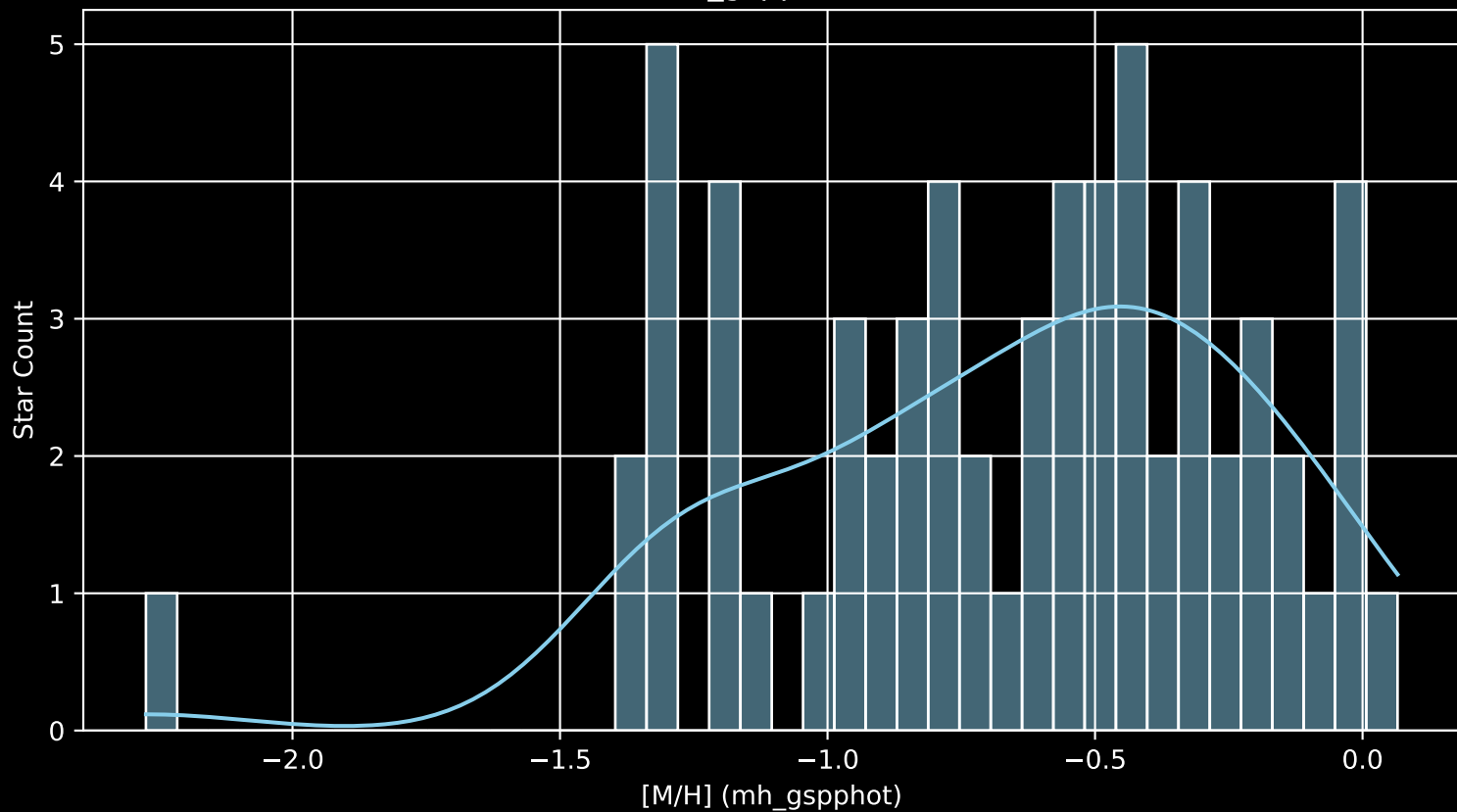
Gaia Cluster: [UPK_155 [M/H] (mh_gspphot) (n= 64)
