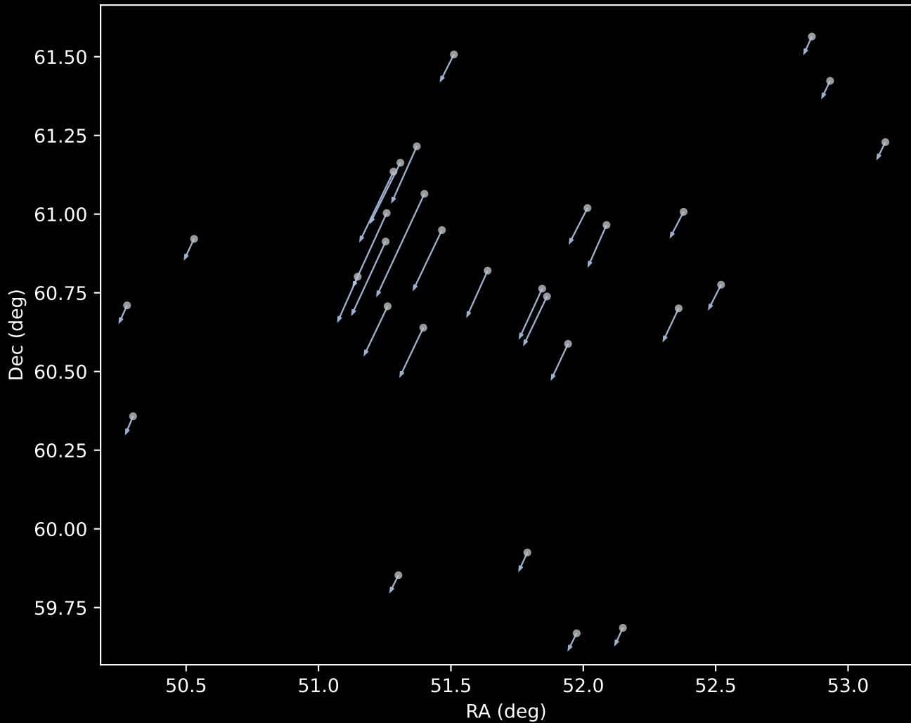
Gaia DR3 Cluster 1 Proper Motion Vectors (n=30)
