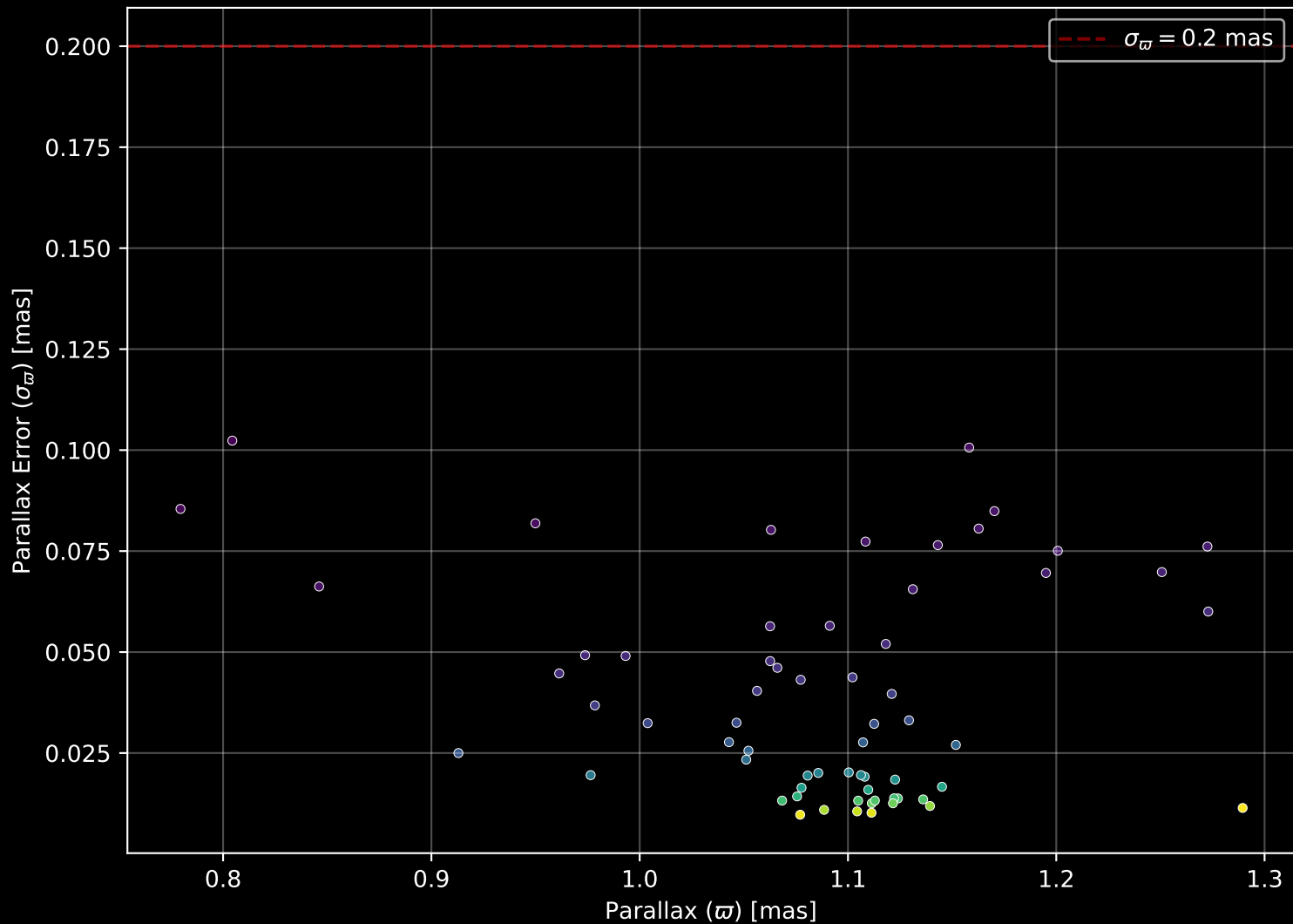
Gaia Cluster: [UPK_155] Parallax Quality (n= 64)
