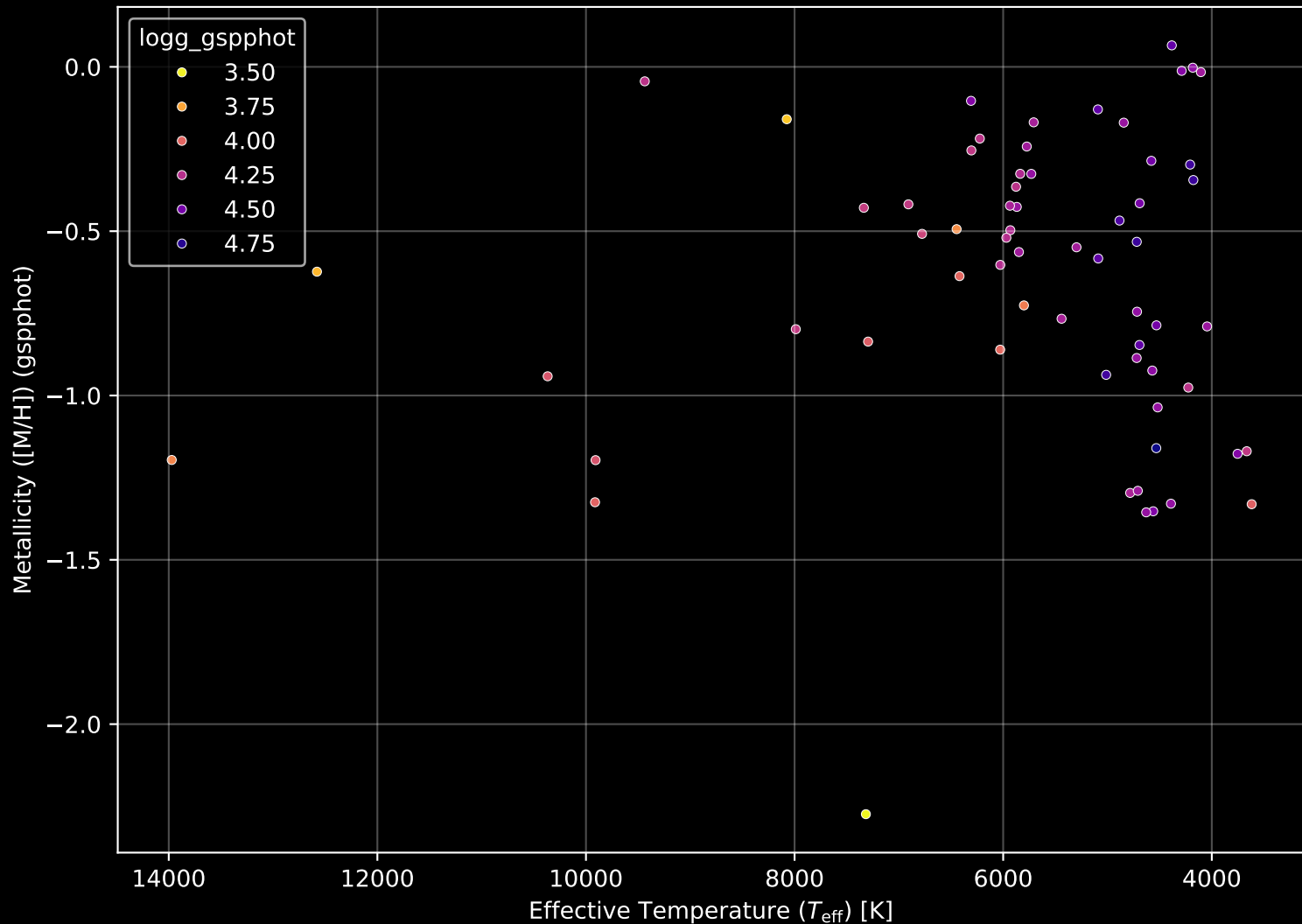
Gaia Cluster: [UPK_155] Stellar Population Parameters (n= 64)
