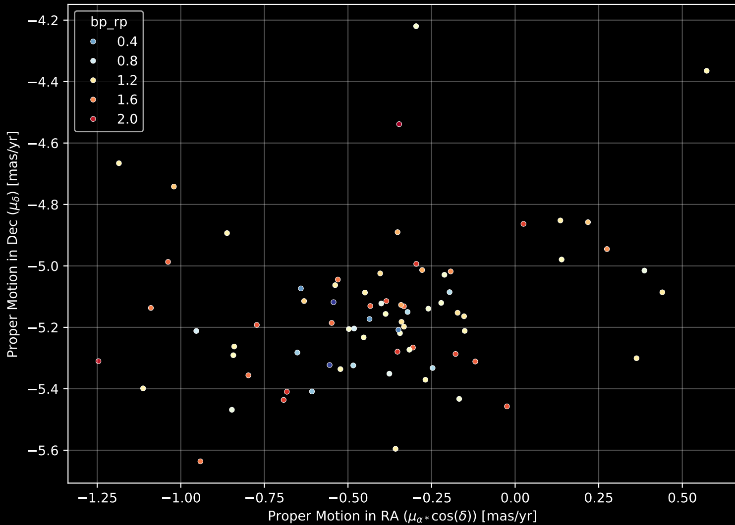
Gaia Cluster: [UPK_16] Proper Motion Diagram (n= 77)
