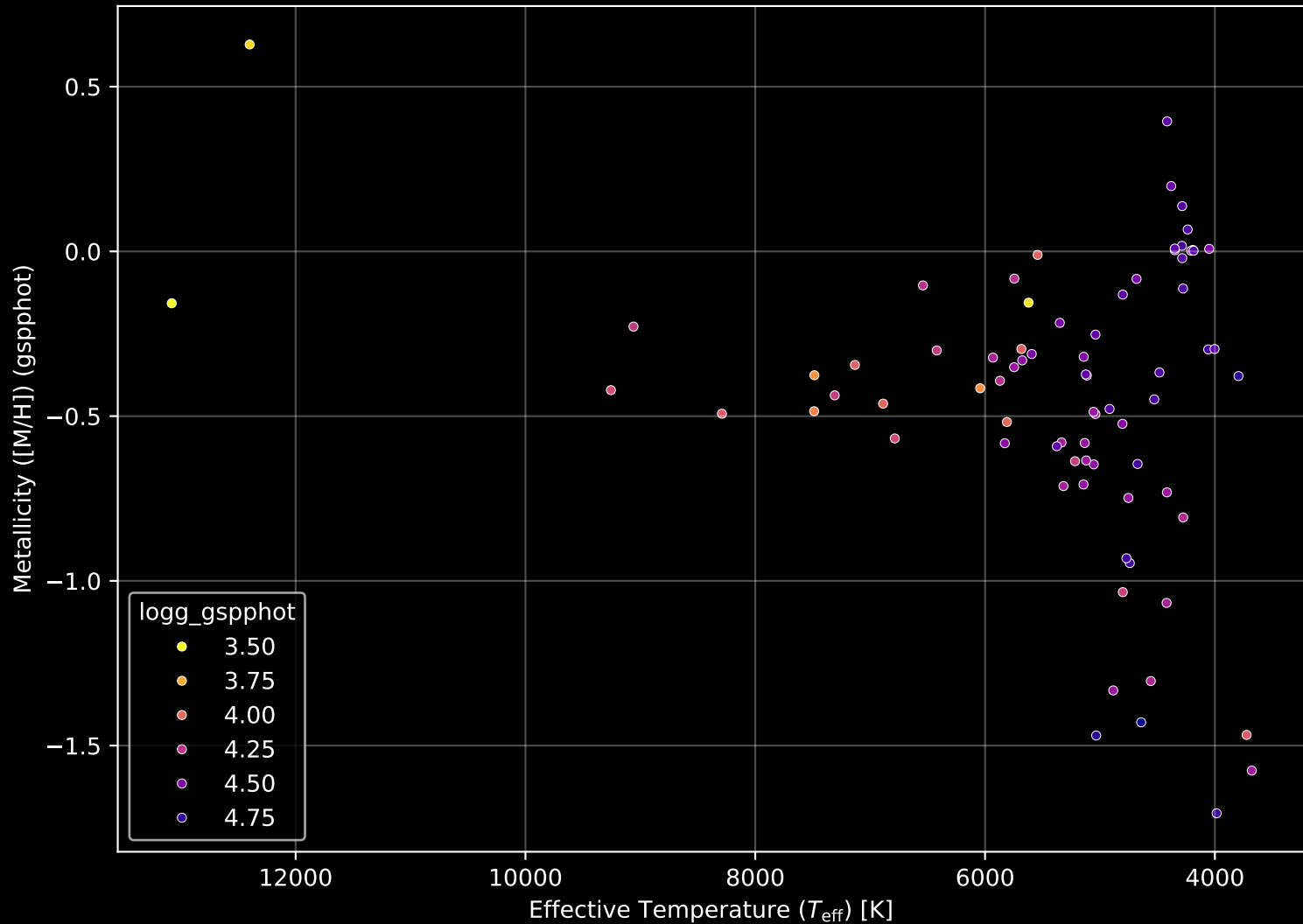
Gaia Cluster: [UPK_16] Stellar Population Parameters (n= 77)
