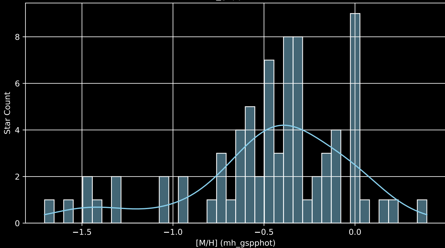
Gaia Cluster: [UPK_16 [M/H] (mh_gspphot) (n= 76)
