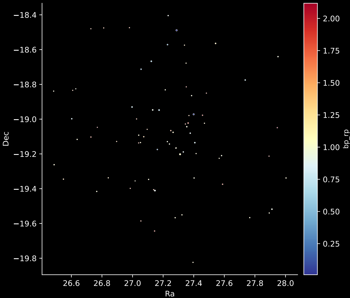
Gaia Cluster: [UPK_16] Stars: 77
