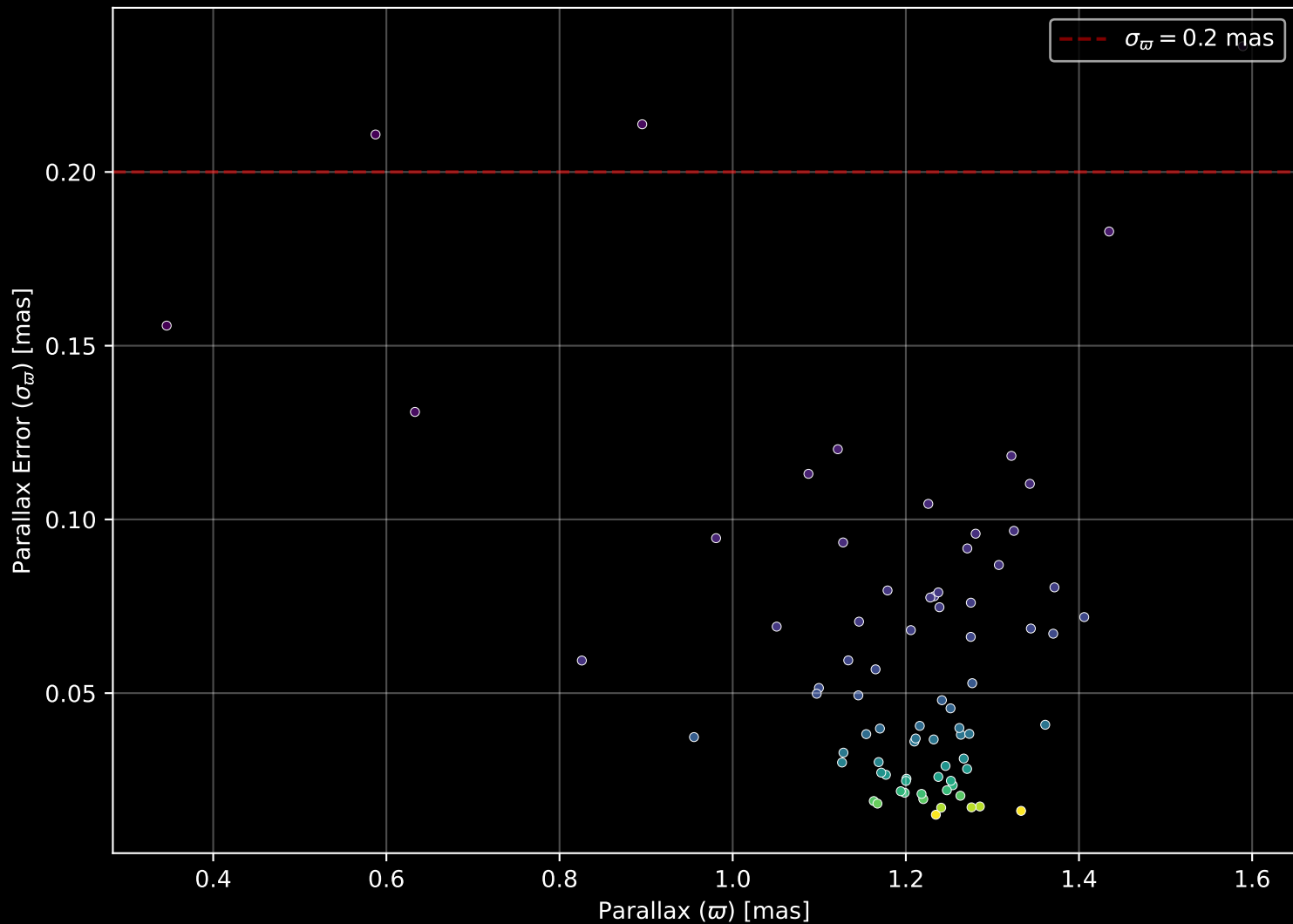
Gaia Cluster: [UPK_16] Parallax Quality (n= 77)
