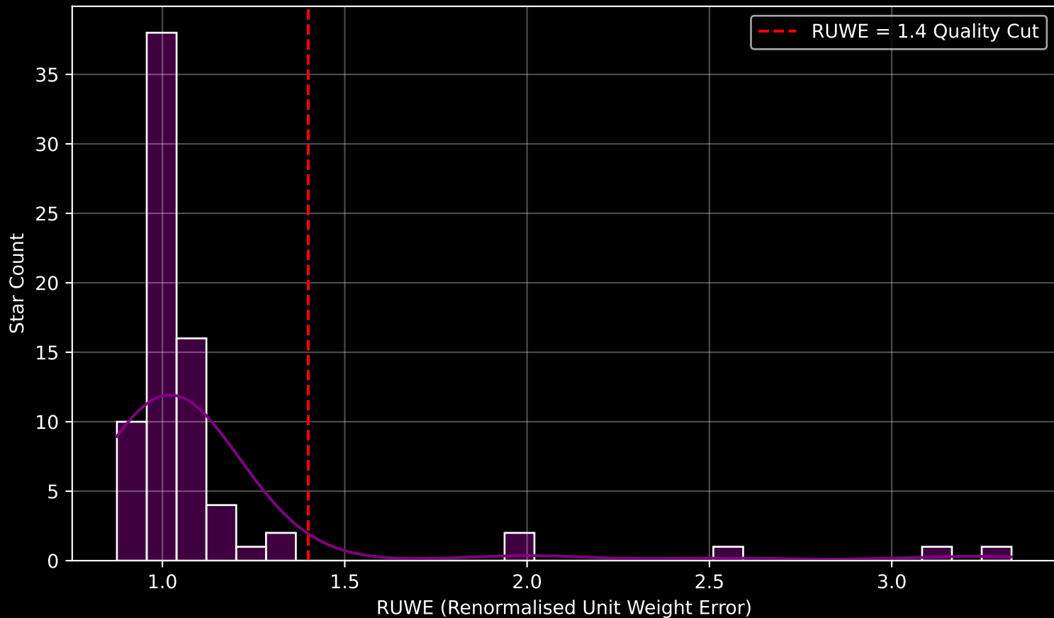
Gaia Cluster: [UPK_16] RUWE Distribution (n= 76)
