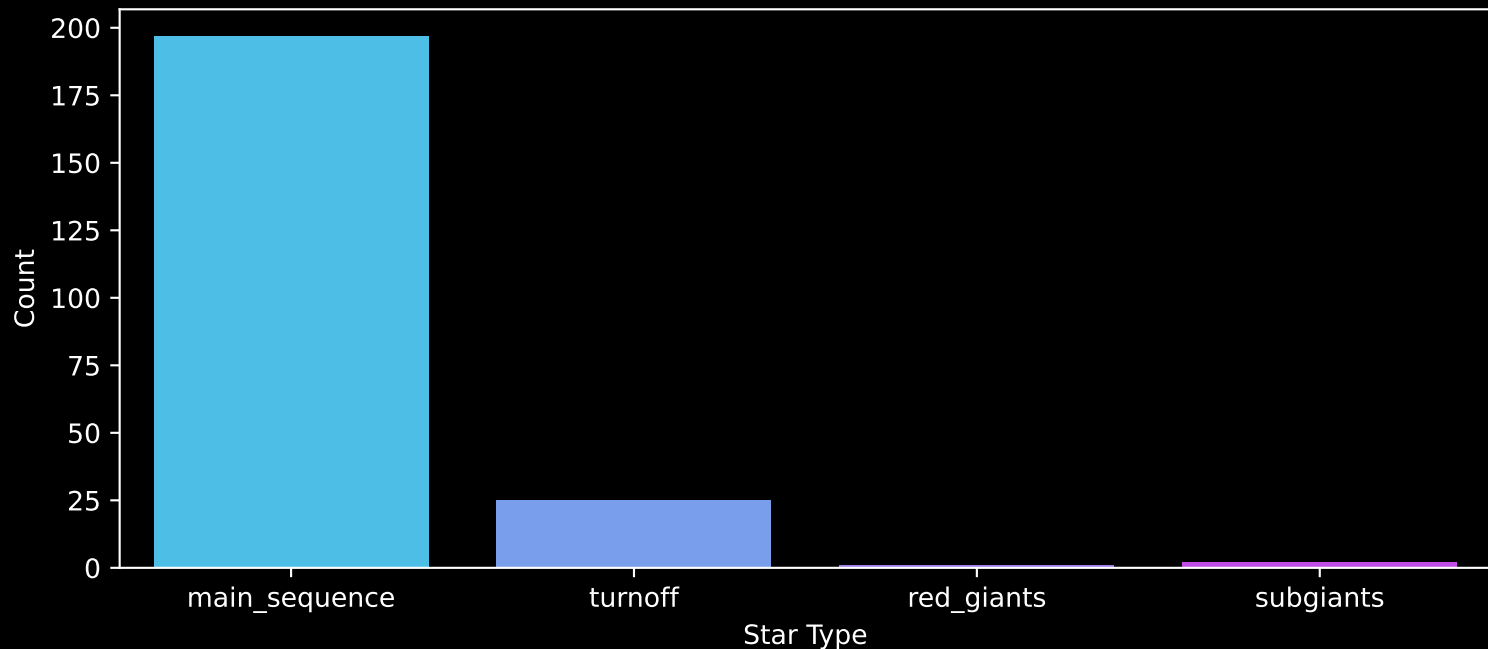
Gaia Cluster: [UPK_166] Count plot of Star Type
