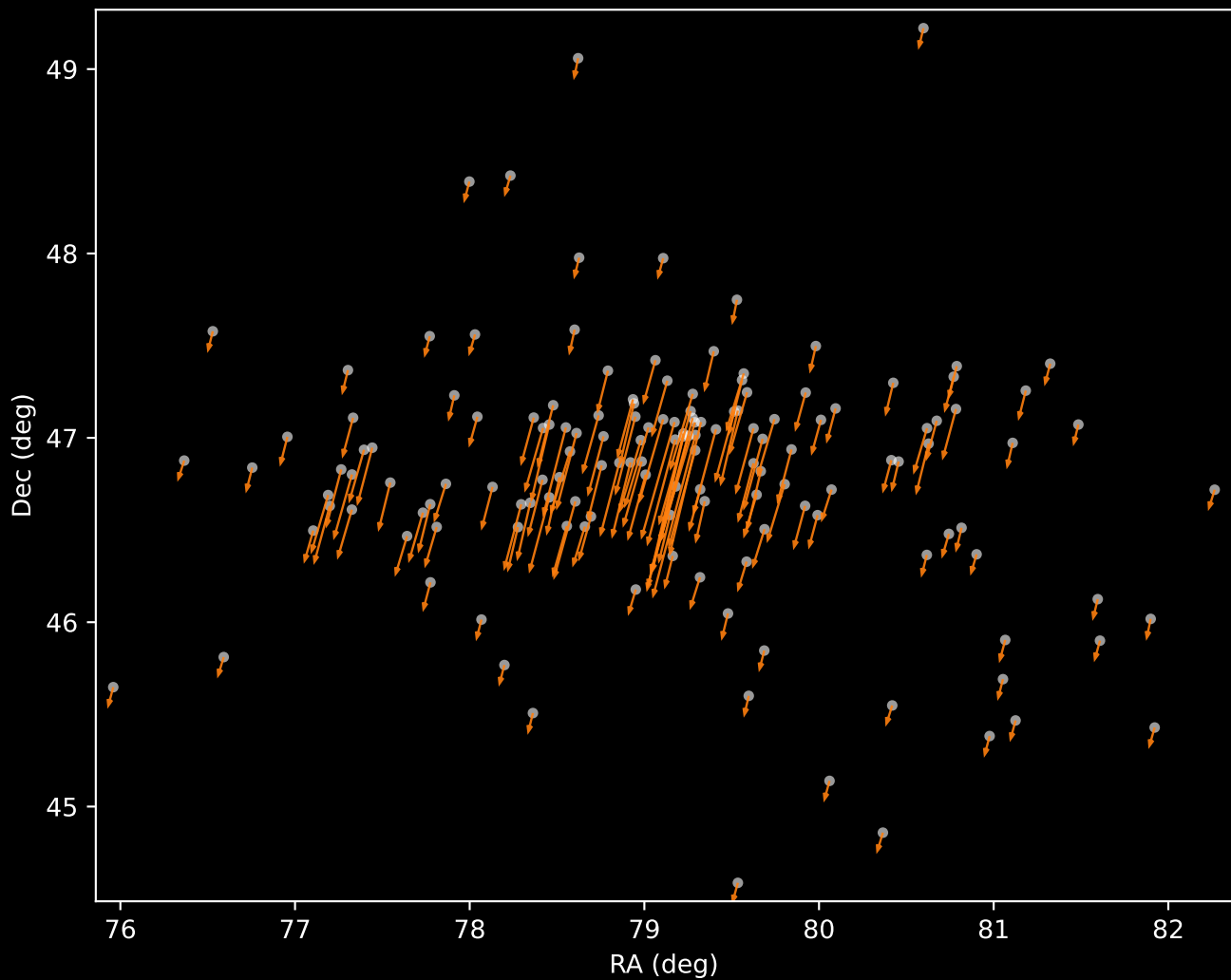
Gaia DR3 Cluster 2 Proper Motion Vectors (n=148)
