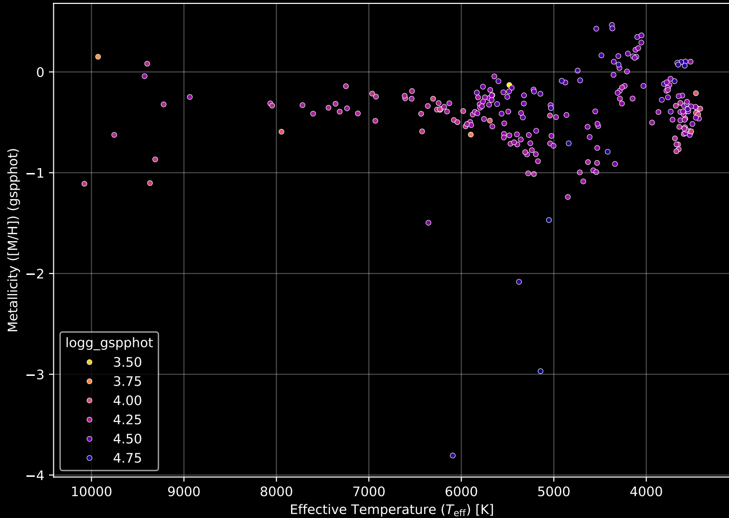
Gaia Cluster: [UPK_166] Stellar Population Parameters (n= 225)
