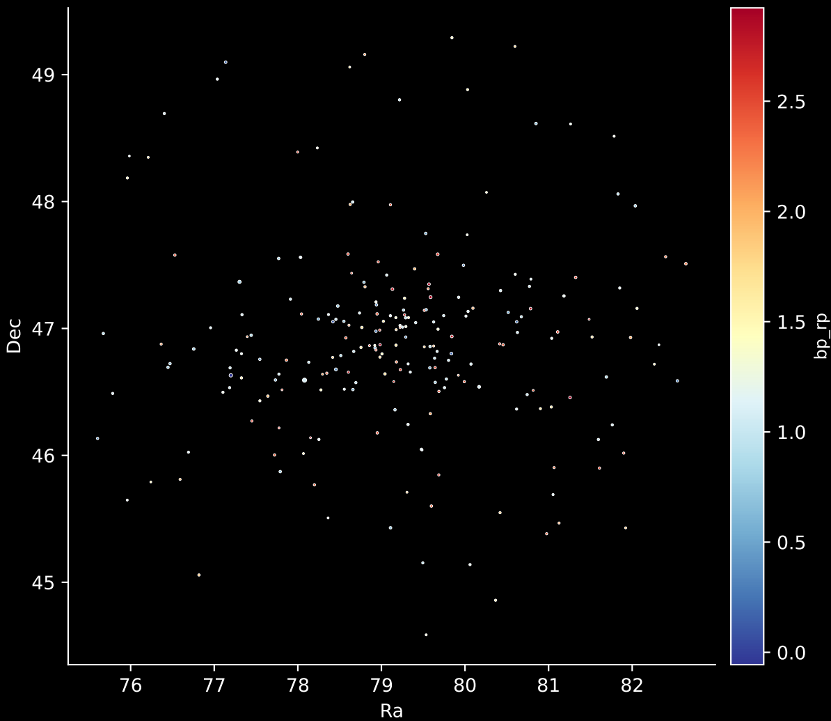
Gaia Cluster: [UPK_166] Stars: 225
