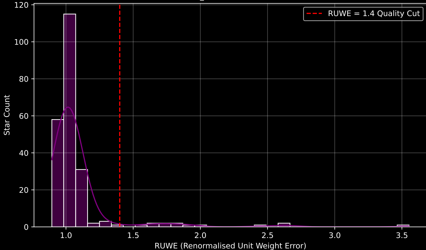
Gaia Cluster: [UPK_166] RUWE Distribution (n= 223)
