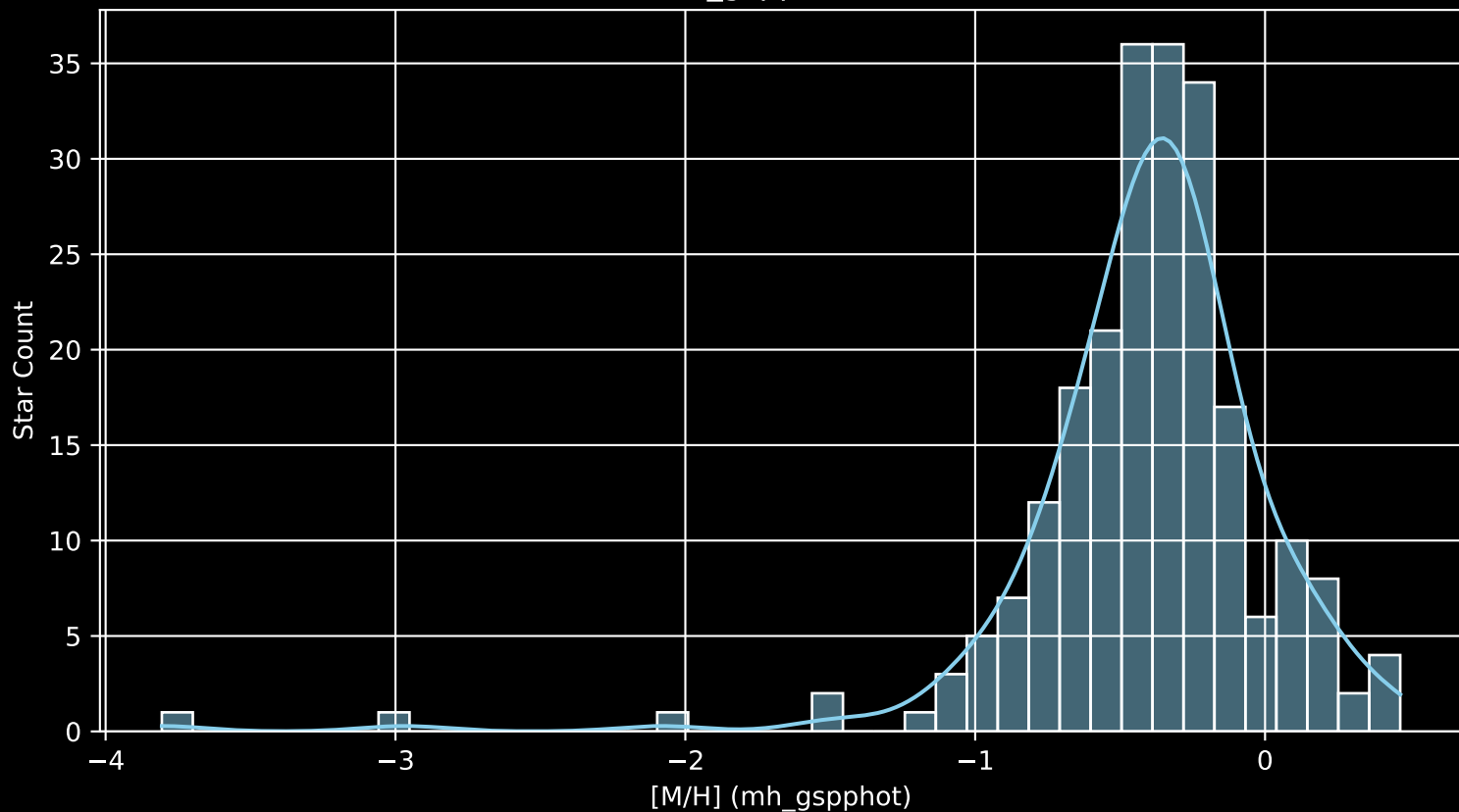
Gaia Cluster: [UPK_166 [M/H] (mh_gspphot) (n= 225)
