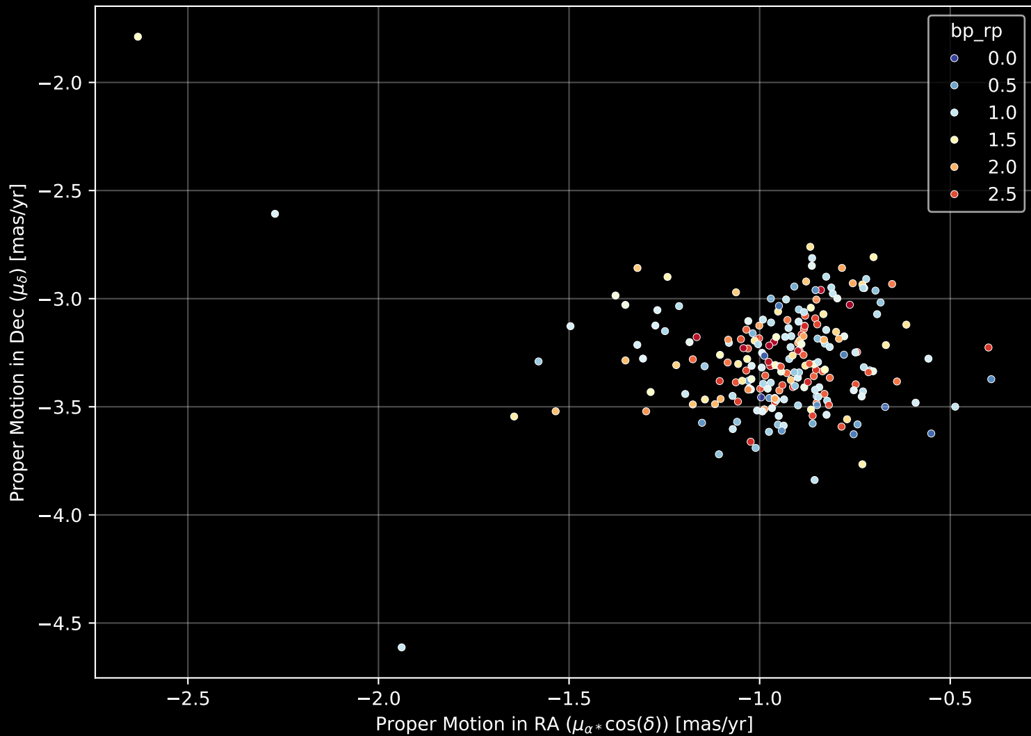
Gaia Cluster: [UPK_166] Proper Motion Diagram (n= 225)
