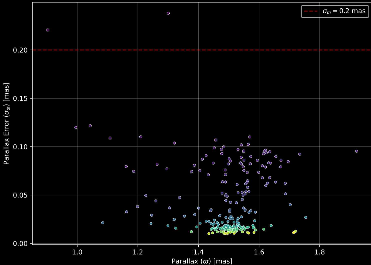
Gaia Cluster: [UPK_166] Parallax Quality (n= 225)
