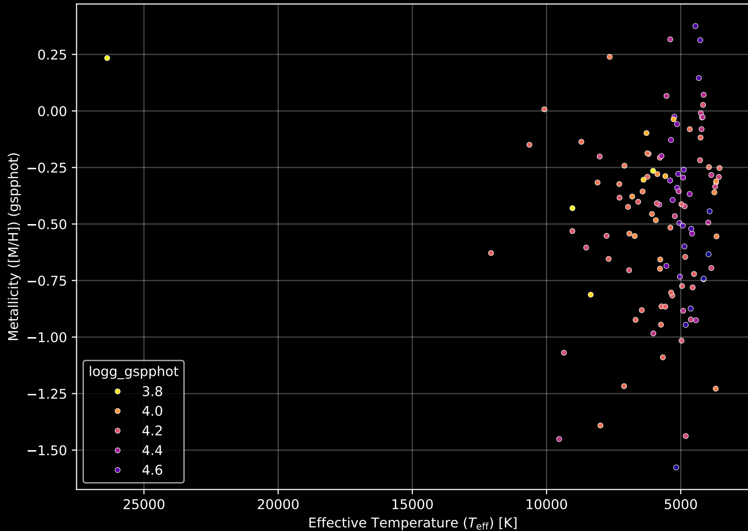
Gaia Cluster: [UPK_169] Stellar Population Parameters (n= 118)
