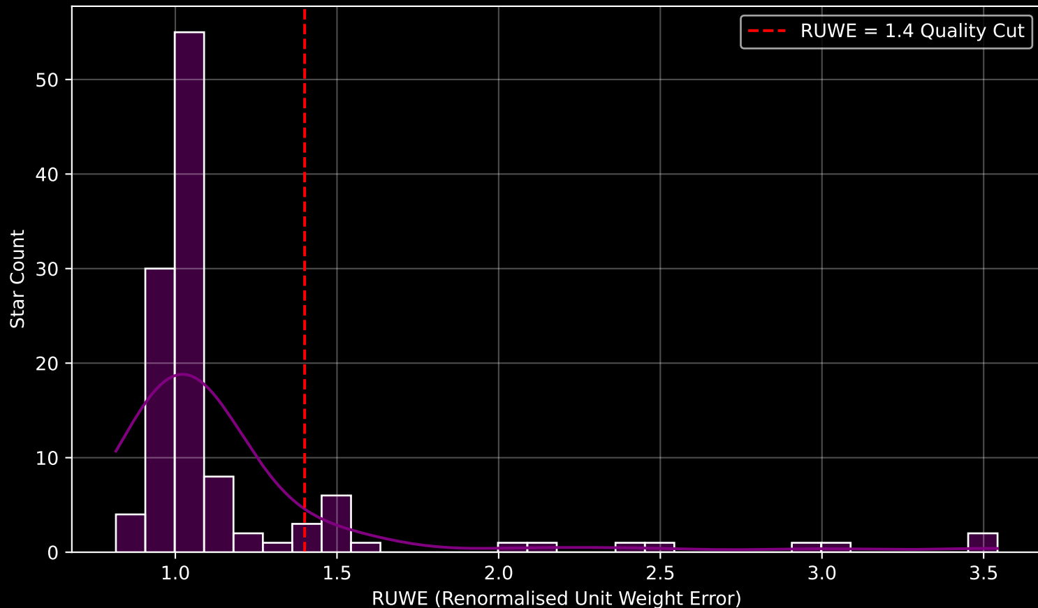
Gaia Cluster: [UPK_169] RUWE Distribution (n= 118)
