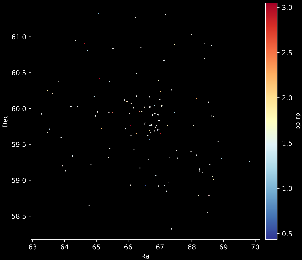
Gaia Cluster: [UPK_169] Stars: 118
