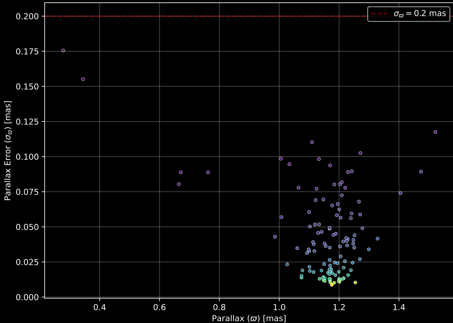
Gaia Cluster: [UPK_169] Parallax Quality (n= 118)
