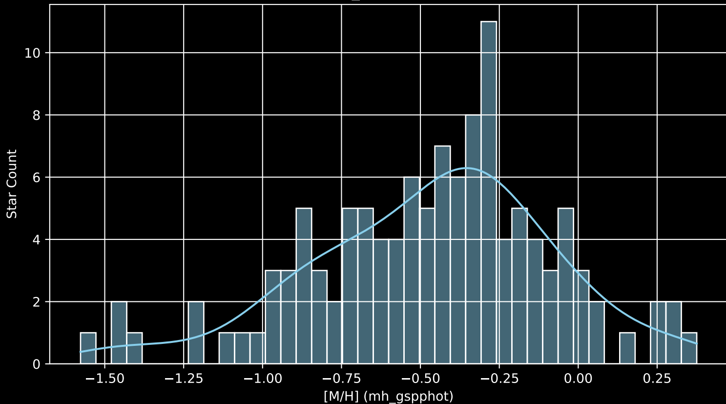
Gaia Cluster: [UPK_169 [M/H] (mh_gspphot) (n= 118)
