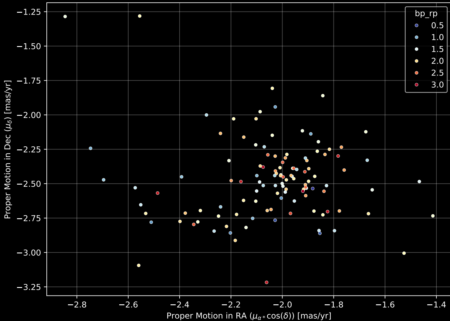
Gaia Cluster: [UPK_169] Proper Motion Diagram (n= 118)
