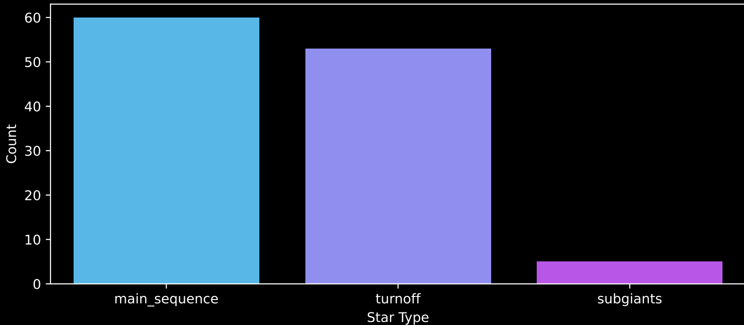
Gaia Cluster: [UPK_169] Count plot of Star Type
