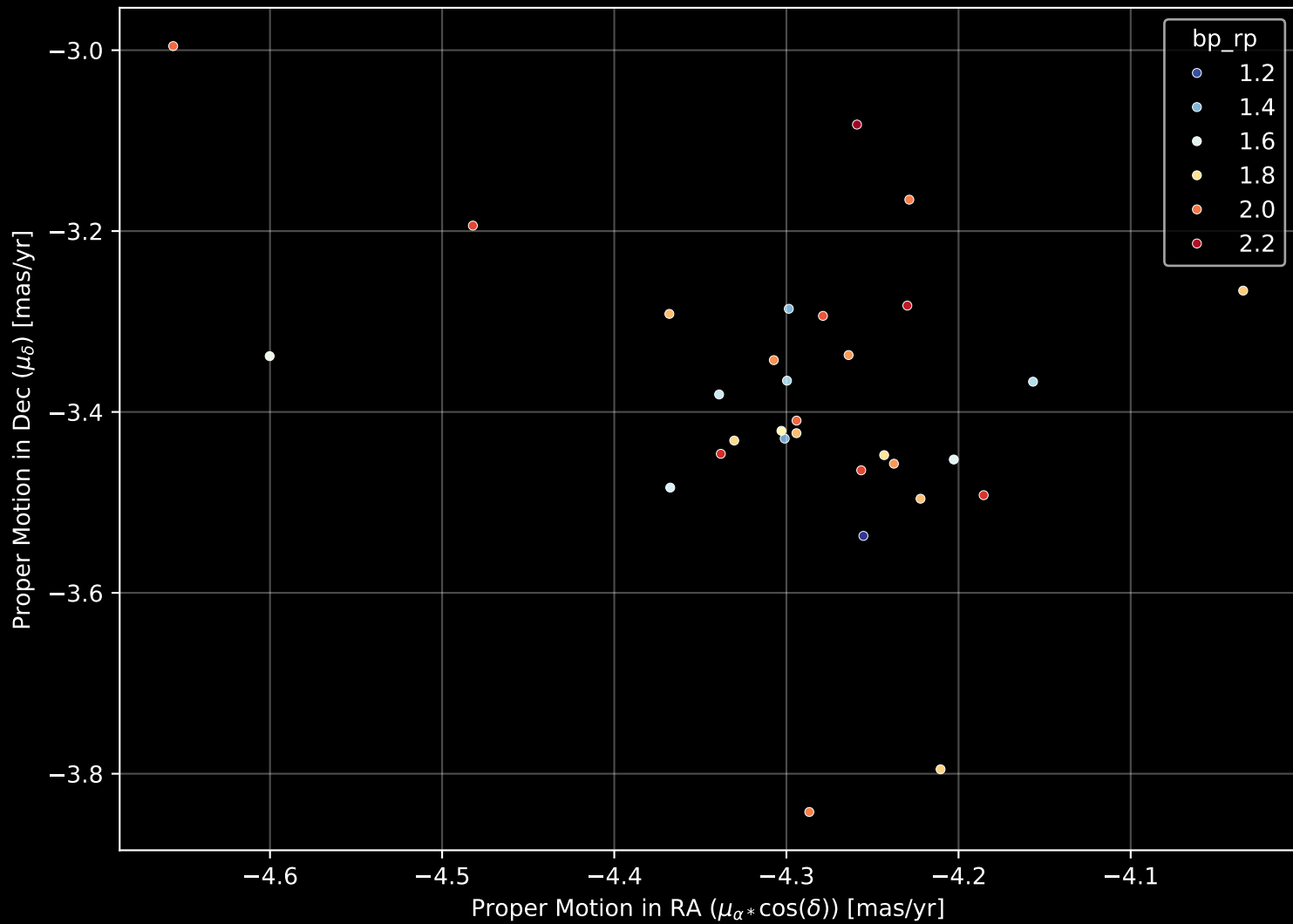
Gaia Cluster: [UPK_178] Proper Motion Diagram (n= 31)
