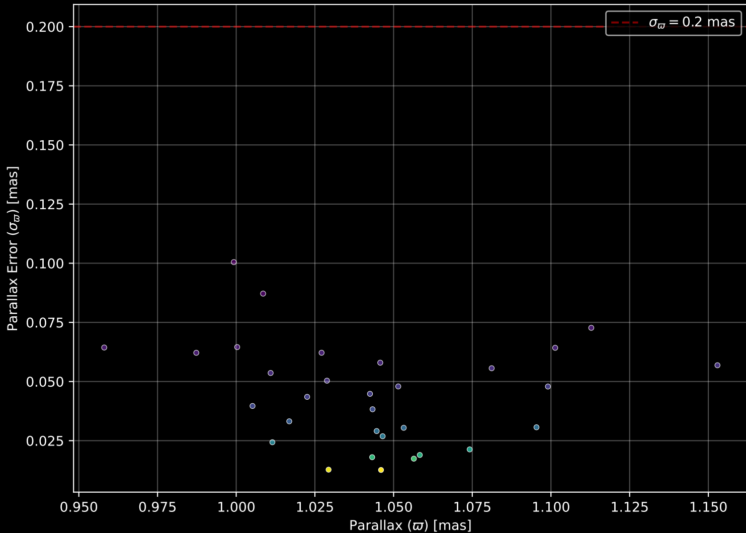
Gaia Cluster: [UPK_178] Parallax Quality (n= 31)
