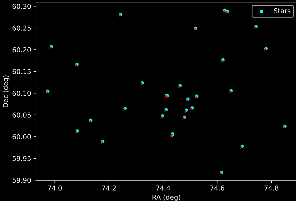
Gaia Cluster: [UPK_178] Proper Motion Vectors for Gaia Star Field (n= 31)
