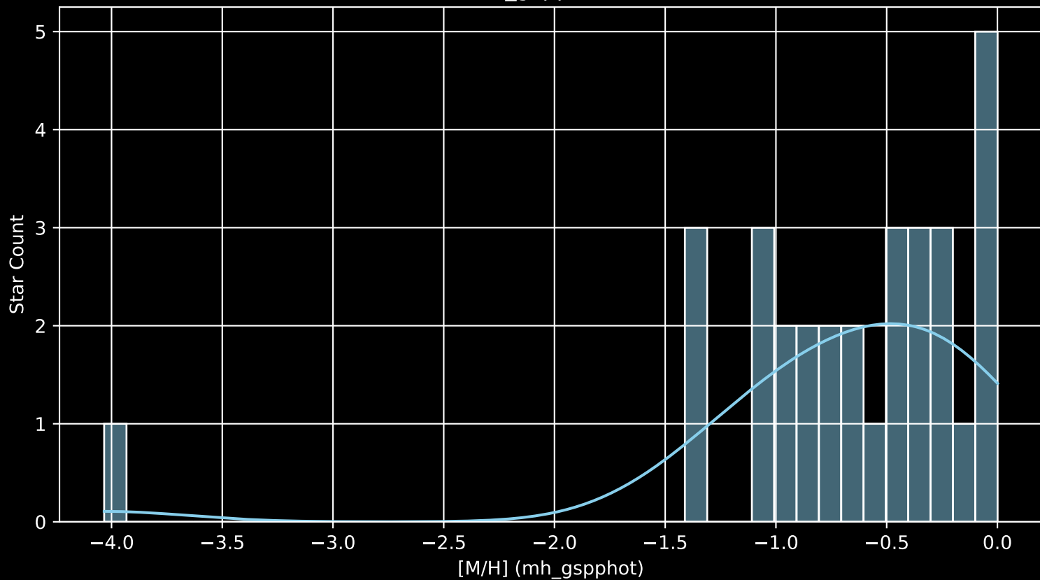
Gaia Cluster: [UPK_178 [M/H] (mh_gspphot) (n= 31)
