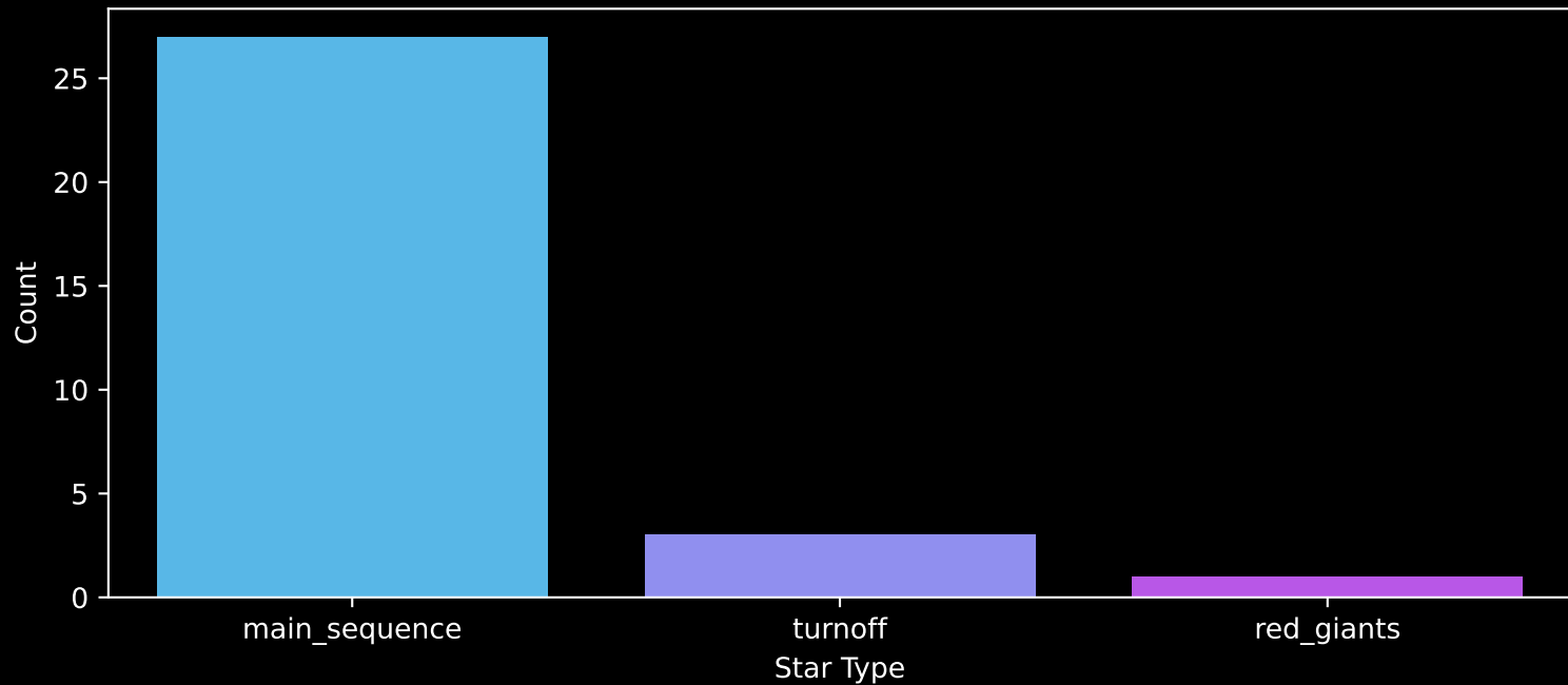
Gaia Cluster: [UPK_178] Count plot of Star Type
