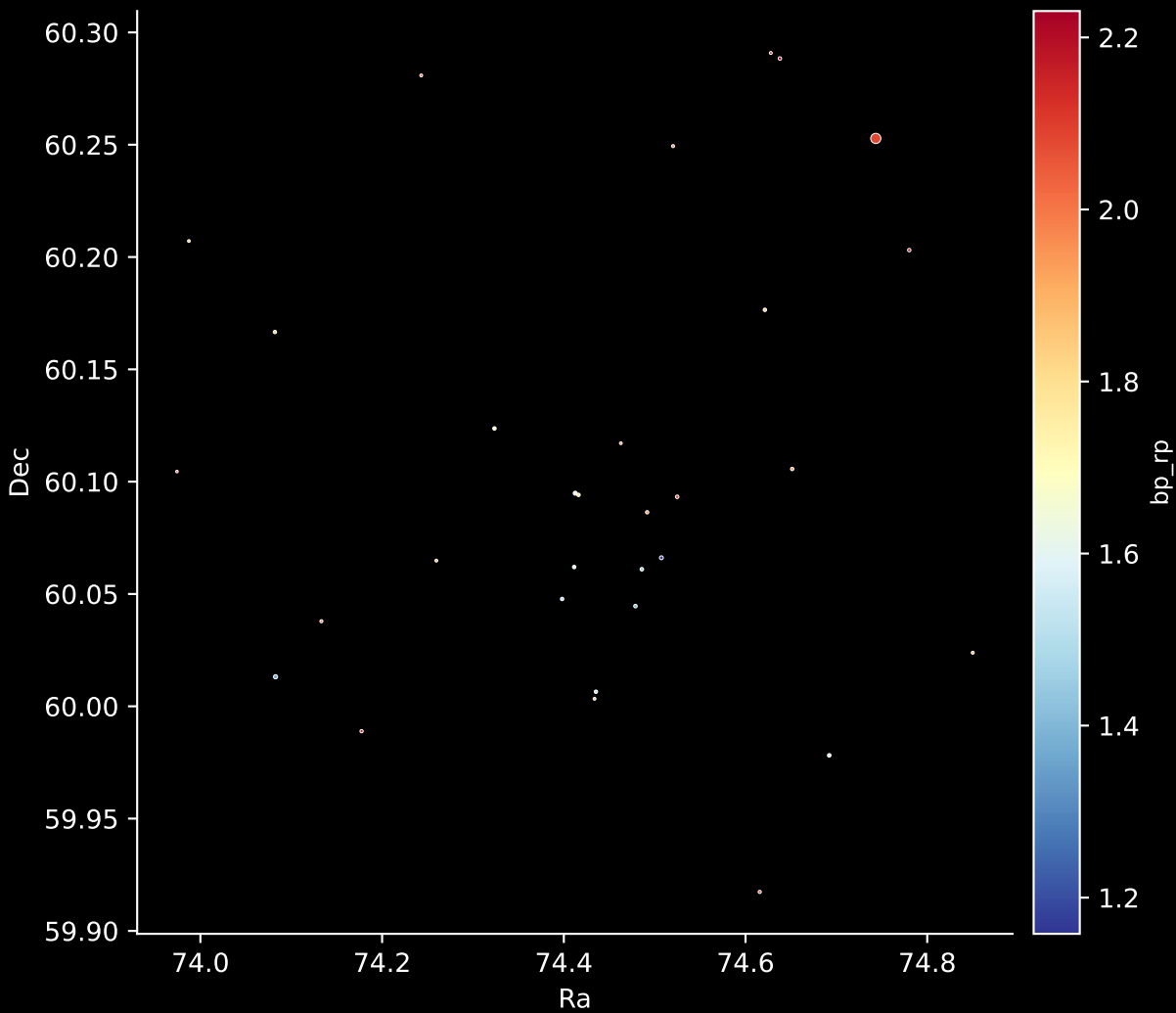
Gaia Cluster: [UPK_178] Stars: 31
