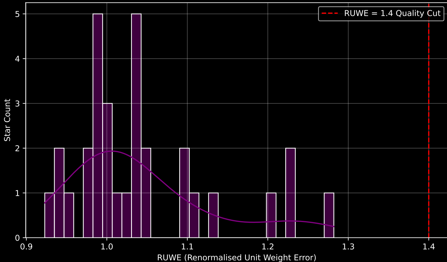
Gaia Cluster: [UPK_178] RUWE Distribution (n= 31)
