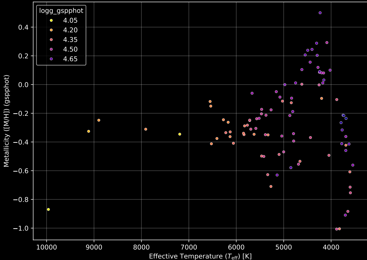
Gaia Cluster: [UPK_185] Stellar Population Parameters (n= 96)
