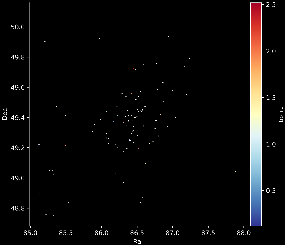
Gaia Cluster: [UPK_185] Stars: 96
