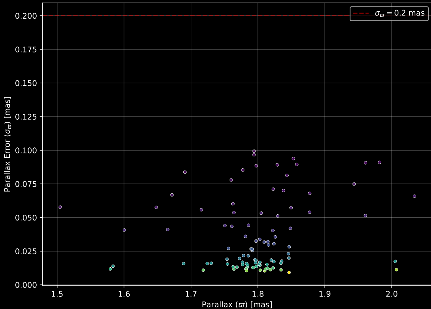
Gaia Cluster: [UPK_185] Parallax Quality (n= 96)
