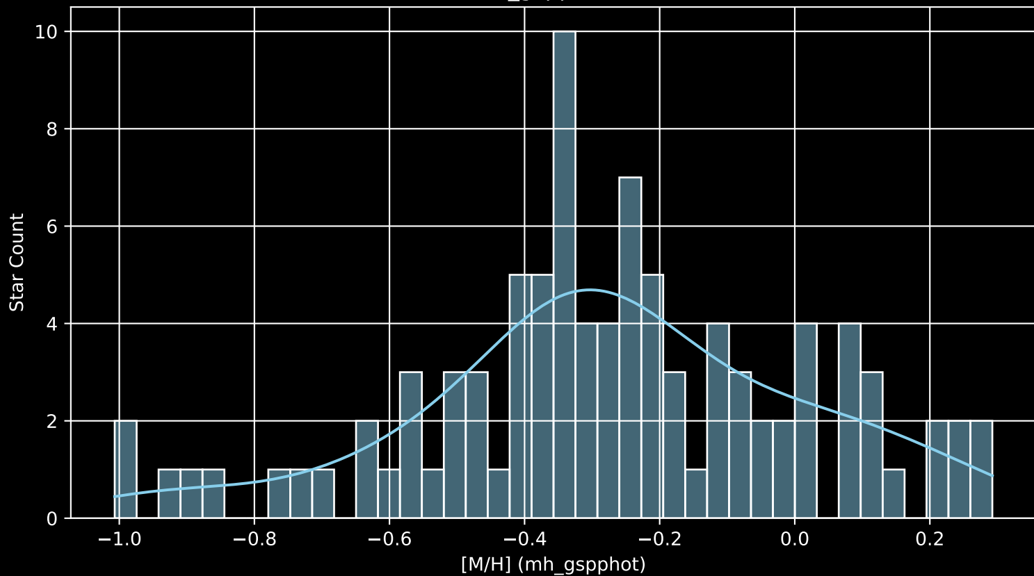
Gaia Cluster: [UPK_185 [M/H] (mh_gspphot) (n= 95)
