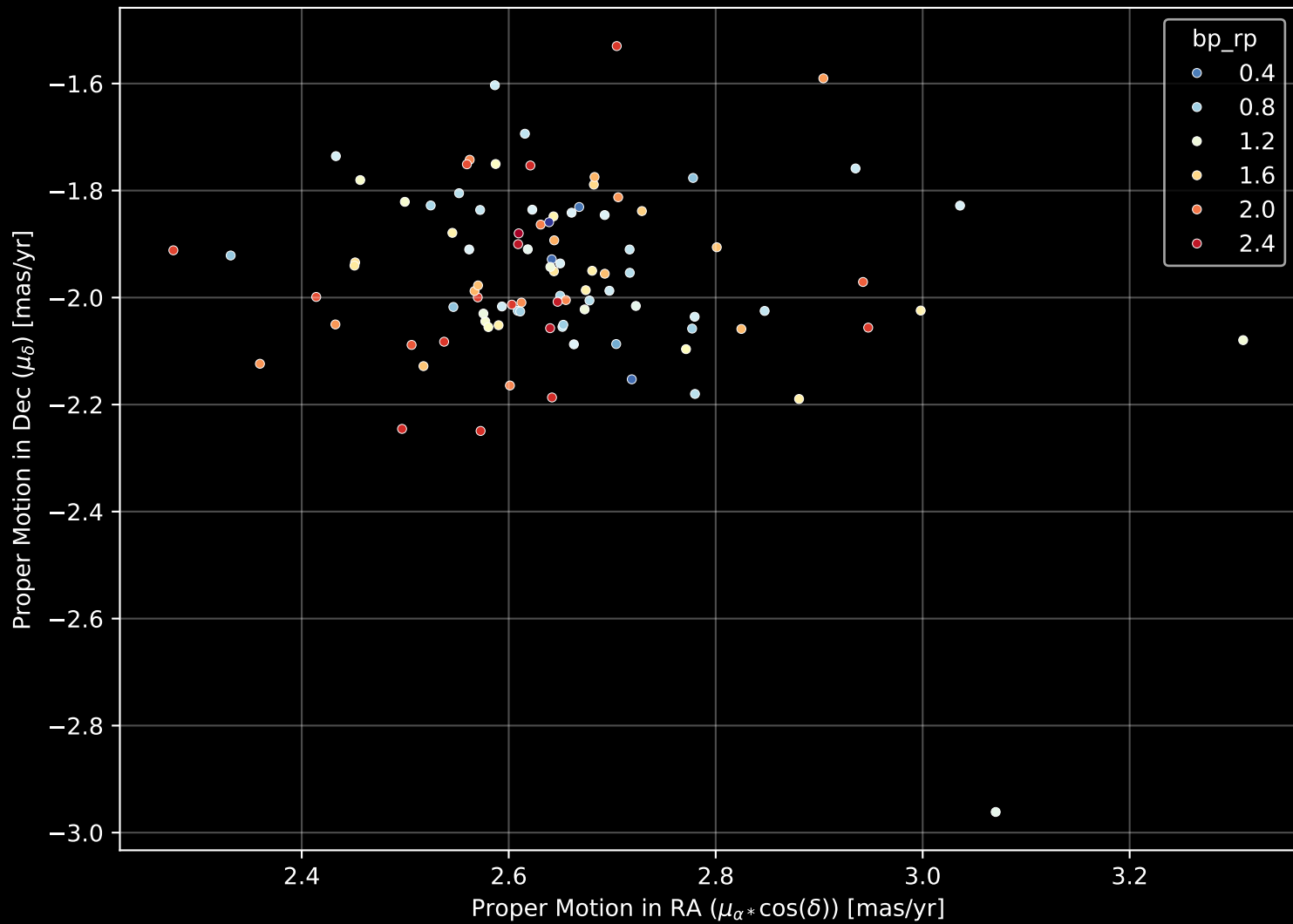
Gaia Cluster: [UPK_185] Proper Motion Diagram (n= 96)
