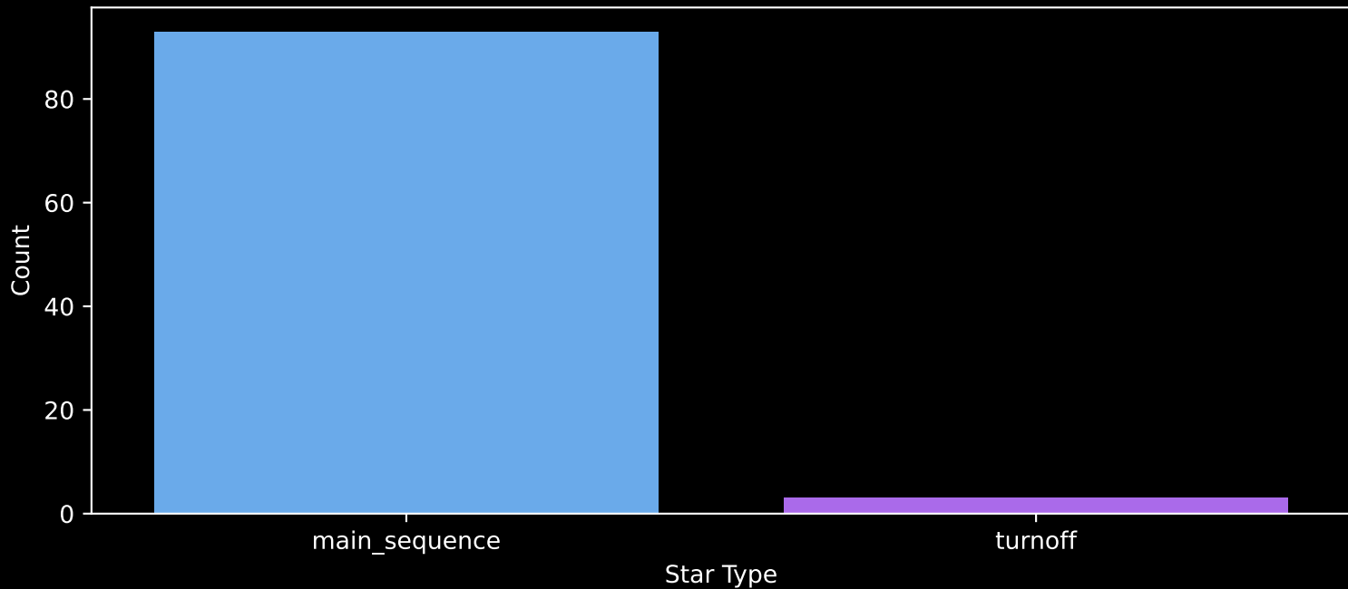
Gaia Cluster: [UPK_185] Count plot of Star Type
