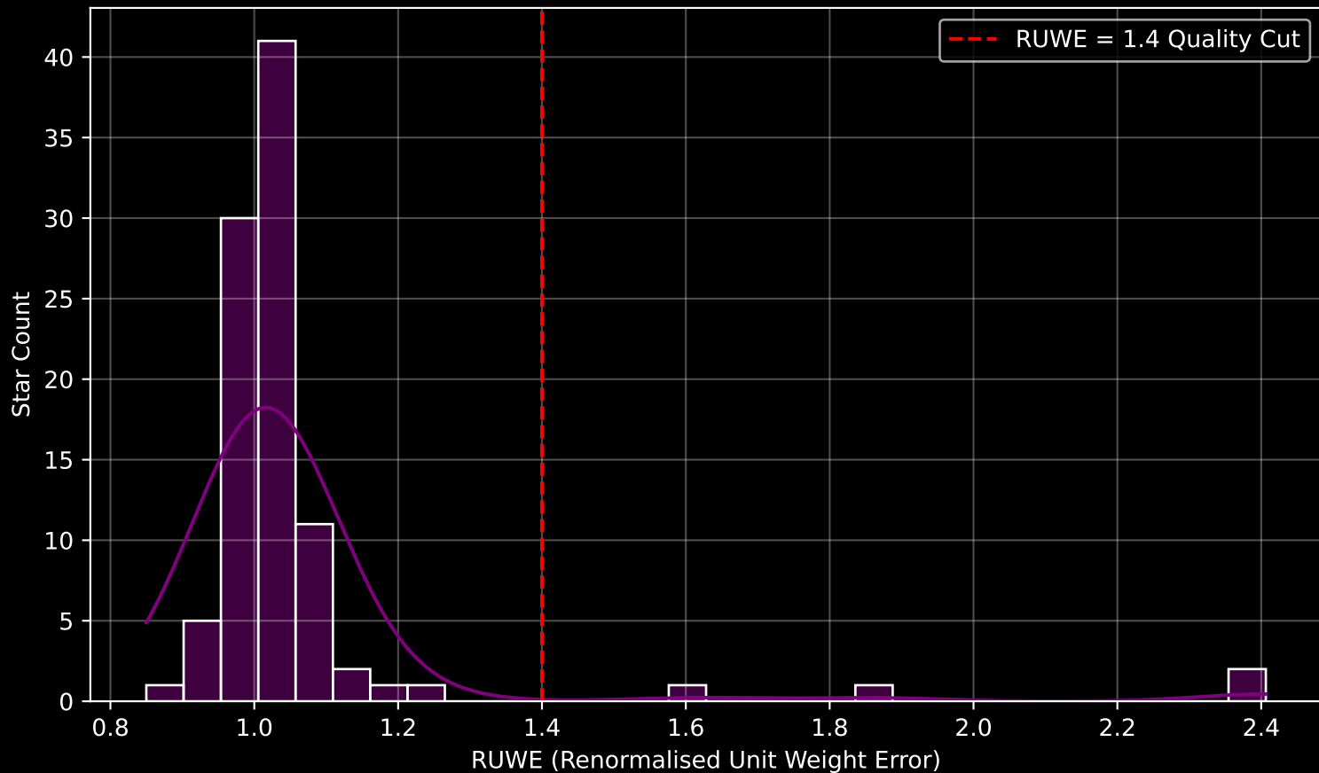
Gaia Cluster: [UPK_185] RUWE Distribution (n= 96)
