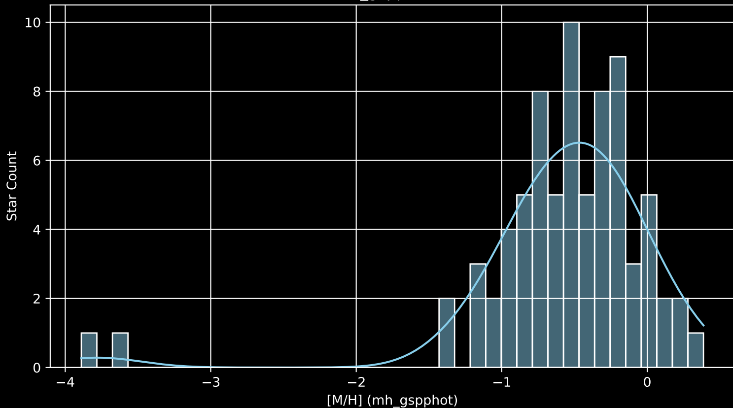
Gaia Cluster: [UPK_20 [M/H] (mh_gspphot) (n= 76)
