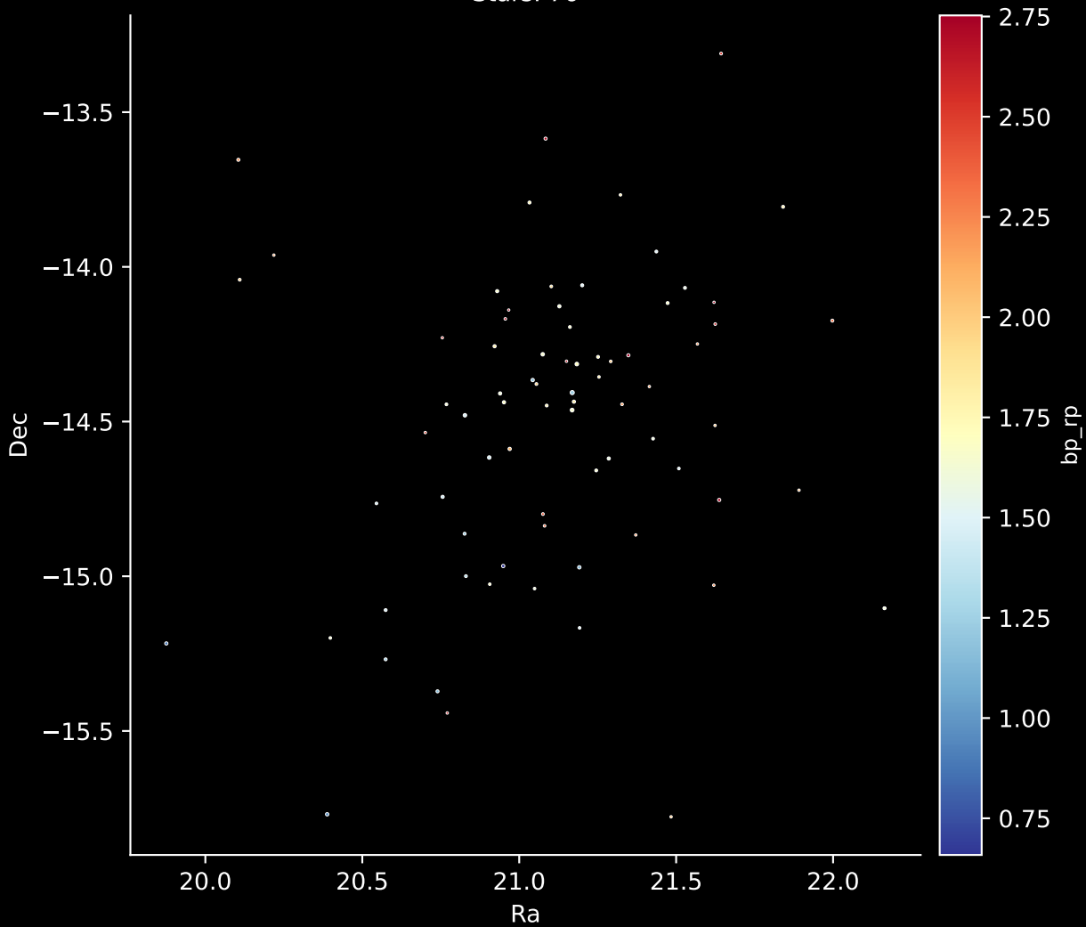
Gaia Cluster: [UPK_20] Stars: 76
