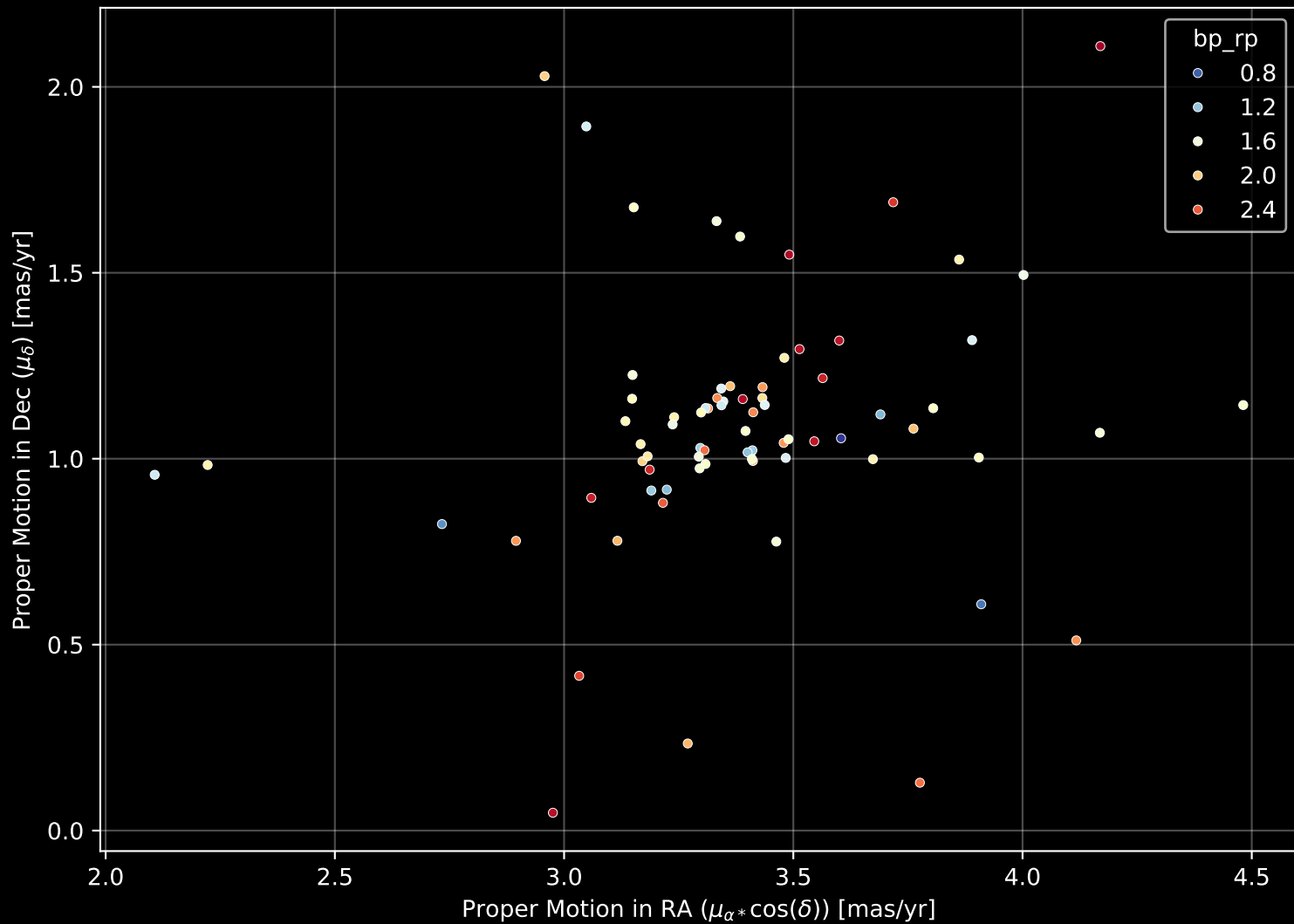
Gaia Cluster: [UPK_20] Proper Motion Diagram (n= 76)
