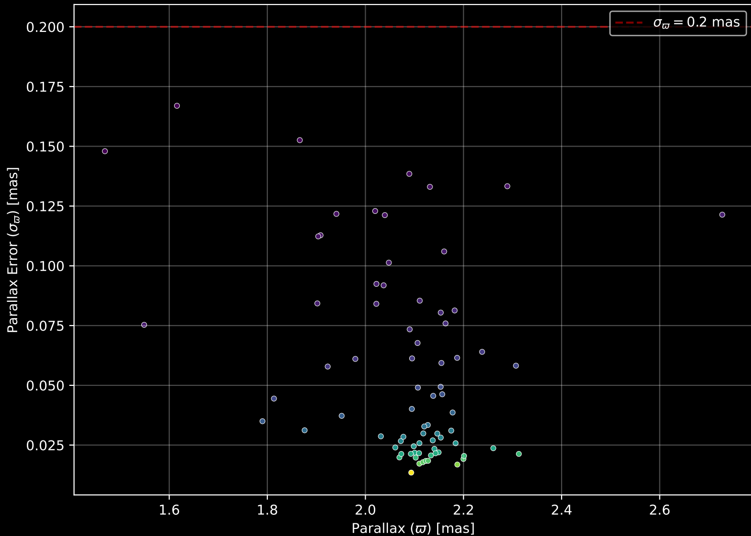
Gaia Cluster: [UPK_20] Parallax Quality (n= 76)
