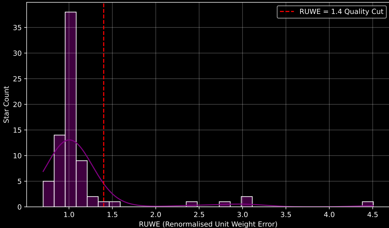
Gaia Cluster: [UPK_20] RUWE Distribution (n= 75)
