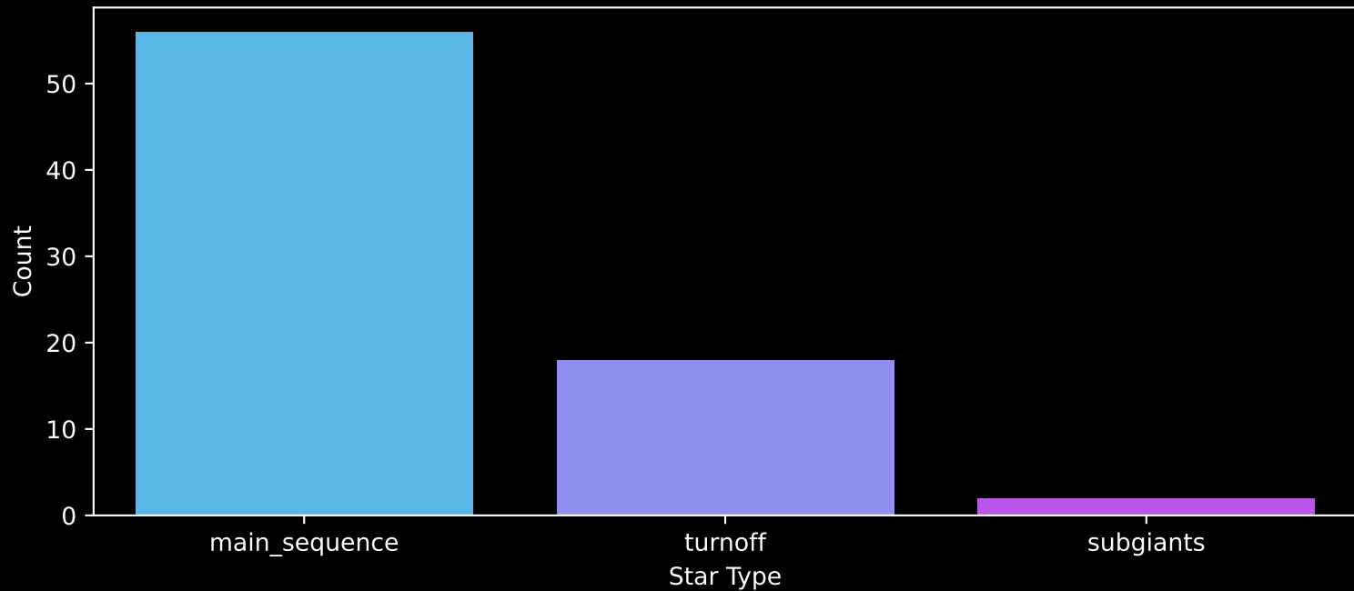
Gaia Cluster: [UPK_20] Count plot of Star Type
