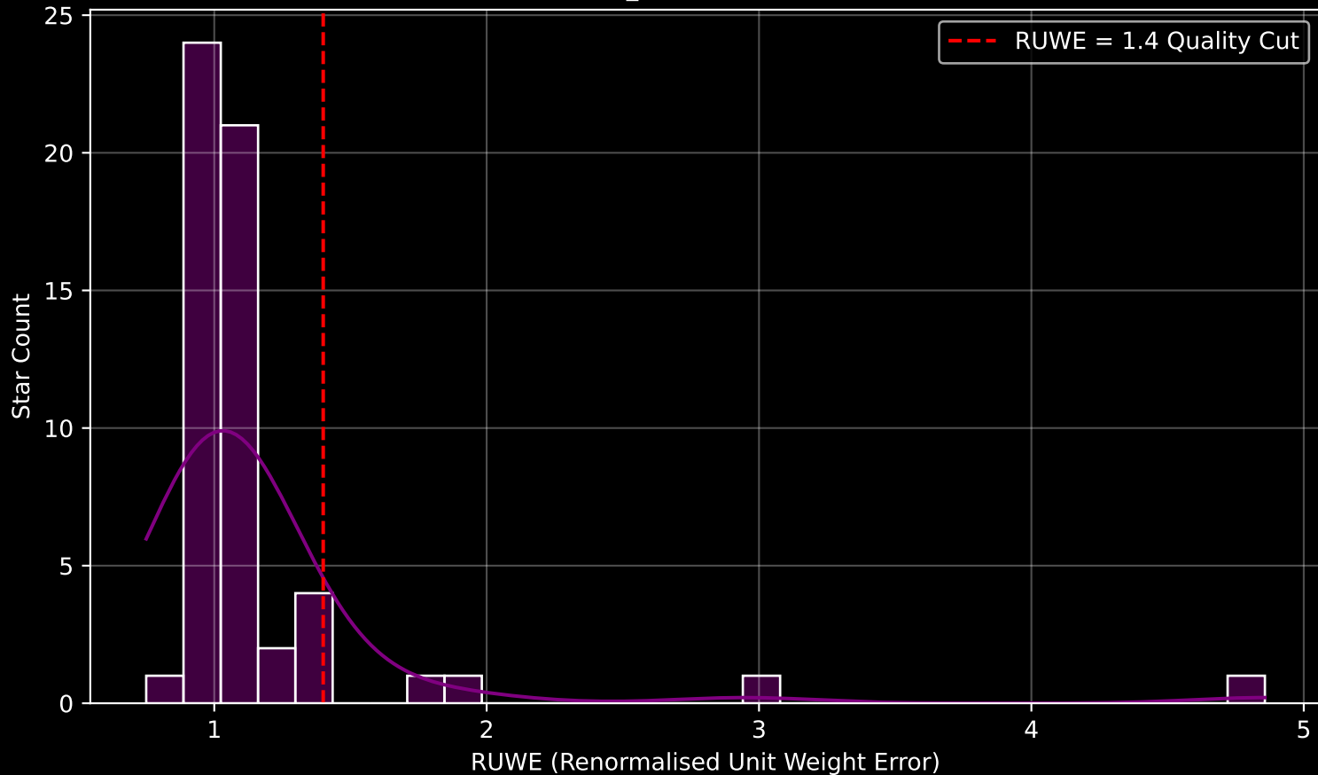
Gaia Cluster: [UPK_23] RUWE Distribution (n= 56)
