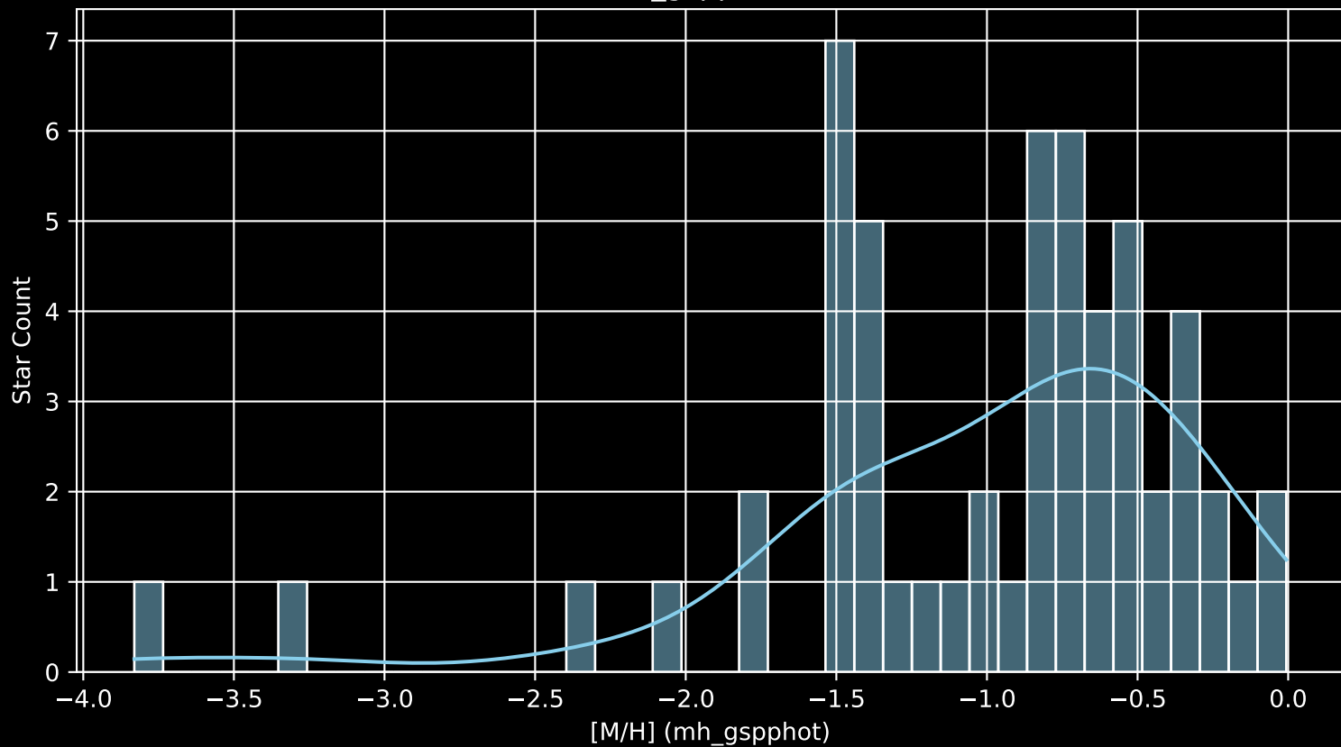
Gaia Cluster: [UPK_23 [M/H] (mh_gspphot) (n= 56)
