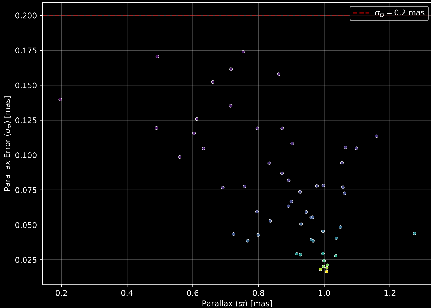
Gaia Cluster: [UPK_23] Parallax Quality (n= 56)
