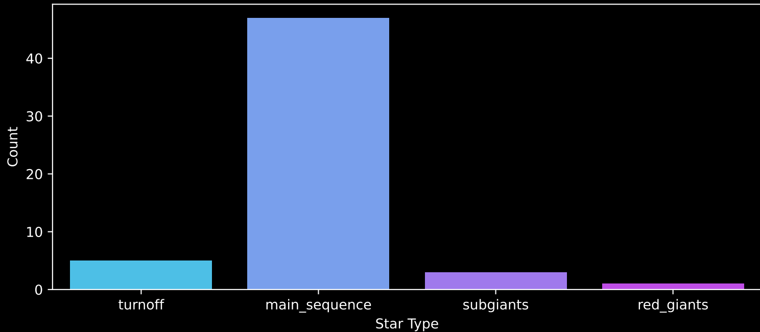
Gaia Cluster: [UPK_23] Count plot of Star Type
