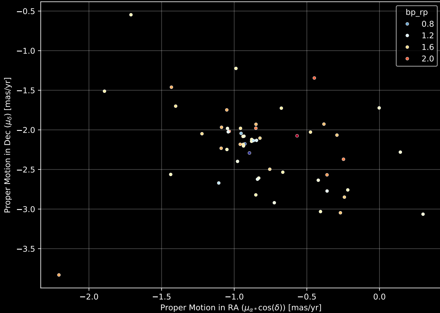
Gaia Cluster: [UPK 23] Proper Motion Diagram (n= 56)
