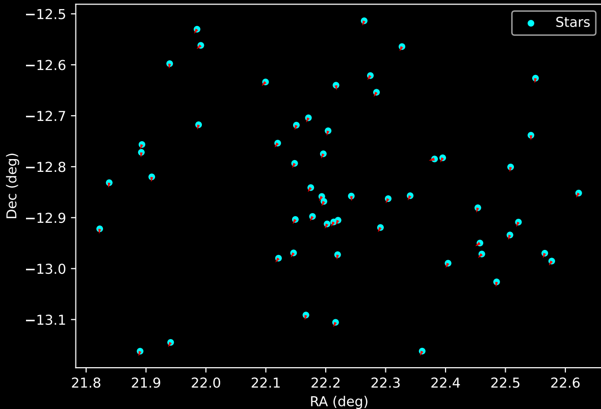
Gaia Cluster: [UPK_23] Proper Motion Vectors for Gaia Star Field (n= 56)
