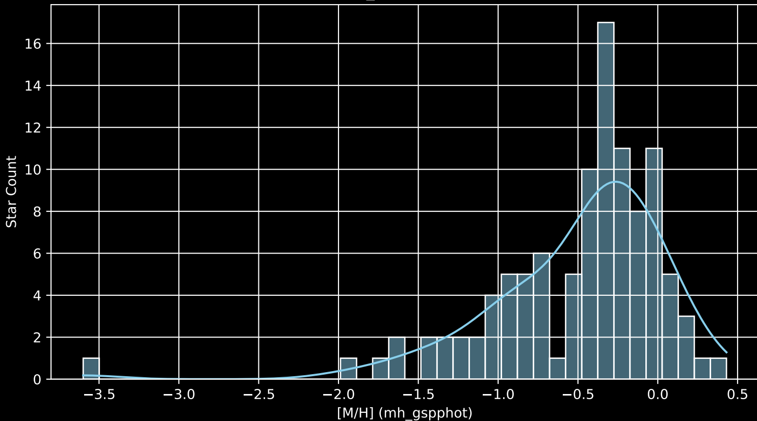
Gaia Cluster: [UPK_265 [M/H] (mh_gspphot) (n= 106)
