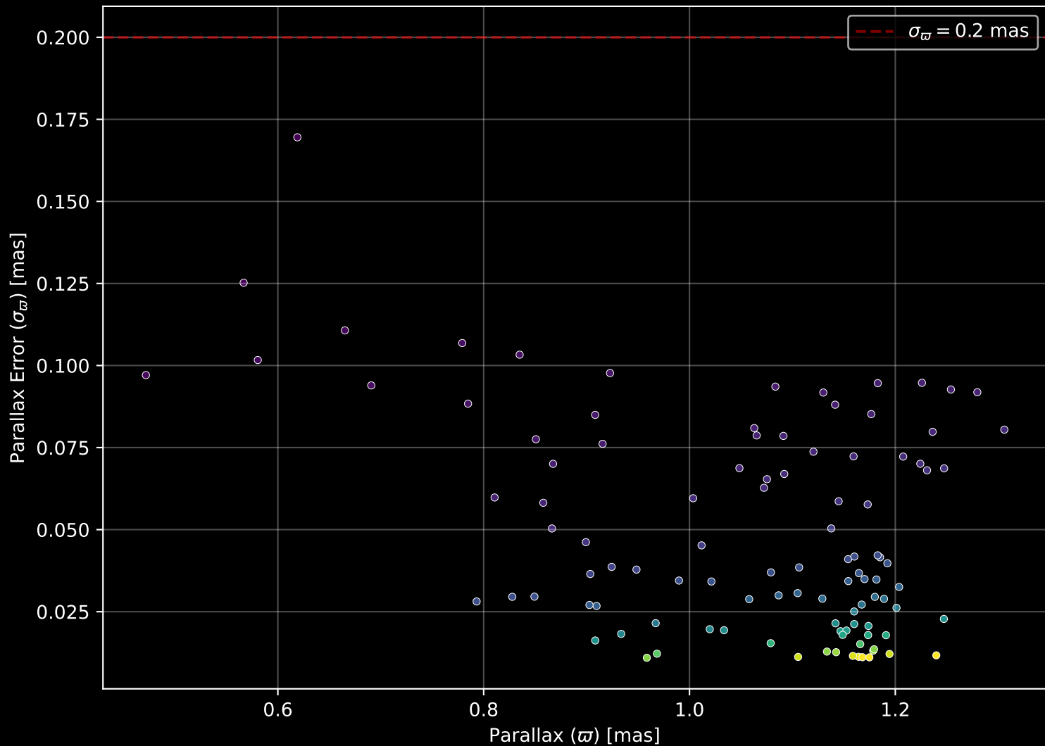
Gaia Cluster: [UPK_265] Parallax Quality (n= 106)
