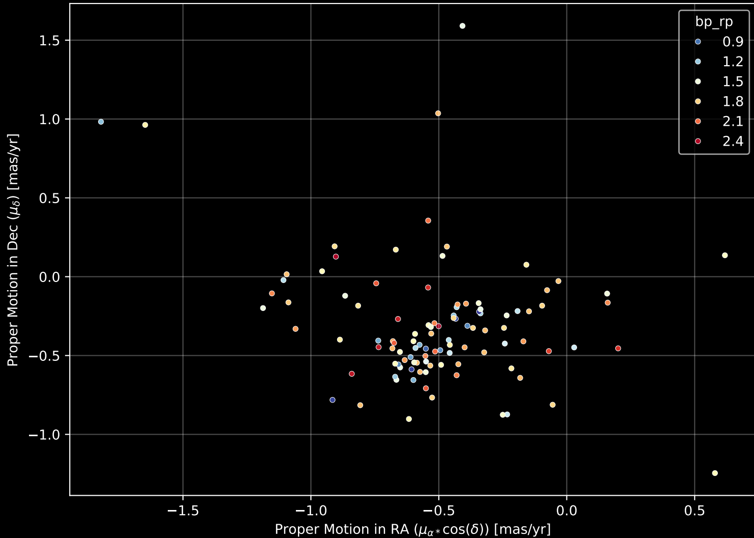
Gaia Cluster: [UPK_265] Proper Motion Diagram (n= 106)
