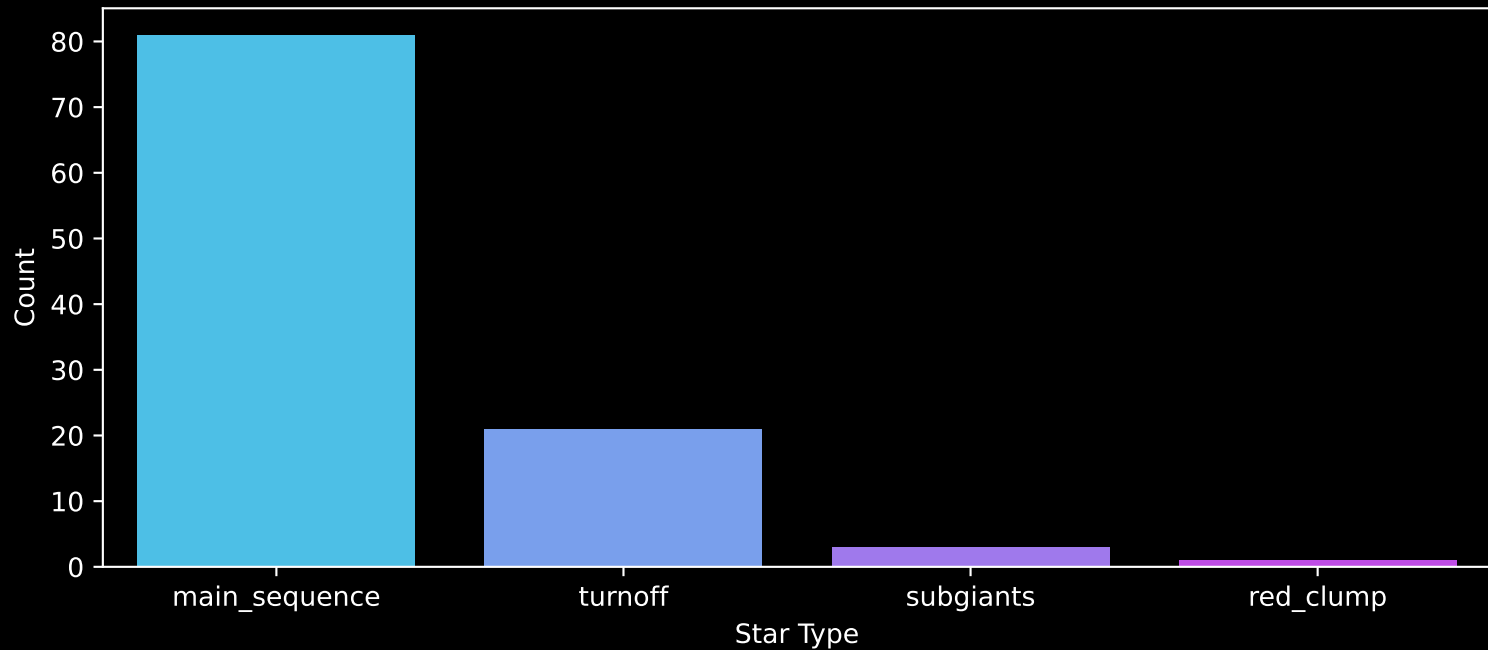
Gaia Cluster: [UPK_265] Count plot of Star Type
