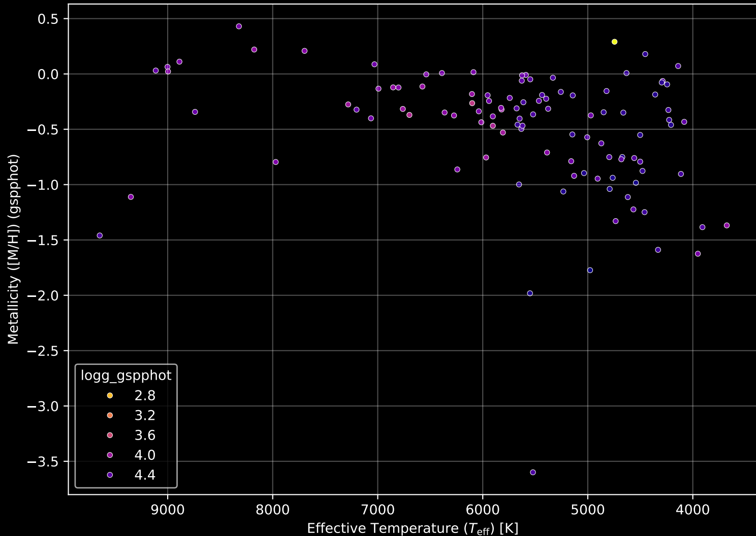
Gaia Cluster: [UPK_265] Stellar Population Parameters (n= 106)
