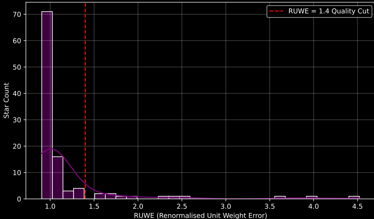
Gaia Cluster: [UPK_265] RUWE Distribution (n= 106)
