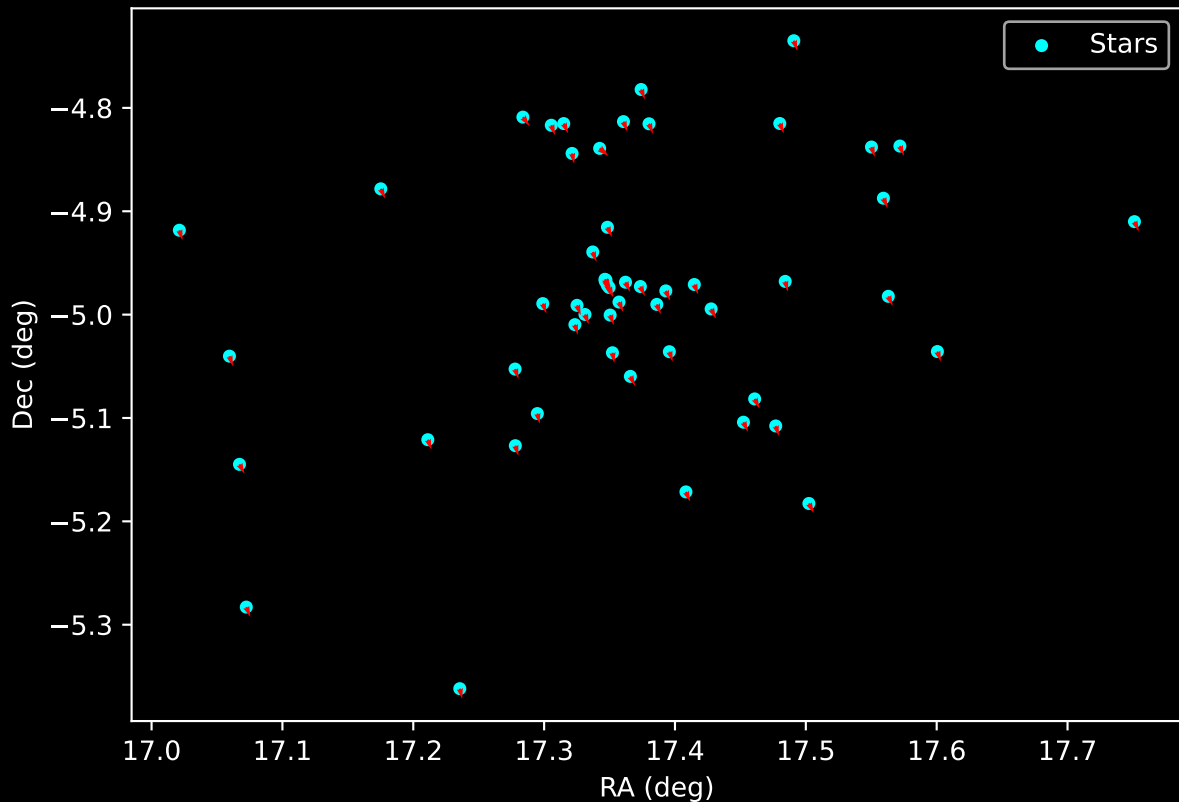
Gaia Cluster: [UPK_28] Proper Motion Vectors for Gaia Star Field (n= 54)
