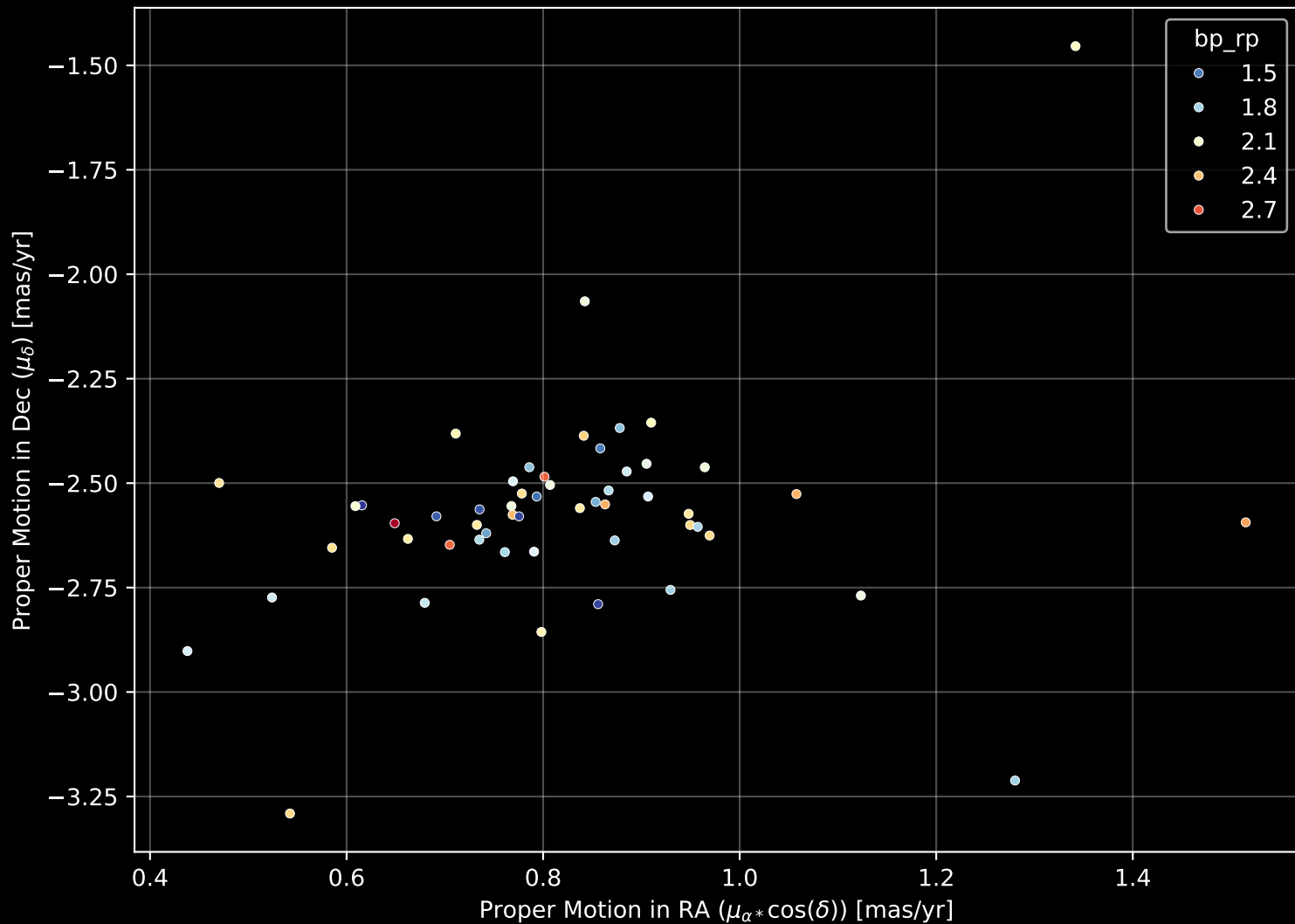
Gaia Cluster: [UPK_28] Proper Motion Diagram (n= 54)
