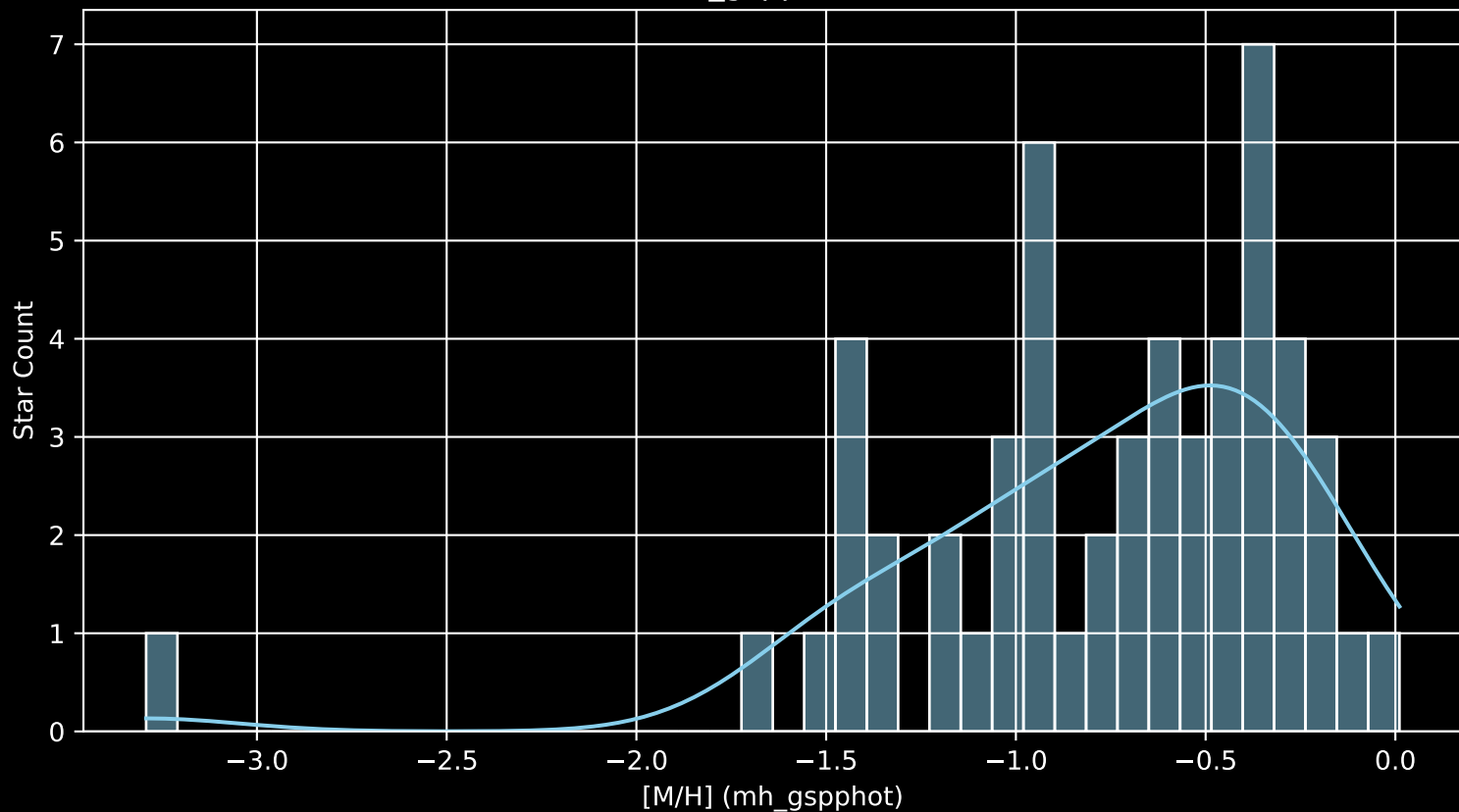
Gaia Cluster: [UPK_28 [M/H] (mh_gspphot) (n= 54)
