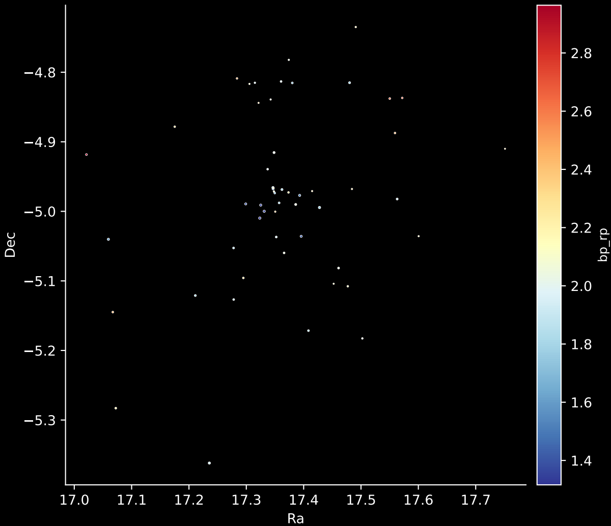
Gaia Cluster: [UPK_28] Stars: 54
