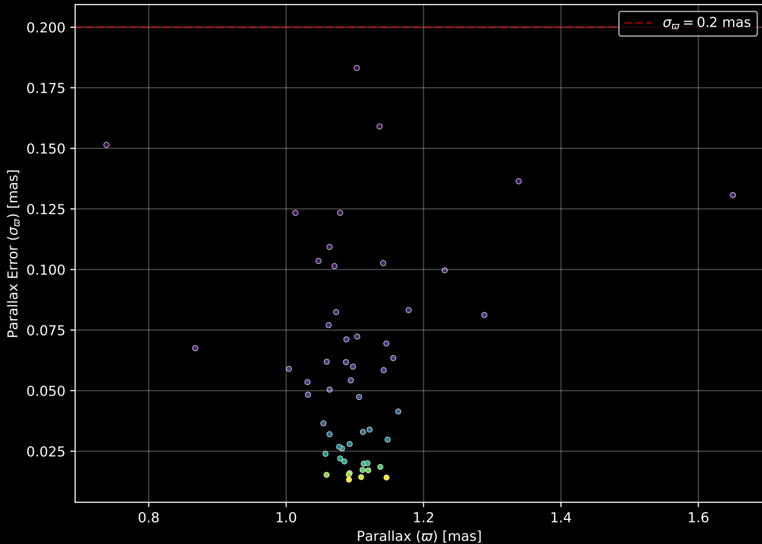
Gaia Cluster: [UPK_28] Parallax Quality (n= 54)
