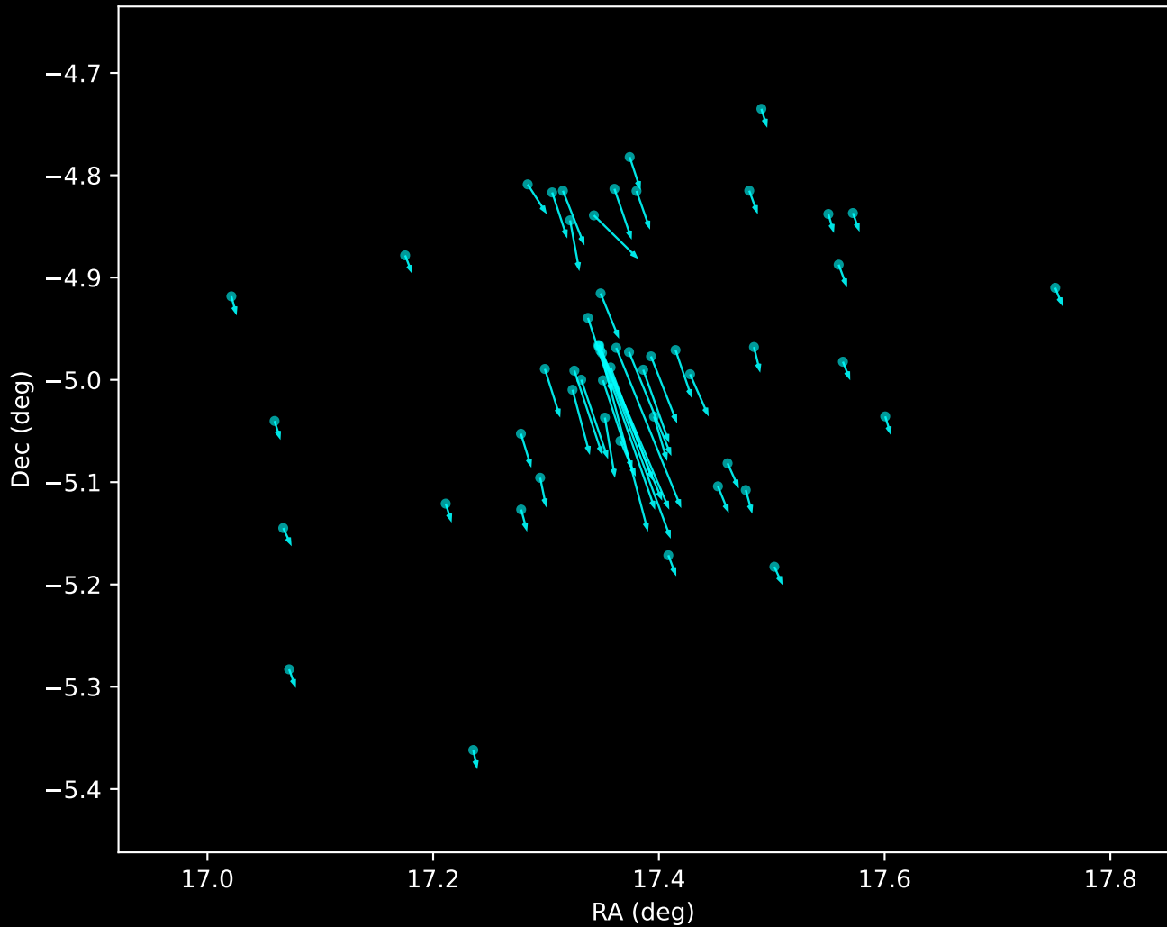
Gaia DR3 Noise Stream Proper Motion Vectors (n=54)
