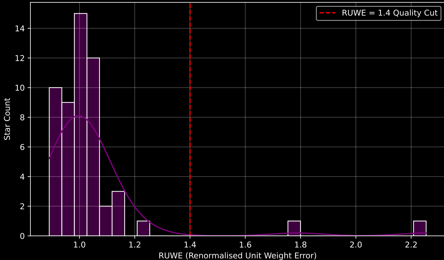
Gaia Cluster: [UPK_28] RUWE Distribution (n= 54)
