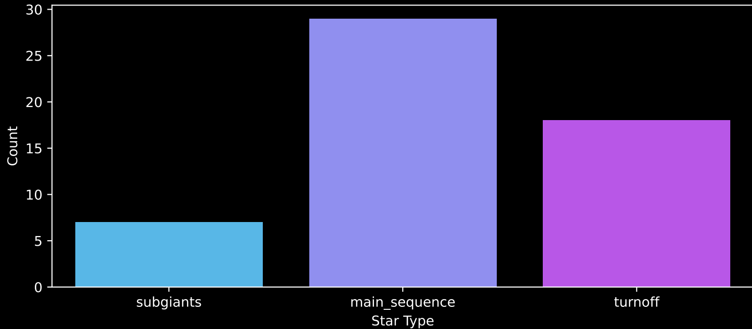
Gaia Cluster: [UPK_28] Count plot of Star Type
