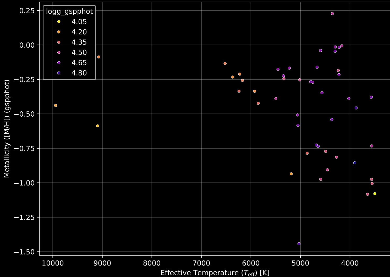
Gaia Cluster: [UPK_282] Stellar Population Parameters (n= 49)
