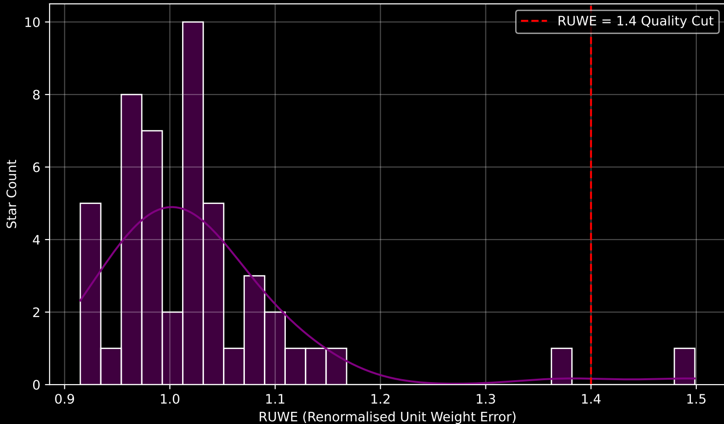
Gaia Cluster: [UPK_282] RUWE Distribution (n= 49)
