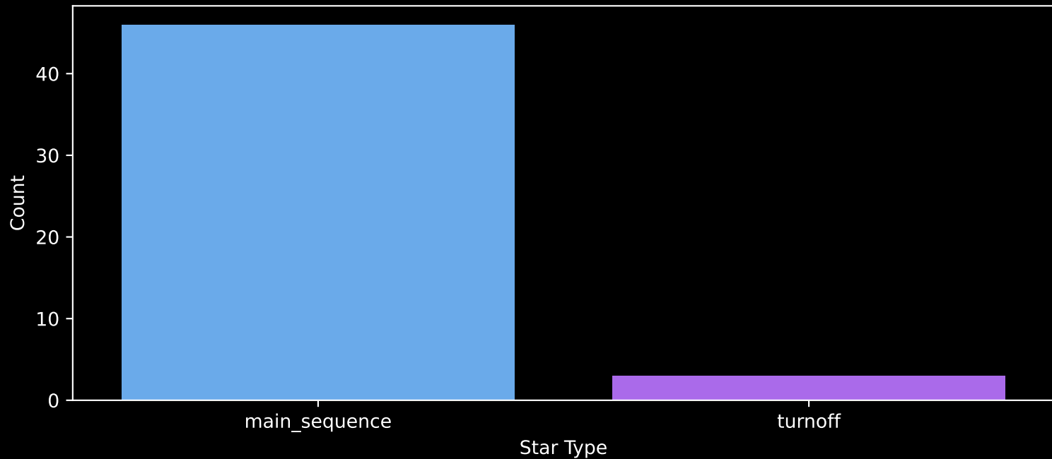
Gaia Cluster: [UPK_282] Count plot of Star Type
