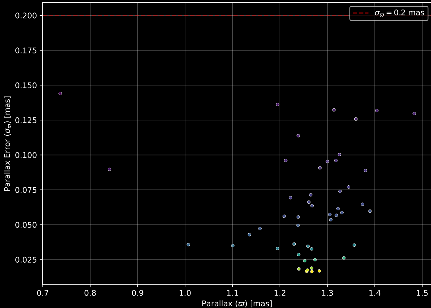
Gaia Cluster: [UPK_282] Parallax Quality (n= 49)
