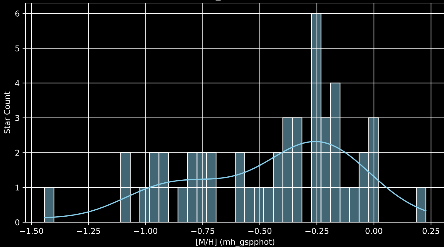
Gaia Cluster: [UPK_282 [M/H] (mh_gspphot) (n= 49)
