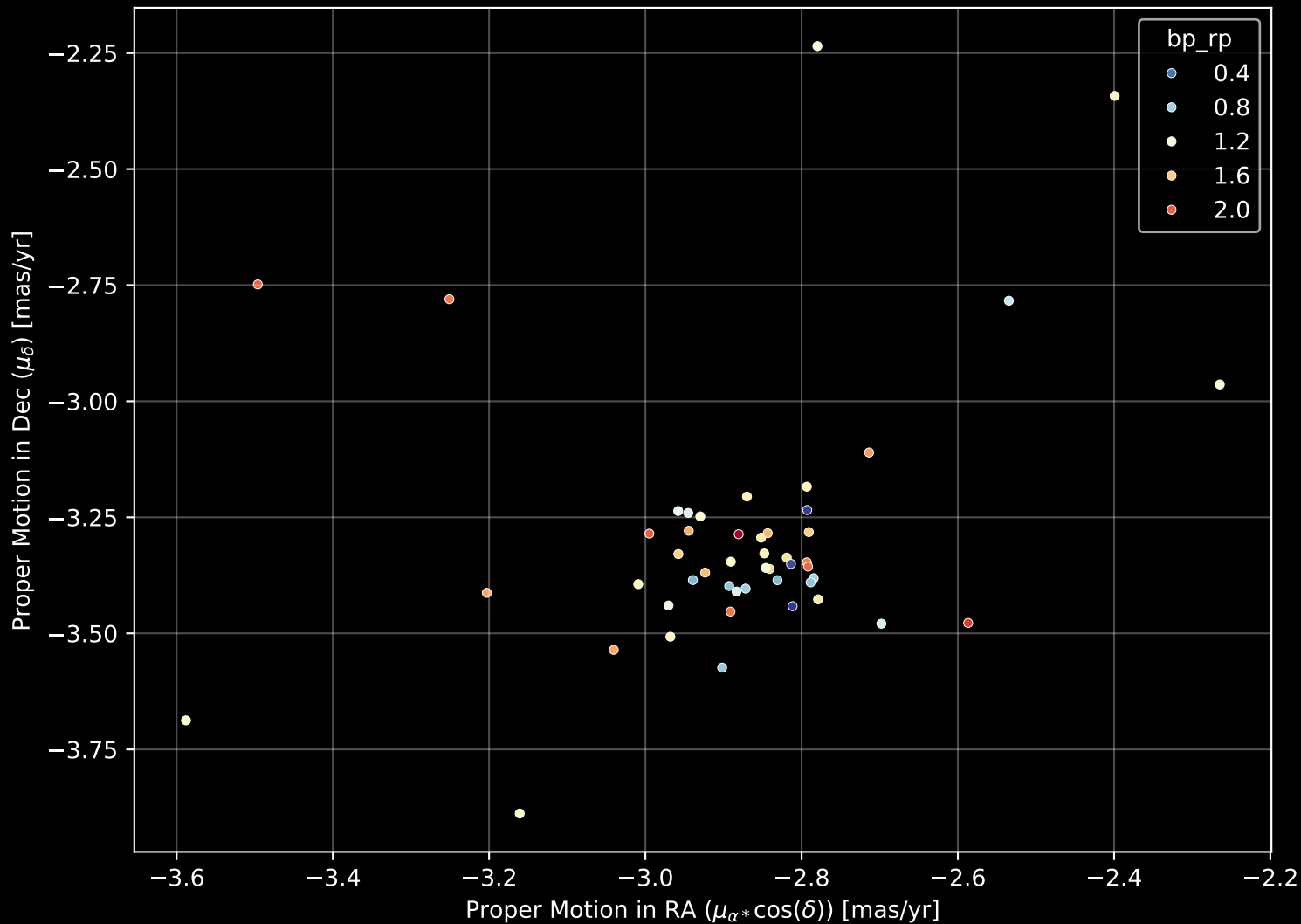
Gaia Cluster: [UPK_282] Proper Motion Diagram (n= 49)
