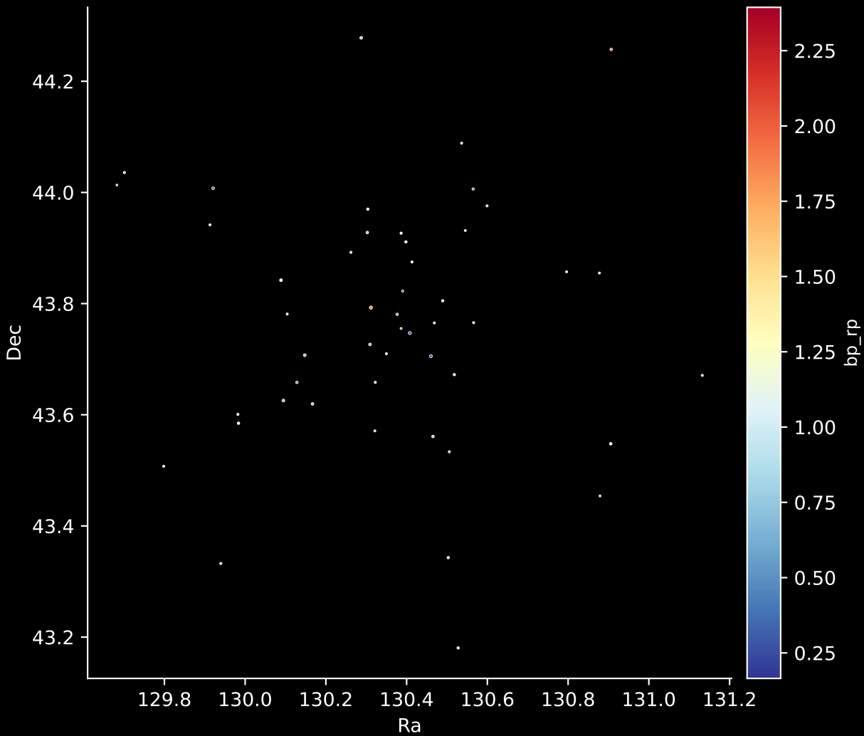
Gaia Cluster: [UPK_282] Stars: 49
