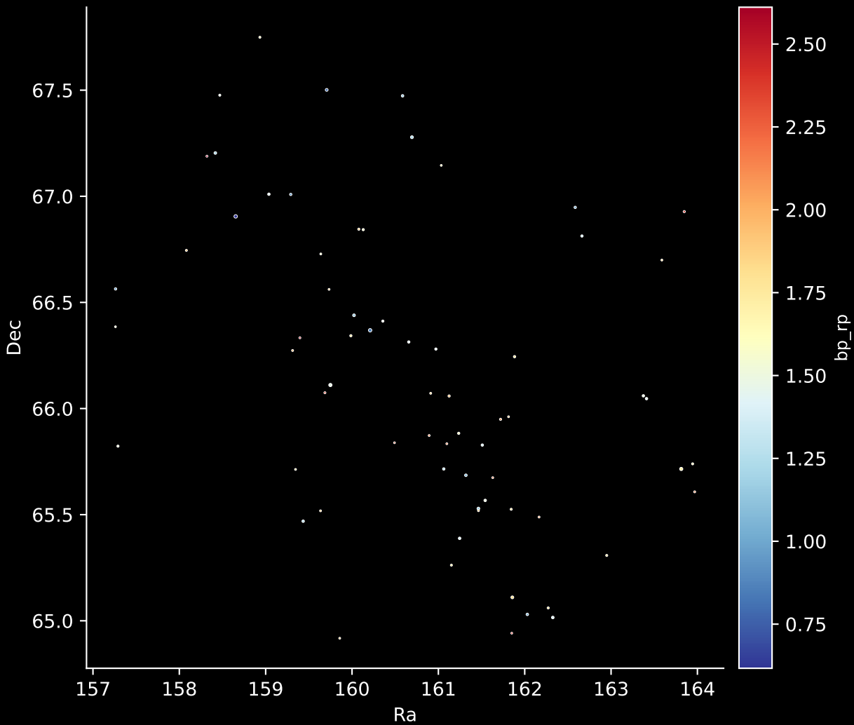
Gaia Cluster: [UPK_294] Stars: 68
