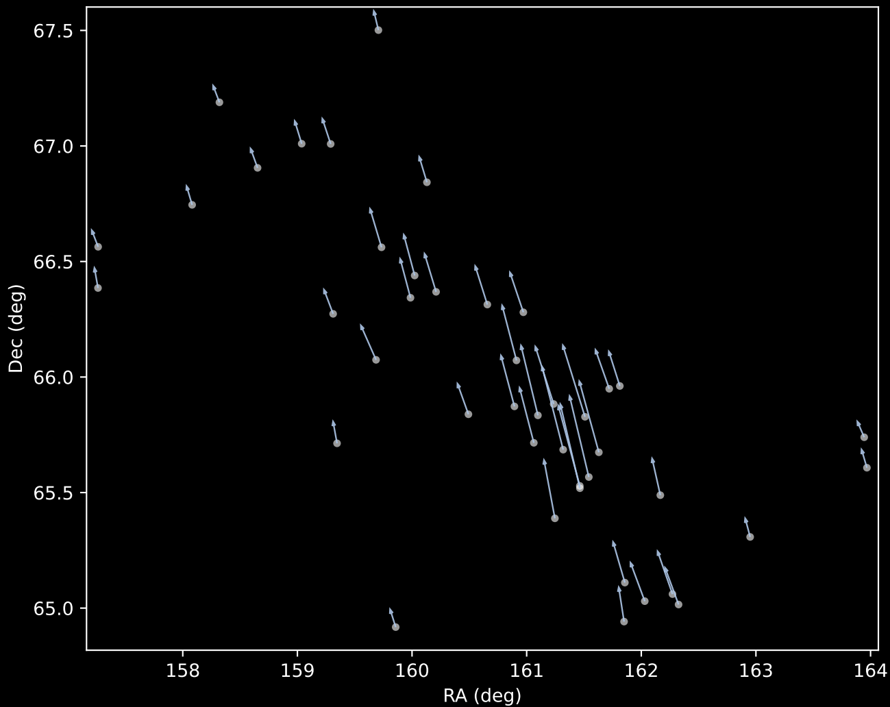
Gaia DR3 Cluster 1 Proper Motion Vectors (n=43)
