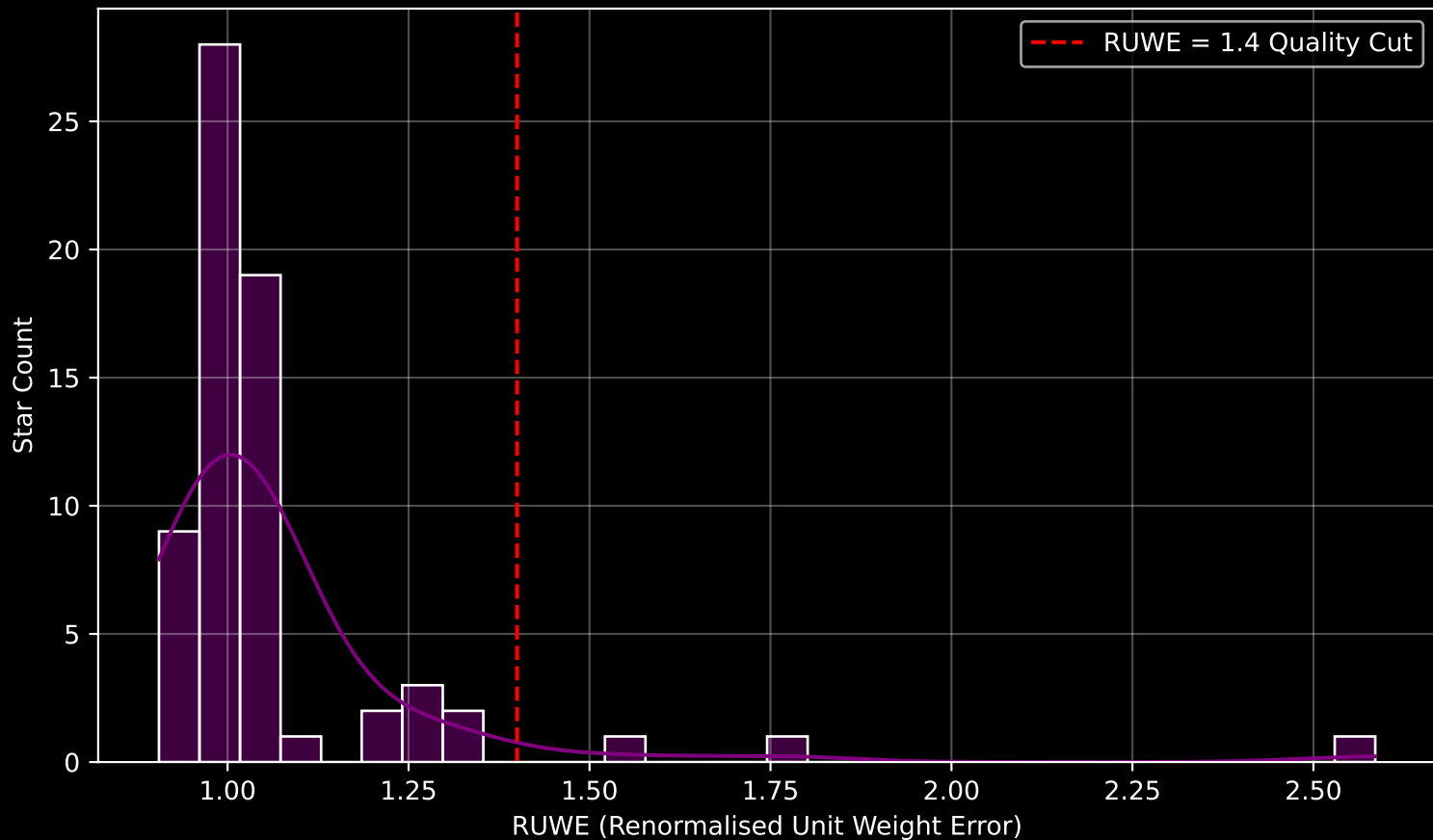
Gaia Cluster: [UPK_294] RUWE Distribution (n= 67)
