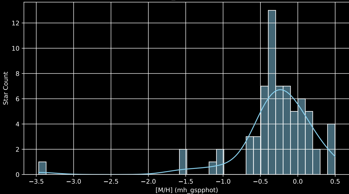
Gaia Cluster: [UPK_294 [M/H] (mh_gspphot) (n= 68)
