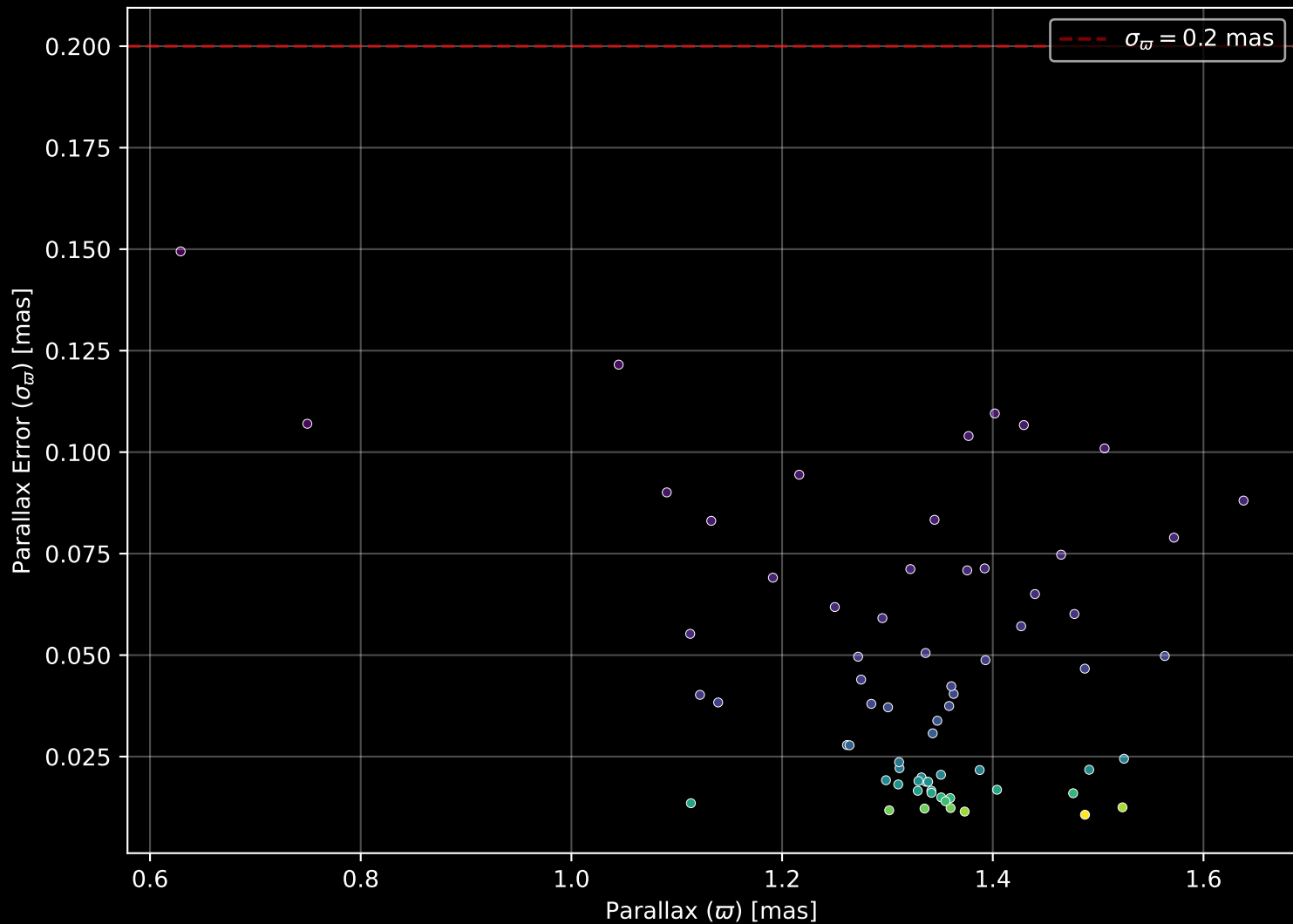
Gaia Cluster: [UPK_294] Parallax Quality (n= 68)
