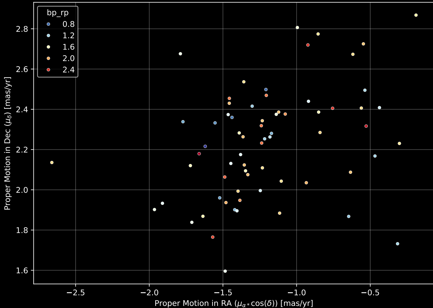
Gaia Cluster: [UPK_294] Proper Motion Diagram (n= 68)
