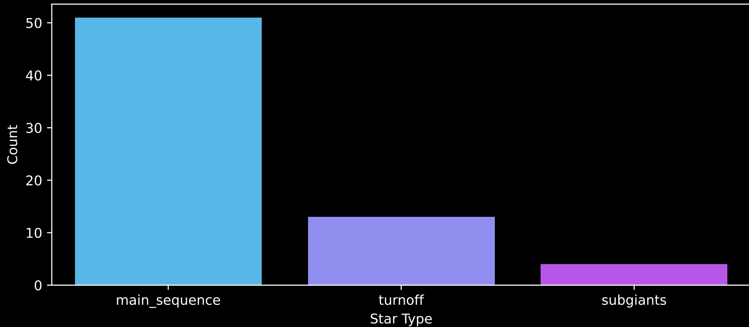
Gaia Cluster: [UPK_294] Count plot of Star Type
