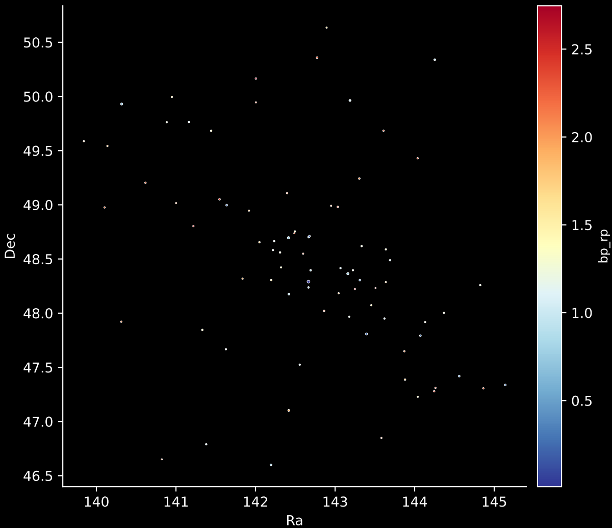
Gaia Cluster: [UPK_296] Stars: 80
