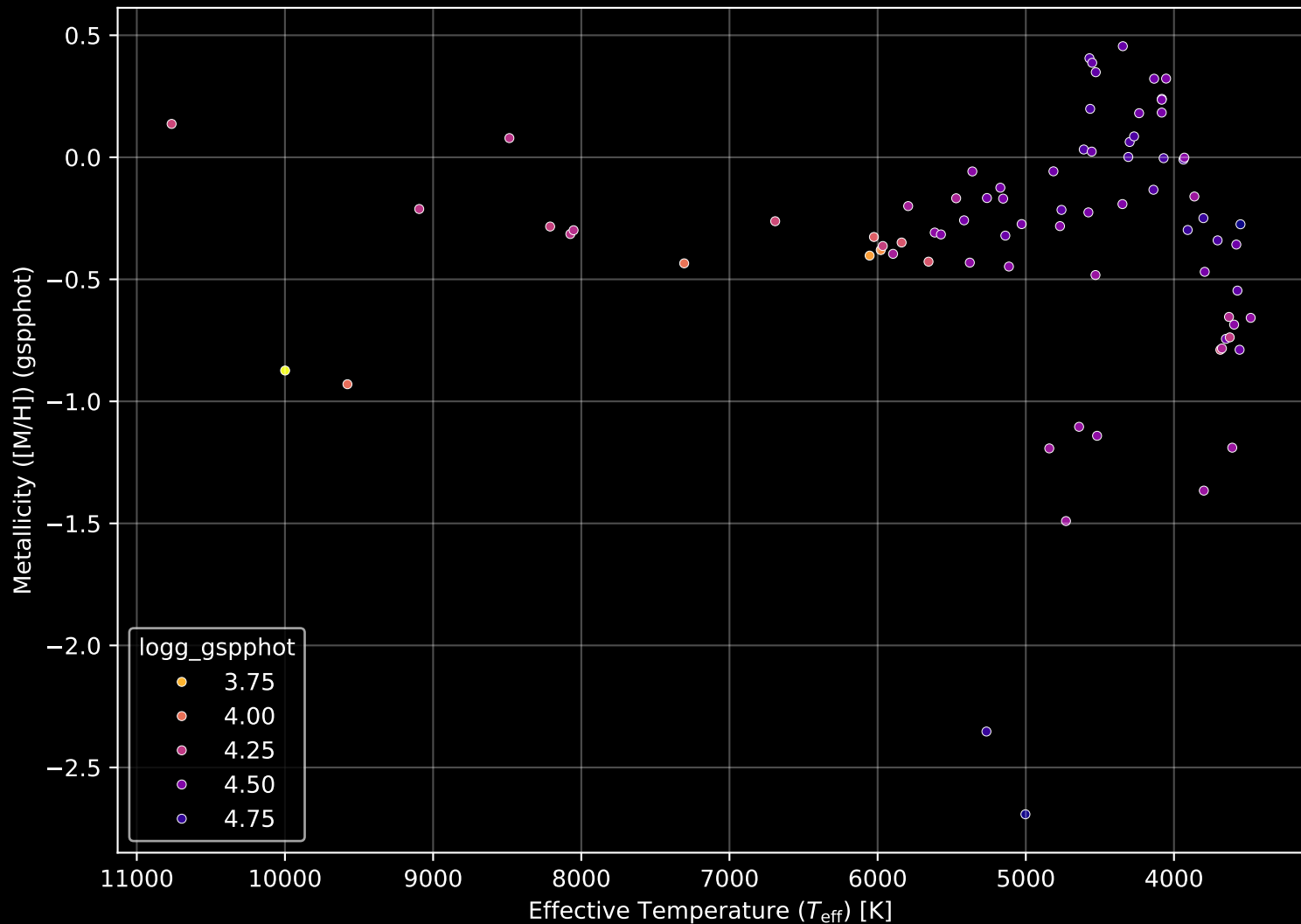
Gaia Cluster: [UPK_296] Stellar Population Parameters (n= 80)
