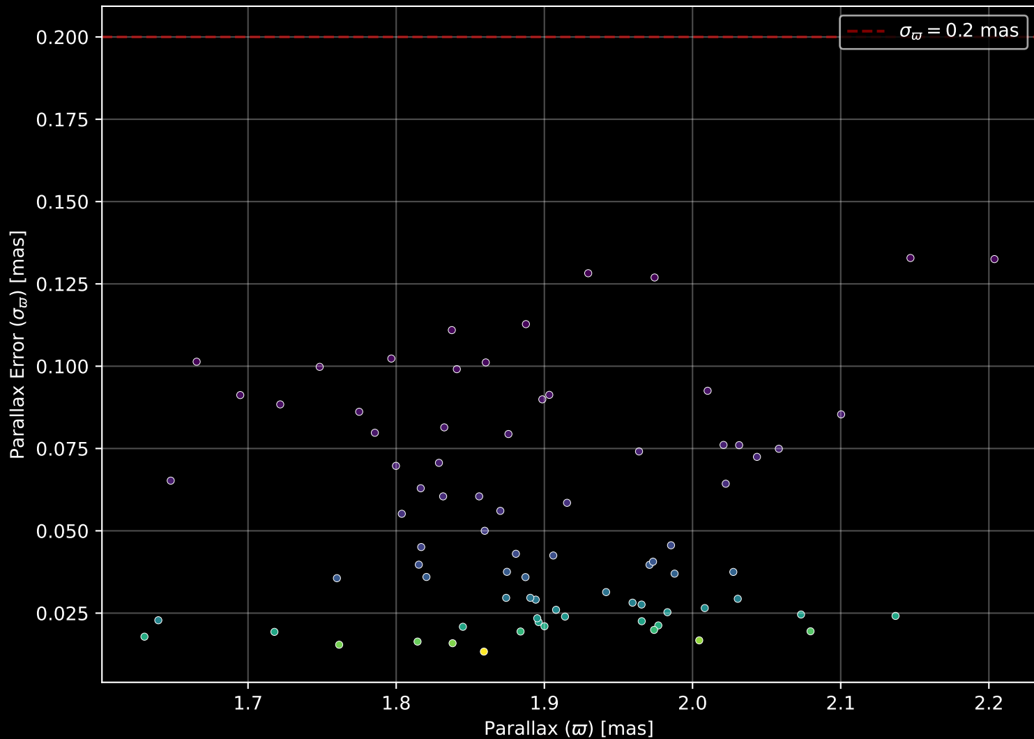
Gaia Cluster: [UPK_296] Parallax Quality (n= 80)
