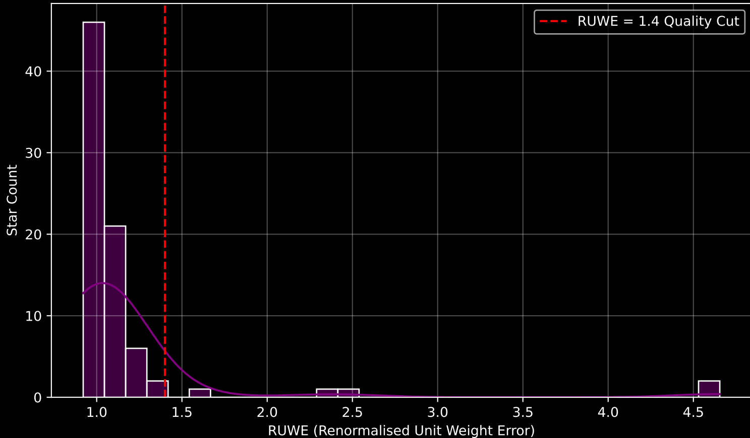
Gaia Cluster: [UPK_296] RUWE Distribution (n= 80)
