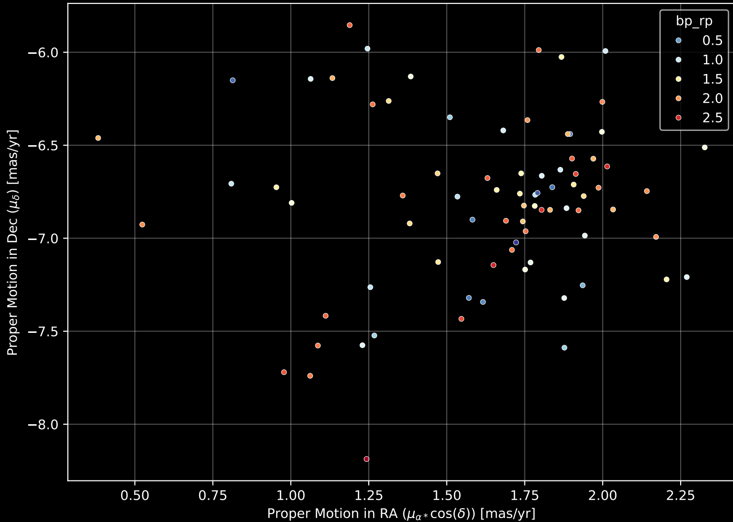
Gaia Cluster: [UPK_296] Proper Motion Diagram (n= 80)
