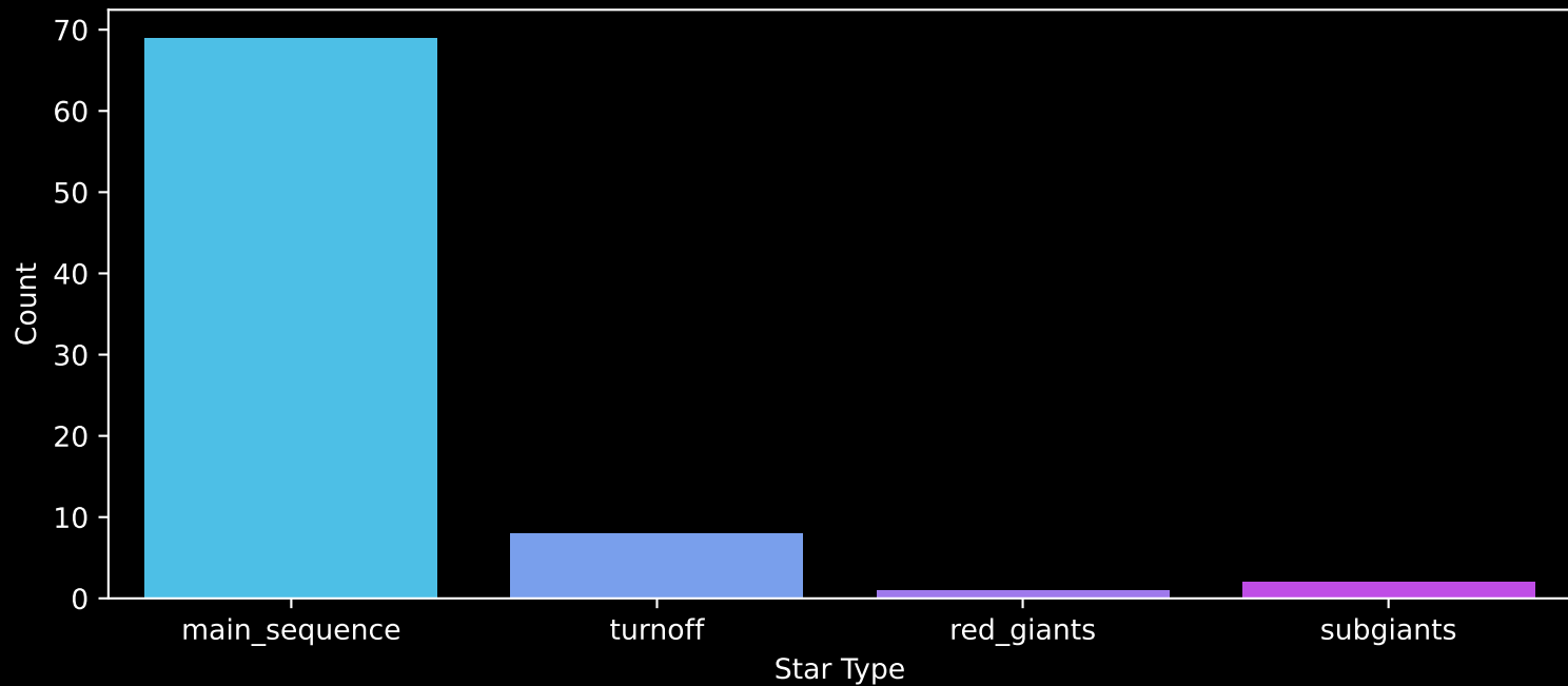
Gaia Cluster: [UPK_296] Count plot of Star Type
