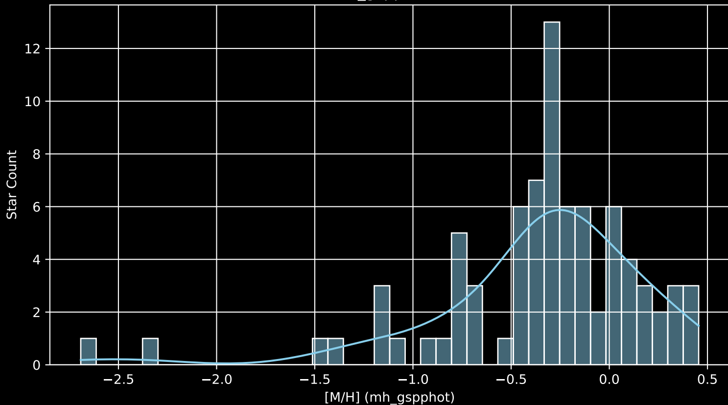
Gaia Cluster: [UPK_296 [M/H] (mh_gspphot) (n= 80)
