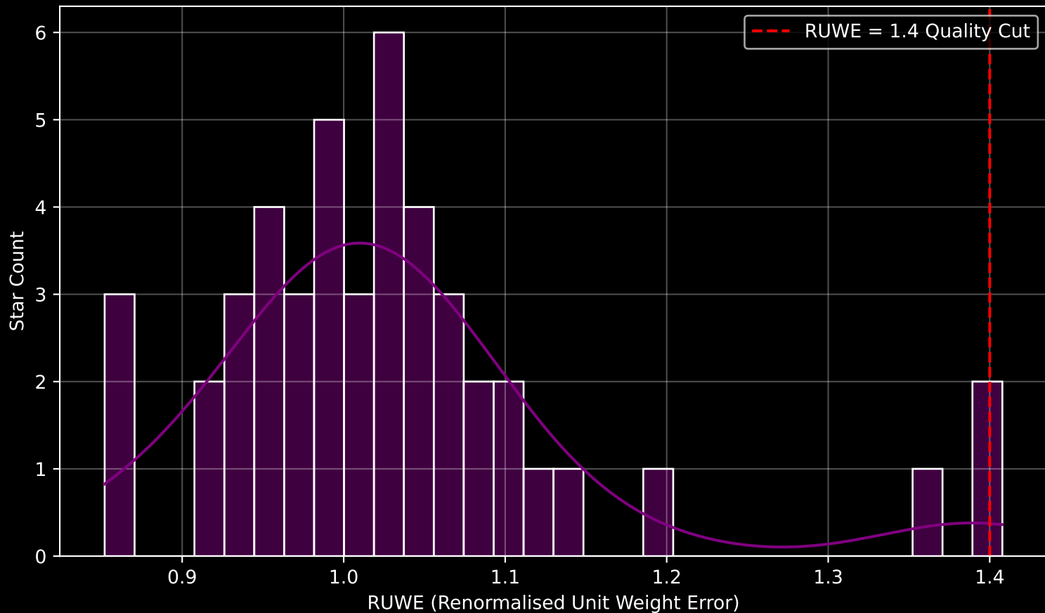
Gaia Cluster: [UPK_31] RUWE Distribution (n= 46)
