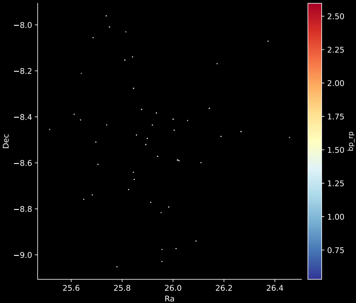
Gaia Cluster: [UPK_31] Stars: 46
