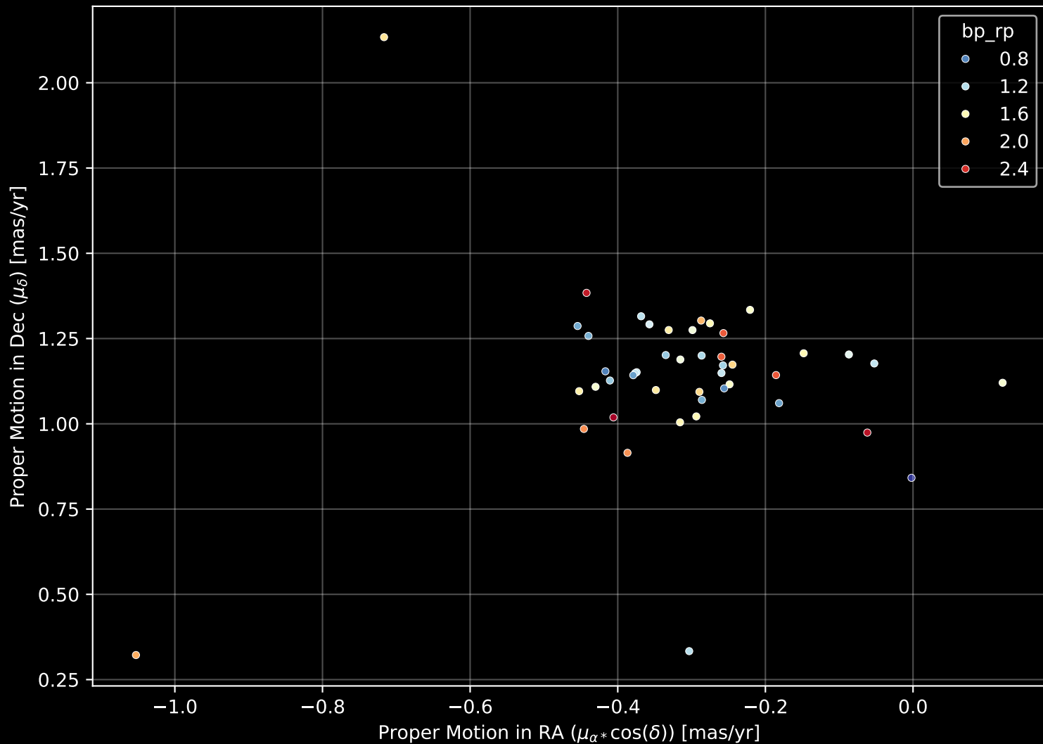
Gaia Cluster: [UPK_31] Proper Motion Diagram (n= 46)
