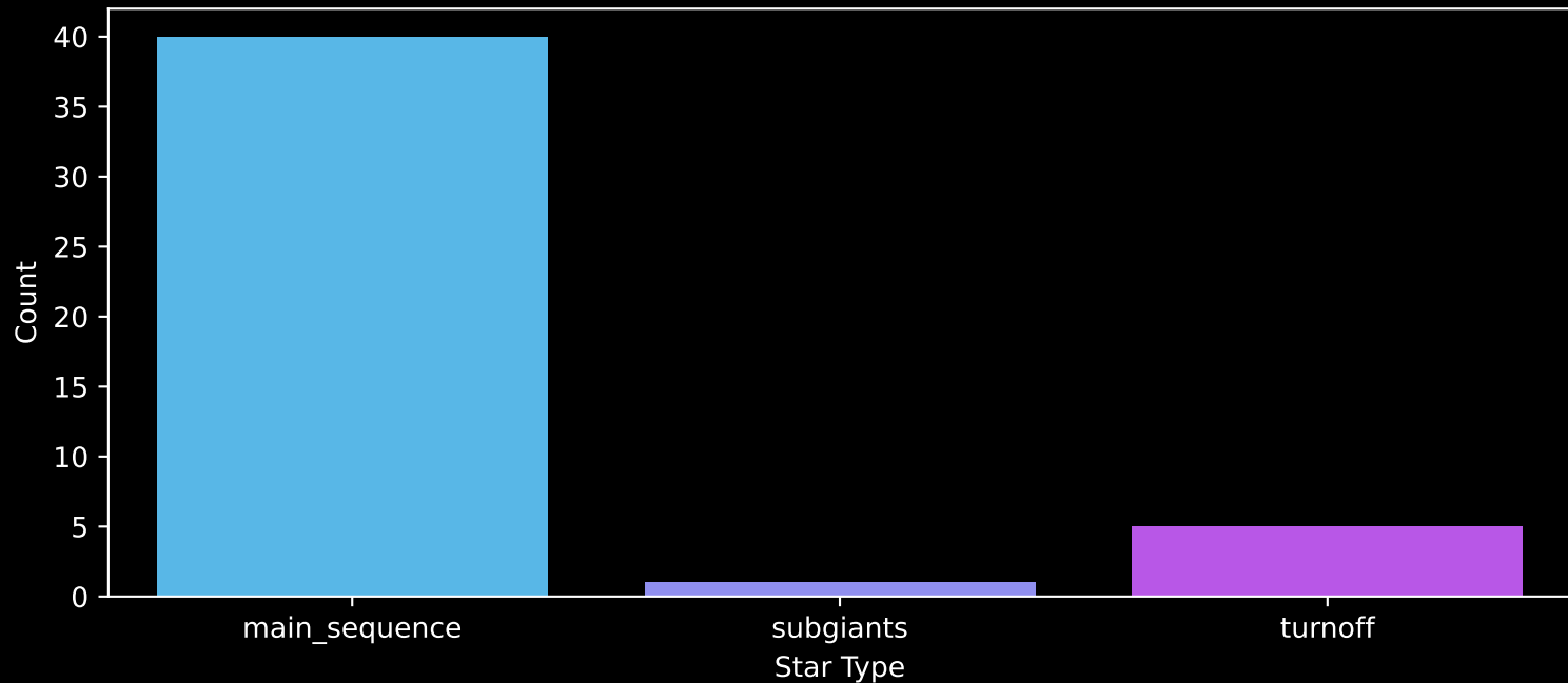
Gaia Cluster: [UPK_31] Count plot of Star Type
