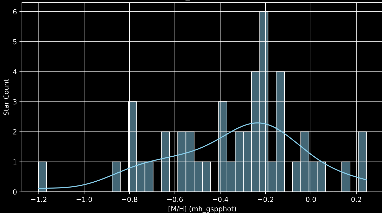
Gaia Cluster: [UPK_31 [M/H] (mh_gspphot) ( \bar{n}= 46 )
