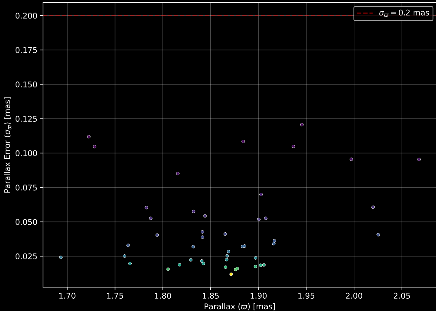
Gaia Cluster: [UPK_31] Parallax Quality (n= 46)
