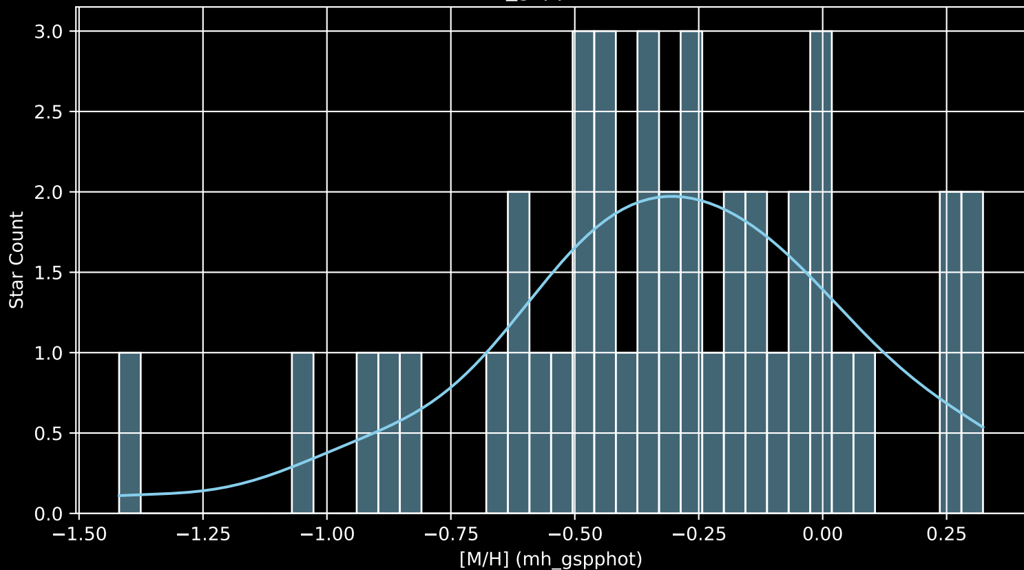
Gaia Cluster: [UPK_312 [M/H] (mh_gspphot) (n= 42)
