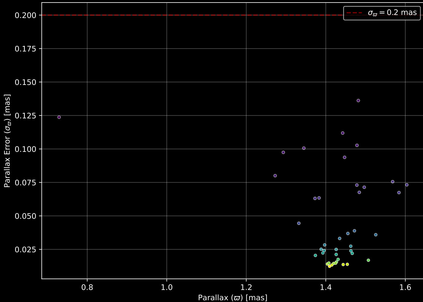
Gaia Cluster: [UPK_312] Parallax Quality (n= 42)
