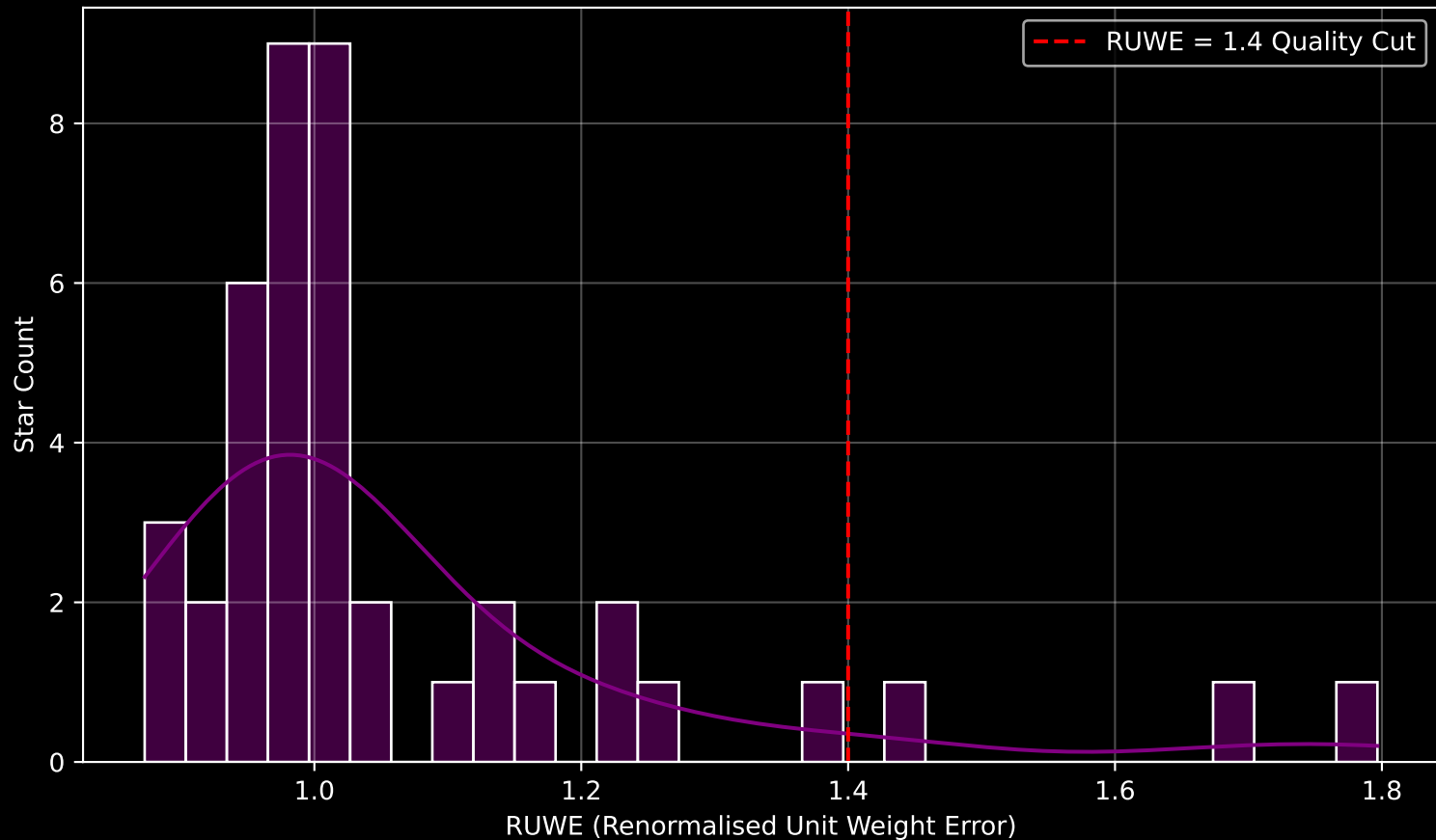
Gaia Cluster: [UPK_312] RUWE Distribution (n= 42)
