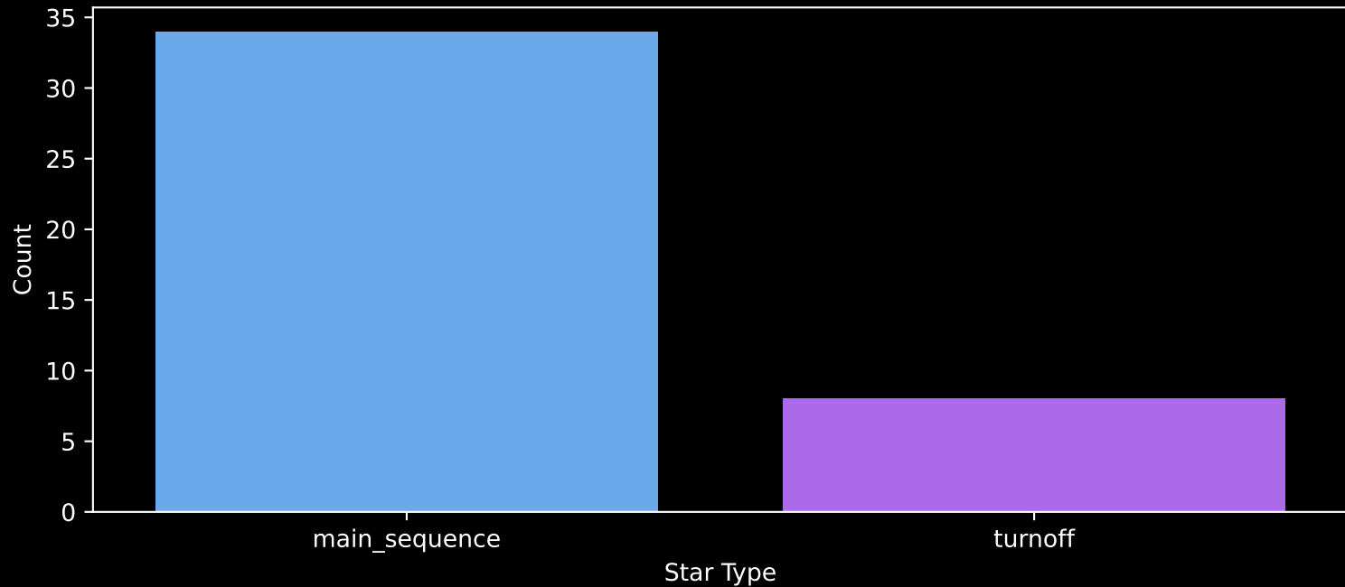
Gaia Cluster: [UPK_312] Count plot of Star Type
