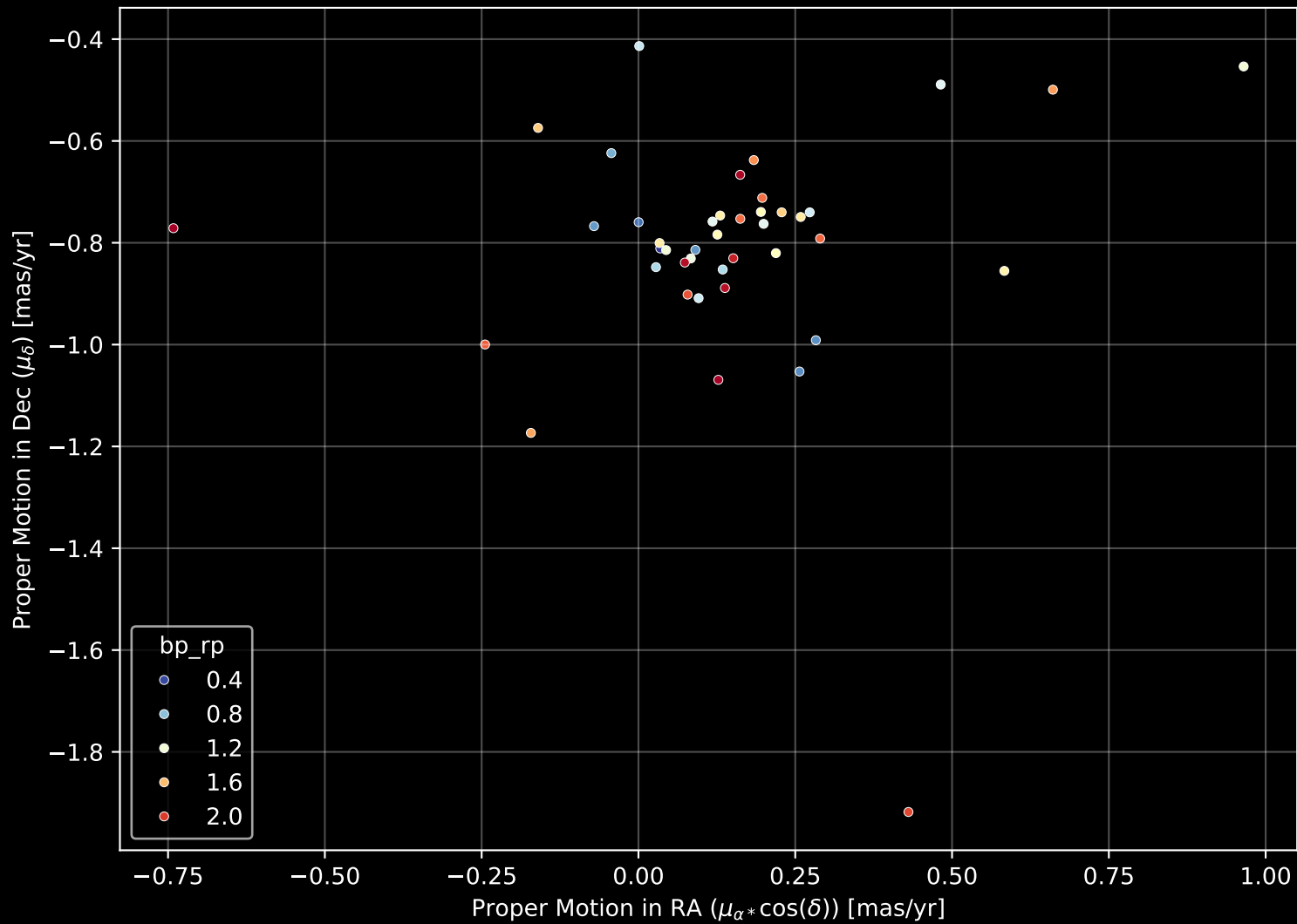
Gaia Cluster: [UPK_312] Proper Motion Diagram (n= 42)
