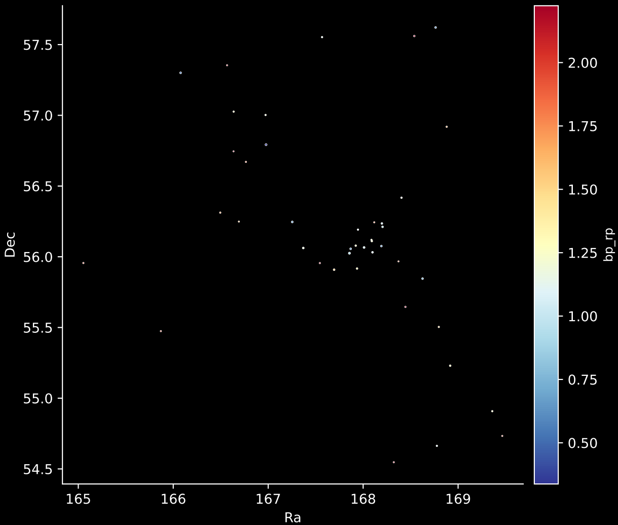
Gaia Cluster: [UPK_312] Stars: 42
