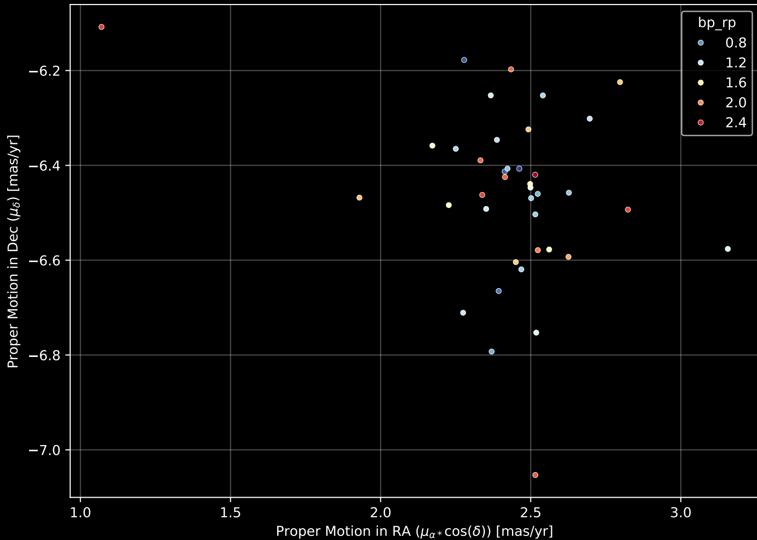
Gaia Cluster: [UPK_333] Proper Motion Diagram (n= 39)
