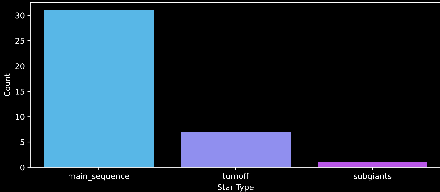
Gaia Cluster: [UPK_333] Count plot of Star Type
