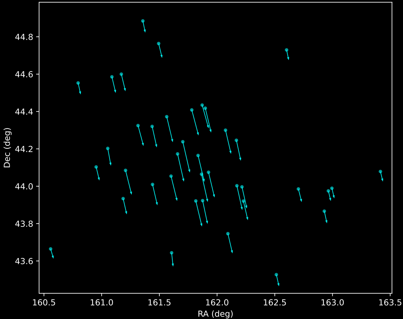
Gaia DR3 Noise Stream Proper Motion Vectors (n=39)
