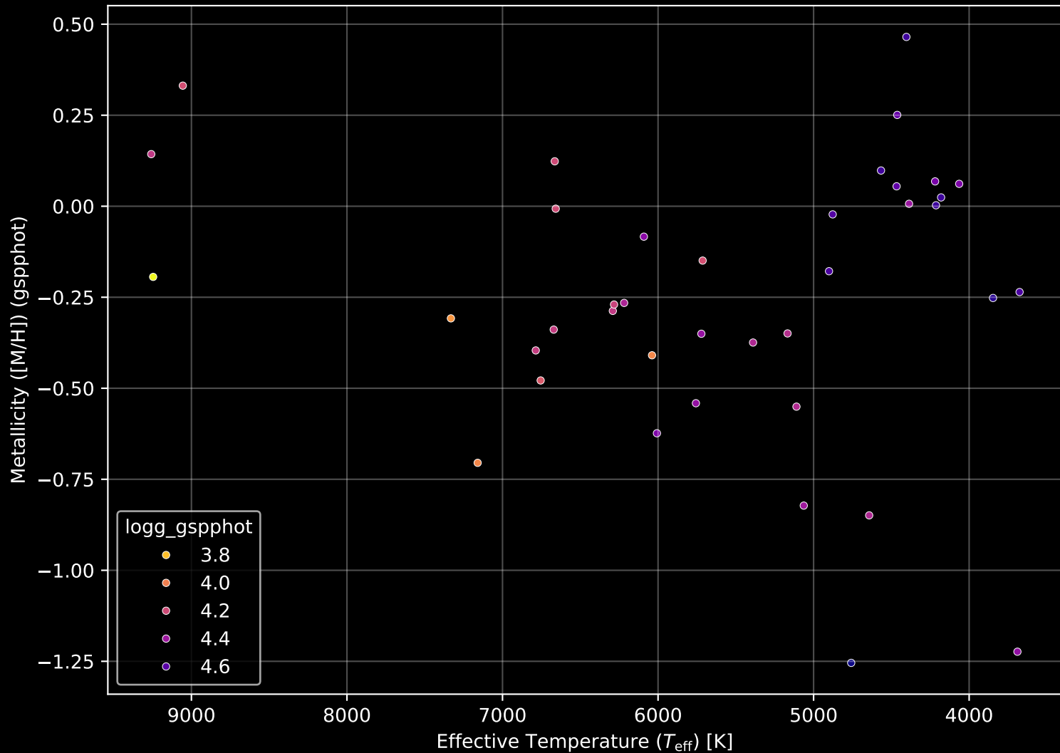
Gaia Cluster: [UPK_333] Stellar Population Parameters (n= 39)
