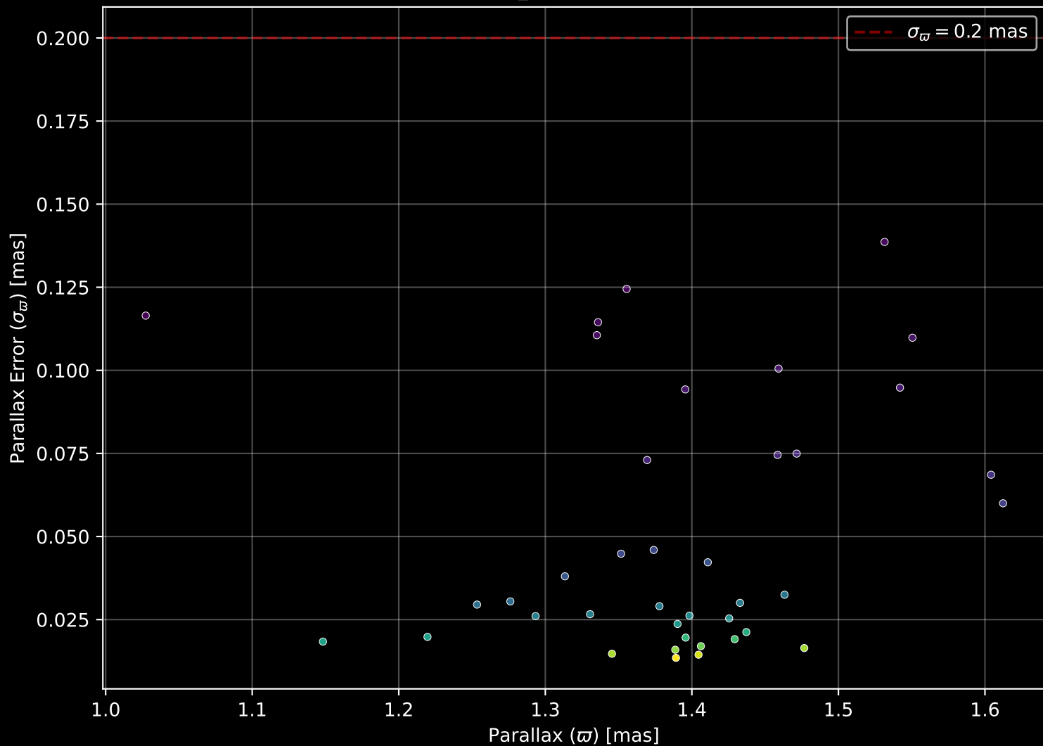
Gaia Cluster: [UPK_333] Parallax Quality (n= 39)
