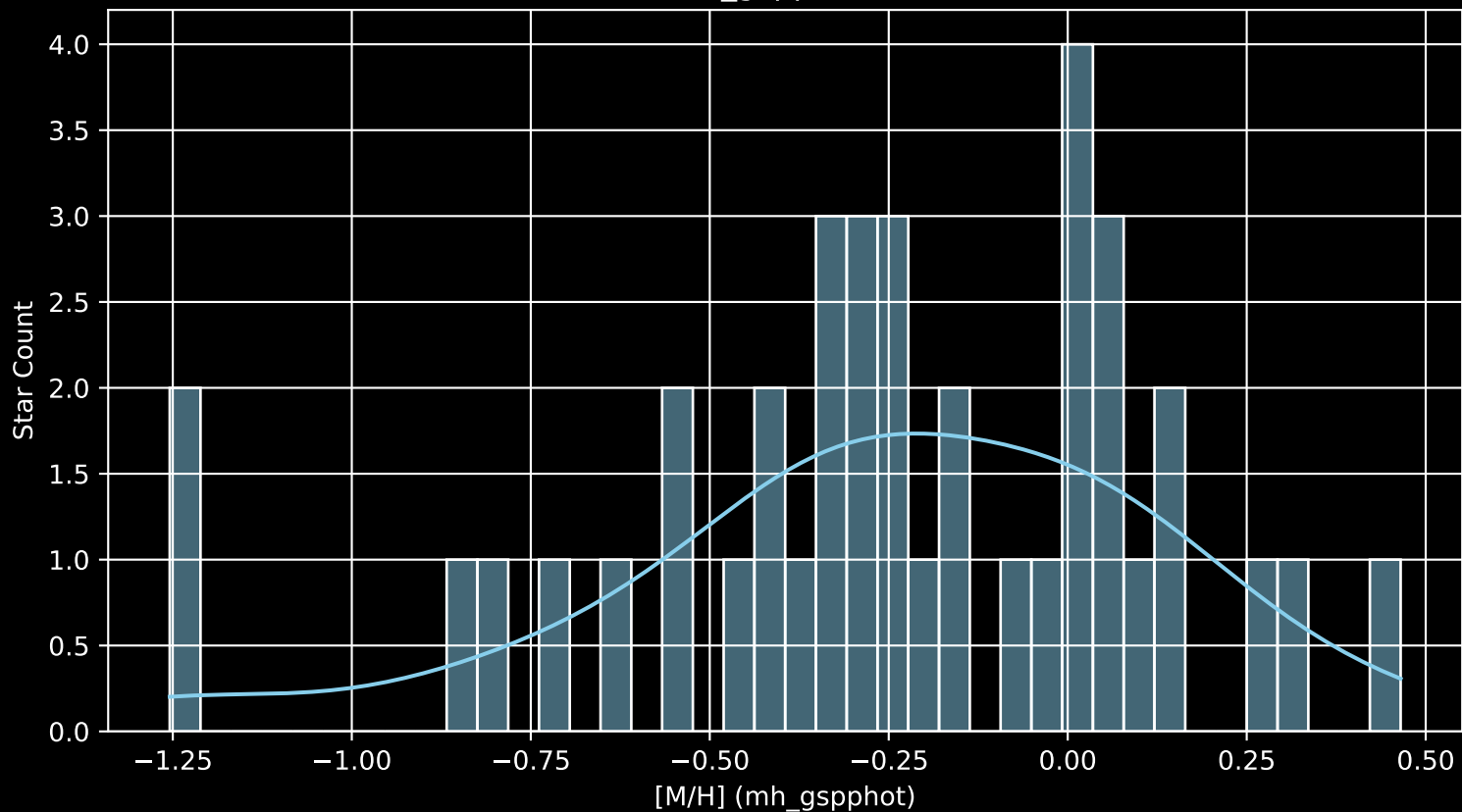
Gaia Cluster: [UPK_333 [M/H] (mh_gspphot) (n= 39)
