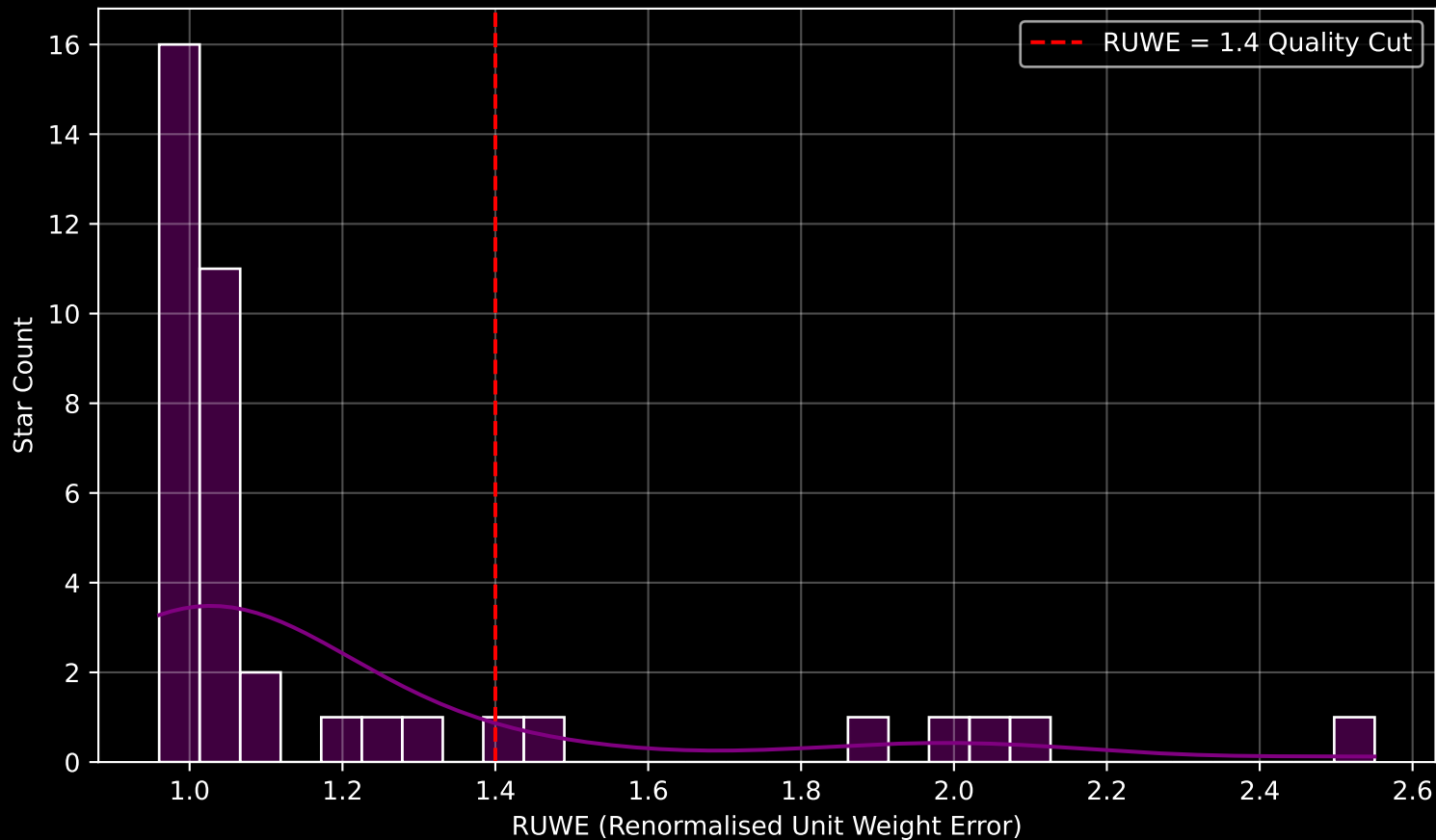
Gaia Cluster: [UPK_333] RUWE Distribution (n= 39)
