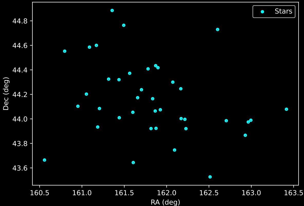
Gaia Cluster: [UPK_333] Proper Motion Vectors for Gaia Star Field (n= 39)
