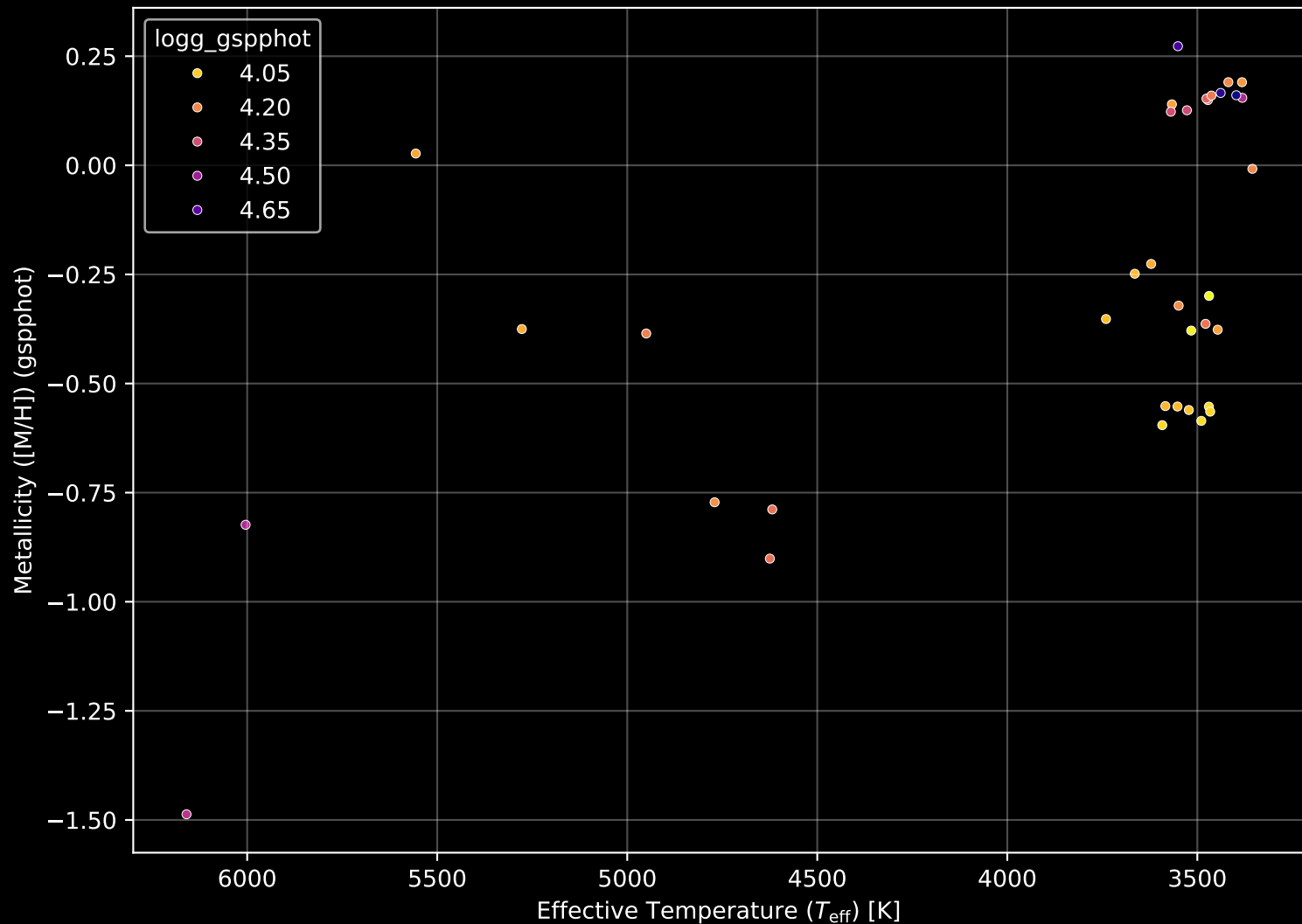
Gaia Cluster: [UPK_398] Stellar Population Parameters (n= 36)
