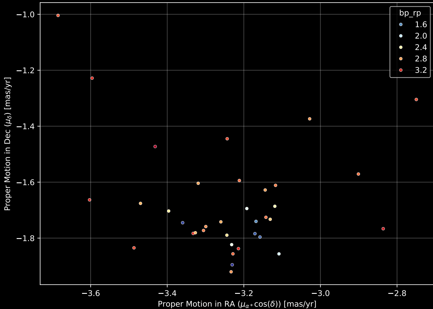
Gaia Cluster: [UPK_398] Proper Motion Diagram (n= 36)
