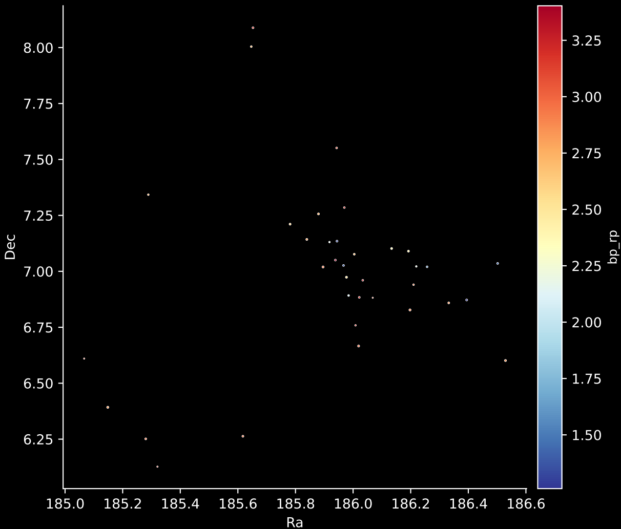
Gaia Cluster: [UPK_398] Stars: 36
