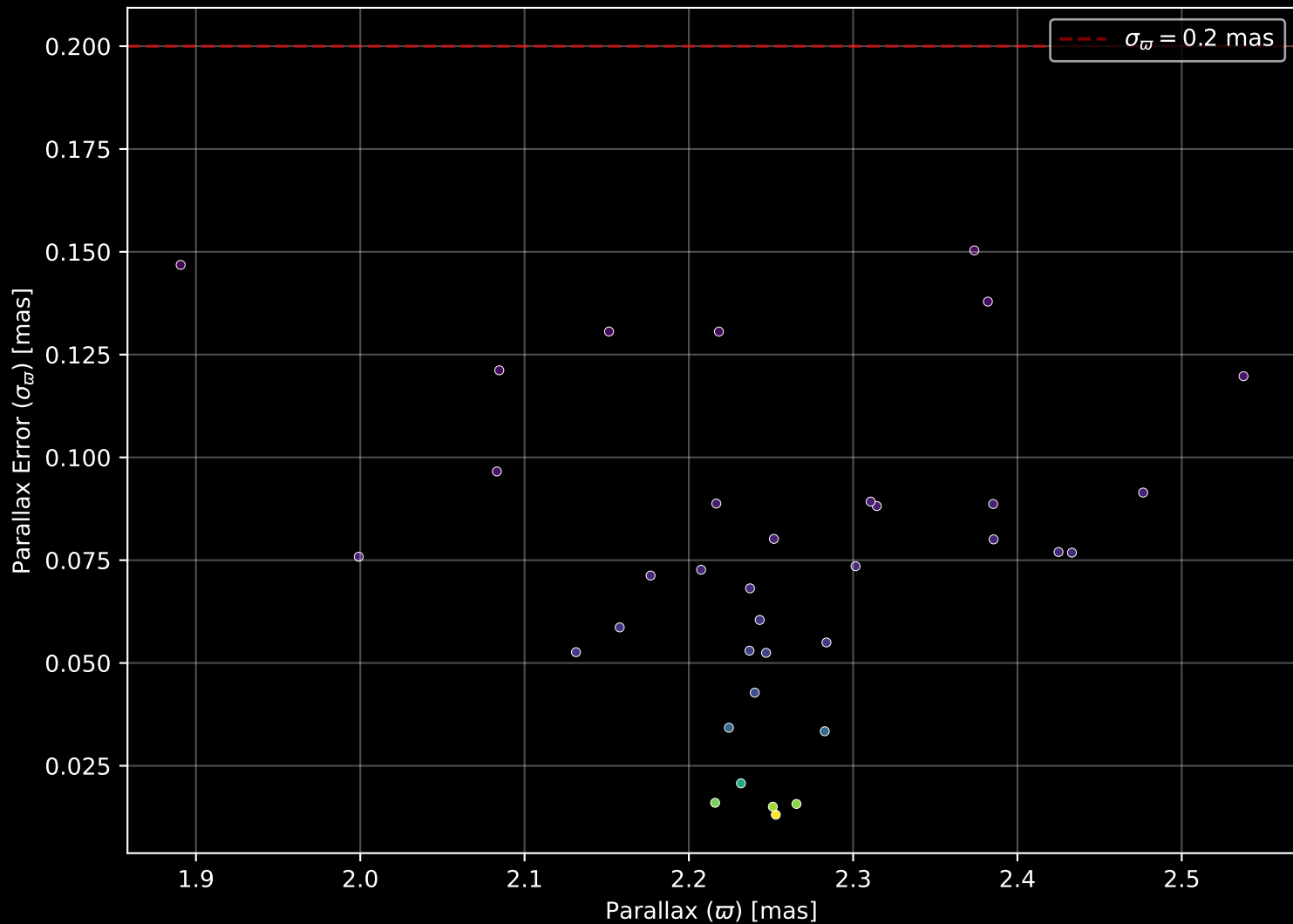
Gaia Cluster: [UPK_398] Parallax Quality (n= 36)
