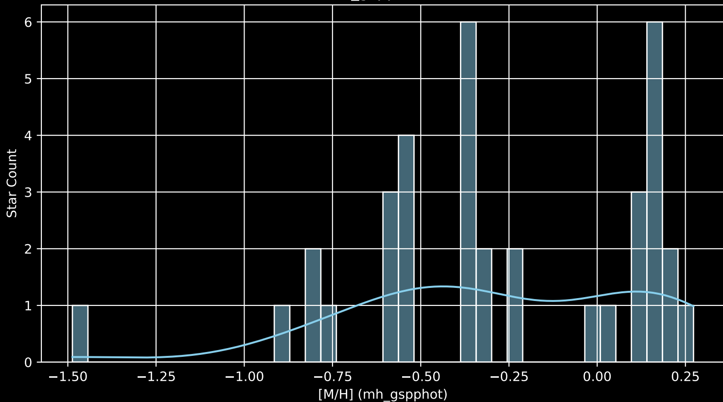
Gaia Cluster: [UPK_398 [M/H] (mh_gspphot) (n= 36)
