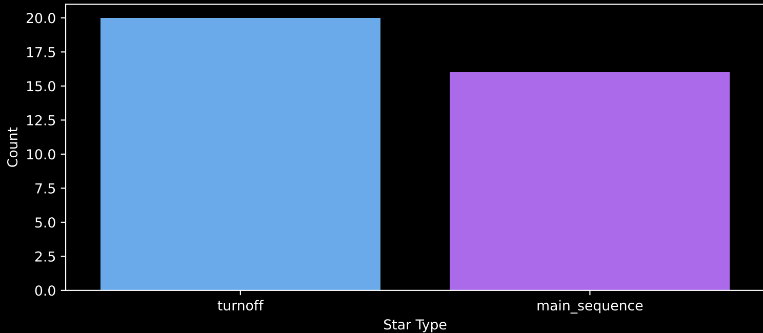
Gaia Cluster: [UPK_398] Count plot of Star Type
