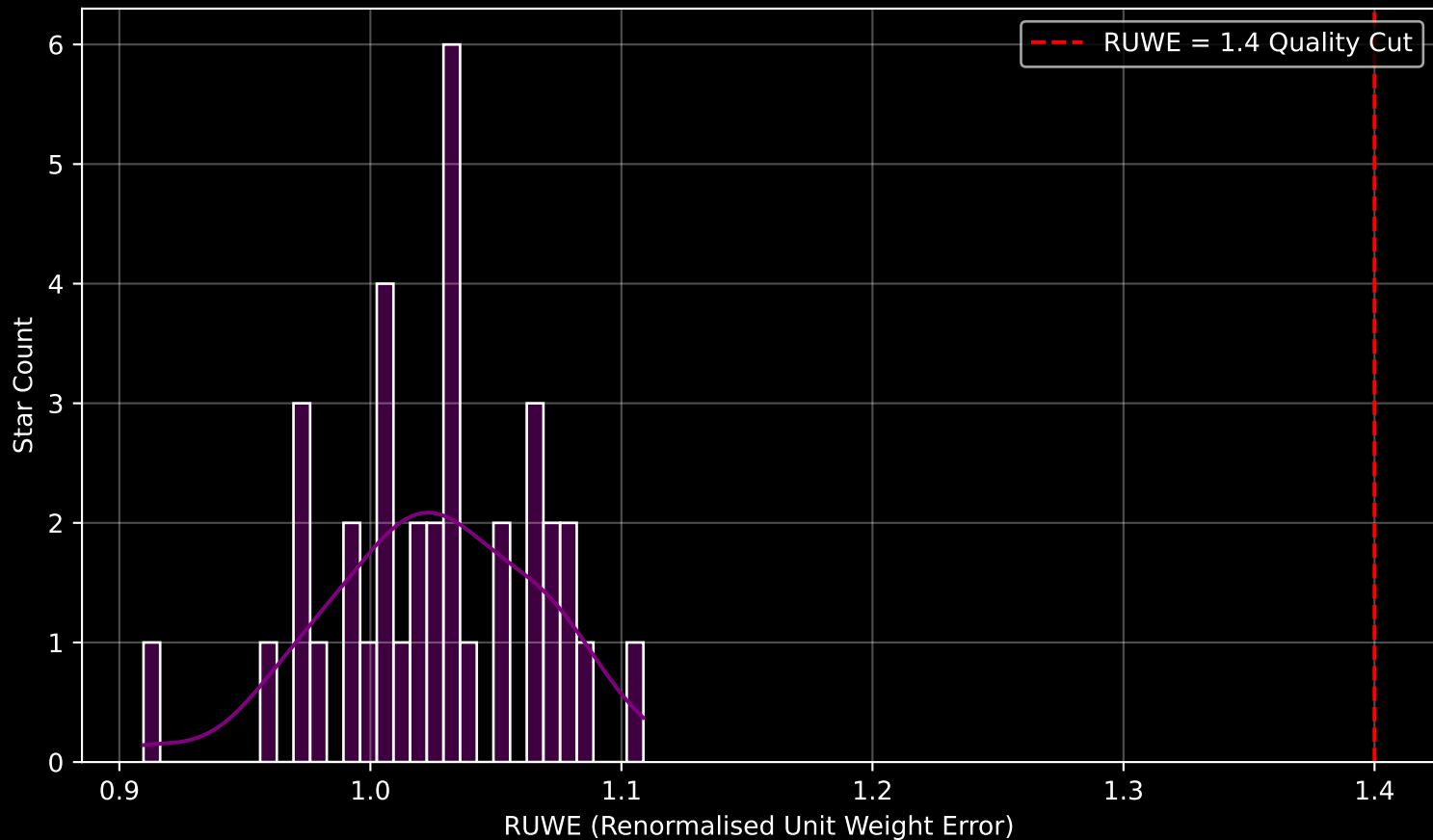
Gaia Cluster: [UPK_398] RUWE Distribution (n= 36)
