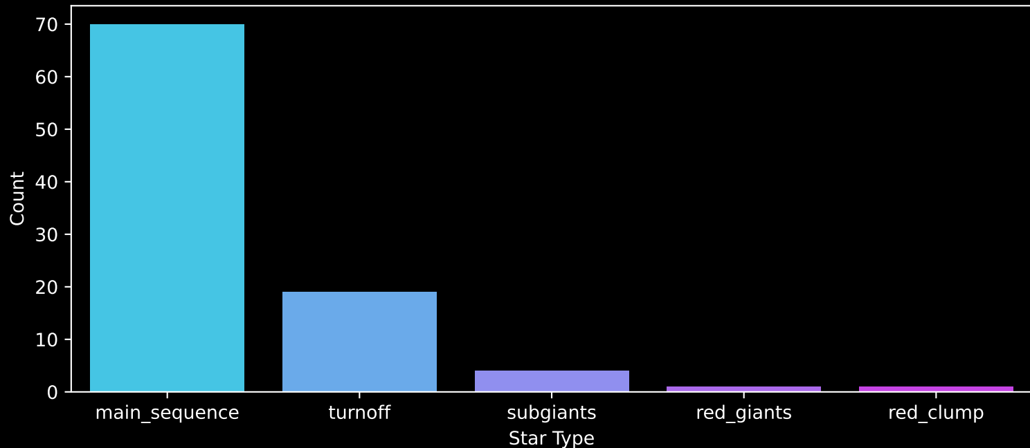
Gaia Cluster: [UPK_40] Count plot of Star Type
