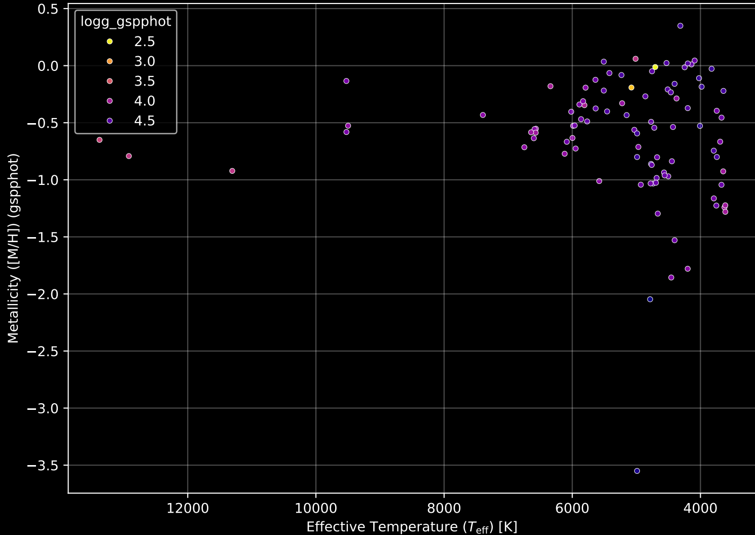
Gaia Cluster: [UPK_40] Stellar Population Parameters (n= 95)
