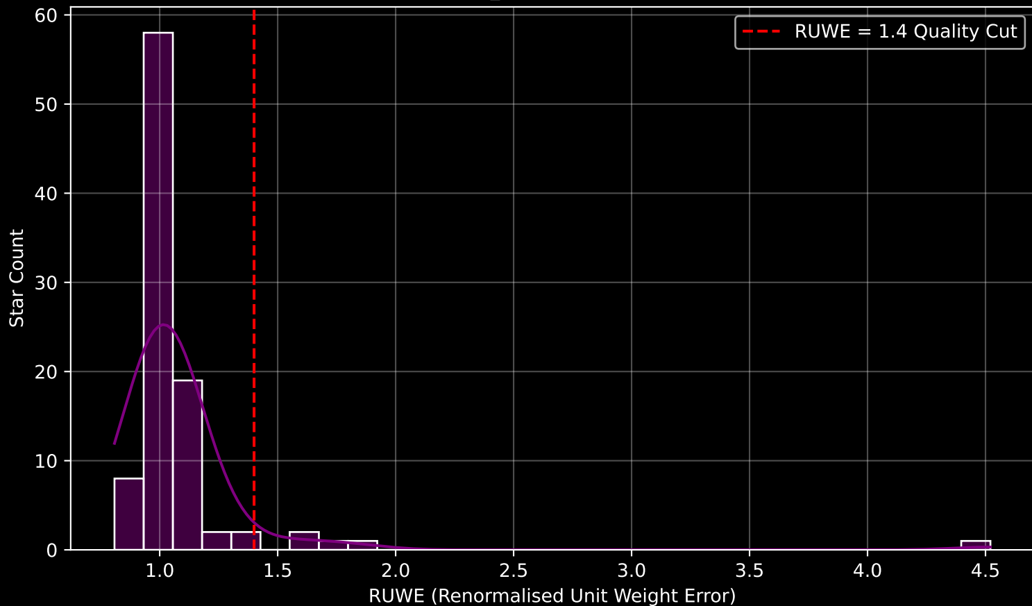
Gaia Cluster: [UPK_40] RUWE Distribution (n= 94)
