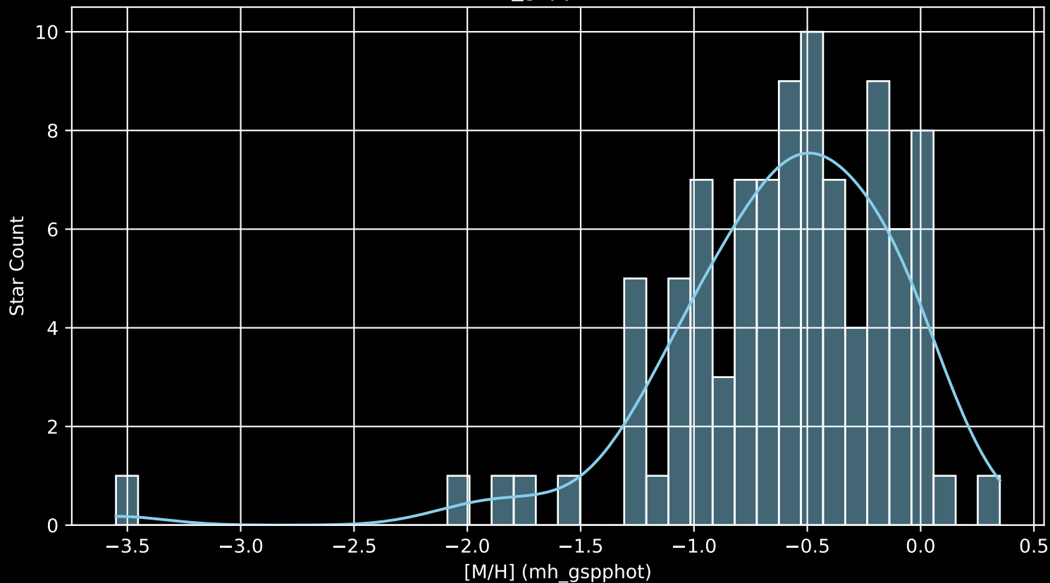
Gaia Cluster: [UPK_40 [M/H] (mh_gspphot) (n= 95)
