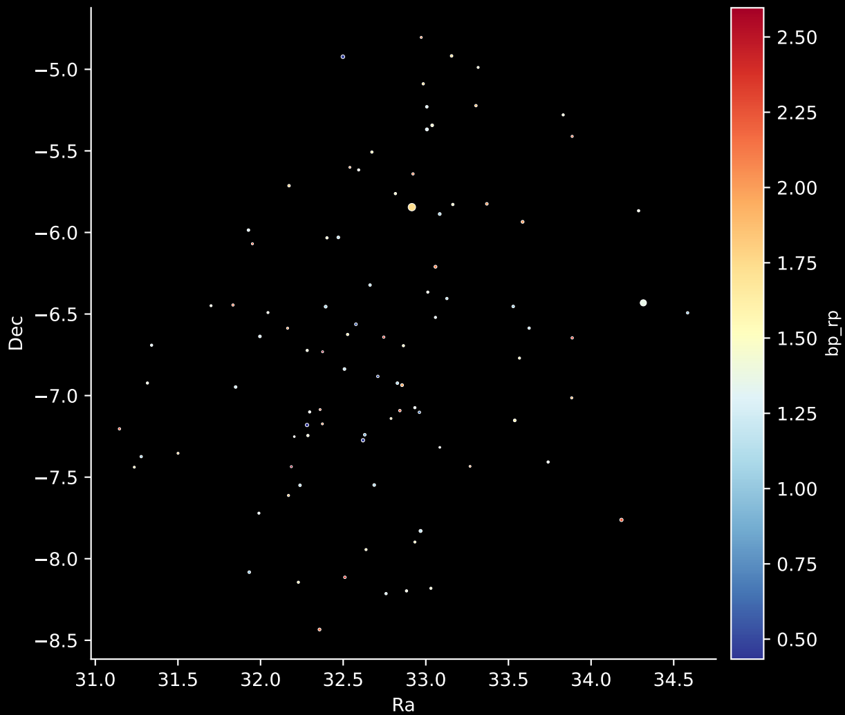
Gaia Cluster: [UPK_40] Stars: 95
