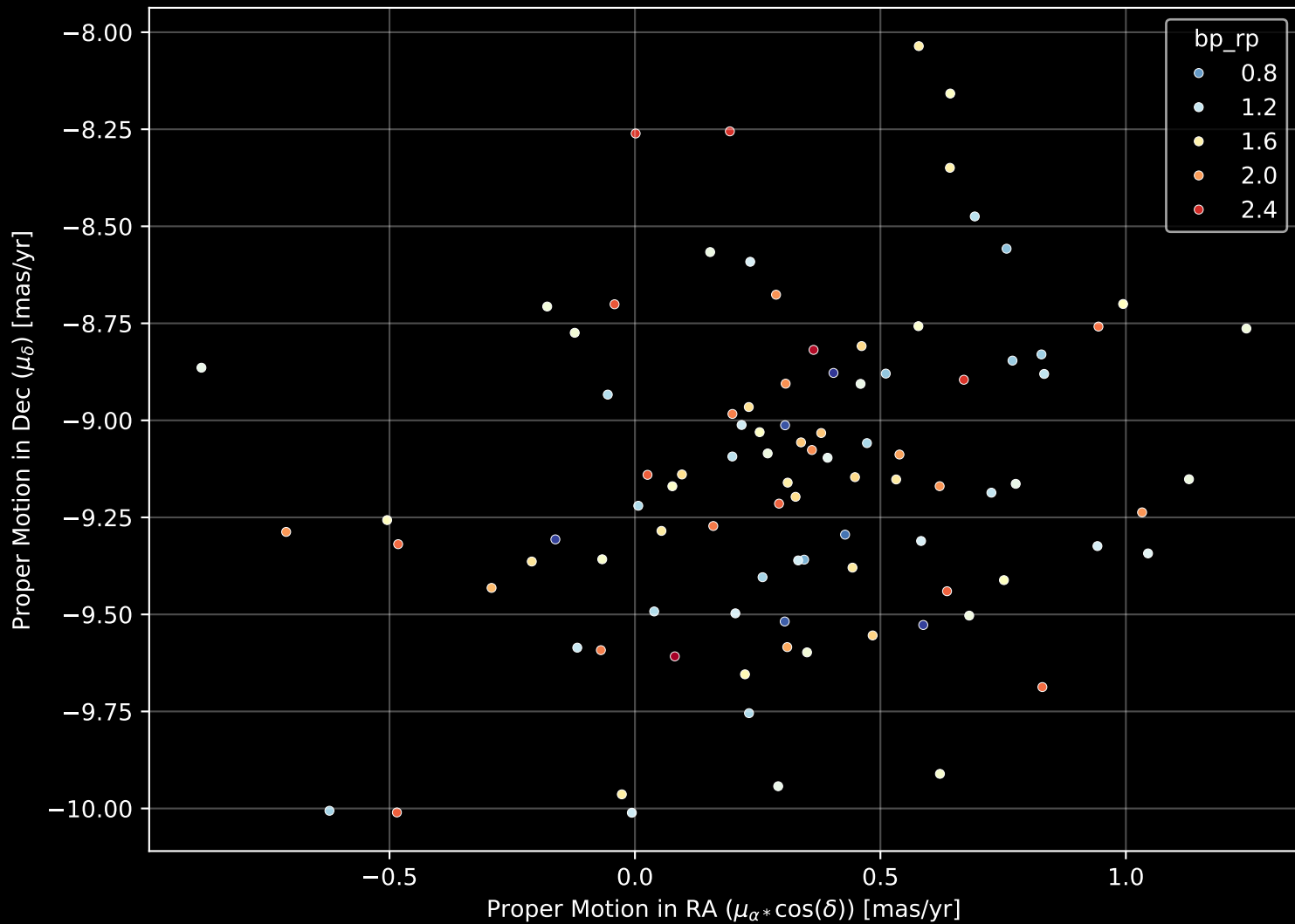
Gaia Cluster: [UPK_40] Proper Motion Diagram (n= 95)
