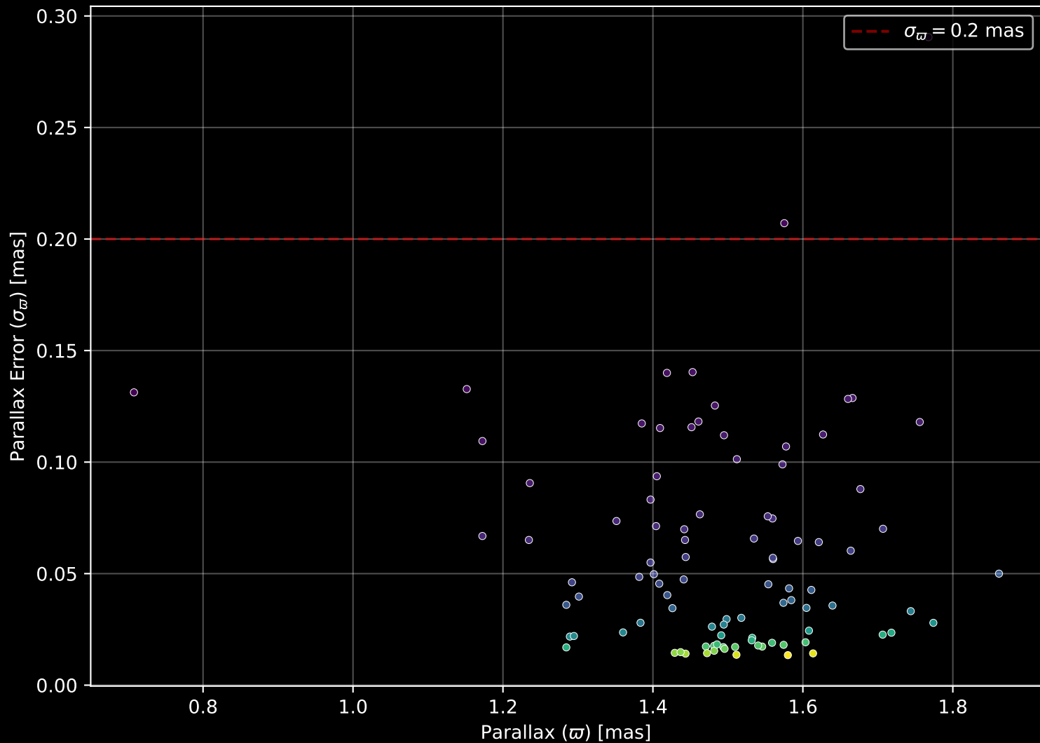
Gaia Cluster: [UPK_40] Parallax Quality (n= 95)
