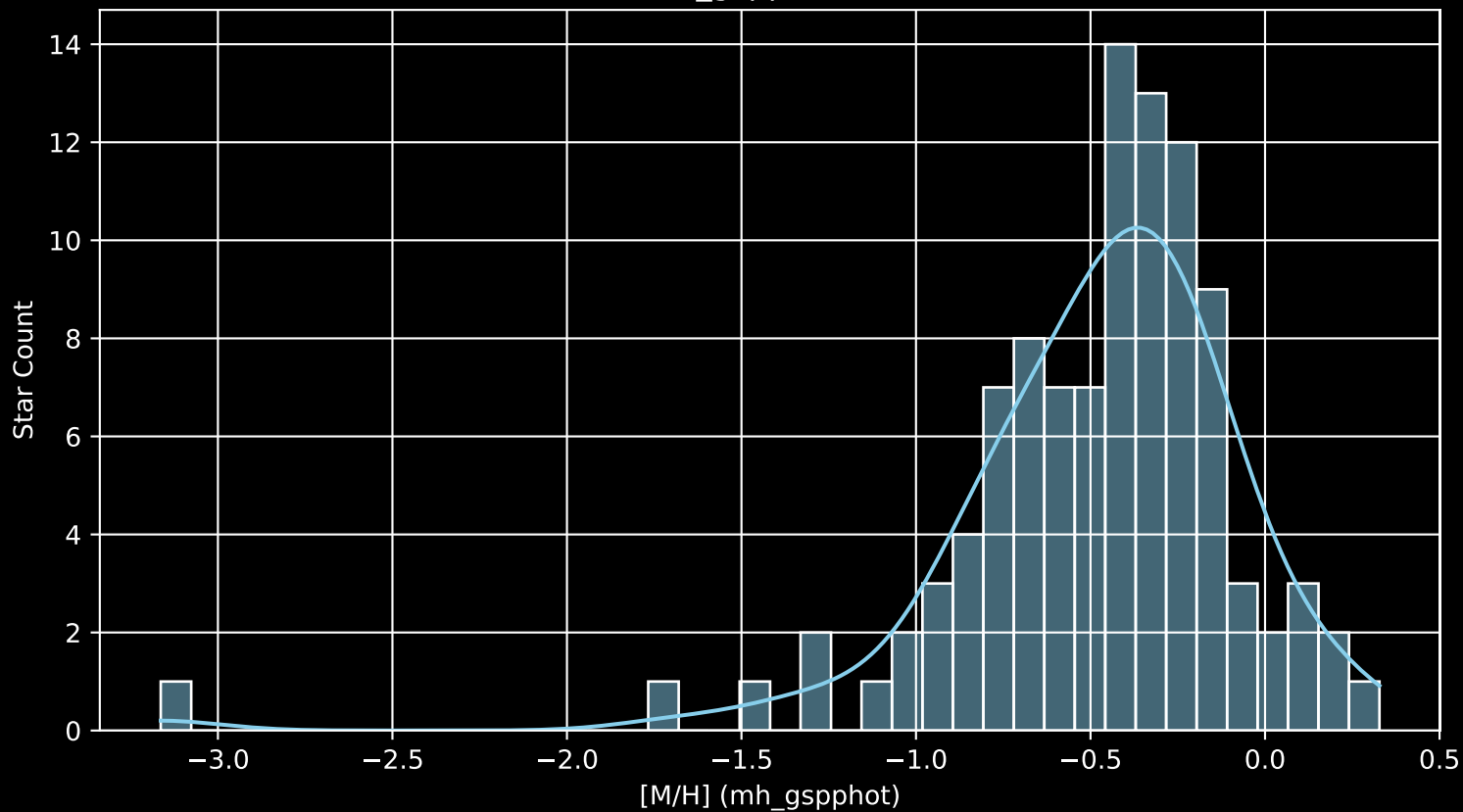
Gaia Cluster: [UPK_436 [M/H] (mh_gspphot) (n= 103)
