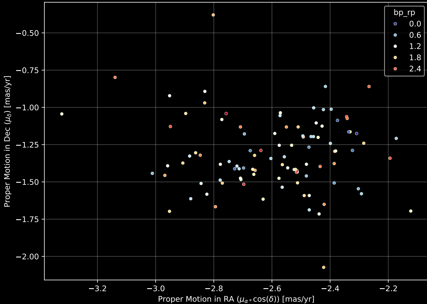
Gaia Cluster: [UPK_442] Proper Motion Diagram (n= 101)
