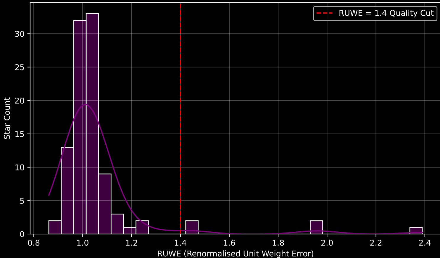
Gaia Cluster: [UPK_442] RUWE Distribution (n= 100)
