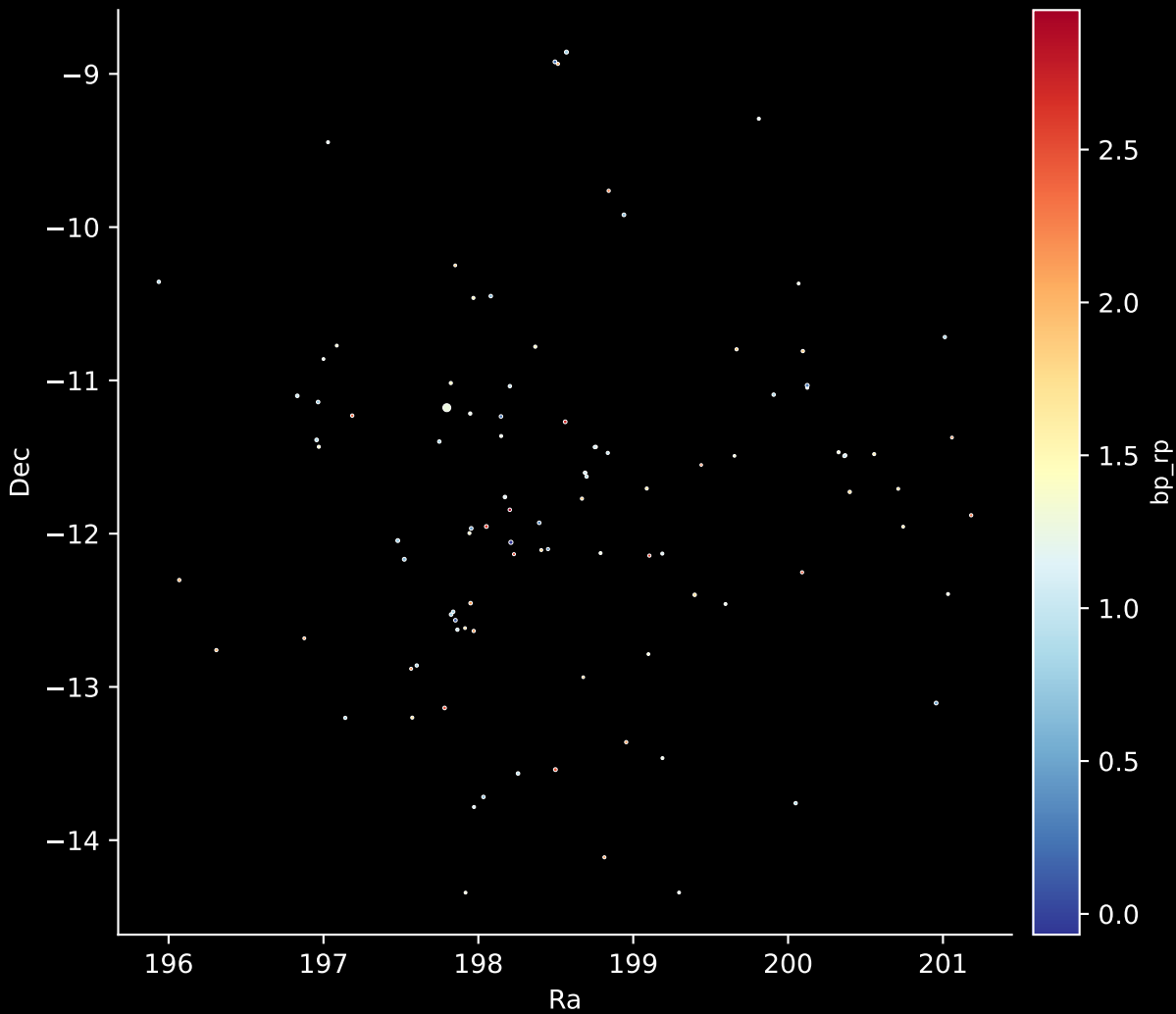
Gaia Cluster: [UPK_442] Stars: 101
