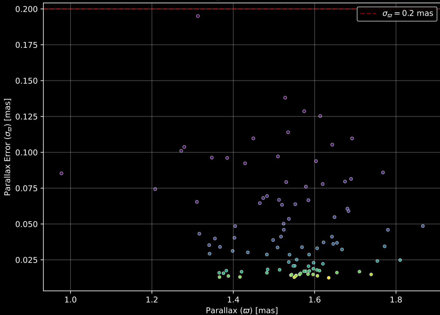
Gaia Cluster: [UPK_442] Parallax Quality (n= 101)
