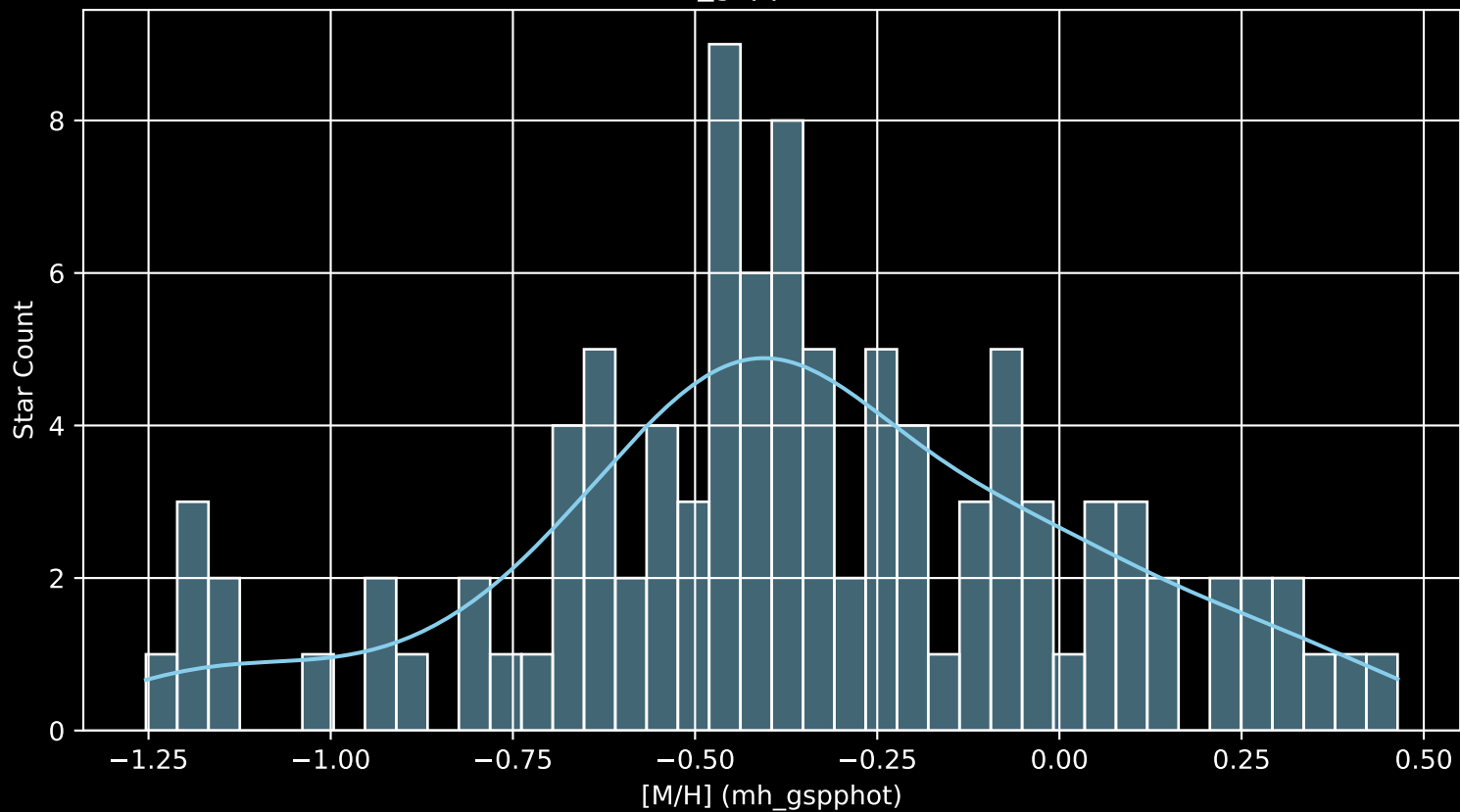
Gaia Cluster: [UPK_442 [M/H] (mh_gspphot) (n= 101)
