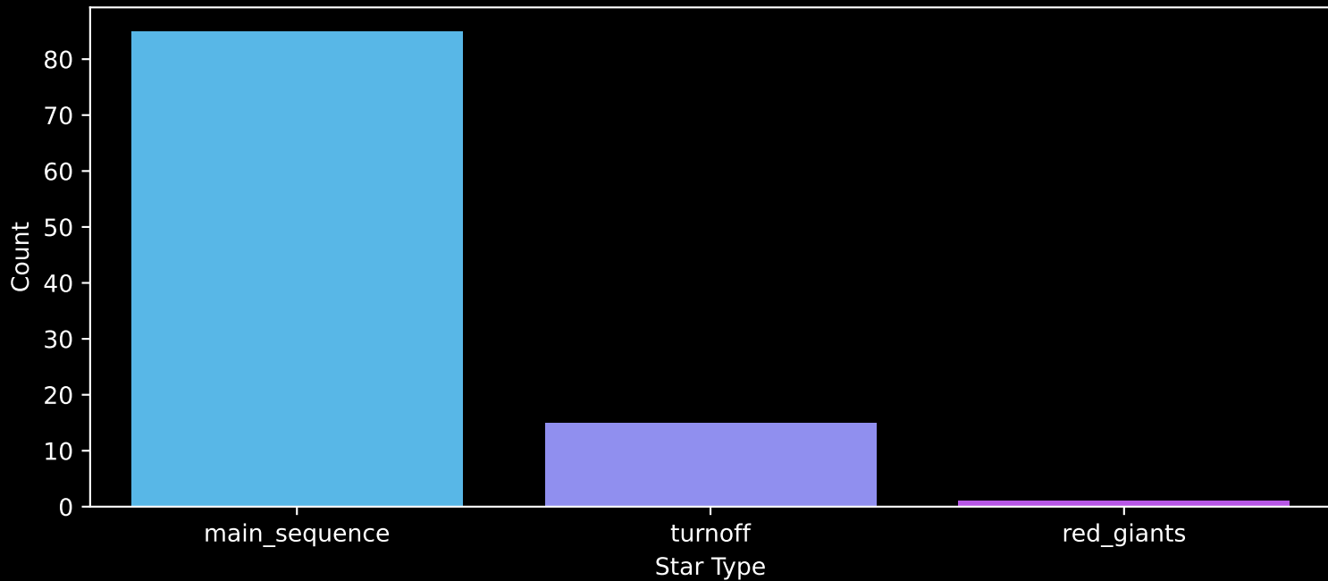
Gaia Cluster: [UPK_442] Count plot of Star Type
