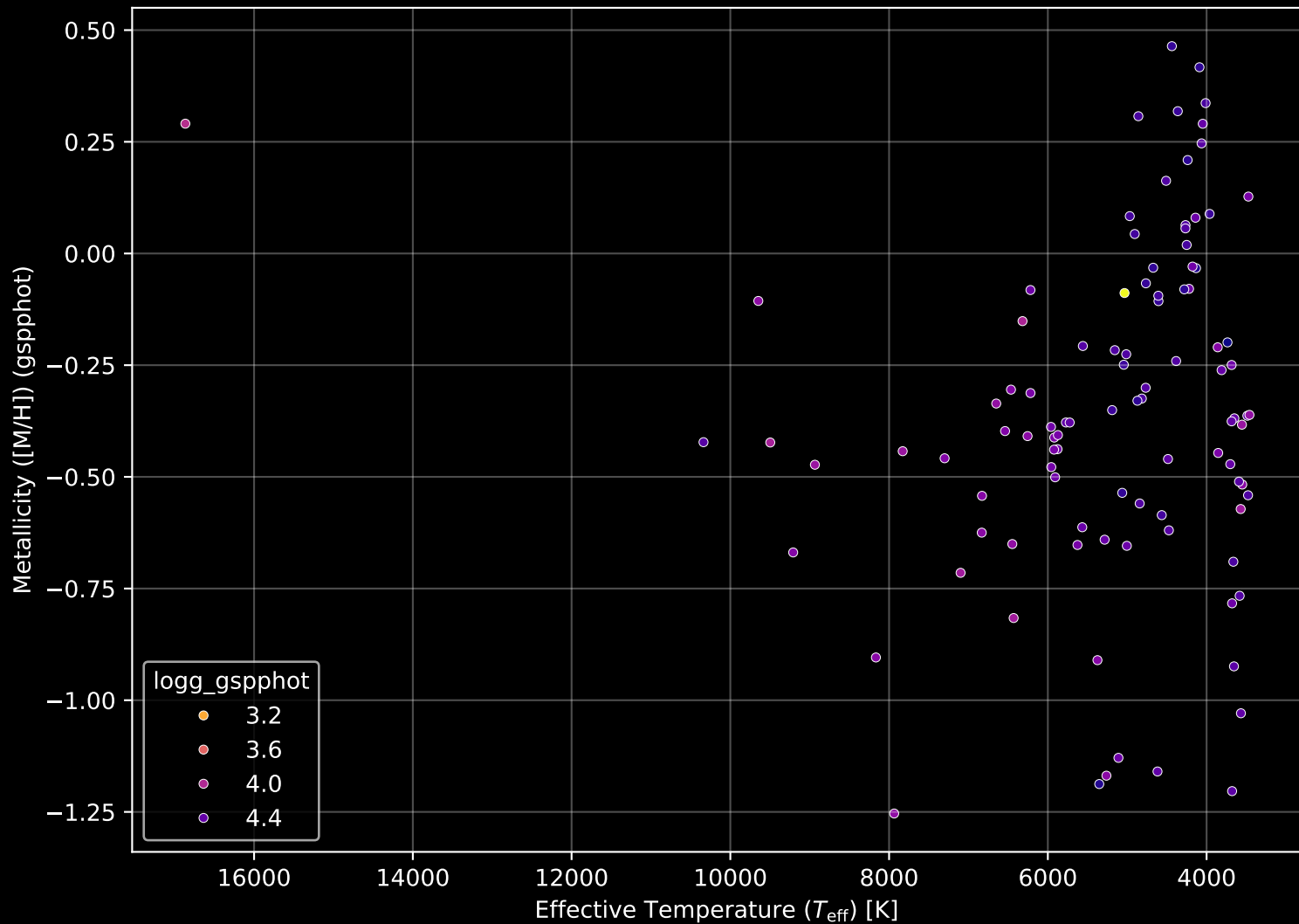
Gaia Cluster: [UPK_442] Stellar Population Parameters (n= 101)
