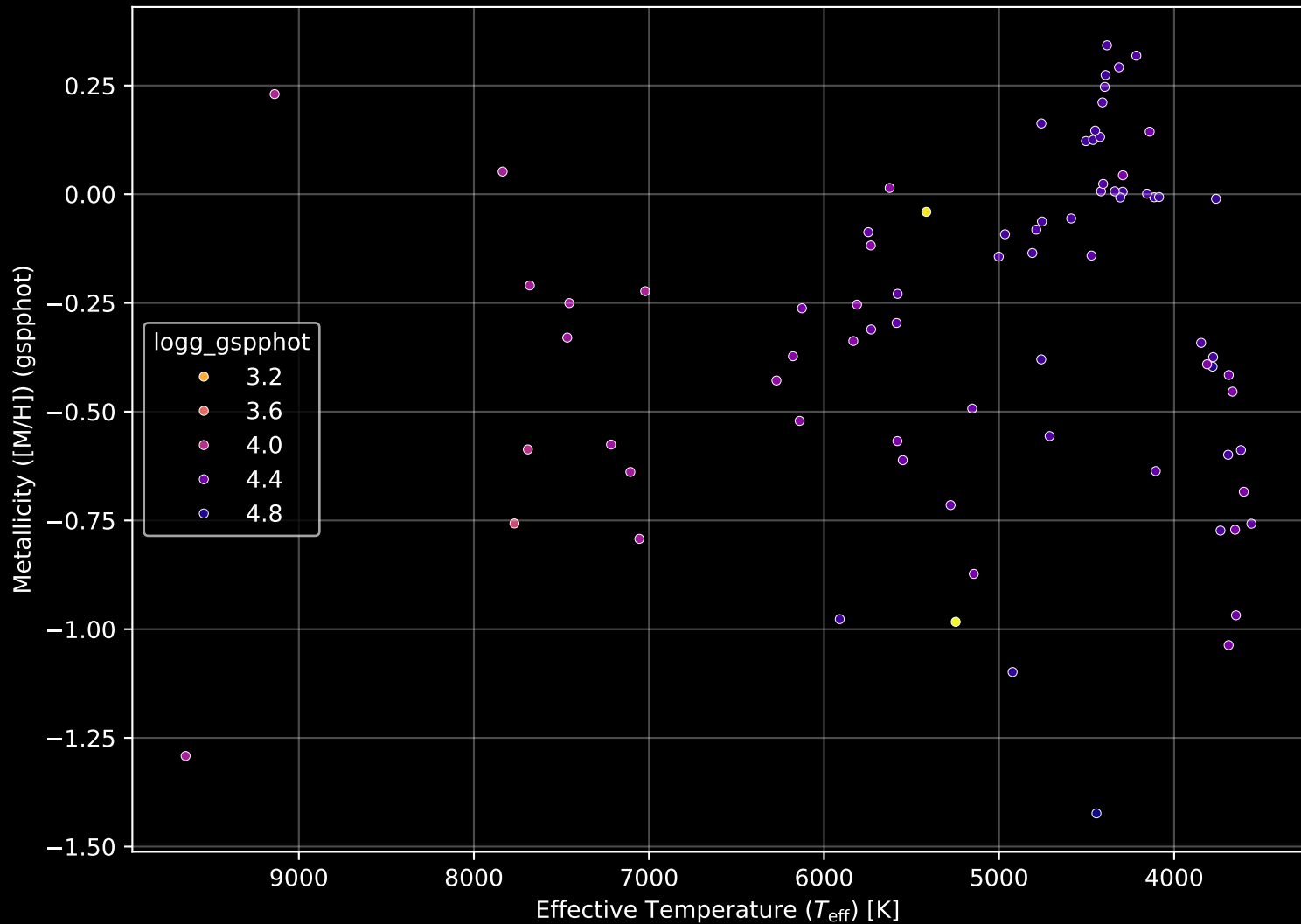
Gaia Cluster: [UPK_495] Stellar Population Parameters (n= 80)
