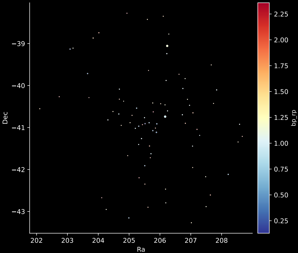
Gaia Cluster: [UPK_495] Stars: 80
