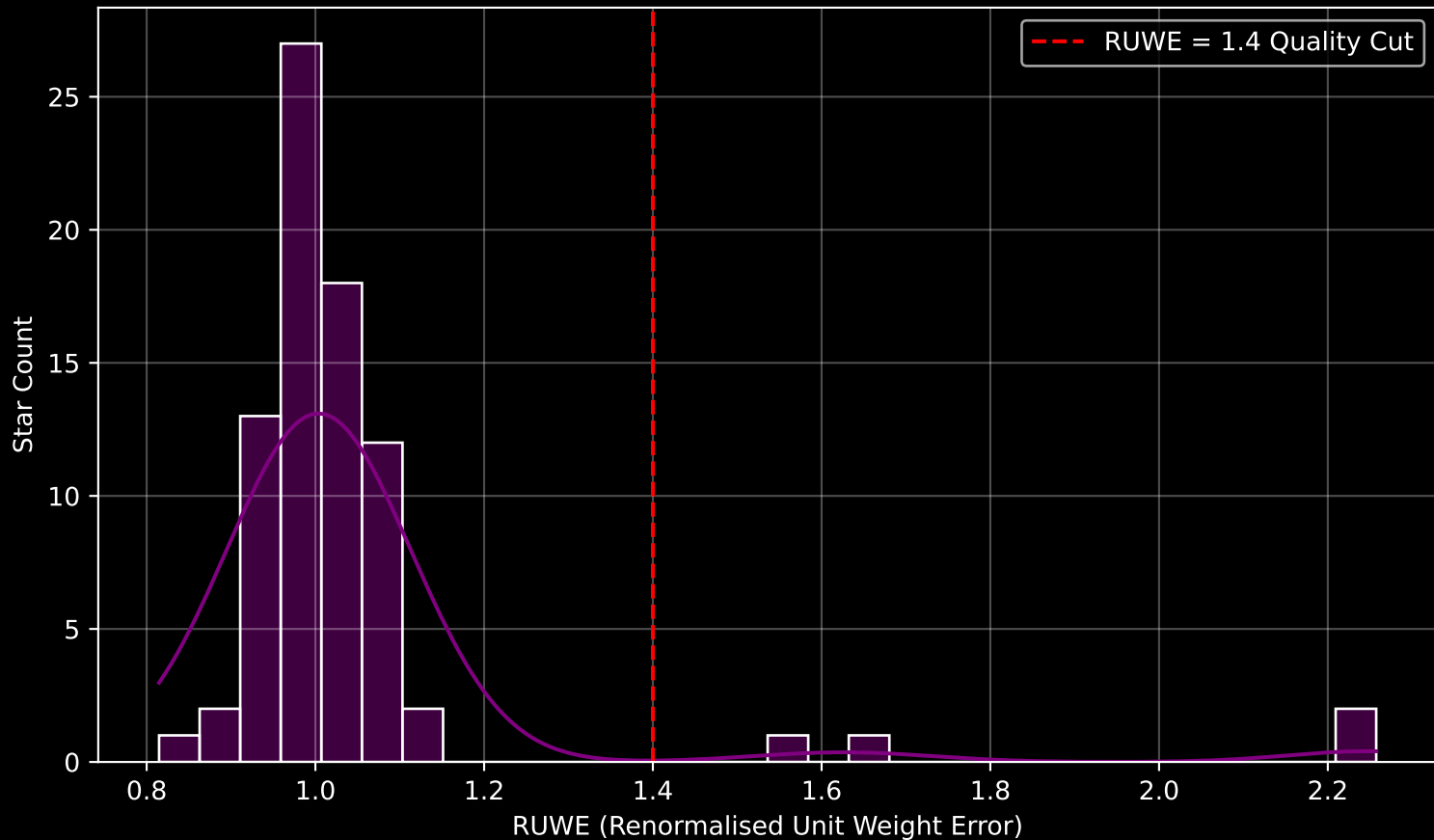
Gaia Cluster: [UPK_495] RUWE Distribution (n= 79)
