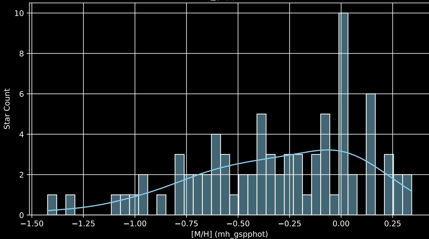
Gaia Cluster: [UPK_495 [M/H] (mh_gspphot) (n= 80)
