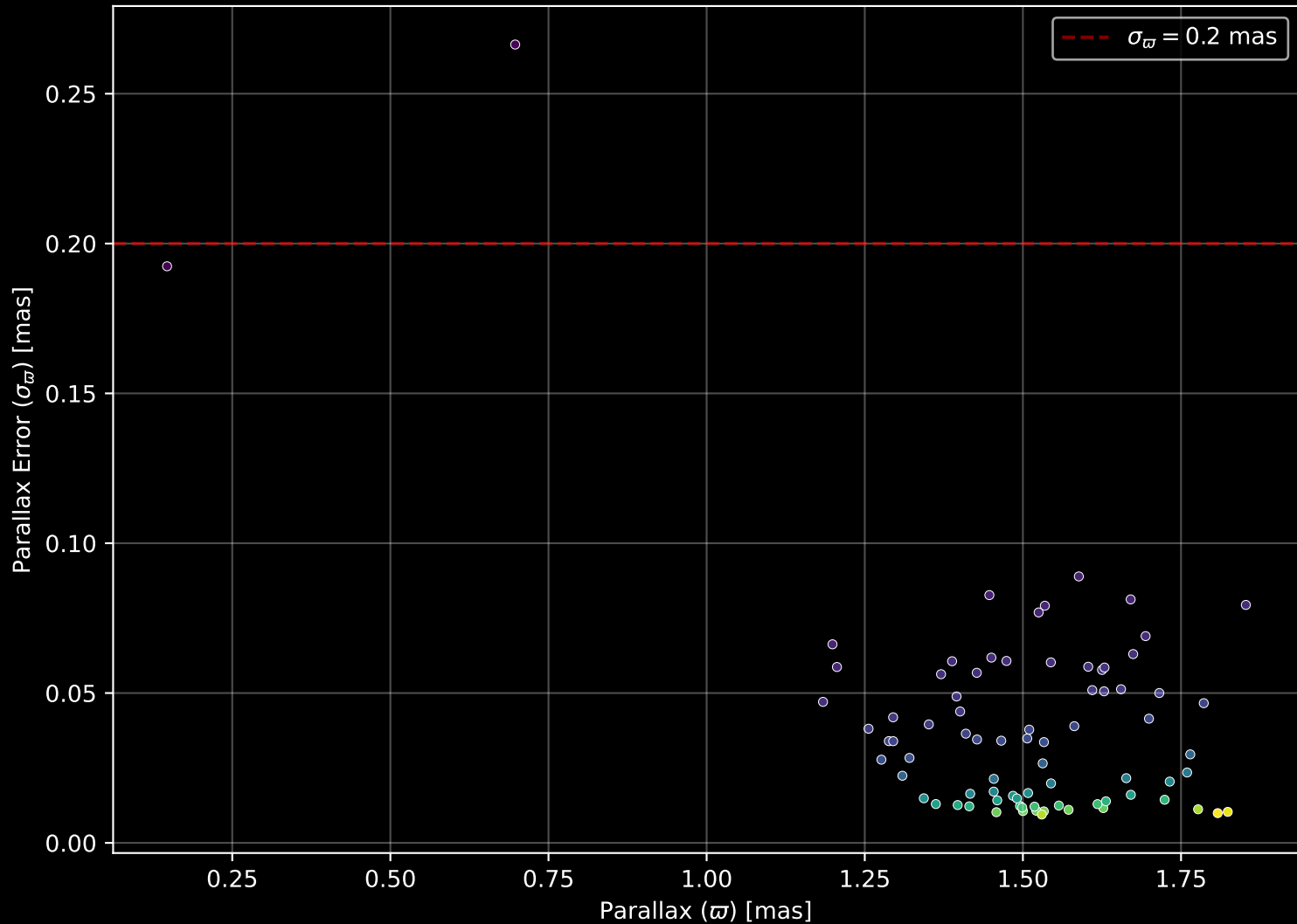
Gaia Cluster: [UPK_495] Parallax Quality (n= 80)
