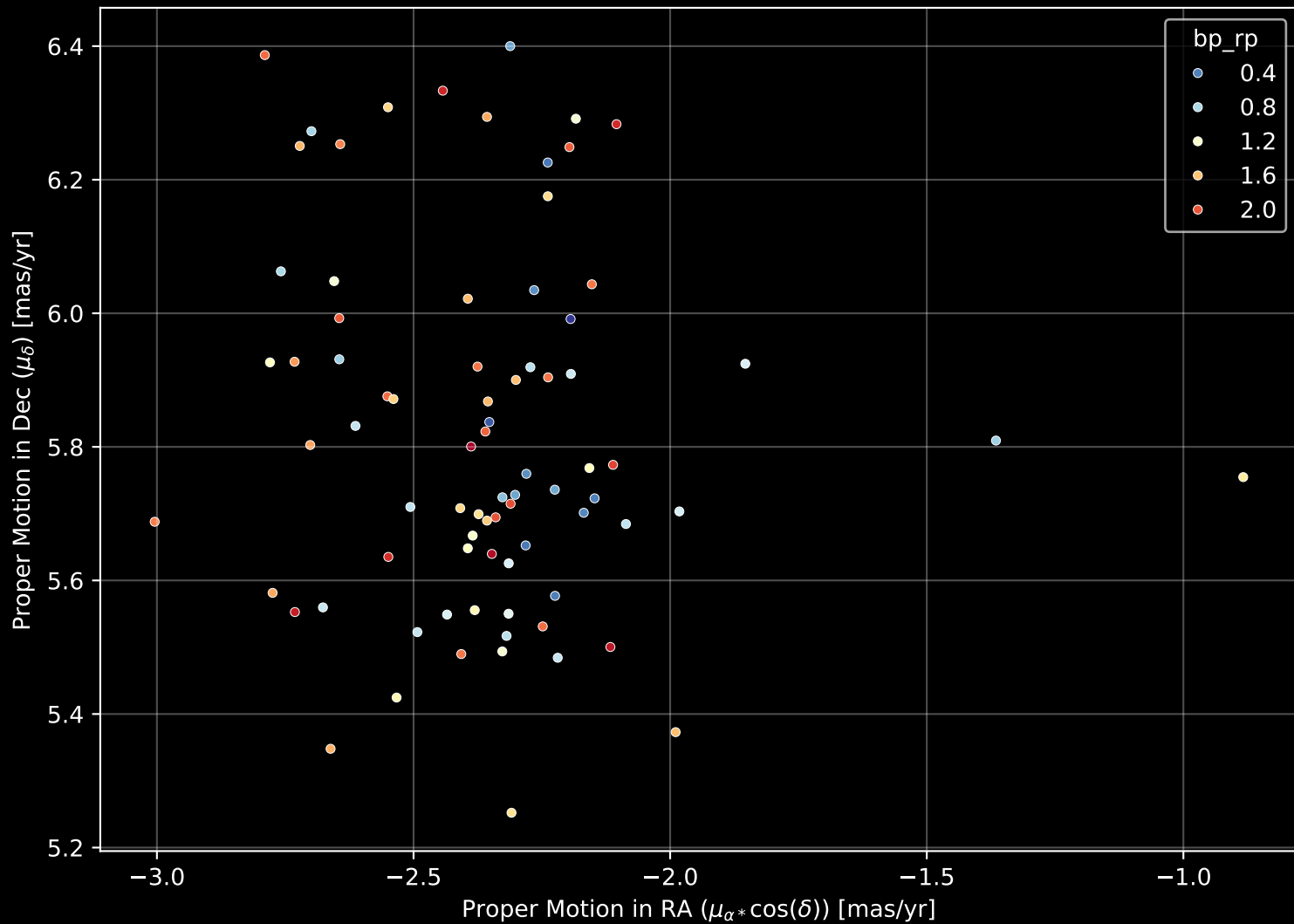
Gaia Cluster: [UPK_495] Proper Motion Diagram (n= 80)
