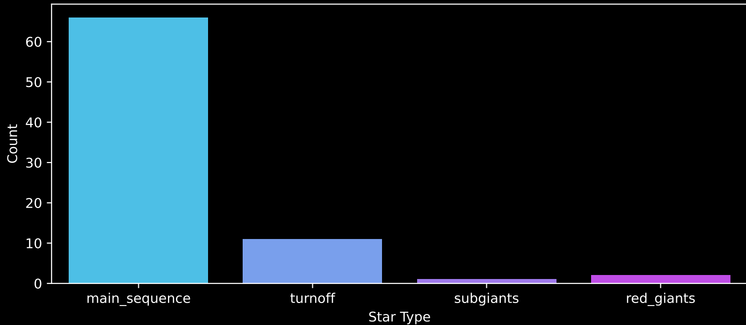
Gaia Cluster: [UPK_495] Count plot of Star Type
