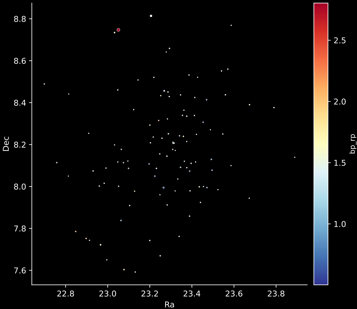
Gaia Cluster: [UPK_50] Stars: 105
