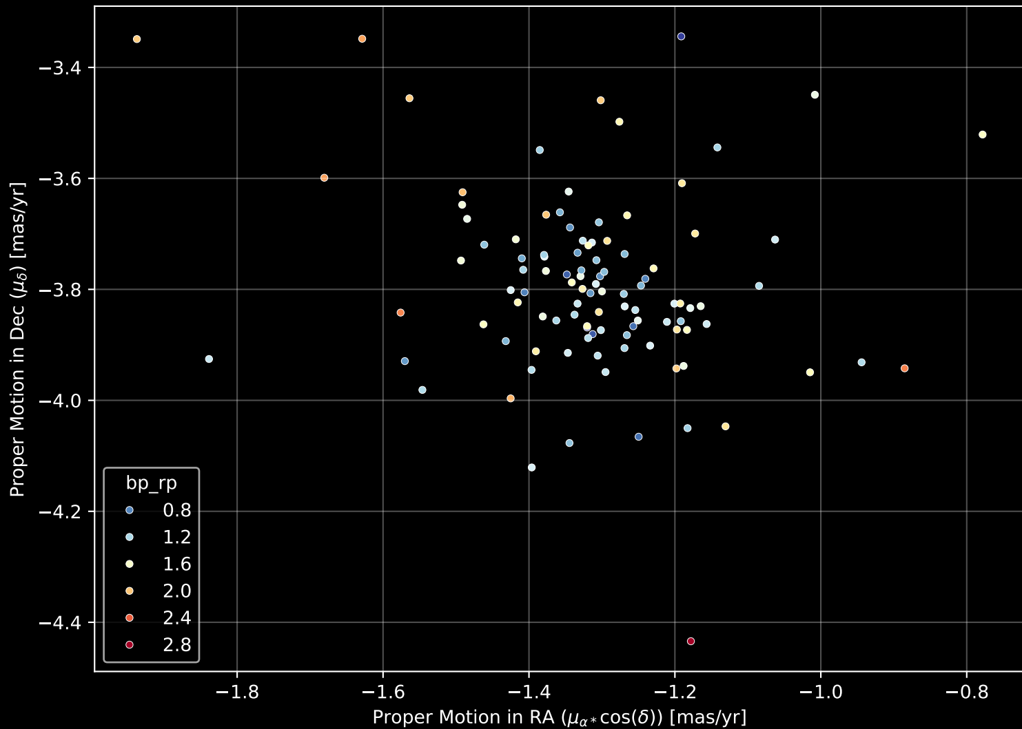
Gaia Cluster: [UPK_50] Proper Motion Diagram (n= 105)
