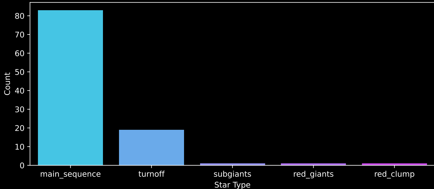
Gaia Cluster: [UPK_50] Count plot of Star Type
