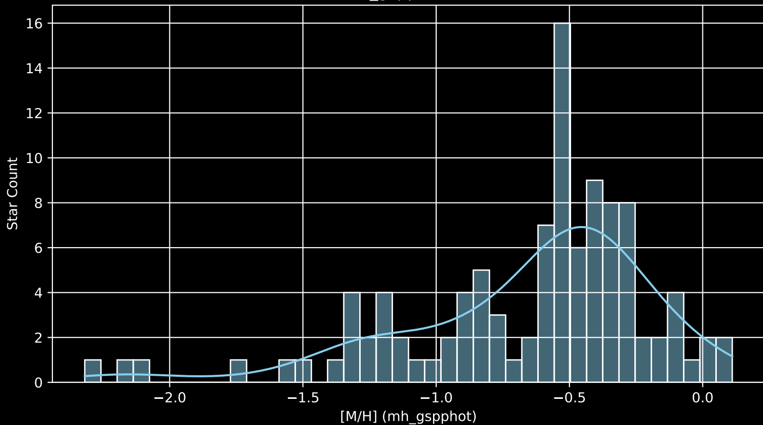
Gaia Cluster: [UPK_50 [M/H] (mh_gspphot) (n= 105)
