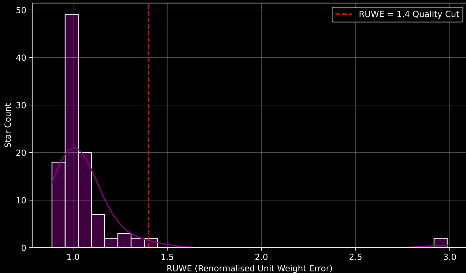
Gaia Cluster: [UPK_50] RUWE Distribution (n= 105)
