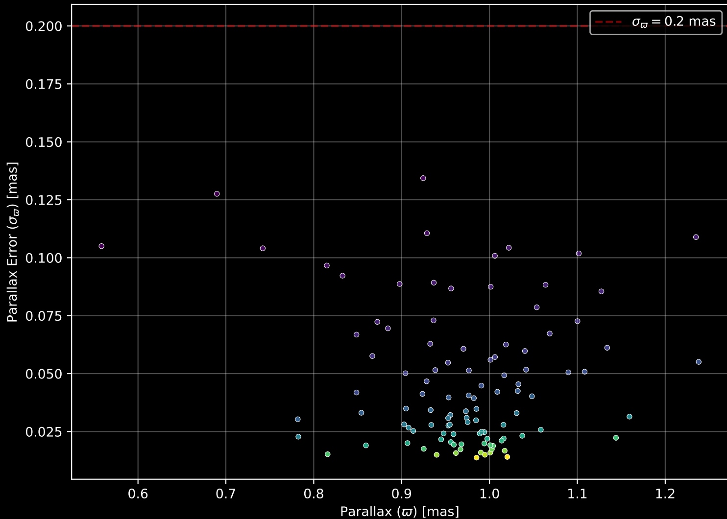
Gaia Cluster: [UPK_50] Parallax Quality (n= 105)
