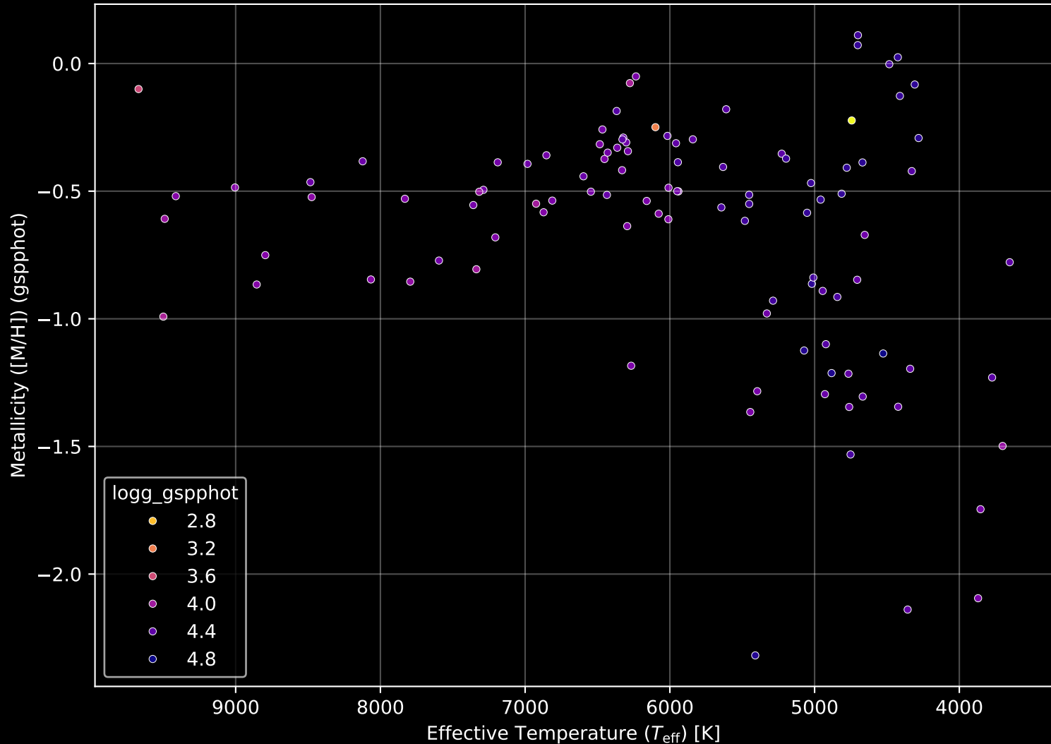
Gaia Cluster: [UPK_50] Stellar Population Parameters (n= 105)
