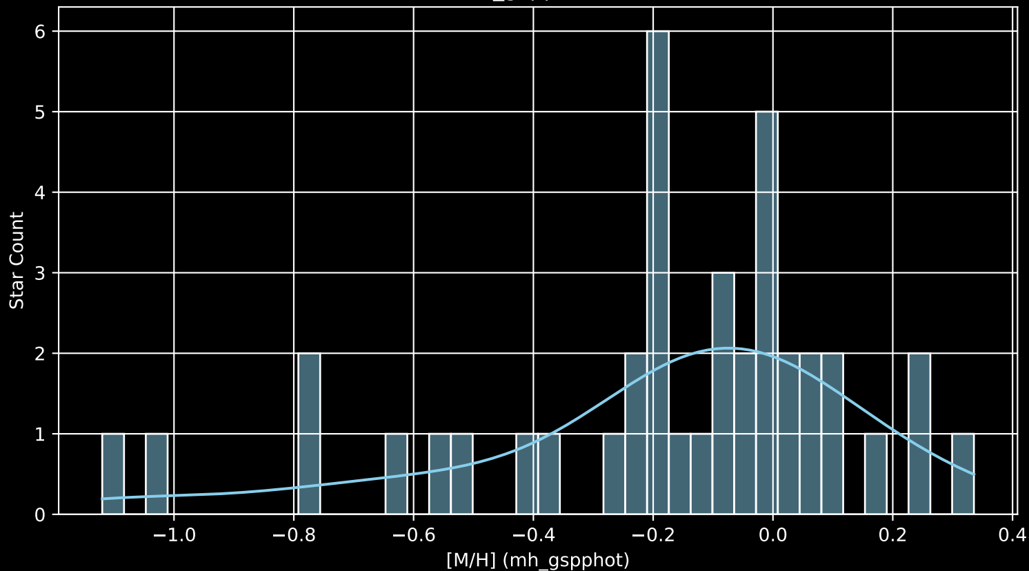
Gaia Cluster: [UPK_502 [M/H] (mh_gspphot) (n= 40)
