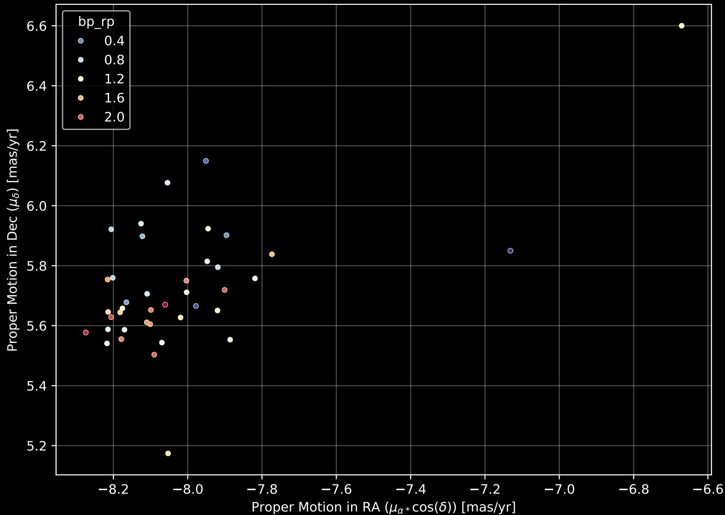
Gaia Cluster: [UPK_502] Proper Motion Diagram (n= 40)
