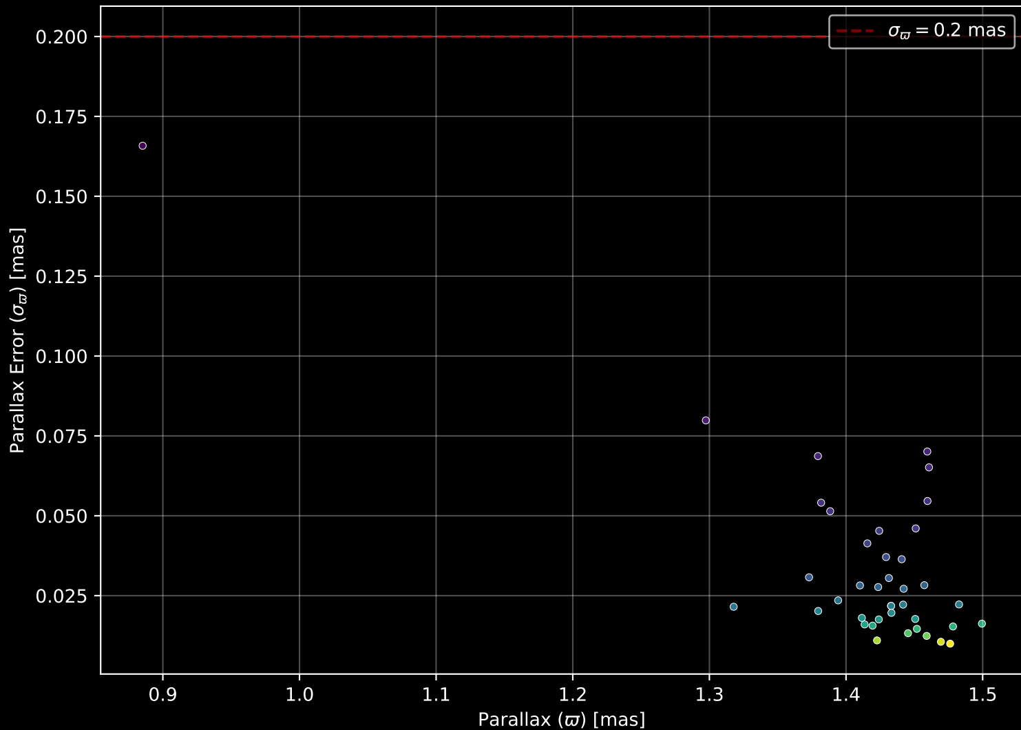
Gaia Cluster: [UPK_502] Parallax Quality (n= 40)
