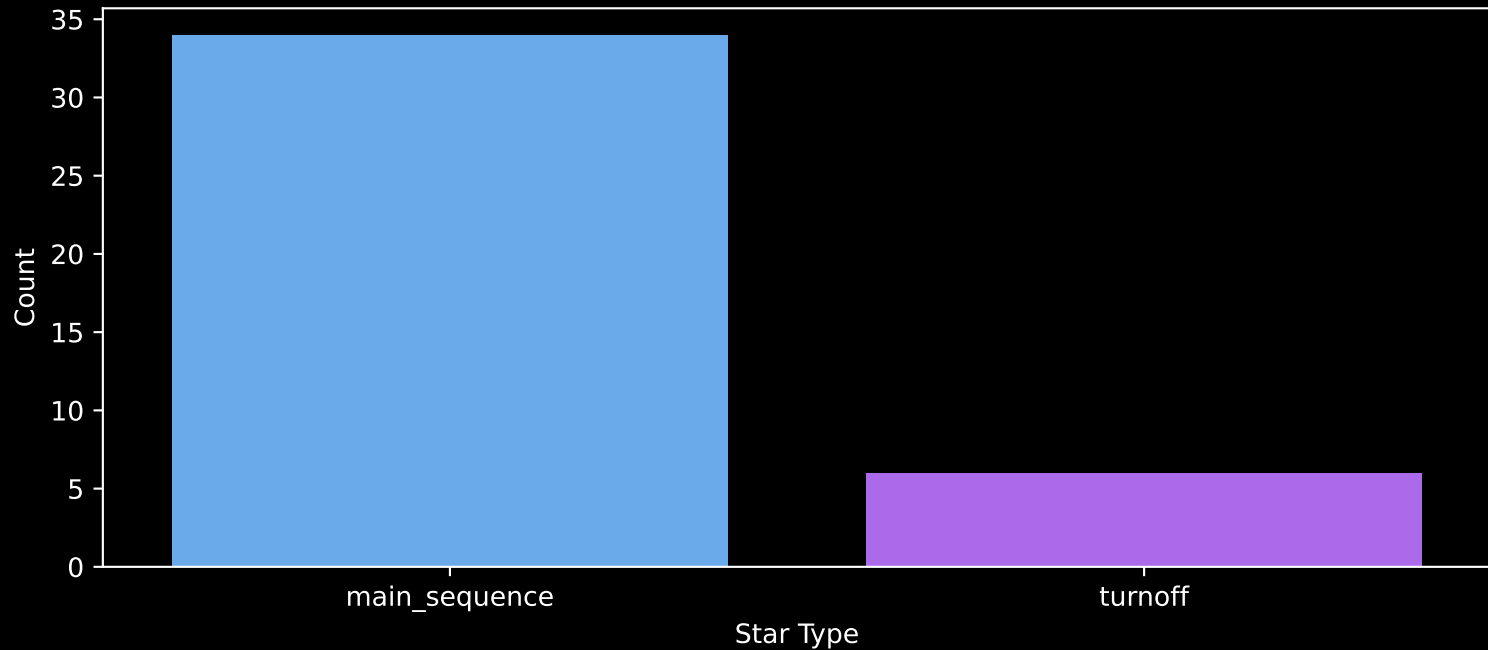
Gaia Cluster: [UPK_502] Count plot of Star Type
