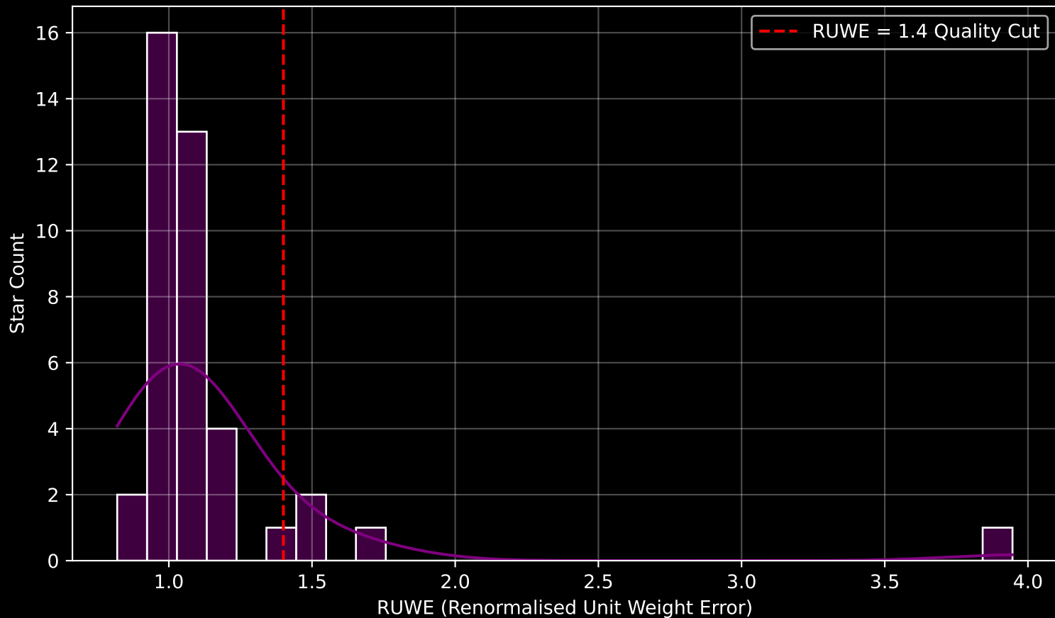
Gaia Cluster: [UPK_502] RUWE Distribution (n= 40)
