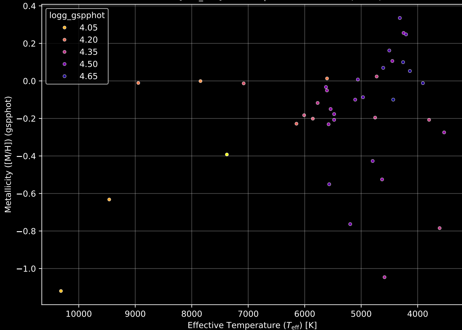
Gaia Cluster: [UPK_502] Stellar Population Parameters (n= 40)
