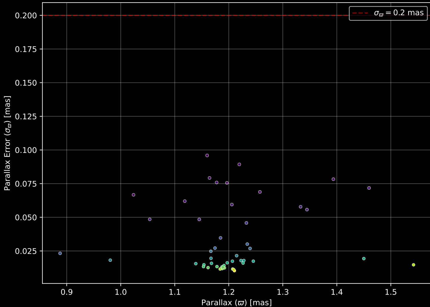
Gaia Cluster: [UPK_508] Parallax Quality (n= 48)
