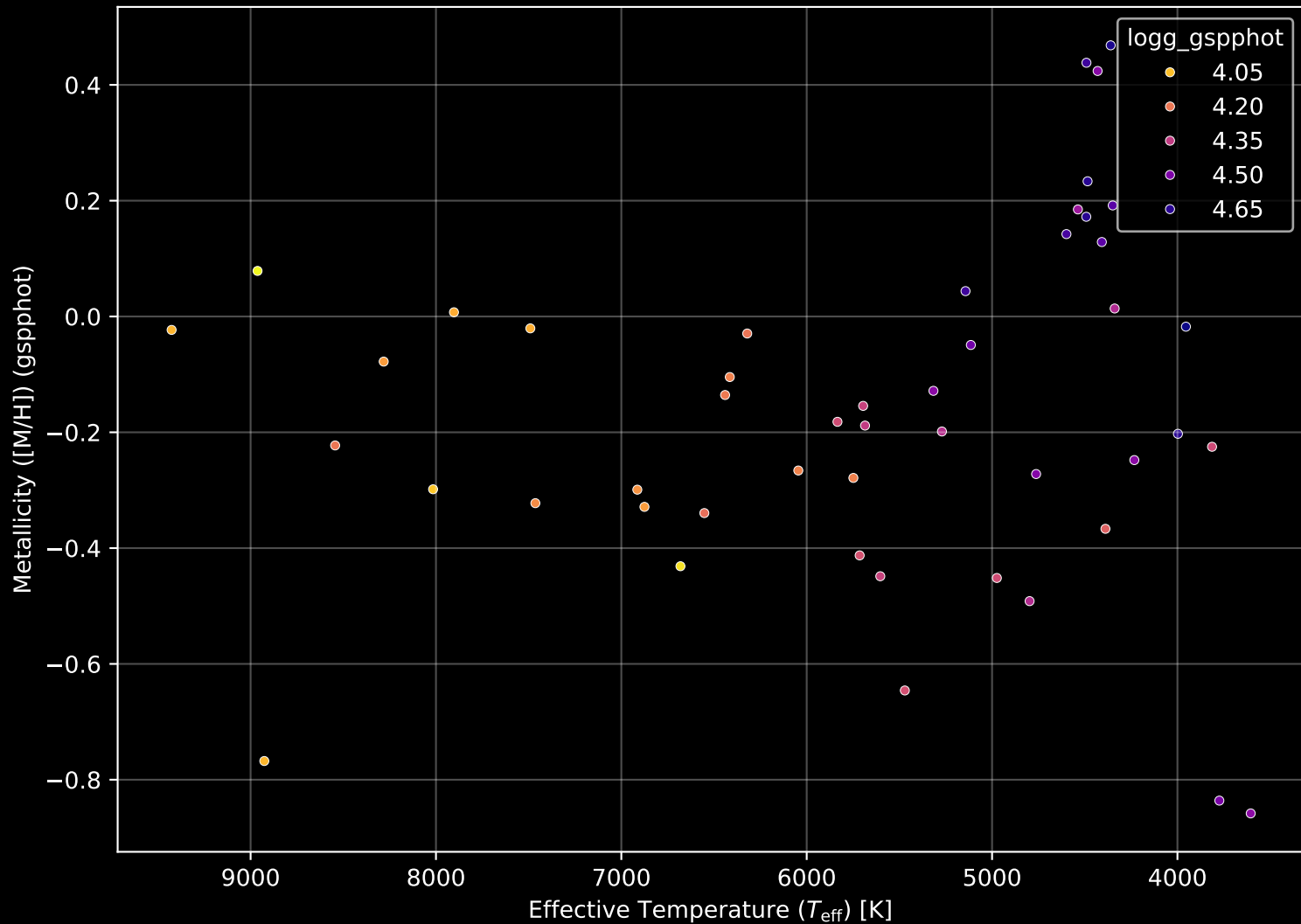
Gaia Cluster: [UPK_508] Stellar Population Parameters (n= 48)
