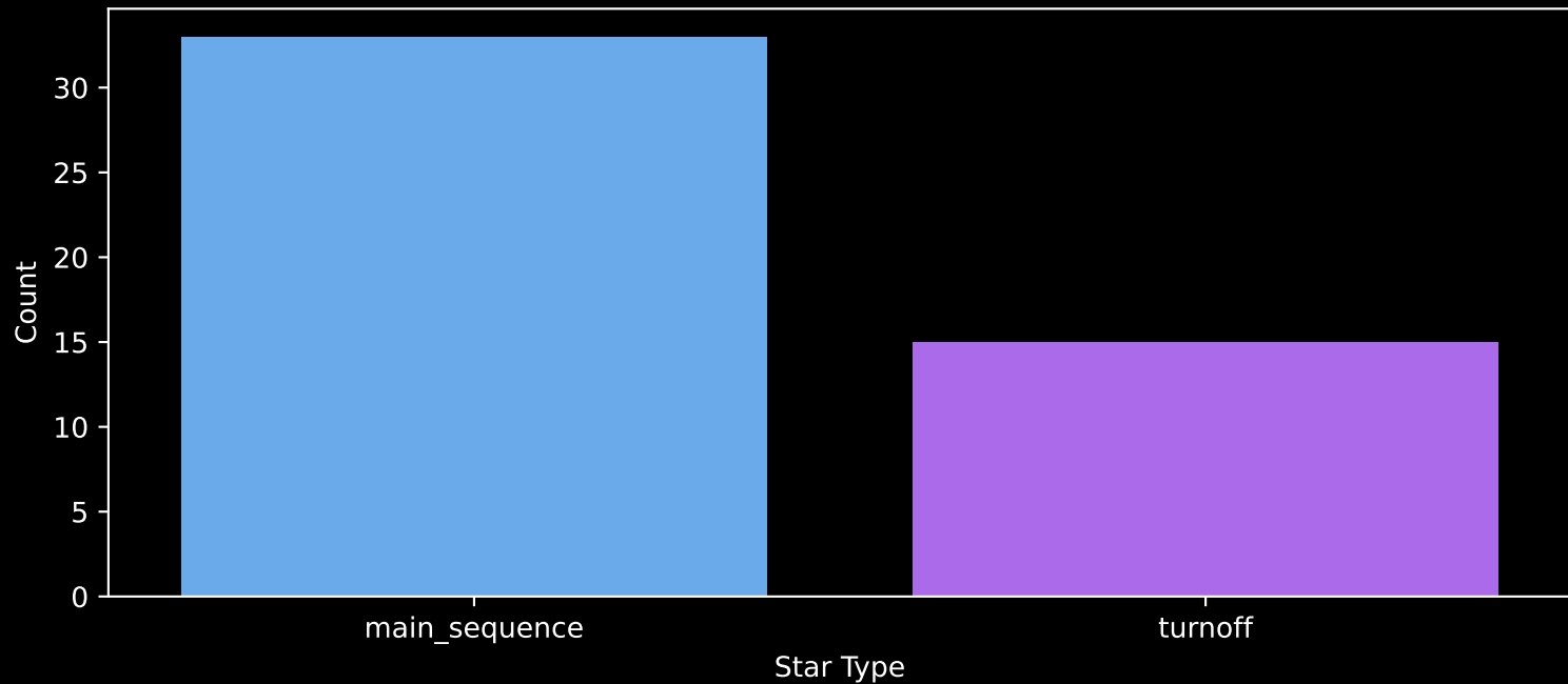
Gaia Cluster: [UPK_508] Count plot of Star Type
