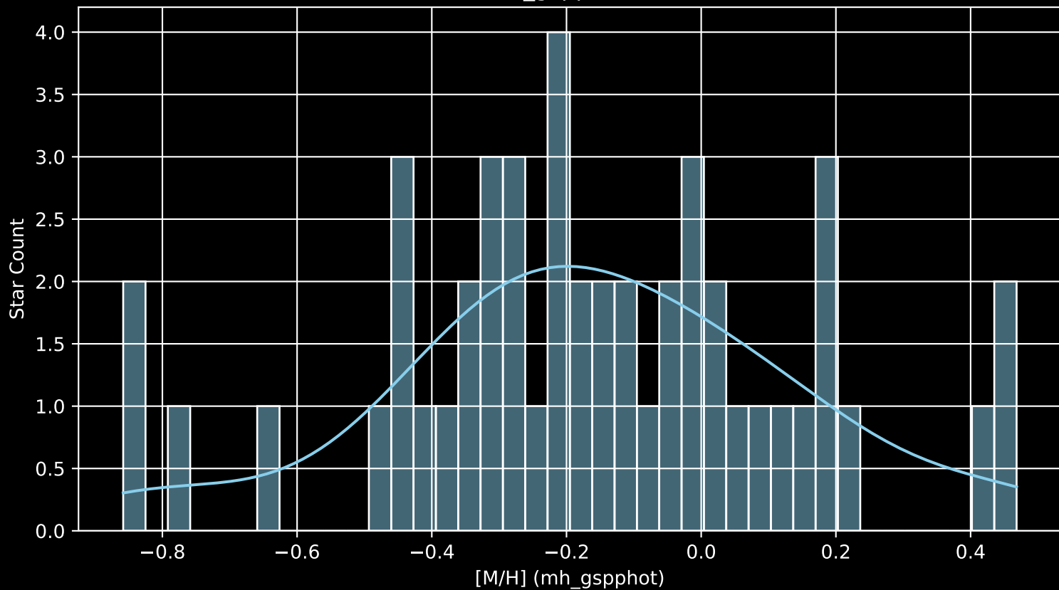
Gaia Cluster: [UPK_508 [M/H] (mh_gspphot) (n= 48)
