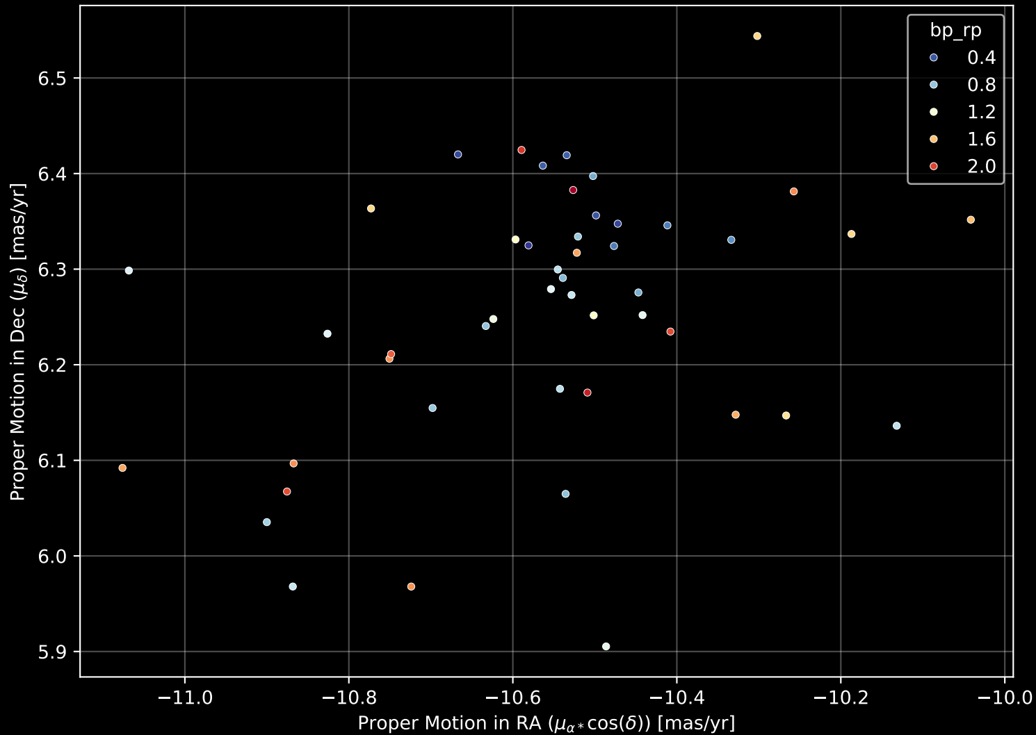
Gaia Cluster: [UPK_508] Proper Motion Diagram (n= 48)
