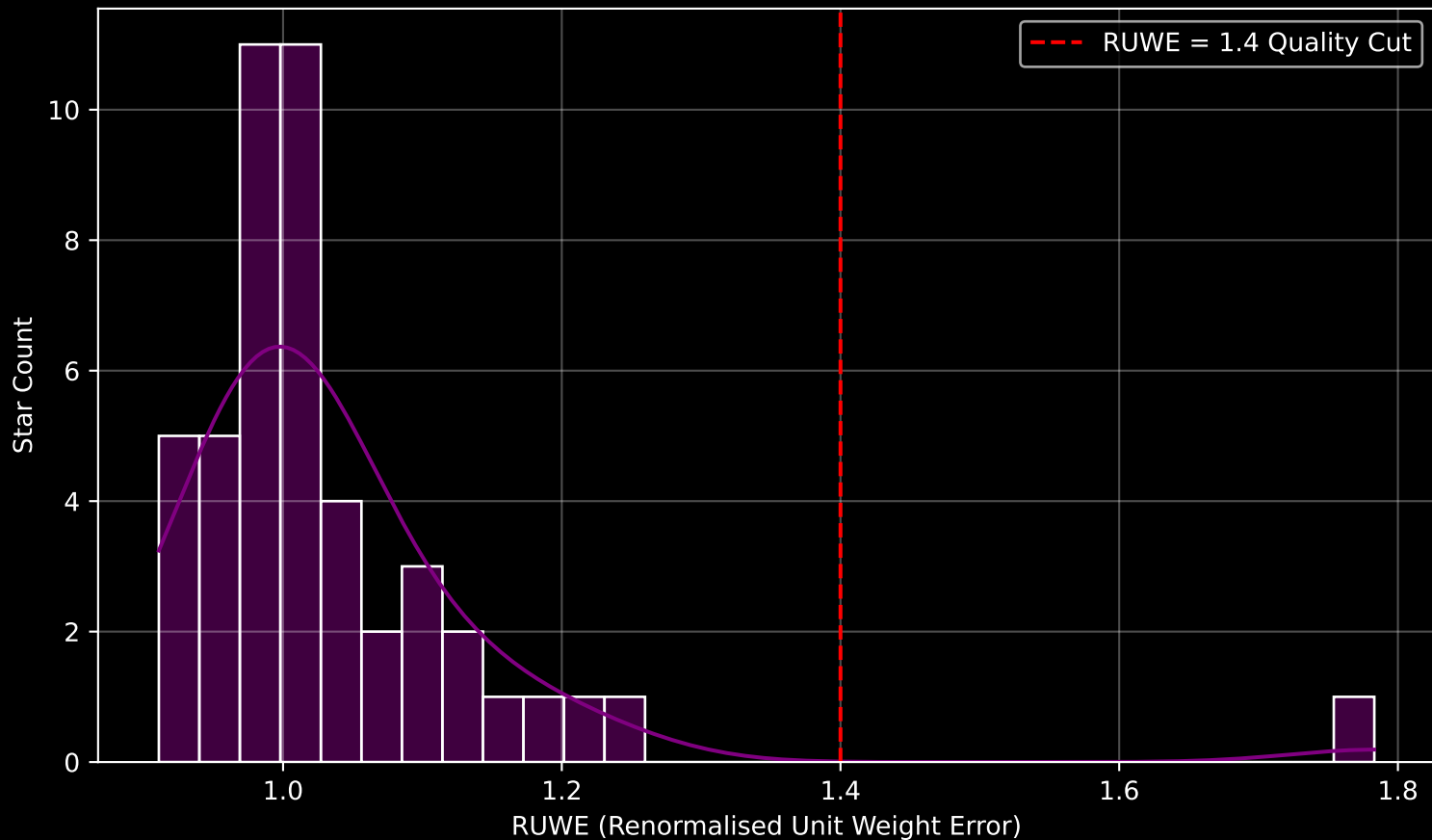
Gaia Cluster: [UPK_508] RUWE Distribution (n= 48)
