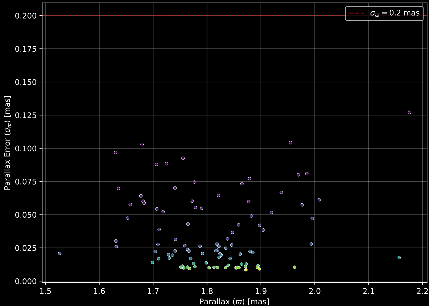
Gaia Cluster: [UPK_524] Parallax Quality (n= 97)
