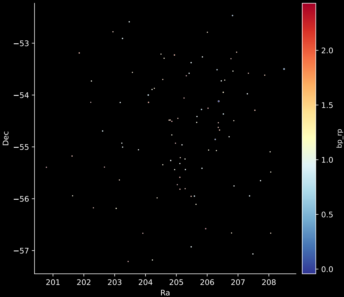
Gaia Cluster: [UPK_524] Stars: 97
