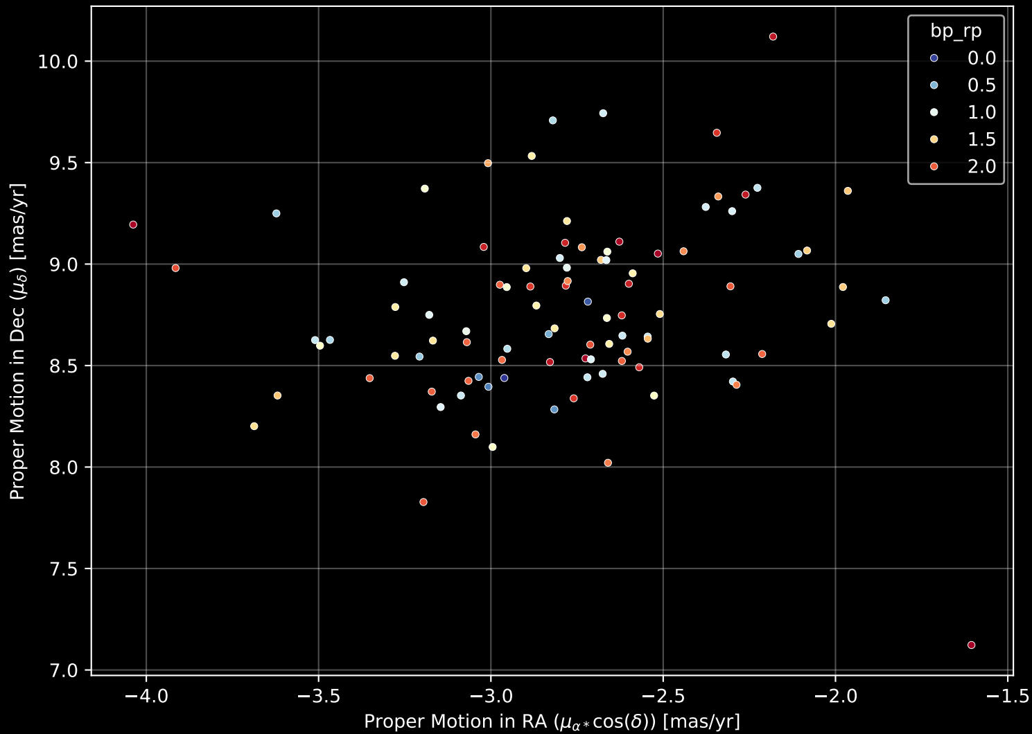
Gaia Cluster: [UPK_524] Proper Motion Diagram (n= 97)
