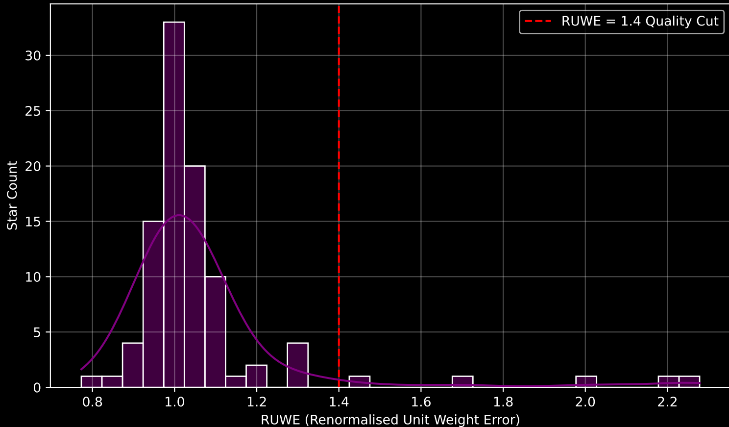
Gaia Cluster: [UPK_524] RUWE Distribution (n= 96)
