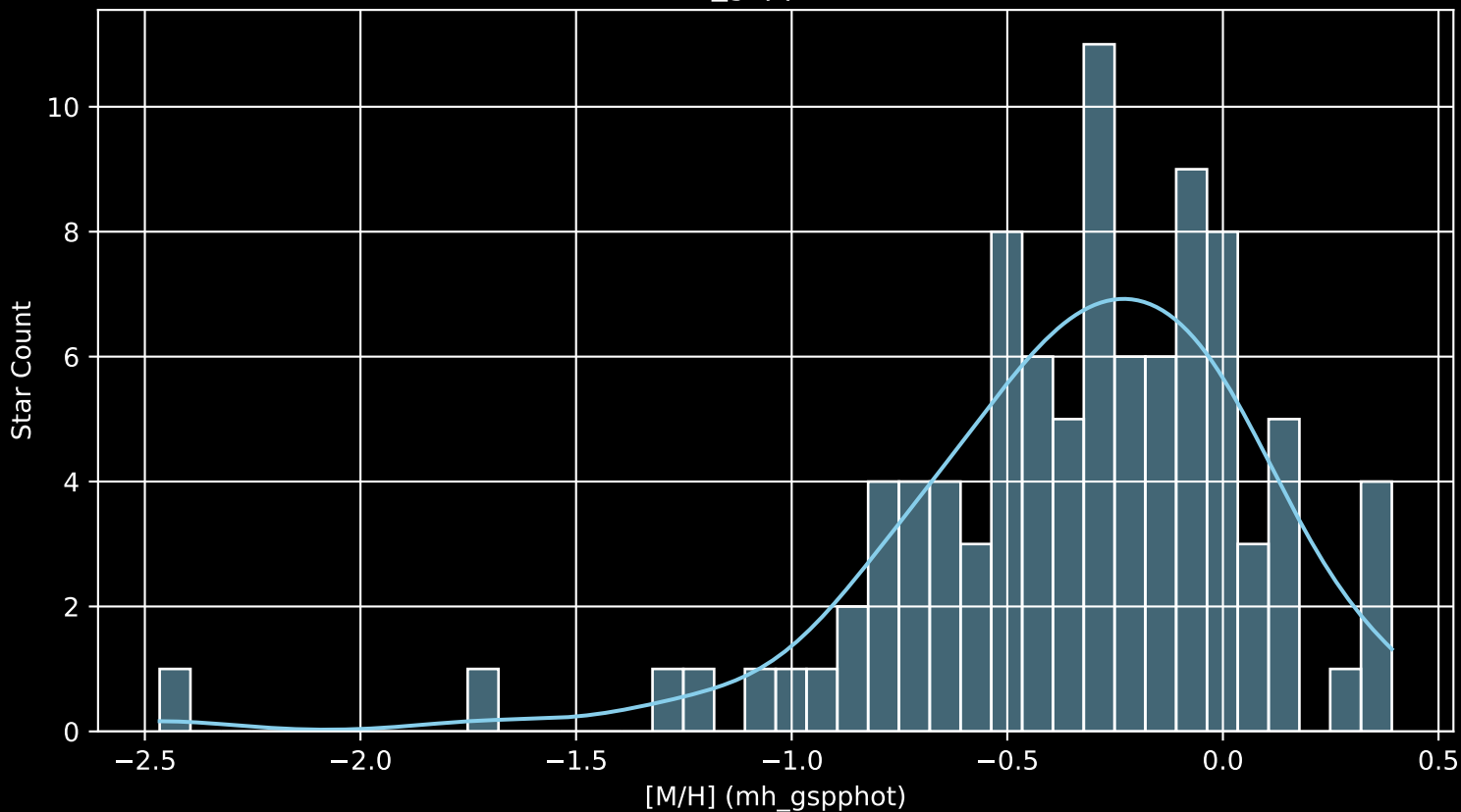
Gaia Cluster: [UPK_524 [M/H] (mh_gspphot) (n= 96)
