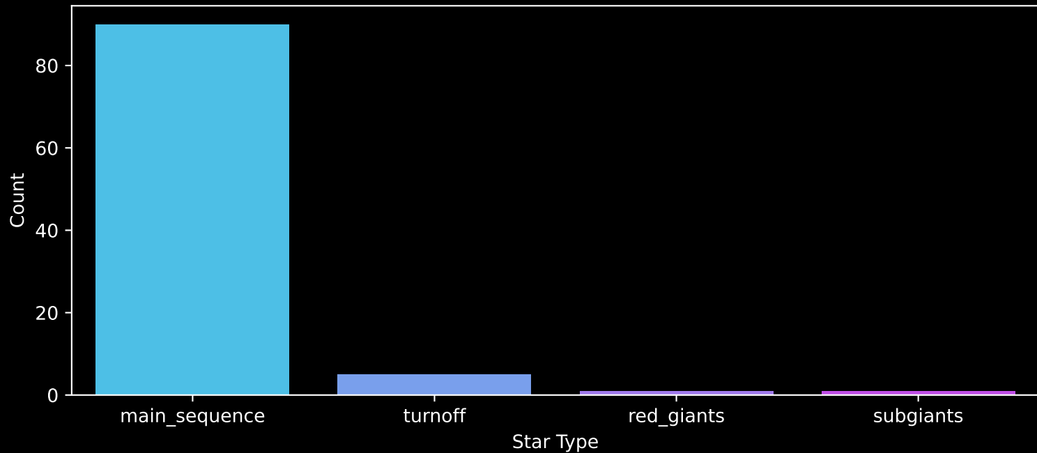
Gaia Cluster: [UPK_524] Count plot of Star Type
