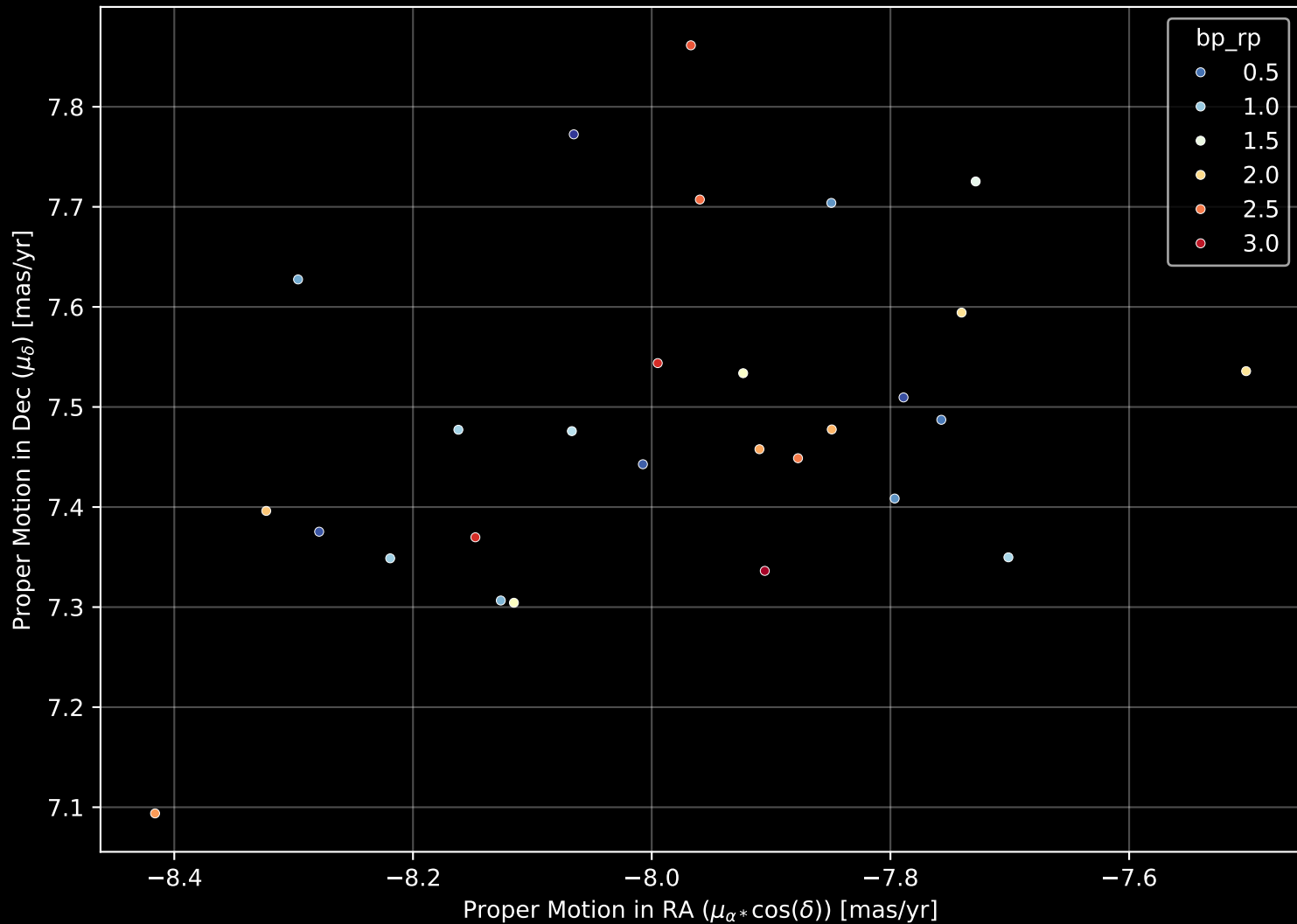
Gaia Cluster: [UPK_526] Proper Motion Diagram (n= 28)
