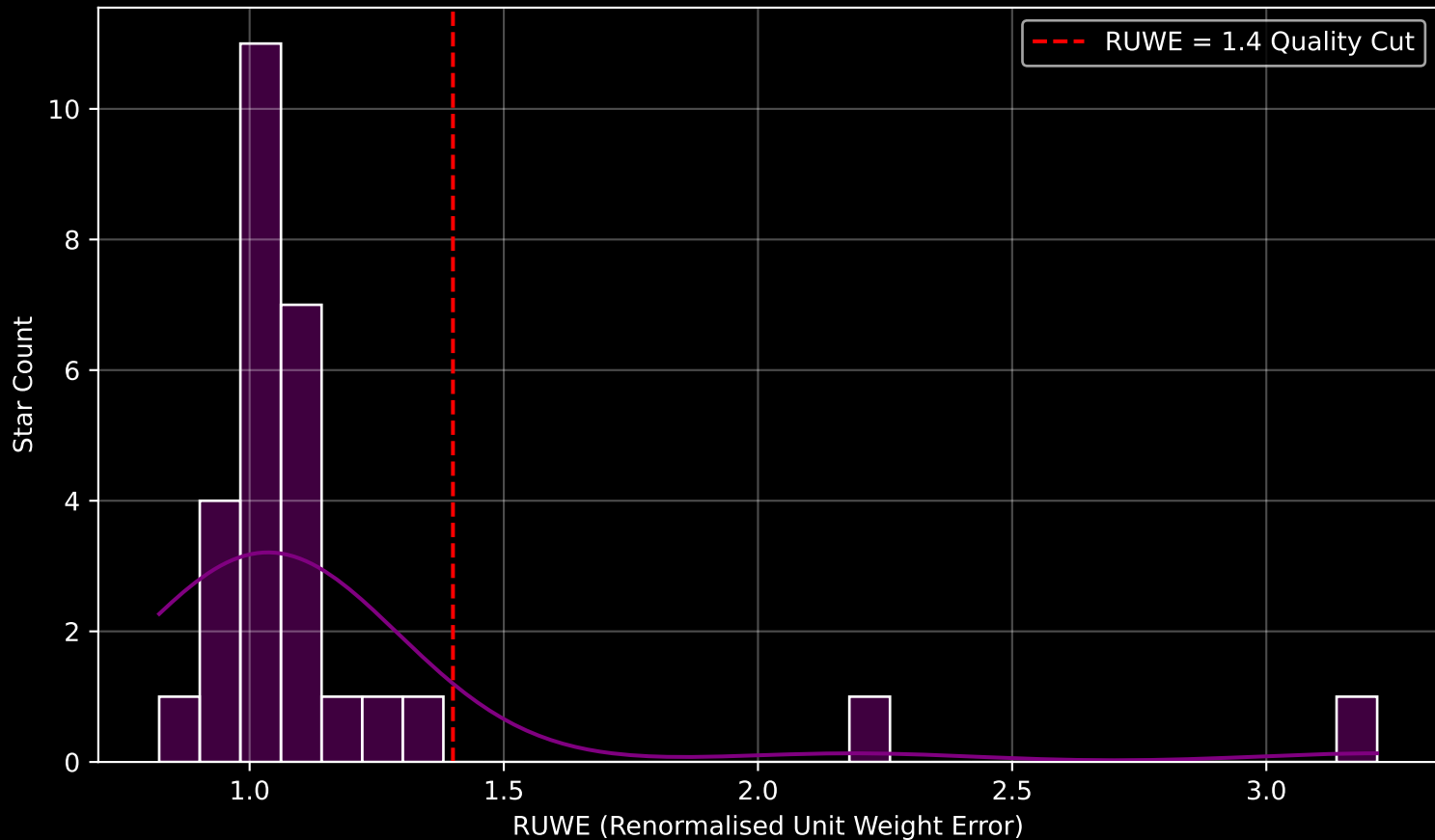
Gaia Cluster: [UPK_526] RUWE Distribution (n= 28)
