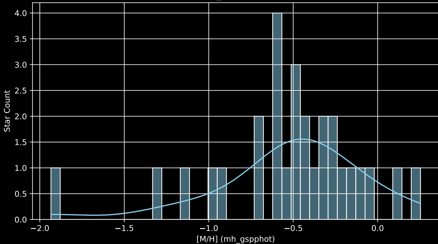
Gaia Cluster: [UPK_526 [M/H] (mh_gspphot) (n= 28)
