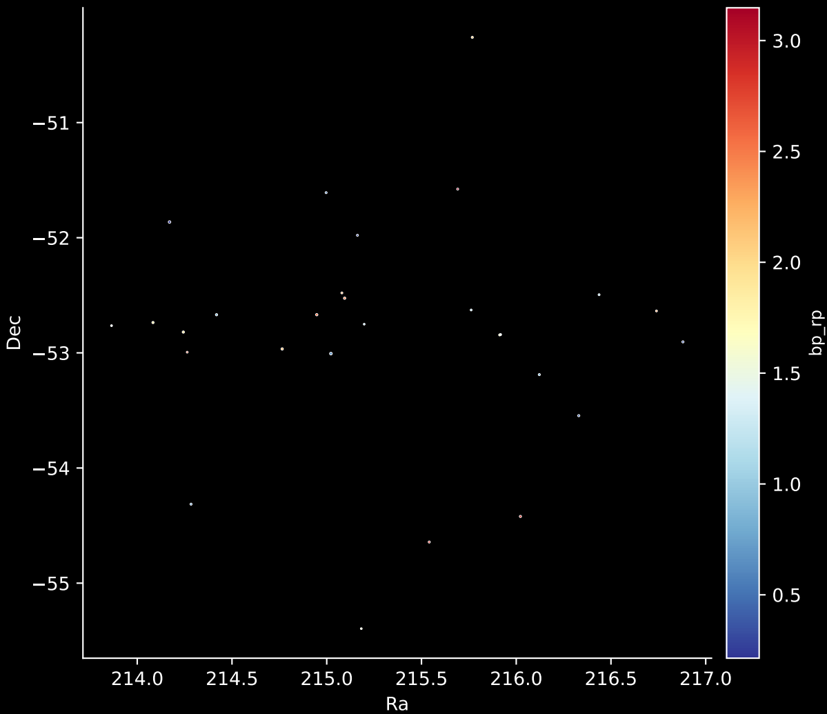
Gaia Cluster: [UPK_526] Stars: 28
