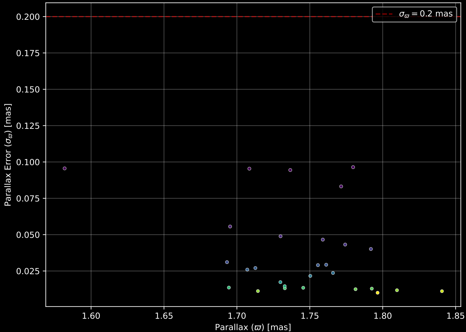
Gaia Cluster: [UPK_526] Parallax Quality (n= 28)
