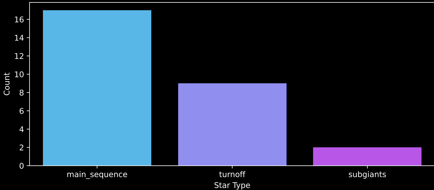
Gaia Cluster: [UPK_526] Count plot of Star Type
