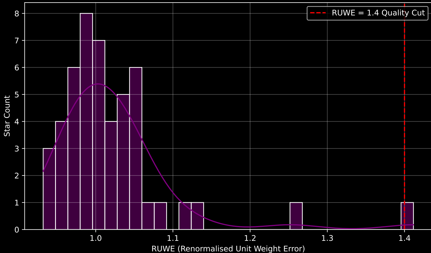
Gaia Cluster: [UPK_528] RUWE Distribution (n= 49)
