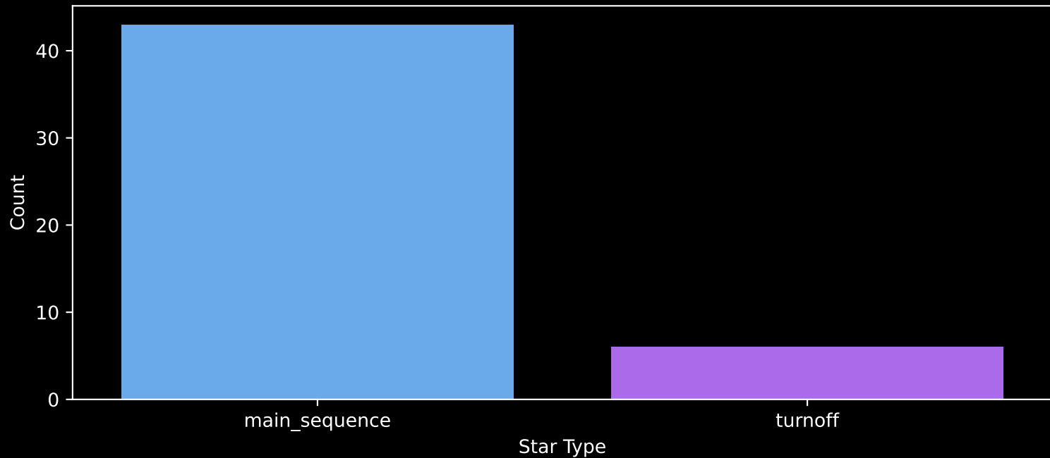
Gaia Cluster: [UPK_528] Count plot of Star Type
