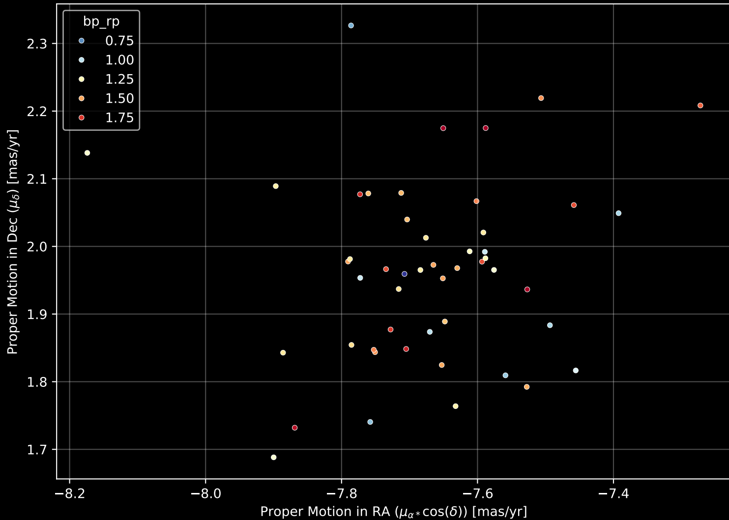
Gaia Cluster: [UPK_528] Proper Motion Diagram (n= 49)
