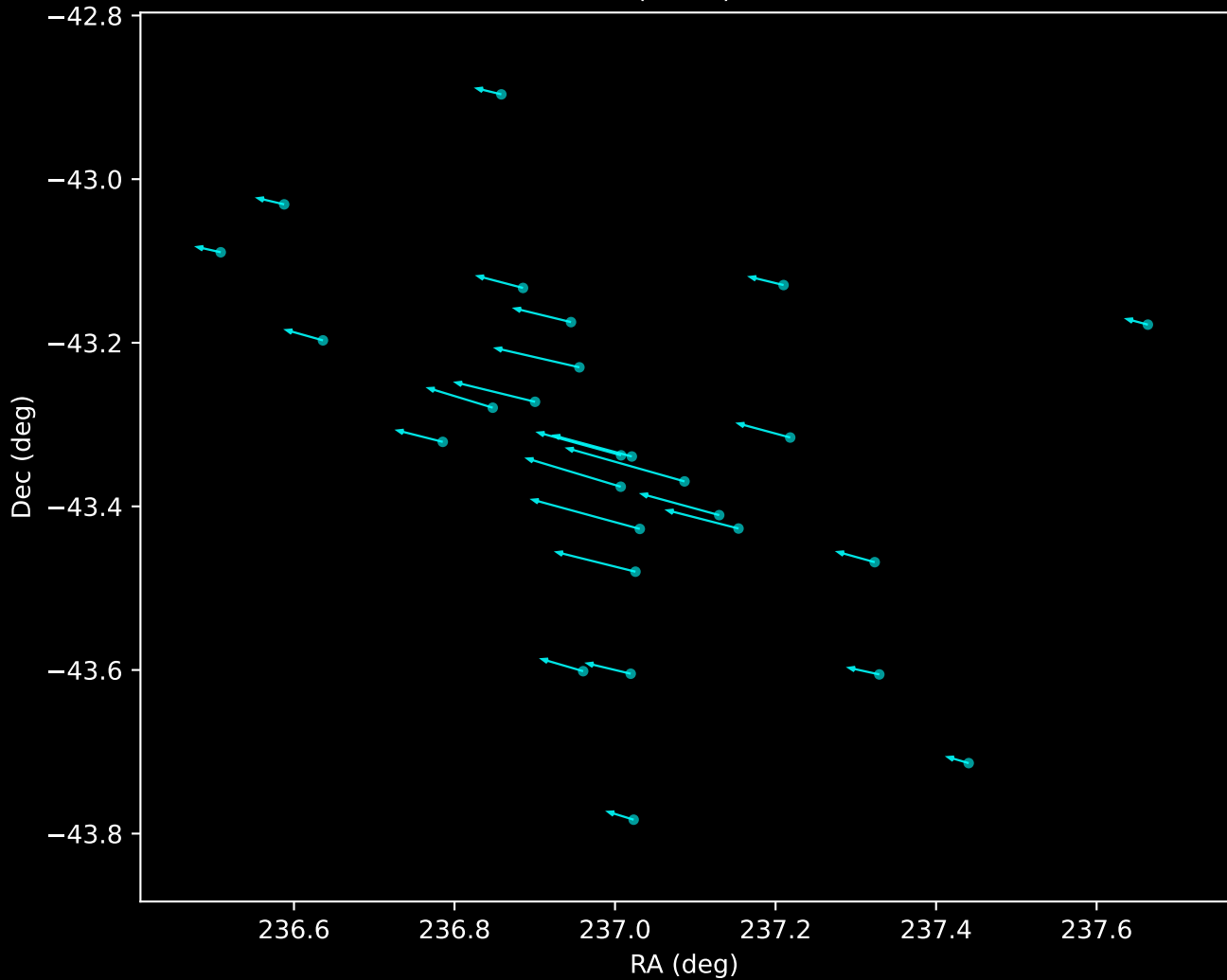
Gaia DR3 Noise Stream Proper Motion Vectors (n=27)
