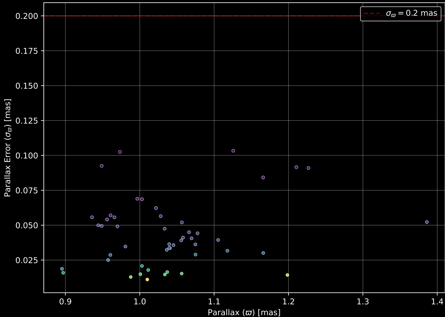
Gaia Cluster: [UPK_528] Parallax Quality (n= 49)
