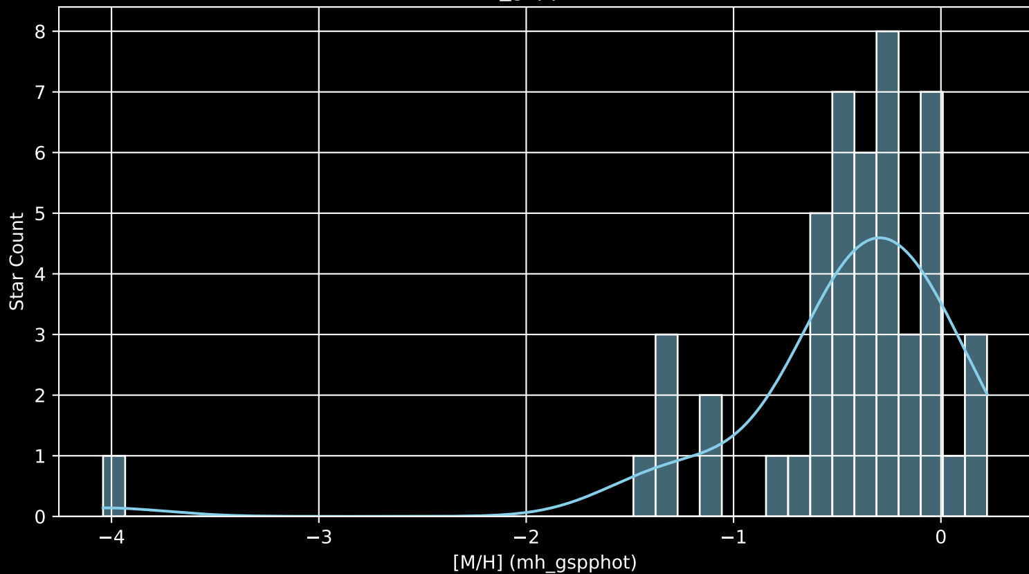
Gaia Cluster: [UPK_528 [M/H] (mh_gspphot) (n= 49)
