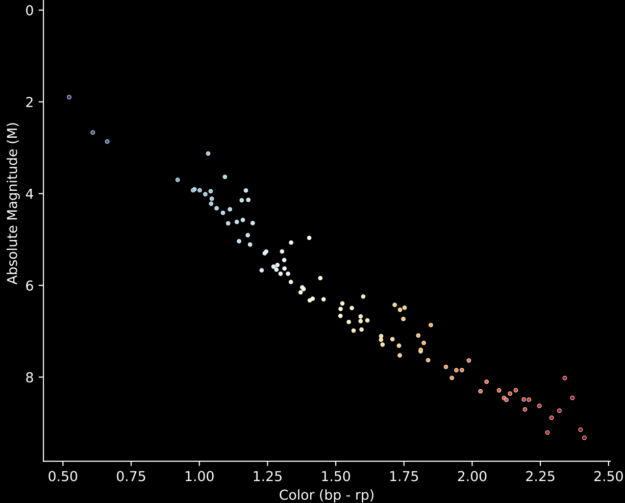
Gaia Cluster: [UPK_53] Stars (n= 98) Hertzsprung-Russel Diagram
