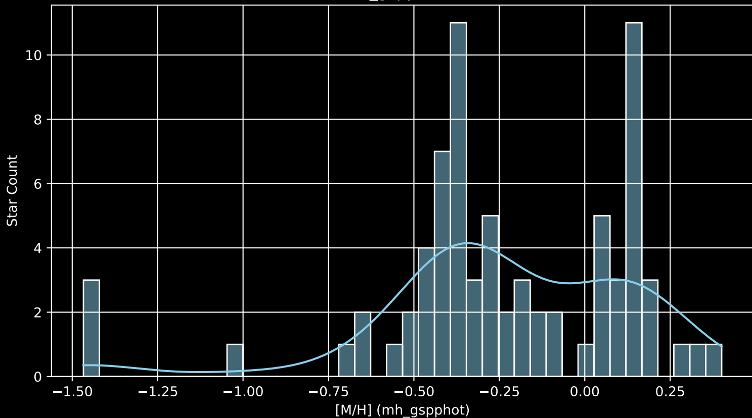
Gaia Cluster: [UPK_535 [M/H] (mh_gspphot) (n= 75)
