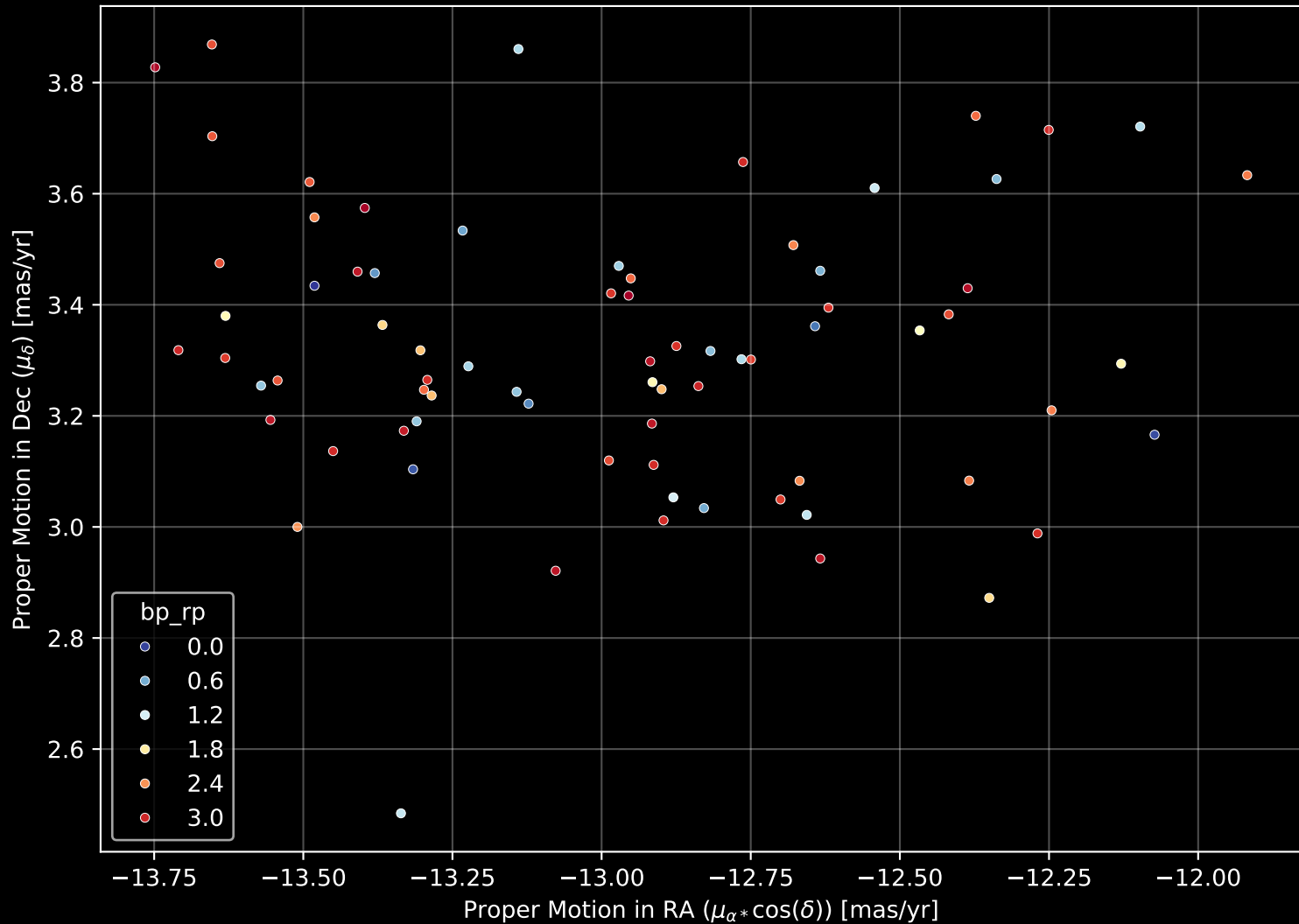
Gaia Cluster: [UPK_535] Proper Motion Diagram (n= 75)
