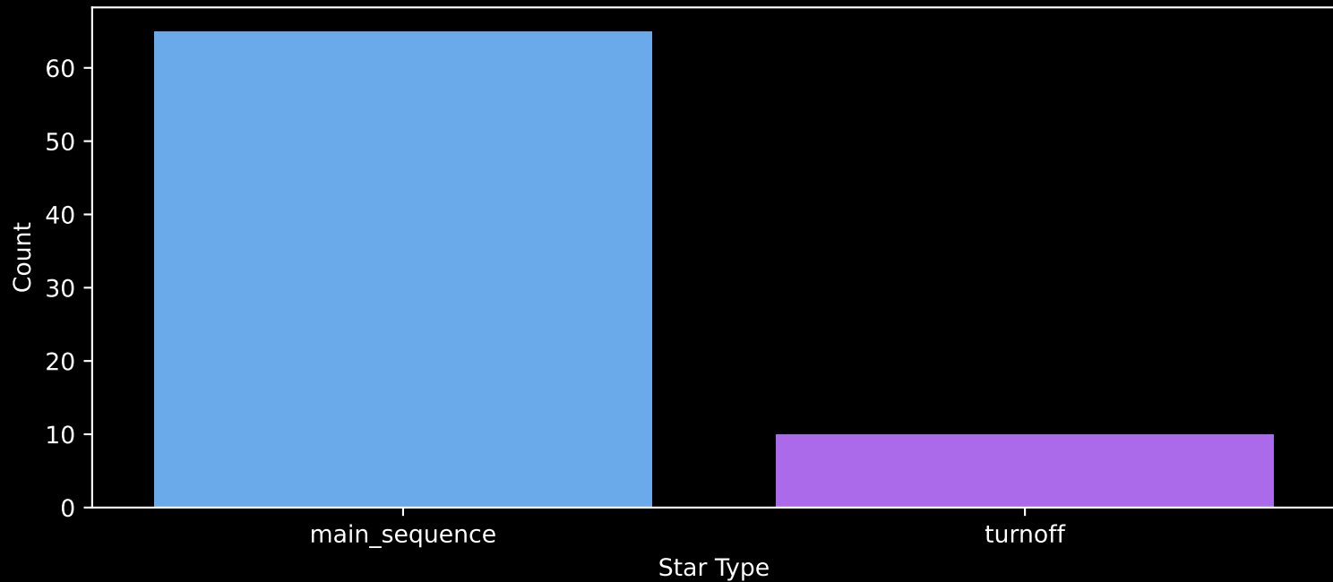
Gaia Cluster: [UPK_535] Count plot of Star Type
