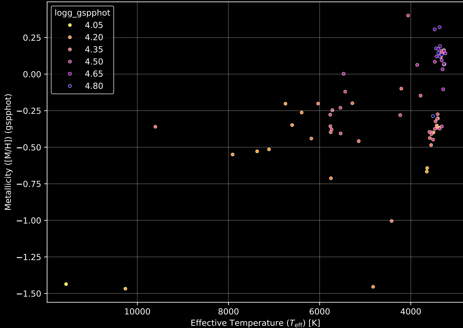
Gaia Cluster: [UPK_535] Stellar Population Parameters (n= 75)
