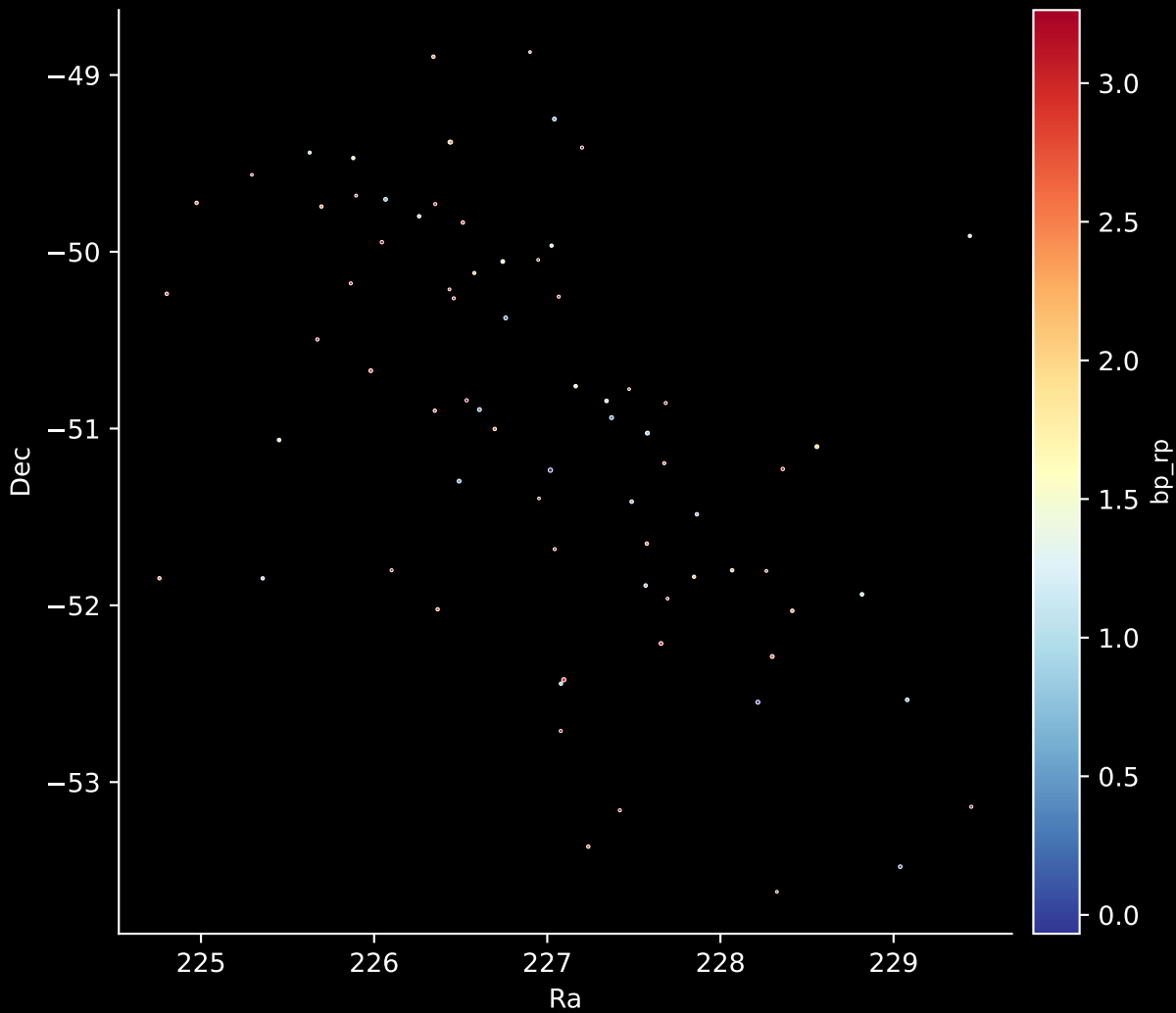
Gaia Cluster: [UPK_535] Stars: 75
