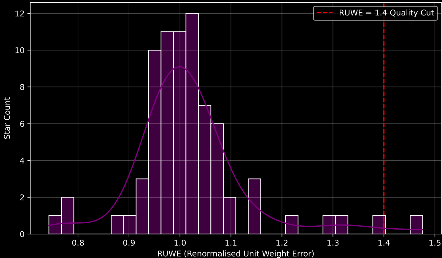
Gaia Cluster: [UPK_535] RUWE Distribution (n= 75)
