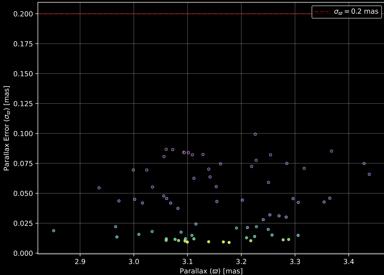
Gaia Cluster: [UPK_535] Parallax Quality (n= 75)
