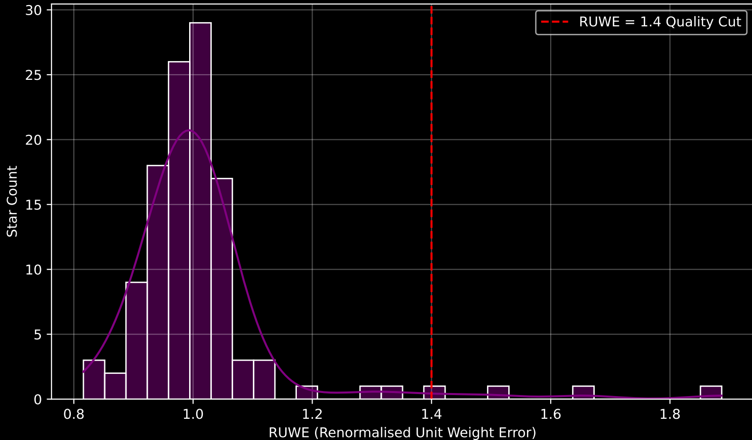
Gaia Cluster: [UPK_54] RUWE Distribution (n= 117)
