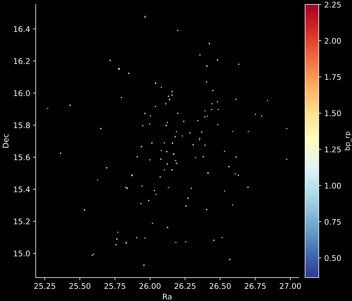
Gaia Cluster: [UPK_54] Stars: 119
