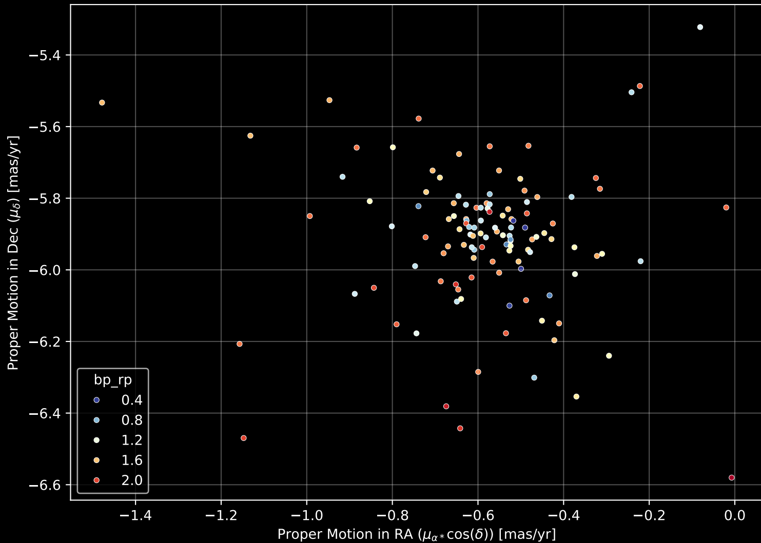
Gaia Cluster: [UPK_54] Proper Motion Diagram (n= 119)
