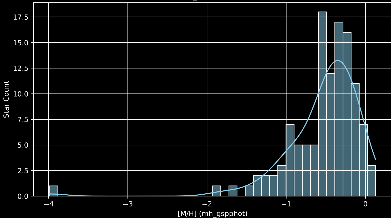
Gaia Cluster: [UPK_54 [M/H] (mh_gspphot) (n= 119)
