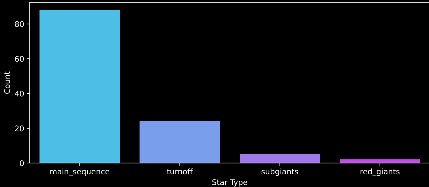
Gaia Cluster: [UPK_54] Count plot of Star Type
