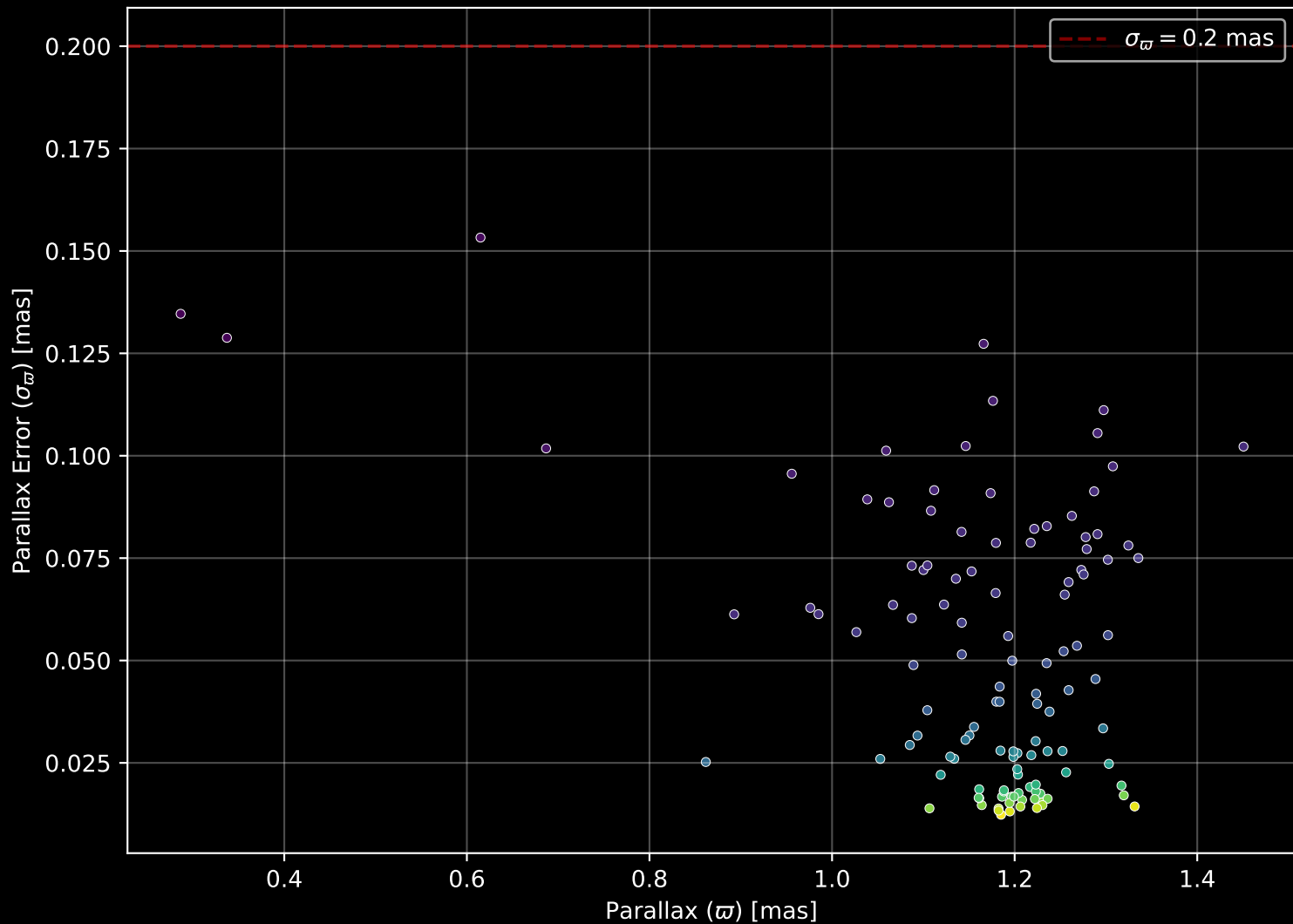
Gaia Cluster: [UPK_54] Parallax Quality (n= 119)
