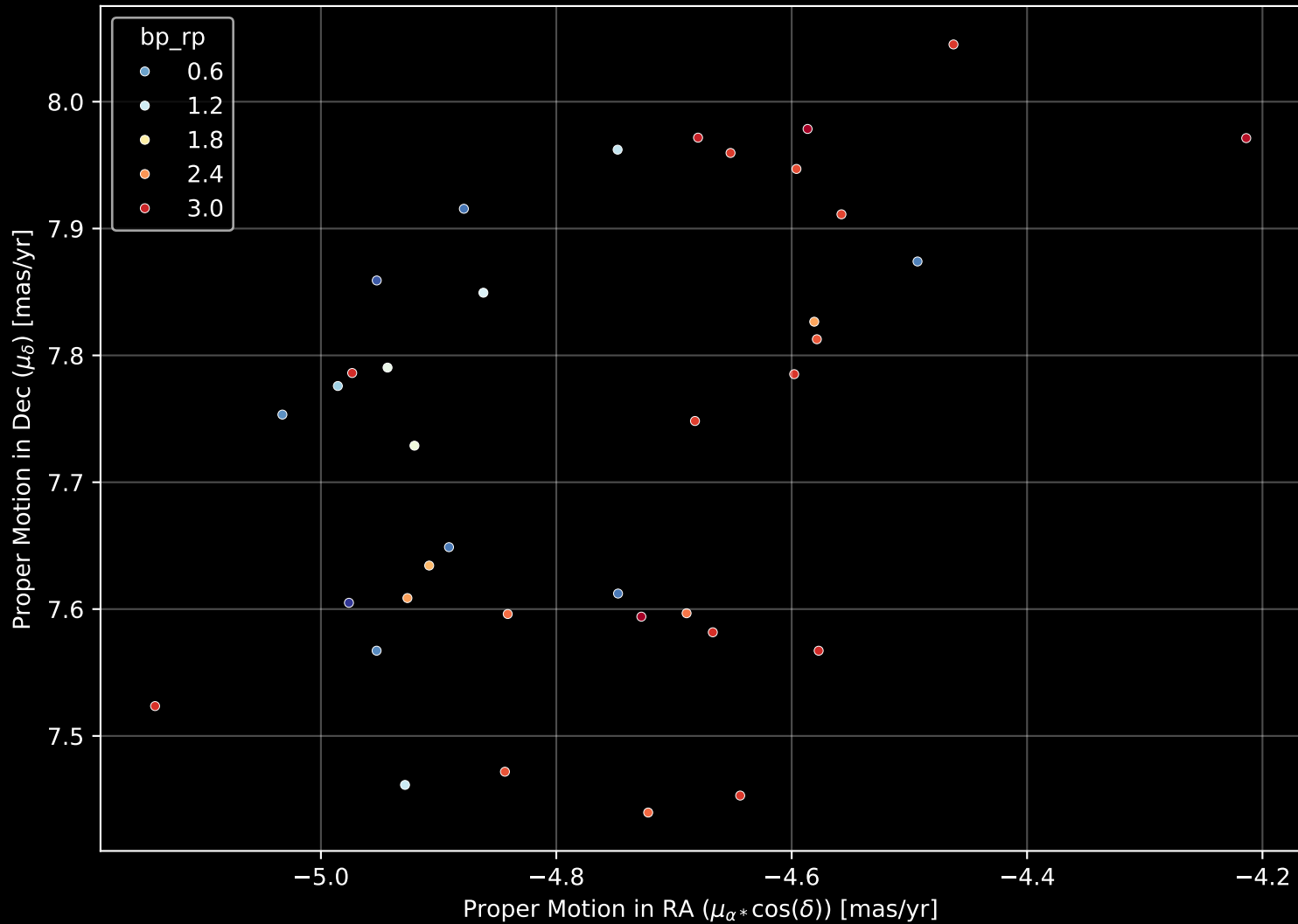
Gaia Cluster: [UPK_540] Proper Motion Diagram (n= 37)
