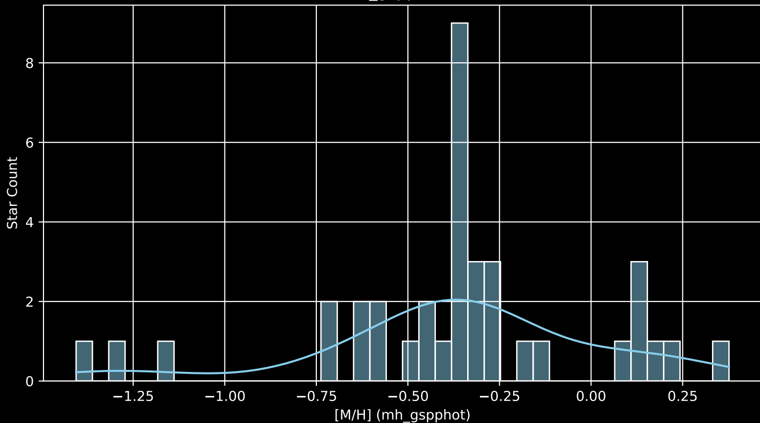
Gaia Cluster: [UPK_540 [M/H] (mh_gspphot) (n= 37)
