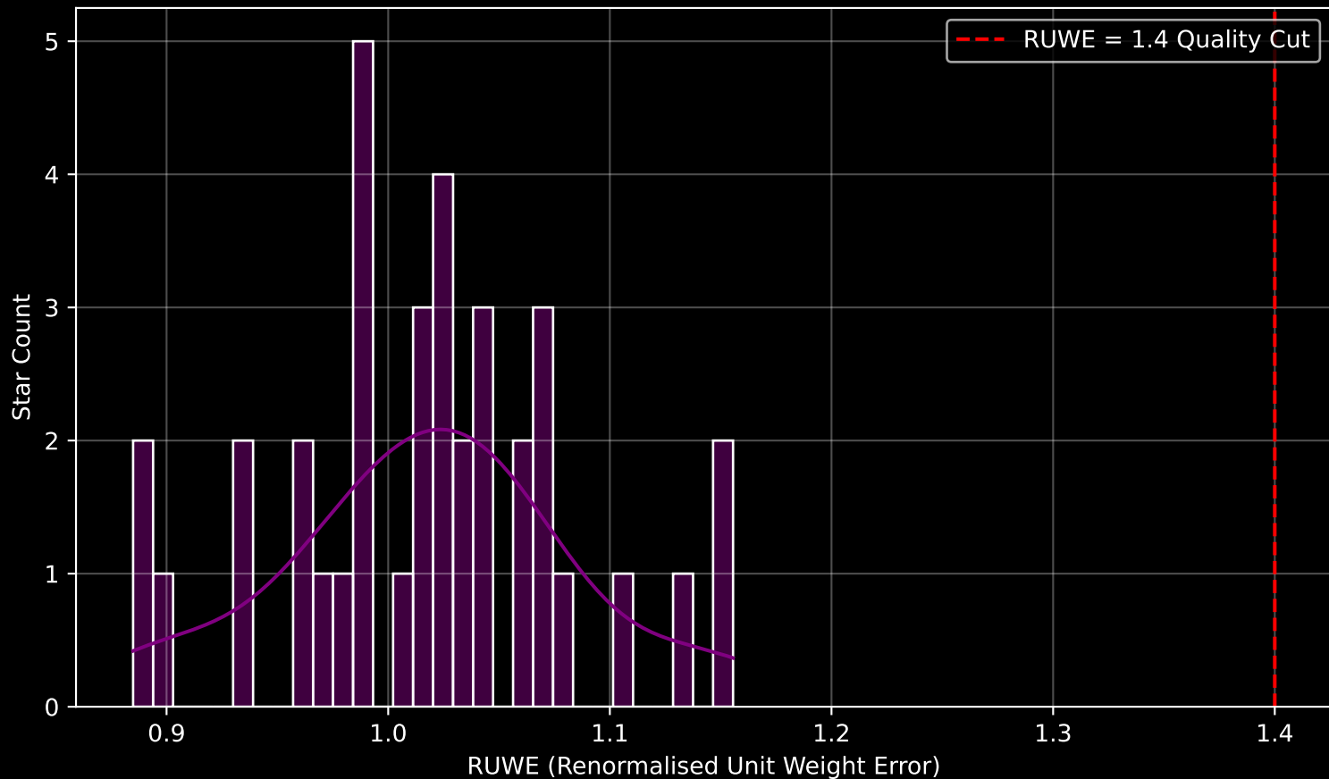
Gaia Cluster: [UPK_540] RUWE Distribution (n= 37)
