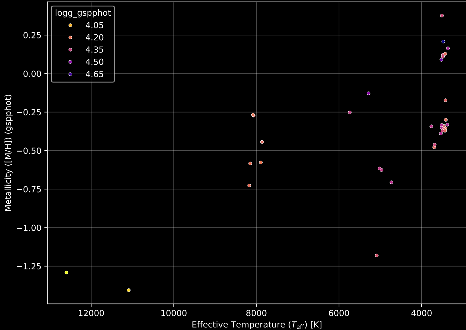
Gaia Cluster: [UPK_540] Stellar Population Parameters (n= 37)
