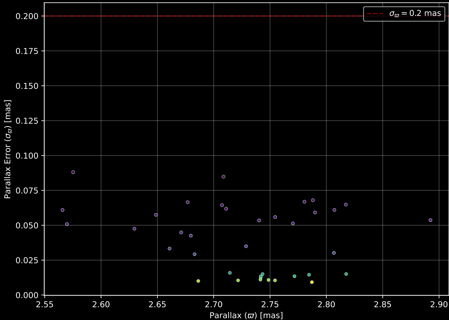
Gaia Cluster: [UPK_540] Parallax Quality (n= 37)
