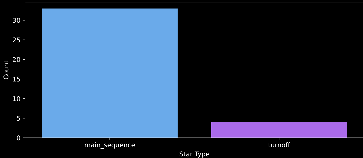
Gaia Cluster: [UPK_540] Count plot of Star Type
