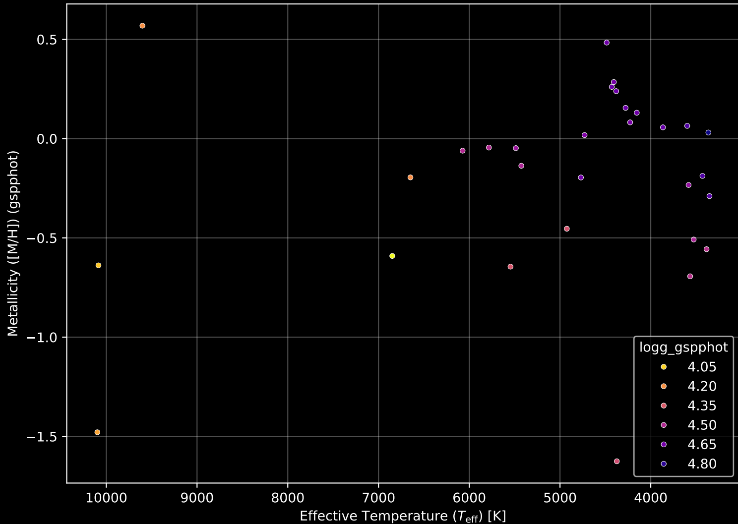
Gaia Cluster: [UPK_552] Stellar Population Parameters (n= 30)
