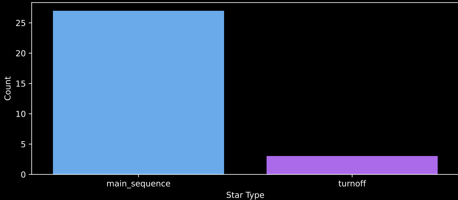
Gaia Cluster: [UPK_552] Count plot of Star Type
