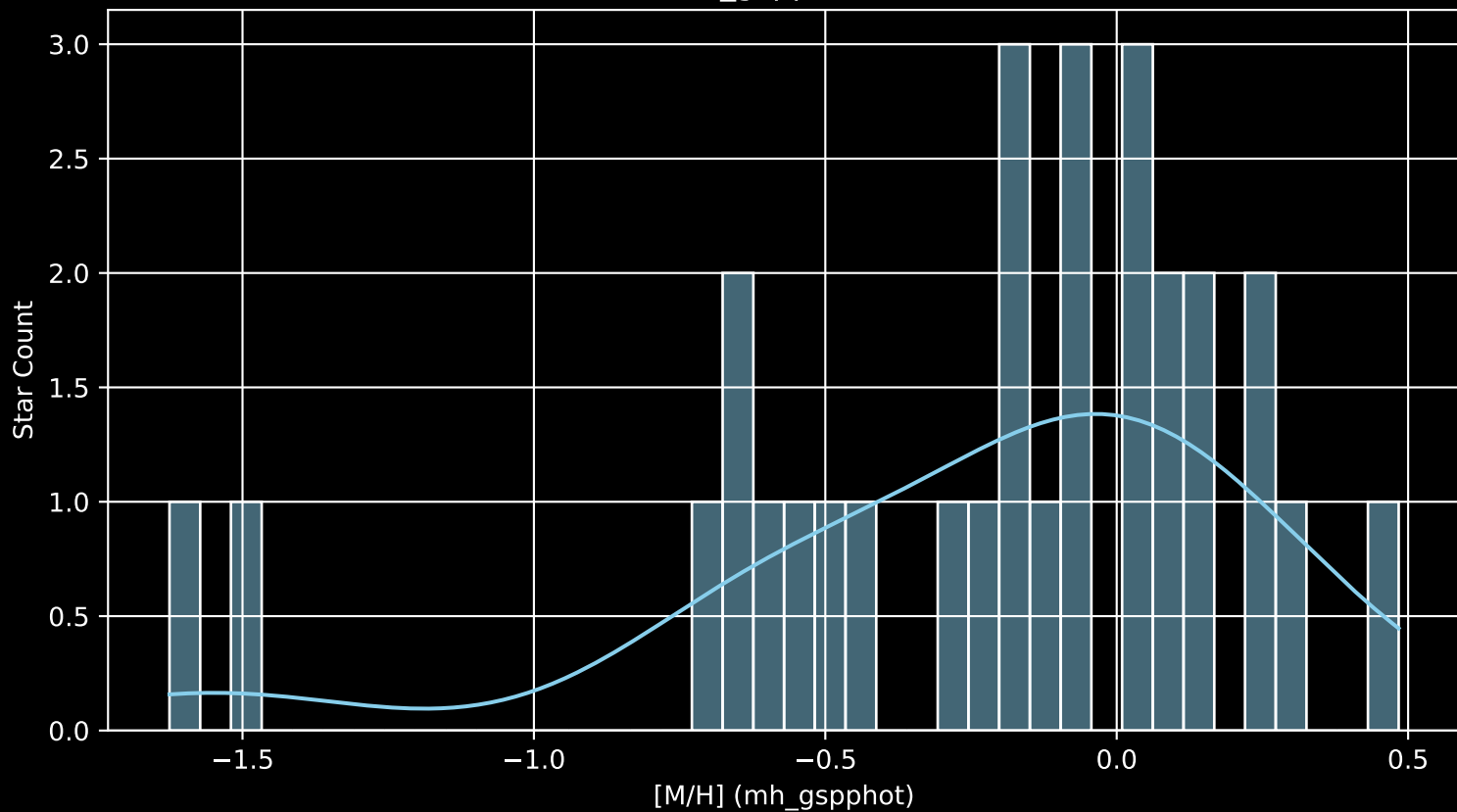
Gaia Cluster: [UPK_552 [M/H] (mh_gspphot) (n= 29)
