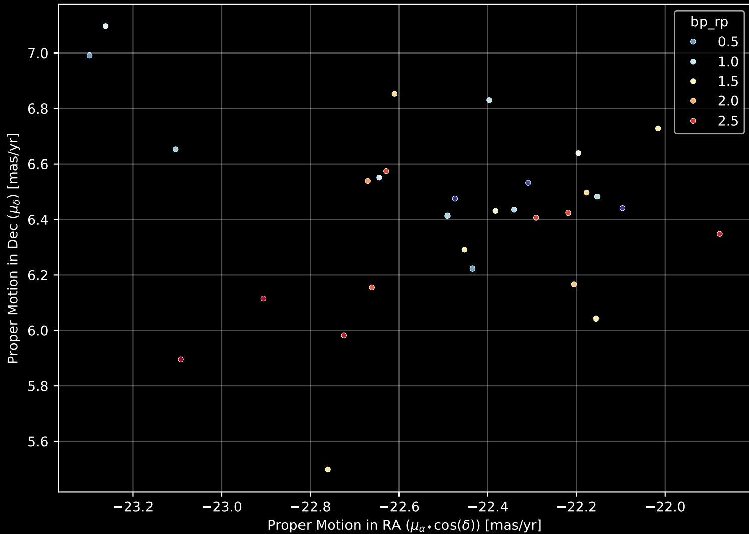
Gaia Cluster: [UPK_552] Proper Motion Diagram (n= 30)
