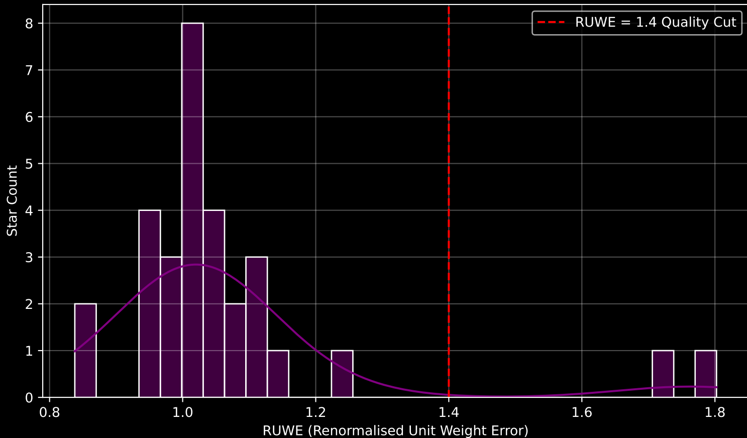
Gaia Cluster: [UPK_552] RUWE Distribution (n= 30)
