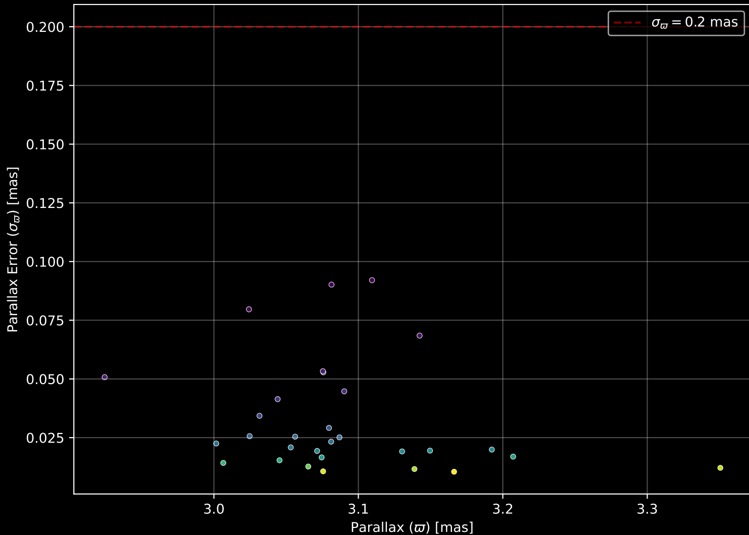
Gaia Cluster: [UPK_552] Parallax Quality (n= 30)
