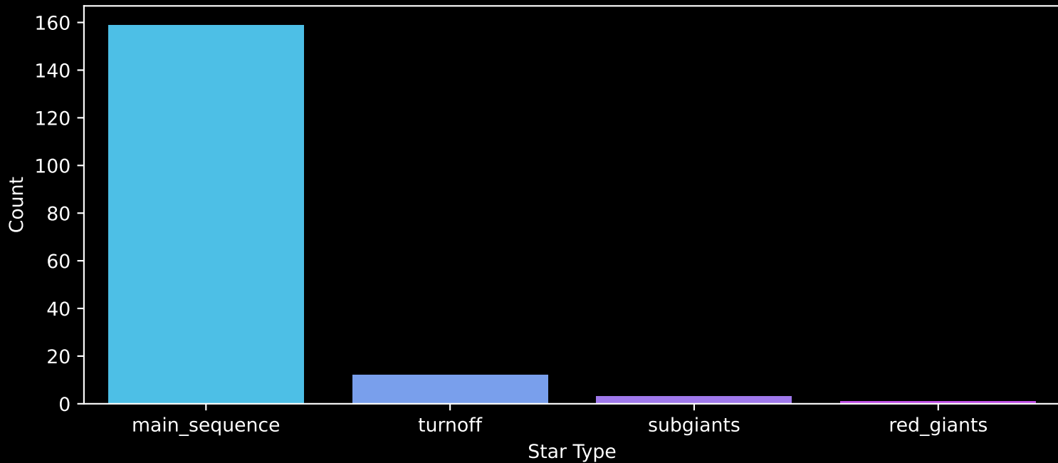
Gaia Cluster: [UPK_560] Count plot of Star Type
