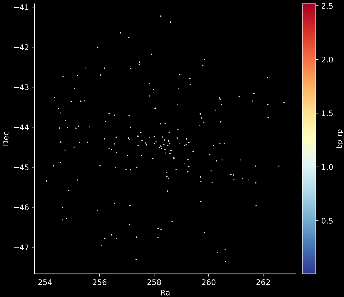
Gaia Cluster: [UPK_560] Stars: 175
