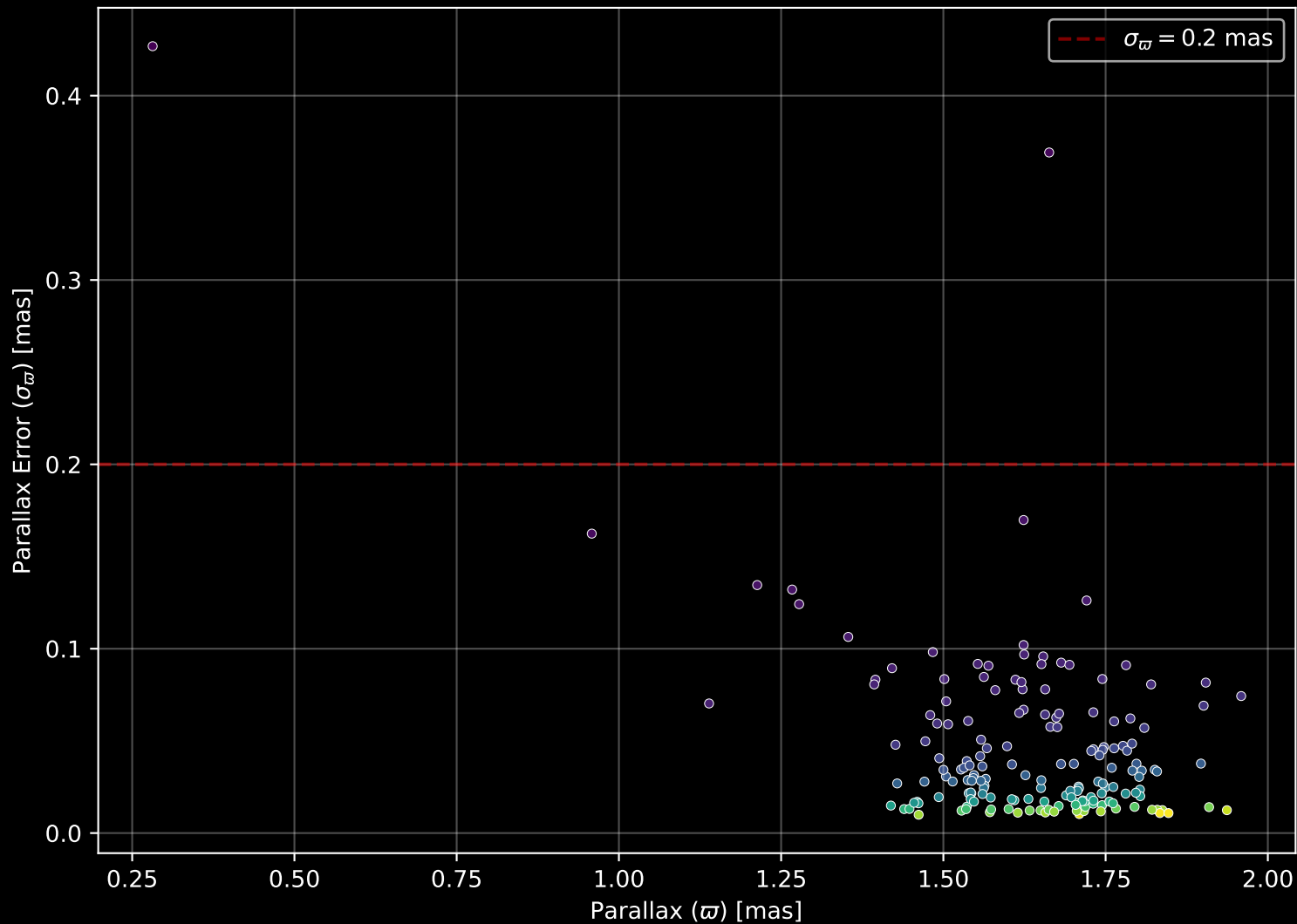
Gaia Cluster: [UPK_560] Parallax Quality (n= 175)
