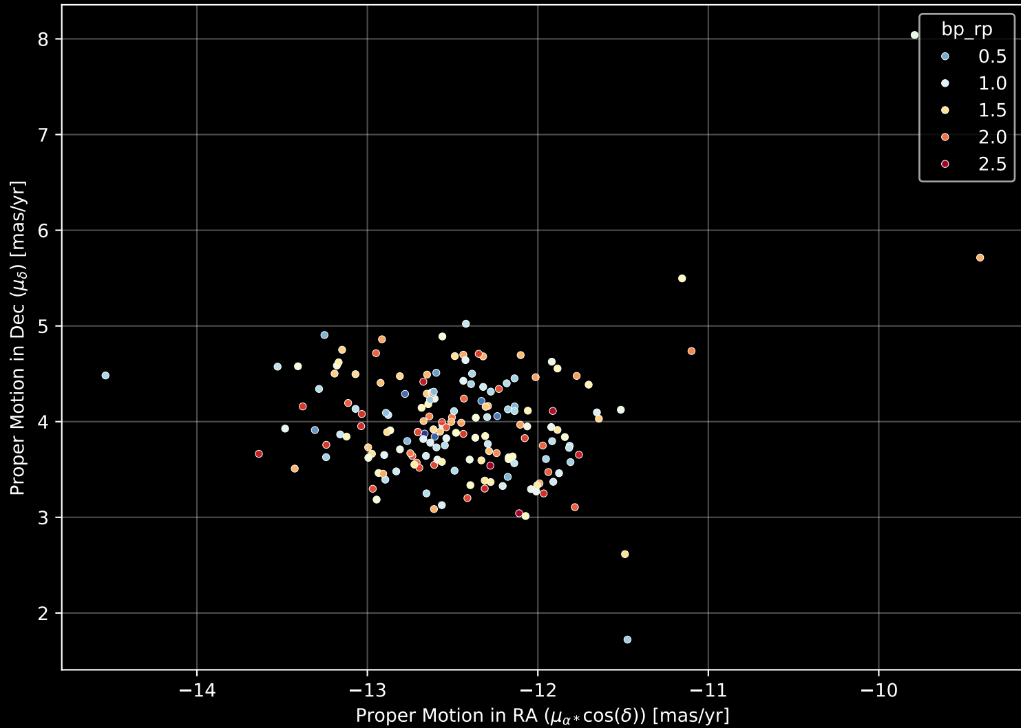
Gaia Cluster: [UPK_560] Proper Motion Diagram (n= 175)
