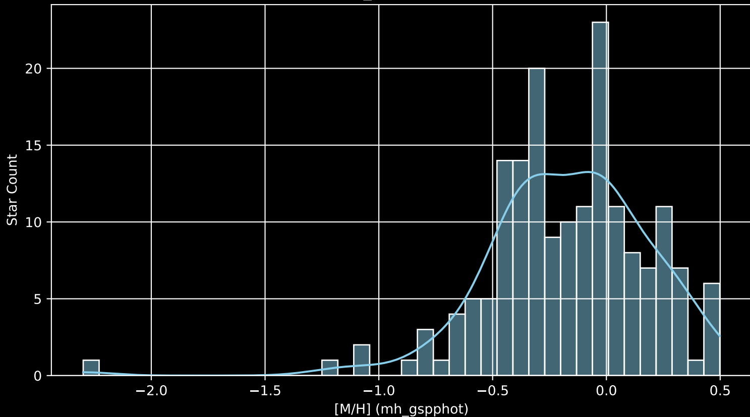
Gaia Cluster: [UPK_560 [M/H] (mh_gspphot) (n= 175)
