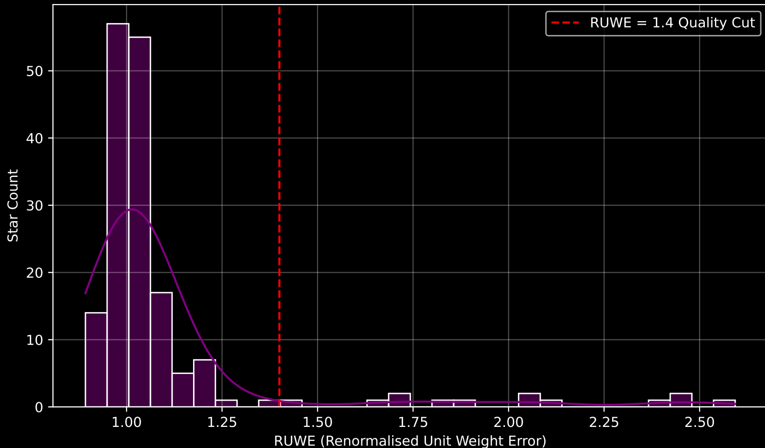
Gaia Cluster: [UPK_560] RUWE Distribution (n= 170)
