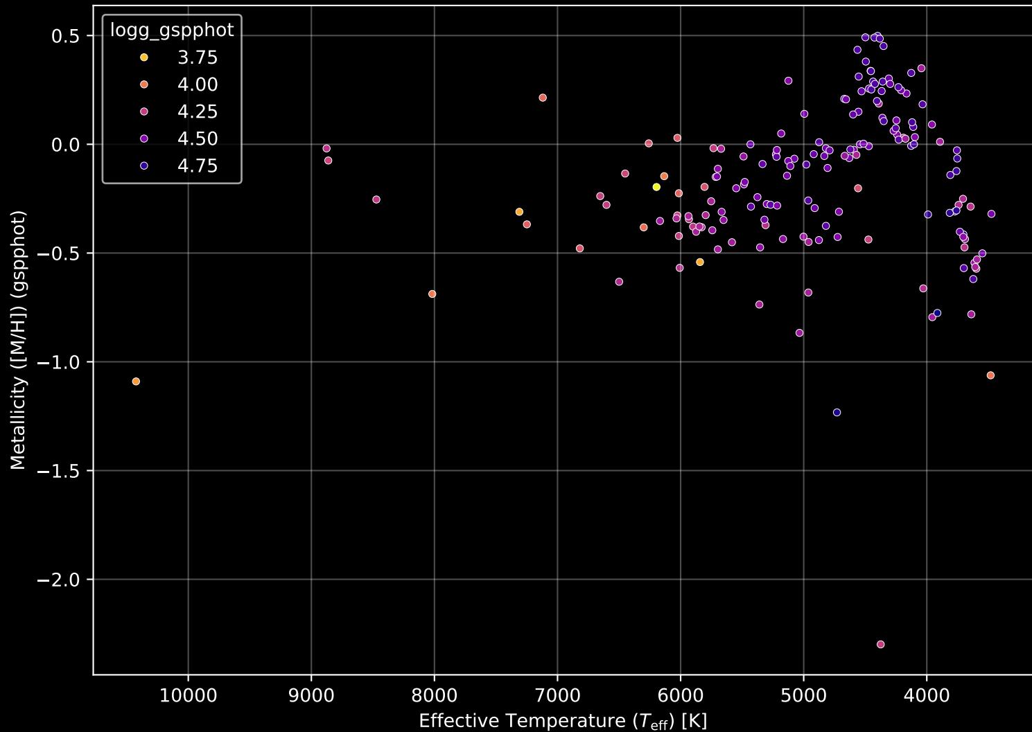
Gaia Cluster: [UPK_560] Stellar Population Parameters (n= 175)
