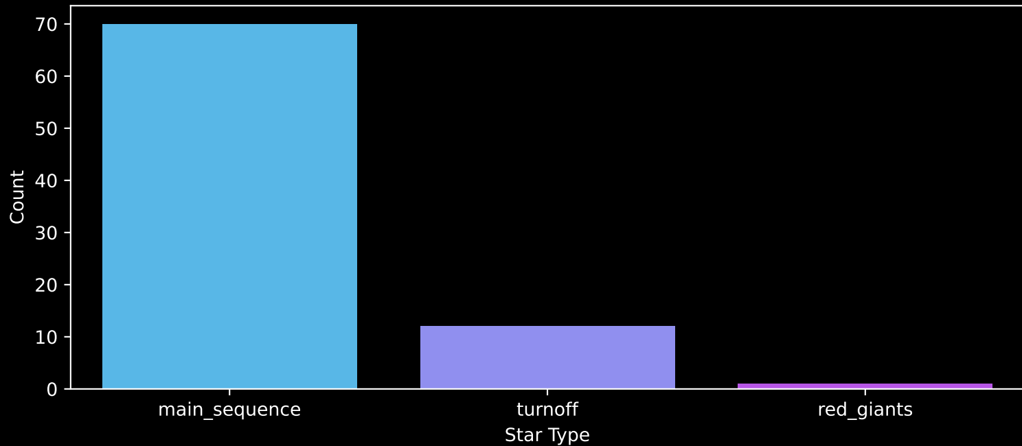
Gaia Cluster: [UPK_567] Count plot of Star Type
