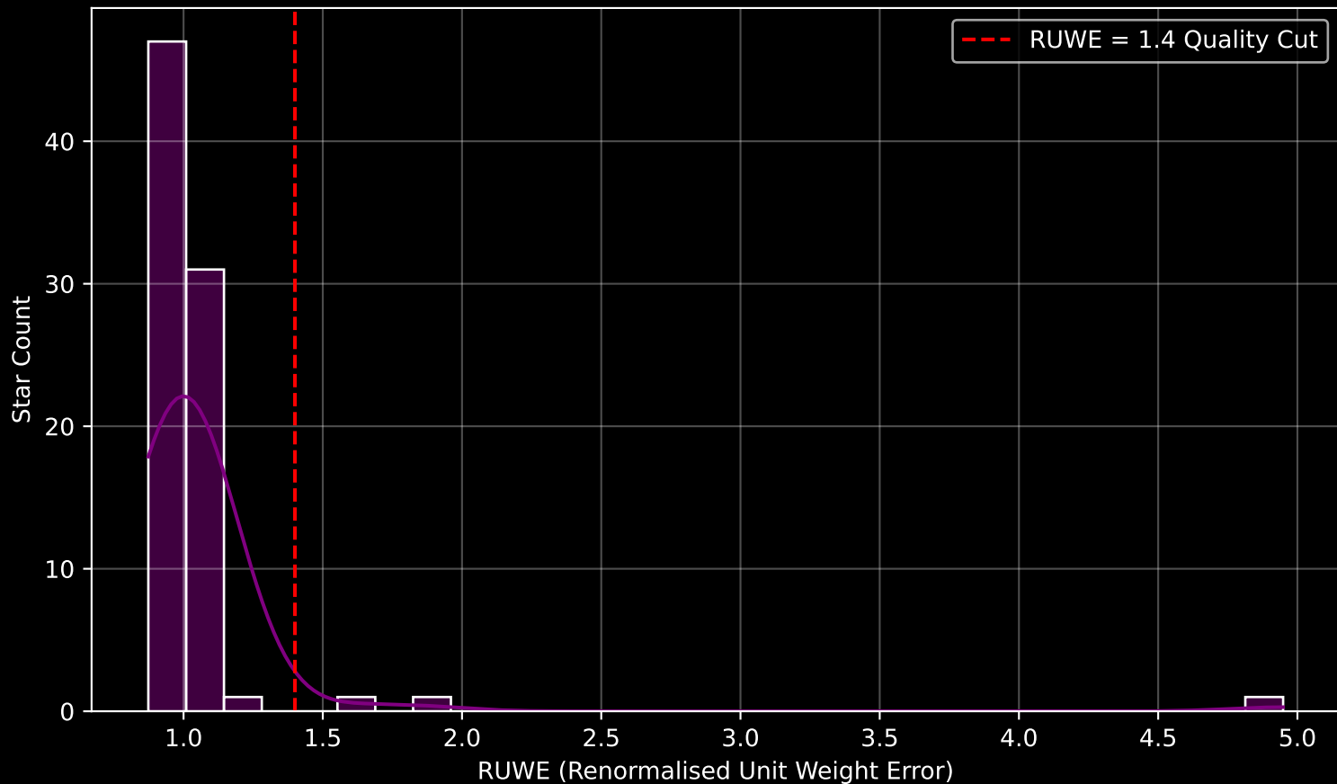
Gaia Cluster: [UPK_567] RUWE Distribution (n= 82)
