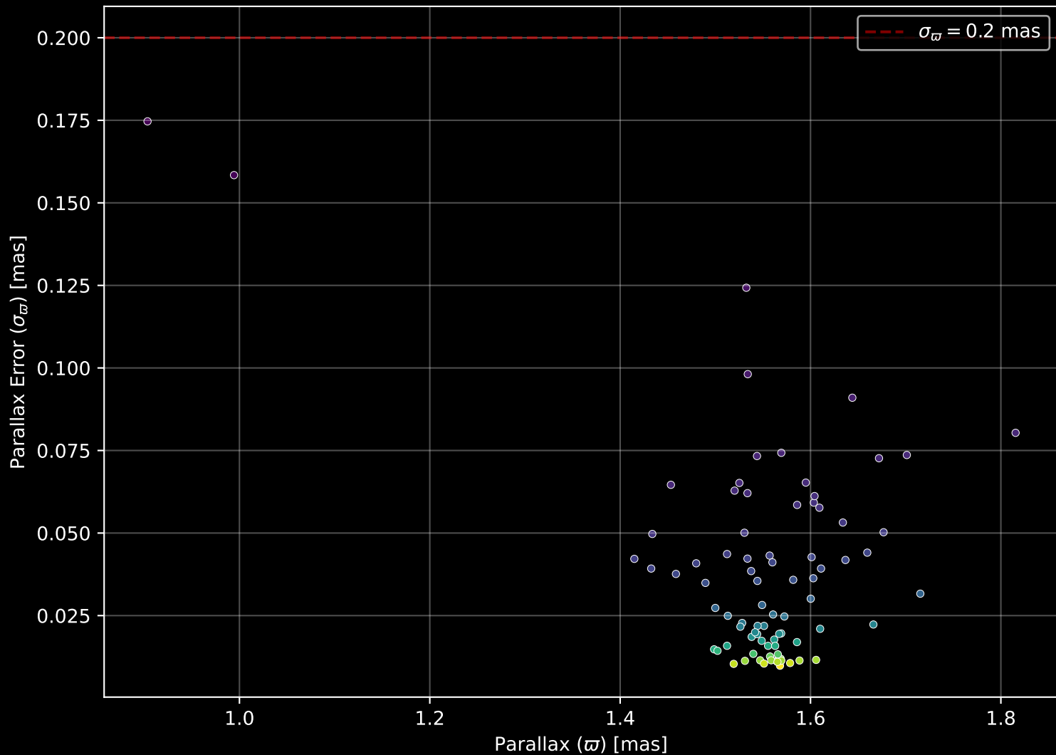
Gaia Cluster: [UPK_567] Parallax Quality (n= 83)
