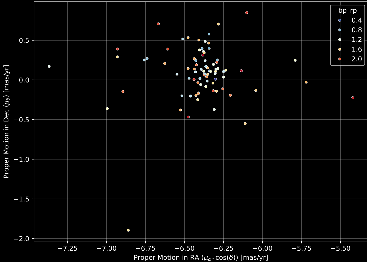
Gaia Cluster: [UPK_567] Proper Motion Diagram (n= 83)
