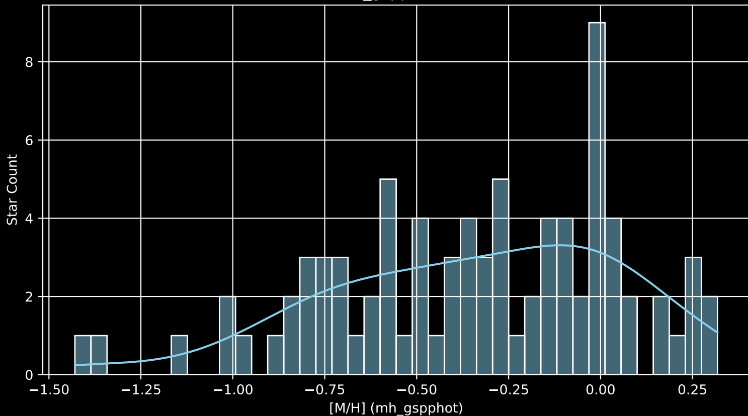
Gaia Cluster: [UPK_567 [M/H] (mh_gspphot) (n= 83)
